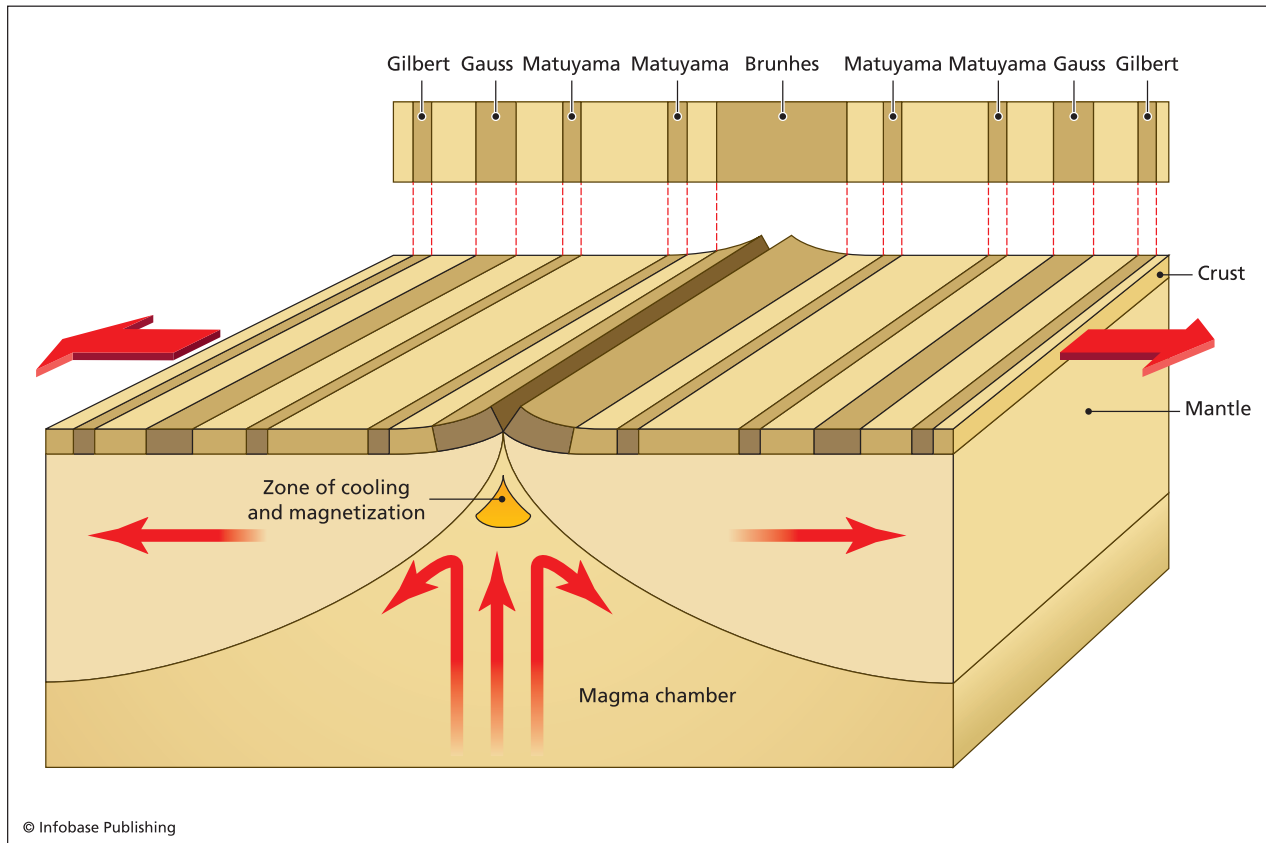
Symmetric magnetic anomalies produced by conveyor-belt style production of oceanic crust in an alternating magnetic field. The magnetic polarity timescale, above, is constructed by dating rocks with different magnetizations.
