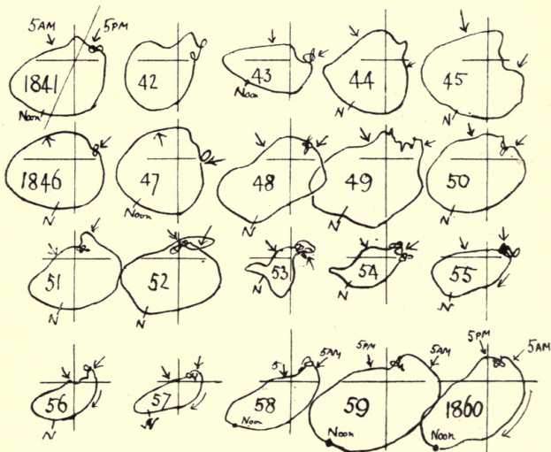
GREENWICH MAGNETIC CURVES FOR APRIL 1841-1860
