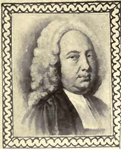
1742 BRADLEY. 1764
