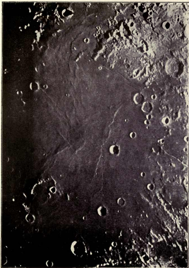
MARE TRANQUILLITATIS AND SURROUNDINGS
