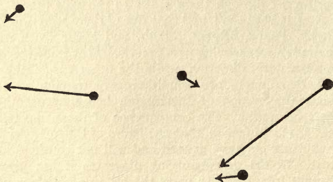
CASSIOPEIA AT PRESENT
