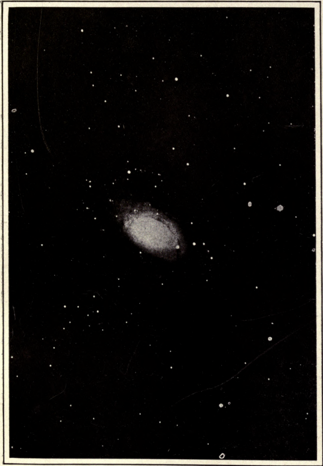
SPIRAL IN URSA MAJOR
