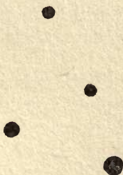
THE "SOUTHERN CROSS" AS IT ONCE WAS
