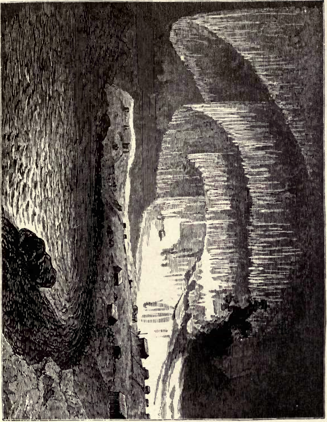
AURORAL ARCHES SEEN IN SCANDINAVIA
