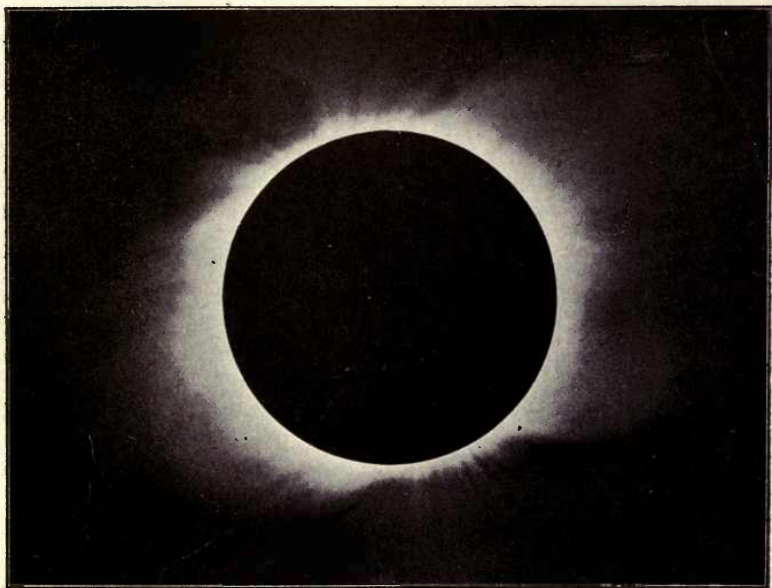
THE CORONA
