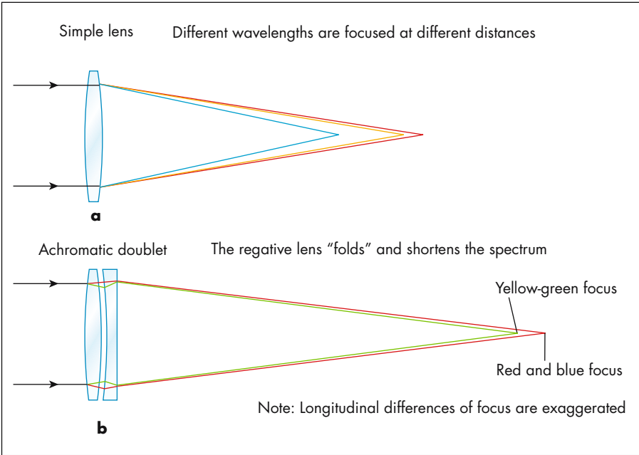
Figure 2.20. Chromatic aberration.
