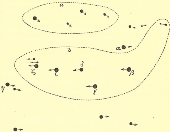
FIG. 6.—Observed Proper Motions of Stars in Ursa Major and Neighborhood.
