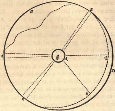
FIG. 2.—The Galactic Cloven Flat Ring (plan).
