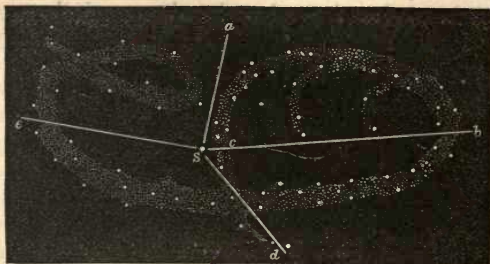
FIG. 5.—The Milky Way regarded as a Spiral.
