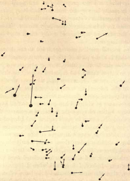
Drift of the Stars in the Constellations Cancer and Gemini.
