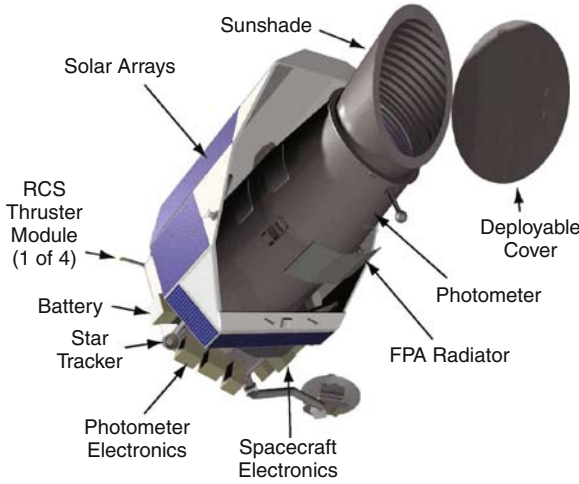
Fig. 8.12 Functional diagram of Kepler (NASA)
