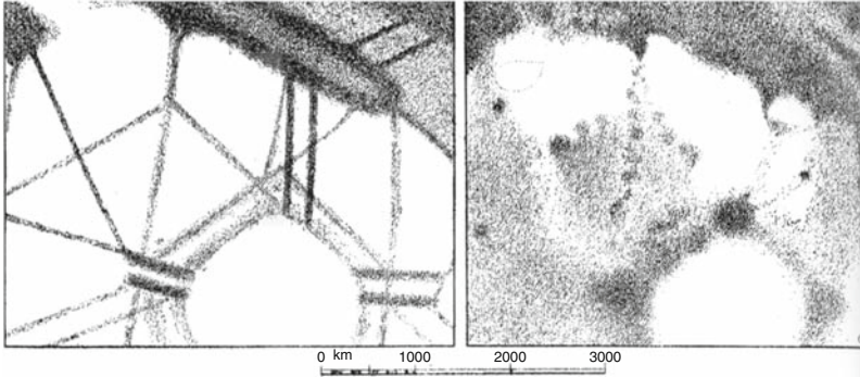
Fig. 9.15 The region of Elysium Planitia on Mars, as drawn by Schiaparelli between 1877 and 1890 ( left ) and by Antoniadi between 1909 and 1926 ( right ). Antoniadi's drawings showed that the quasi-linear structures seen by Schiaparelli were nothing like that when spatial resolution was increased (After Antoniadi, La planète Mars , 1930)
