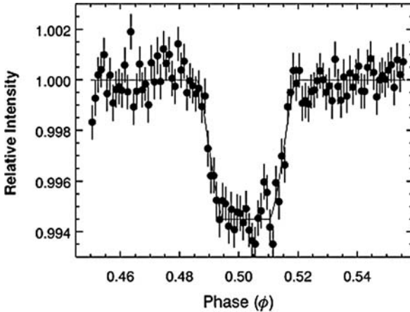
Fig. 7.14 Secondary transit of HD 189733b (the passage of the planet behind the star), observed by Spitzer/IRS in a band at 16\mu\text{m} . The Spitzer space observatory has been able to detect the thermal emission from Pegasids during their secondary transits. The flux of the system star + planet decreases when the planet passes behind the star. The difference in the flux before and after, and during the transit therefore gives the thermal emission from the day side of the planet (After Deming et al., 2006)
