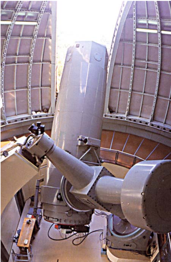
Fig. 1.7 The 193-cm telescope at the Observatoire de Haute Provence. Equipped with the high-resolution Elodie spectrograph, it enabled the first exoplanet orbiting a solar-type star, 51 Peg, to be discovered in 1995
