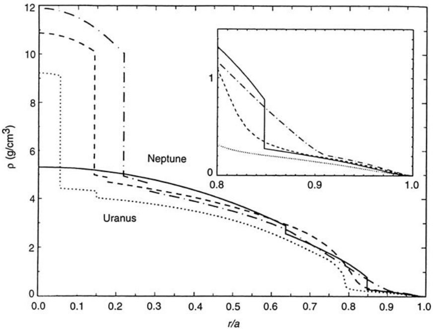
Fig. 7.4 Examples of models of the internal structure of Uranus ( dotted line ) and Neptune (3 models, continuous , chain-dotted and dashed lines ). In the case of Neptune, the size of the central core is poorly constrained (After Marley, 1999)
