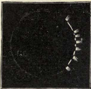
FIG. 8.—Brushes of light.
