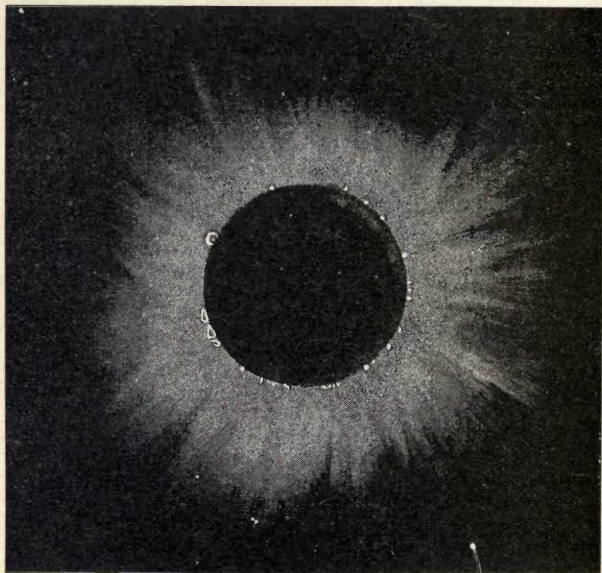
FIG. 10.—Corona of 1882. (Sun-spot maximum.)
