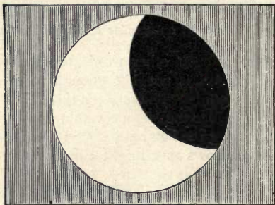
FIG. 5.—Partial eclipse of the Sun.
