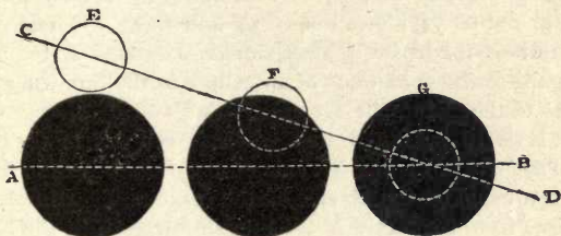
FIG. 14.—Conditions of eclipses of the Moon.
