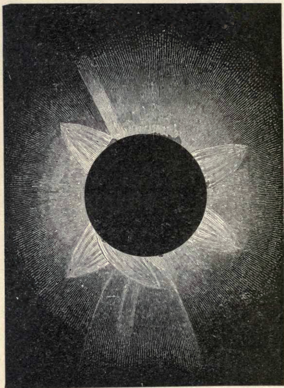
THE TOTAL ECLIPSE OF THE SUN, Sept. 7, 1858 ( Liais ).
