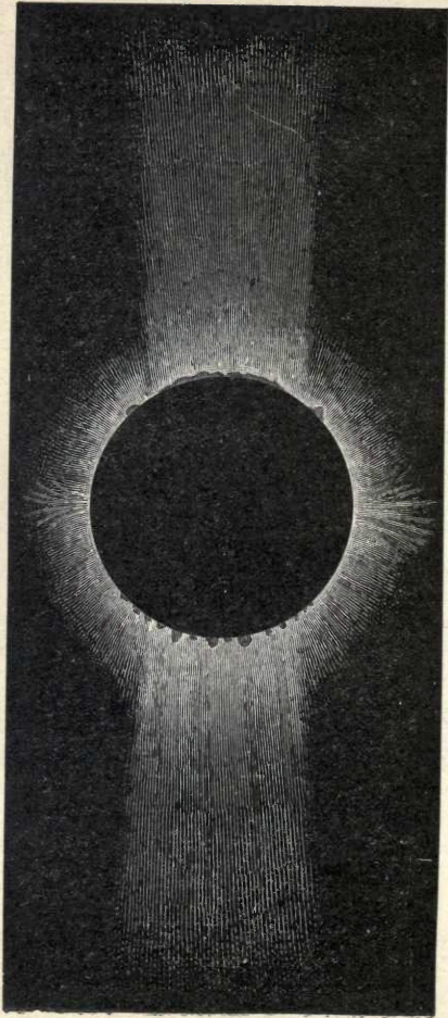
FIG. 11.—Corona of 1867. (Sun-spot minimum.)
