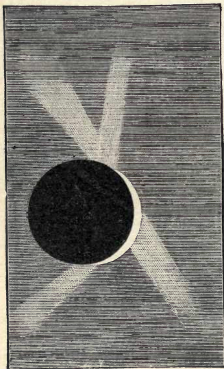
FIG. 7.—Rays of light seen near the time of totality.
