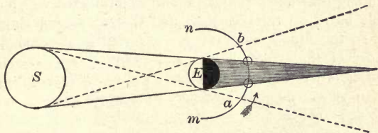
FIG. 13.—Theory of an eclipse of the Moon.
