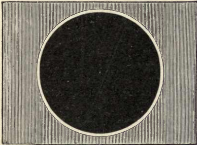
FIG. 4.—Annular eclipse of the Sun.
