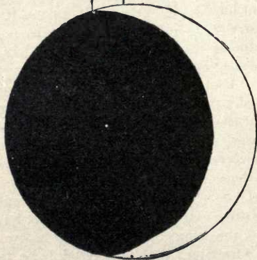
FIG. 12.—Solar eclipse at Jerusalem, 11th January, B. C. 689.
