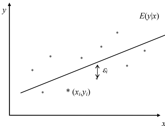
Figure 7.1 Linear regression. Dots represent real observations (x_i, y_i) . The line E(y|x) shows the expected value of dependent variable. The errors \varepsilon_i are the deviation of the observations from their expected values
