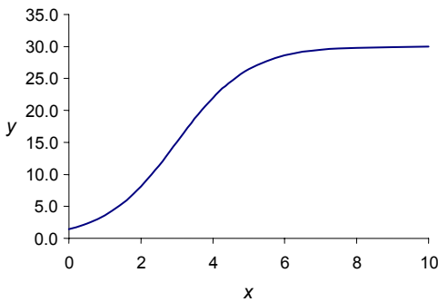
Figure 10.3 Logistic function with the parameters: \beta_0 = 30 , \beta_1 = 20 , and \beta_2 = -1
