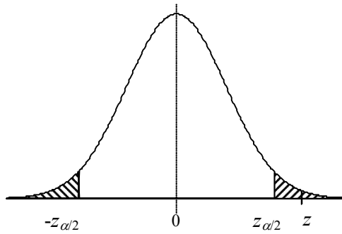
Figure 6.3 The calculated z is in the critical region and H_0 is rejected with an \alpha level of significance. The probability that the calculated z belongs to the H_0 population is less than \alpha
