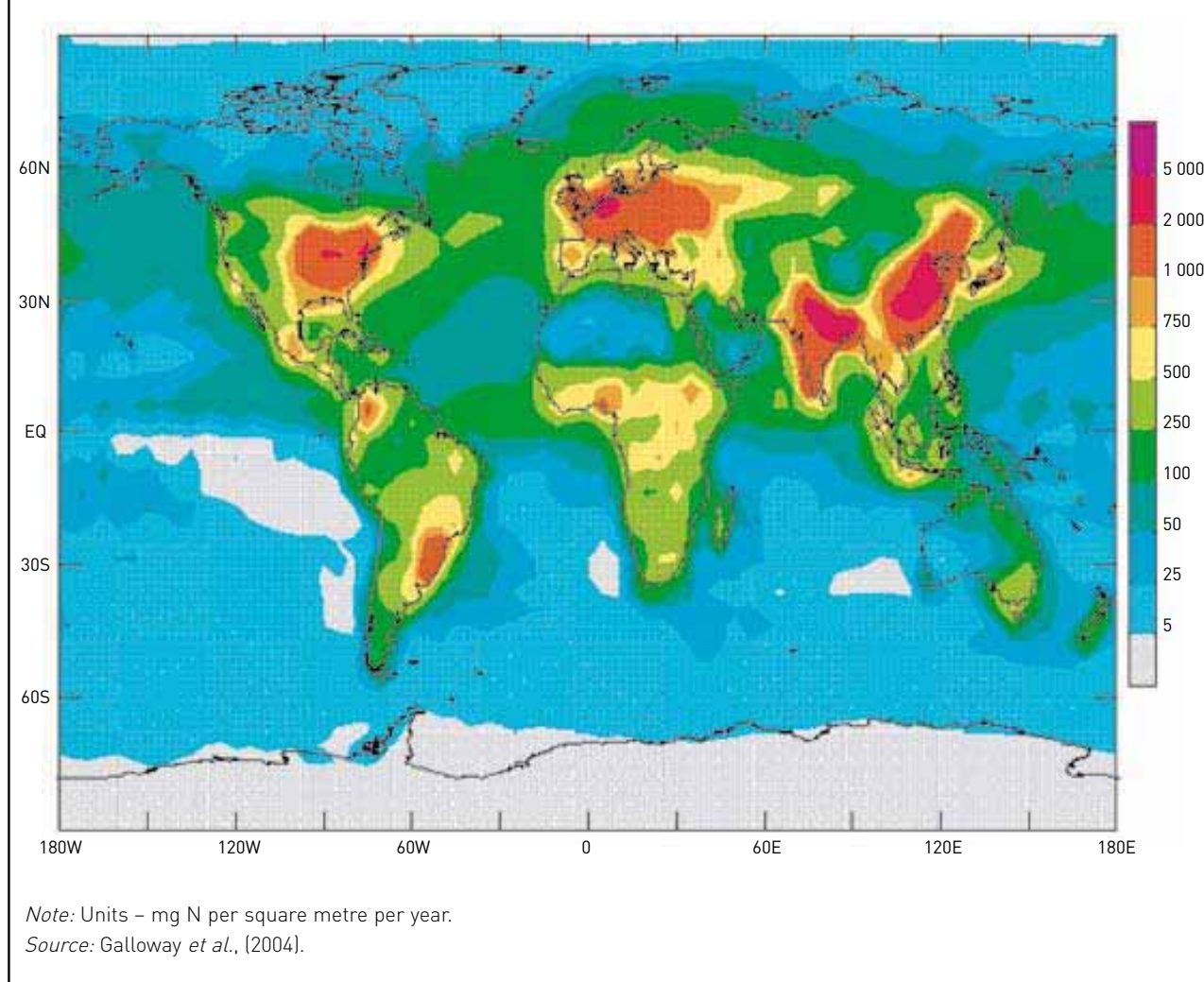
Figure 3.3 Spatial pattern of total inorganic nitrogen deposition in the early 1990s
