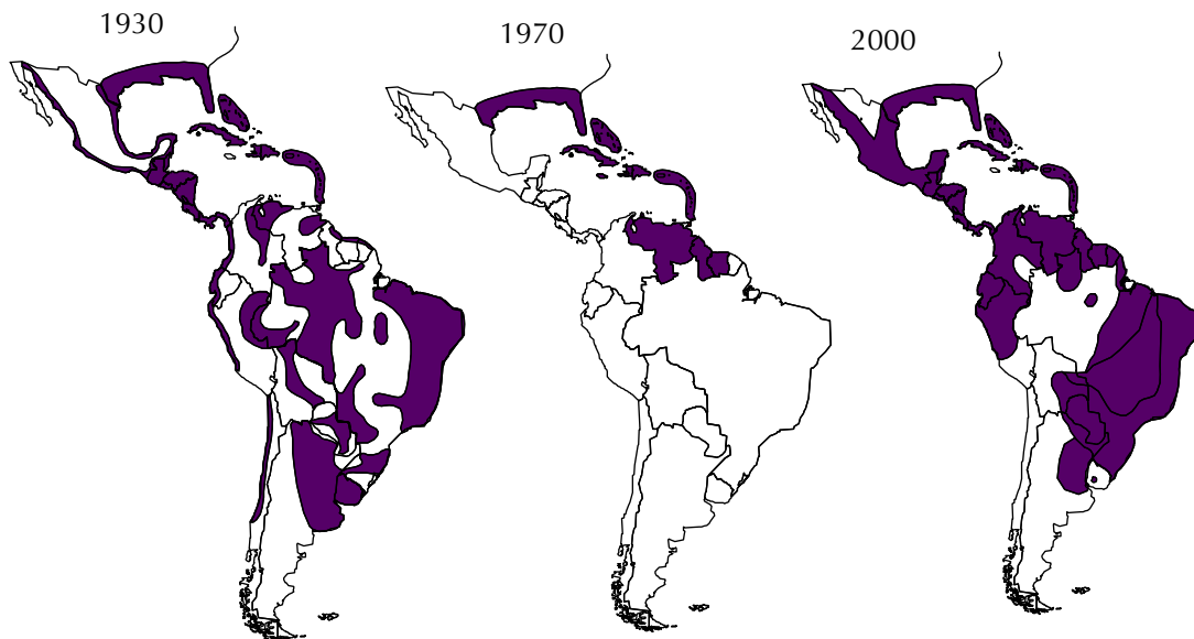
FIGURE 2. Changes in the distribution of Aedes aegypti in the Americas, 1930–2000.
