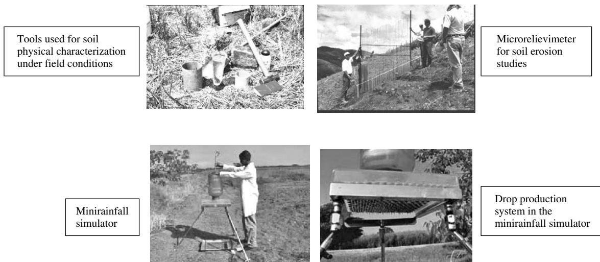
Figure 12. Field tools developed by CIAT to assess soil degradation in hillside areas.
