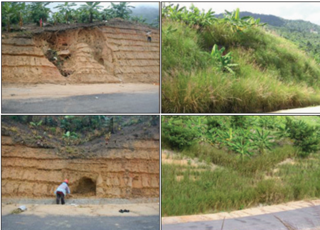
Photo 22: Pham Hong Duc Phuoc, a road protection project in Khanh Hoa province, road to Hon Ba): left two photos: severe erosion on newly built batter occurs after only a few rains; right two photos: eight months after vetiver planting: Vetiver stabilized this slope, totally stopping and preventing further erosion during the next wet season.
