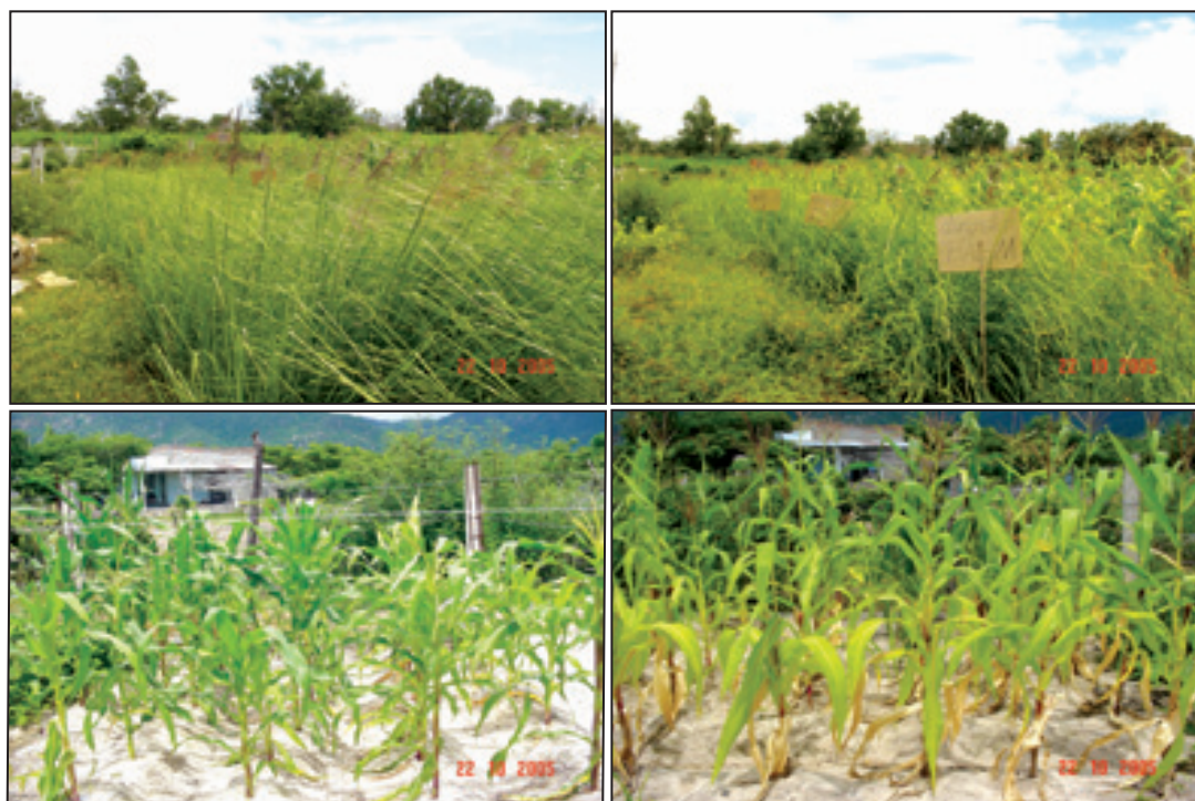
Photo 17: Vetiver roots penetrated compacted gypsum barrier to tap ground water.
