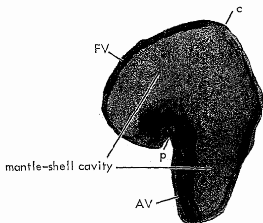
FIG. E228. Sellaea sp. (Caprotinidae), L.Cret. (Alb.), USA (Texas); long. sec. both valves showing mantle-shell cavity open without tabulae ( p-c ; commissural plane), \times 0.7 (Perkins, n).
