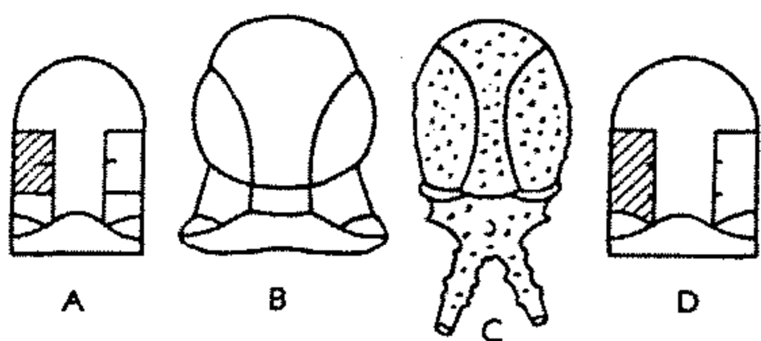
FIG. 34. Composite lateral glabellar lobes in the Lichidae.— A, B . Bicomposite lobes ( Dicranopeltis ); shaded area in schematic interpretation ( A ) represents bicomposite lateral lobe resulting from fusion of 1st ( 4p ) and 2nd ( 3p ) lateral glabellar lobes.— C, D . Tricomposite lobes ( Hoplolichas ); shaded area in schematic interpretation ( D ) represents tricomposite lateral lobe resulting from fusion of 1st ( 4p ), 2nd ( 3p ), and 3rd ( 2p ) lateral glabellar lobes.
