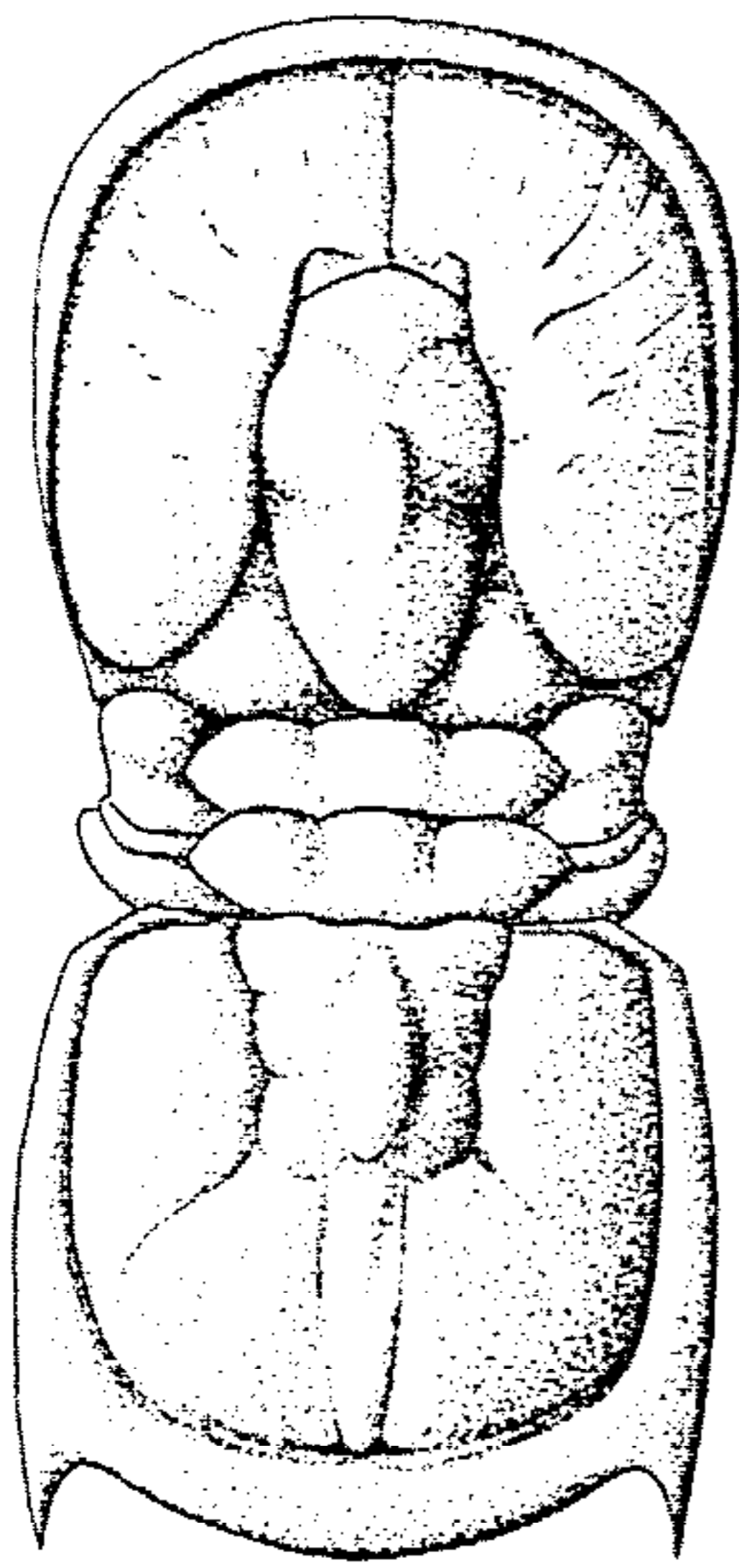
FIG. 121. * Machairagnostus tmectus HARRINGTON & LEANZA (Pseudagnostidae), L.Ord., Arg., \times 18.5 (59*, 1957).
