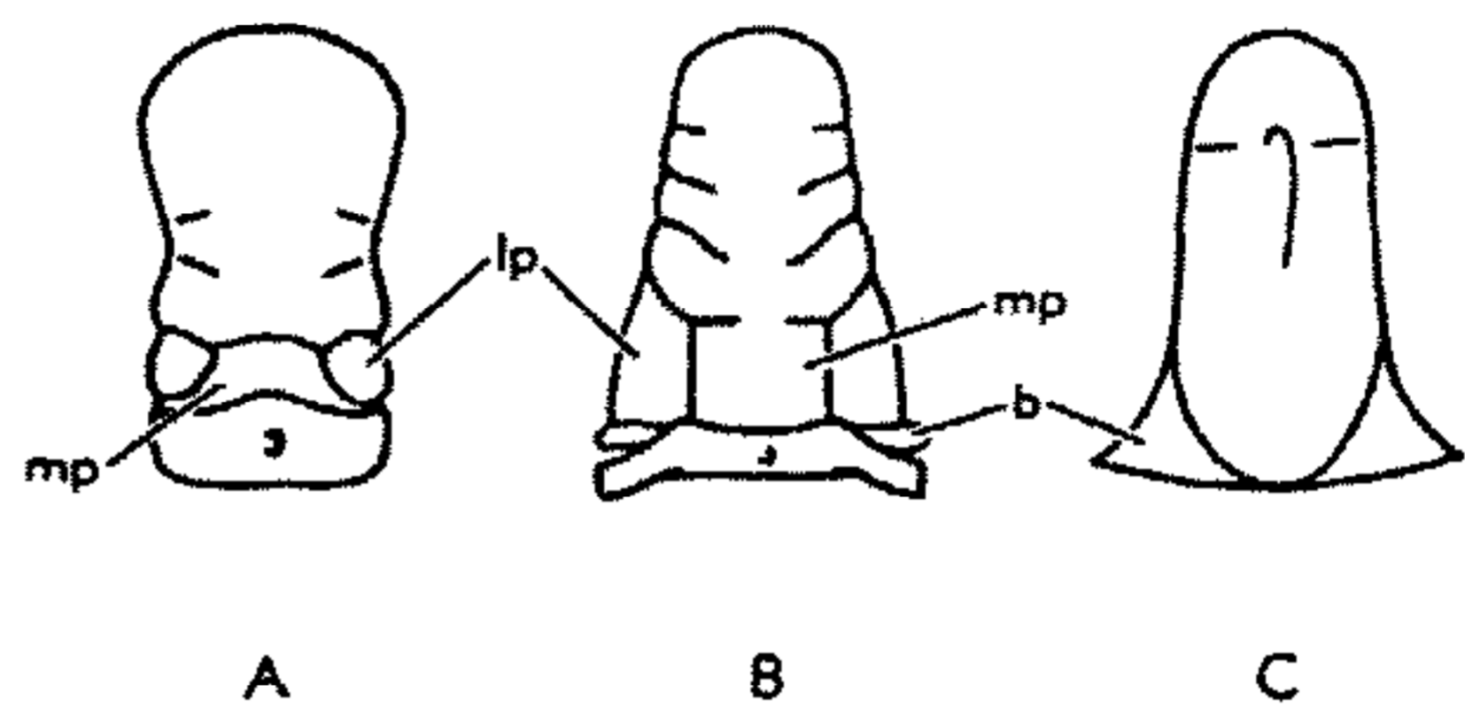
FIG. 35. Preoccipital and basal glabellar lobes. A , Ditomopyge ; B , Schizoproetus ; C , Geragnostus . (Explanation: bl , basal lobes; mp , median preoccipital lobes; lp , lateral preoccipital lobes).
