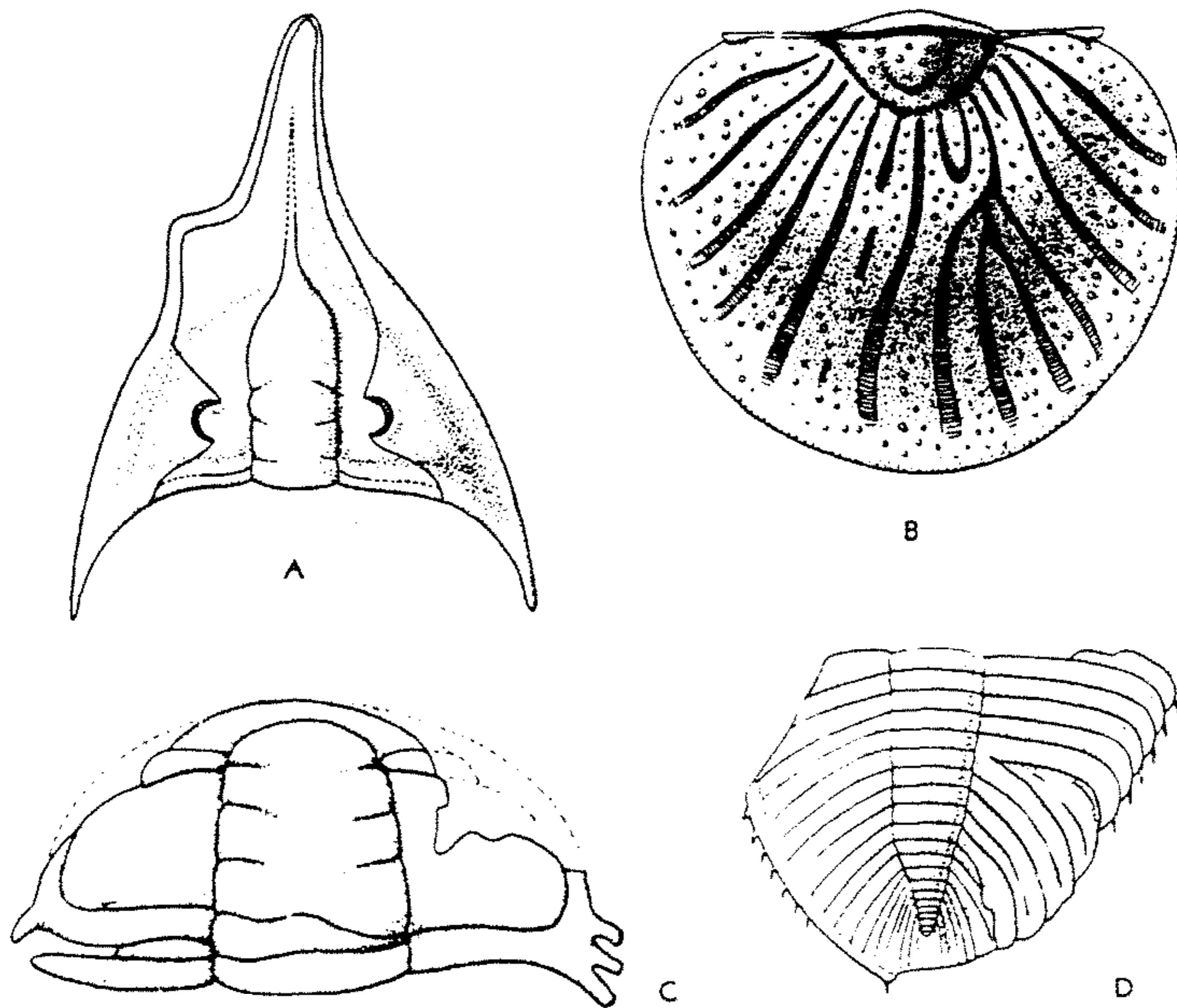
FIG. 82. Pathological and teratological individuals.—A. Pathological cephalon of Megistaspis acuticauda (ANGELIN) JAANUSSON, Ord., Baltic region, \times 0.6 , showing tumor on left side and deformation of anterior section of facial suture (after 24).—B. Pathological pygidium of Scutellum (Scutellum) flabelliferum (GOLDFUSS), M.Dev., Ger., \times 3 (after 24, from 48).—C. Teratological specimen of Rossaspis superciliosa (ROSS) HARRINGTON, L.Ord., USA(Utah), \times 1 ; the 2 anterior thoracic segments of the right side are fused with the cephalon, whereas on the left side the 1st thoracic pleura is abortive (after 24, from 49).—D. Pathological pygidium of Coronura aspectans (CONRAD) HALL & CLARK, L.Dev., USA(Ohio), \times 1.33 (after 17).
