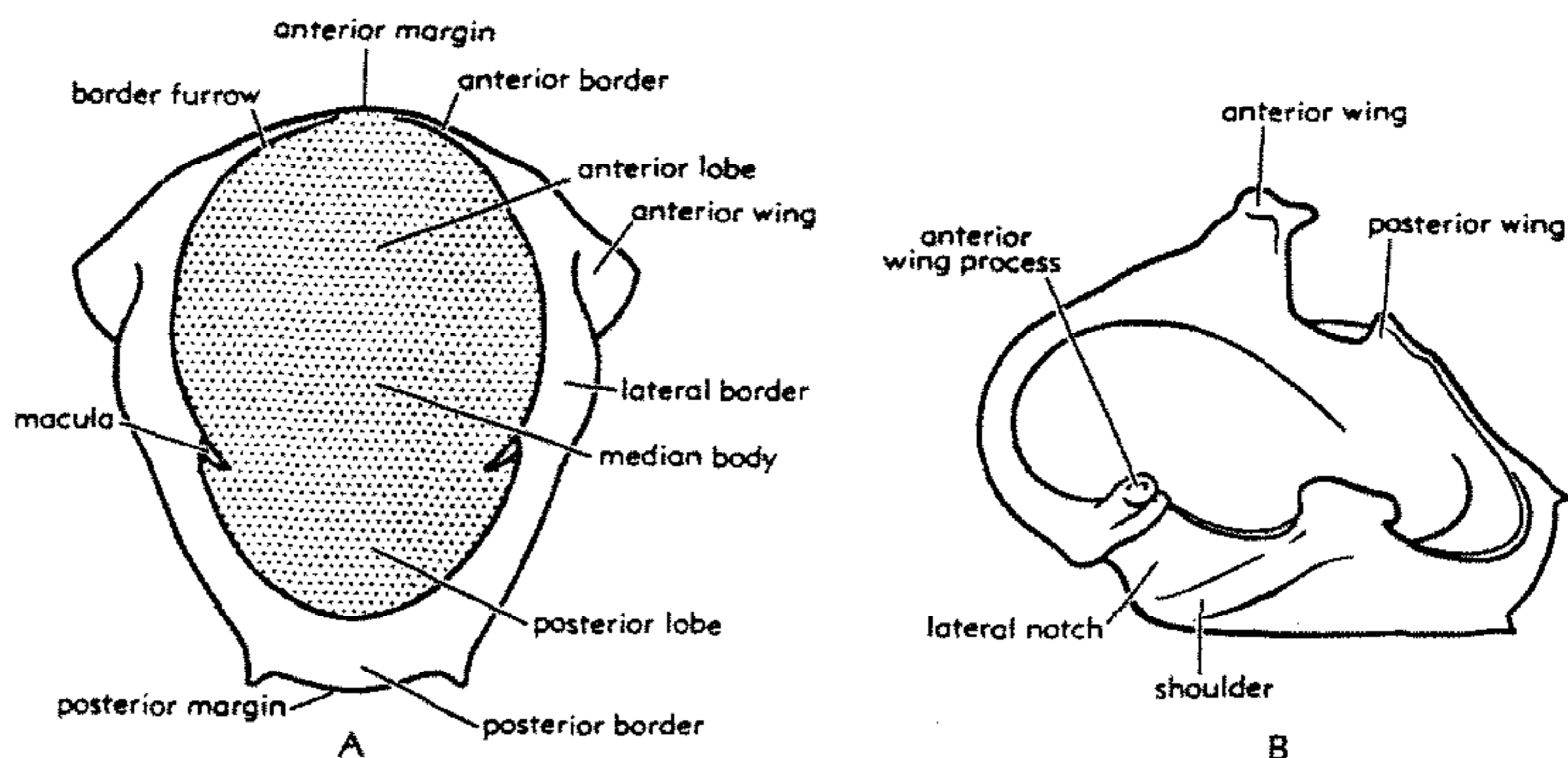
FIG. 39. Nomenclature of hypostoma, illustrated by Ceraurina typa B.N. COOPER, M.Ord., USA (Virginia), \times 5 . A, Exterior view; B, oblique interior view (after 71).
