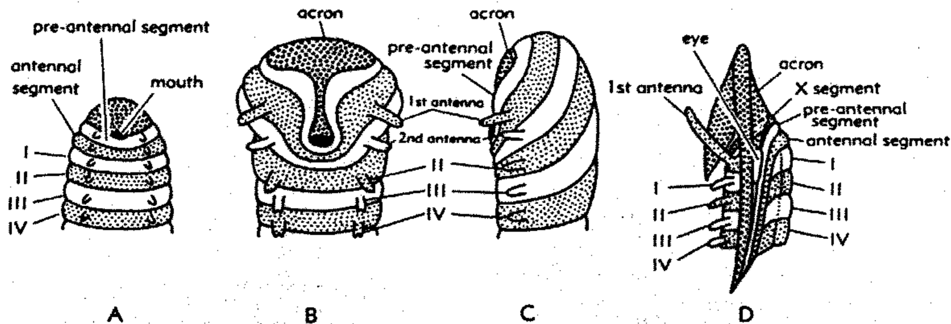
Fig. 7. Cephalic segmentation in an annelid-like arthropod prototype (A), generalized typical arthropod (B,C), and a trilobite (D). Ventral views in A,B; lateral views in C,D. The backward migration of the mouth is indicated in B,C. Traces of an "x segment" in trilobites (D) suggest that at least one segment is incorporated in the acron. (Mod. from Weber and Hupé.)
