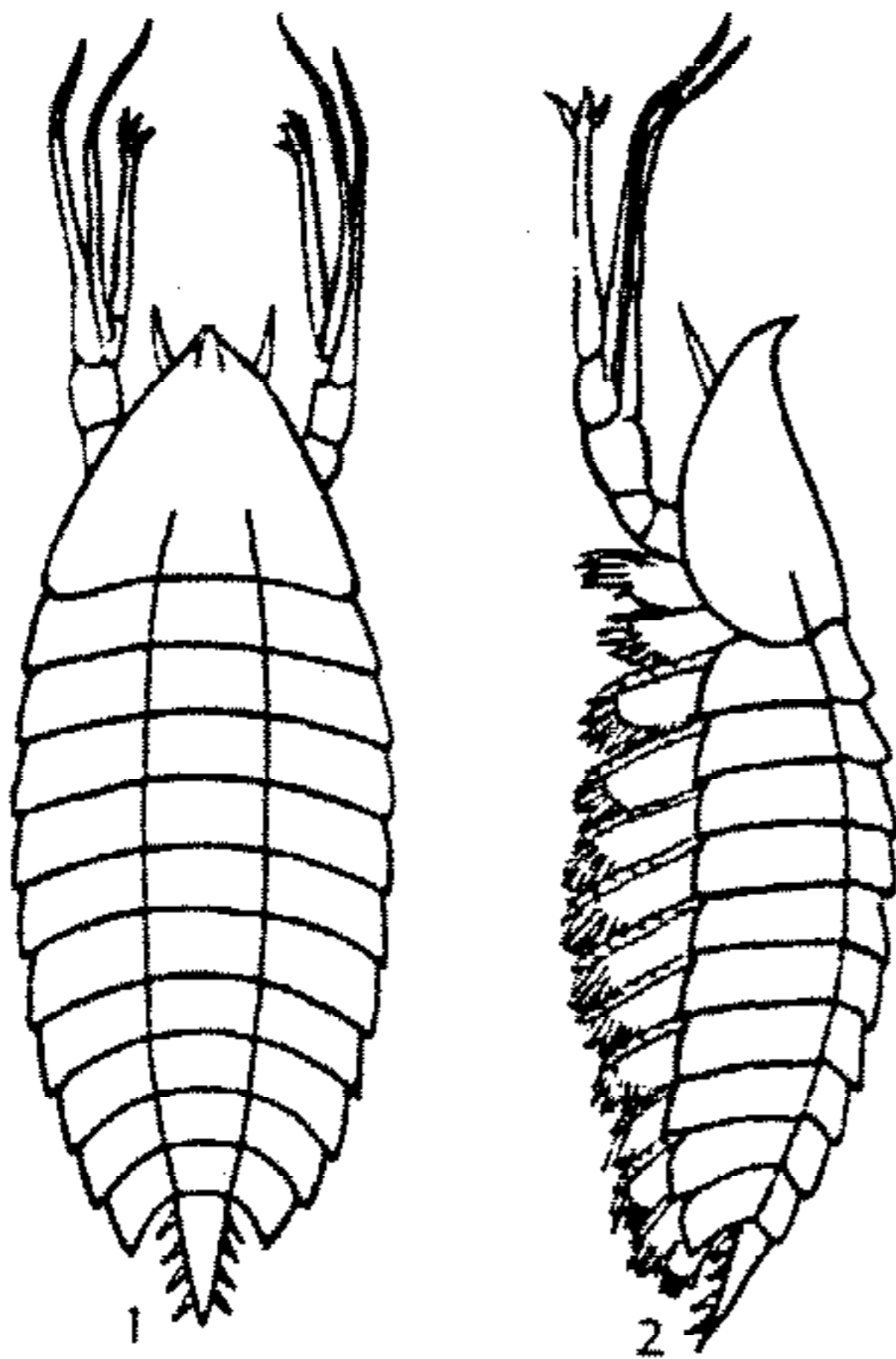
FIG. 20. Leanchoilia superlata WALCOTT, M.Cam., W.Can.(B.C.); 1,2, dorsal and lateral views (reconstr.), convexity probably exaggerated, \times 0.7 (4).
