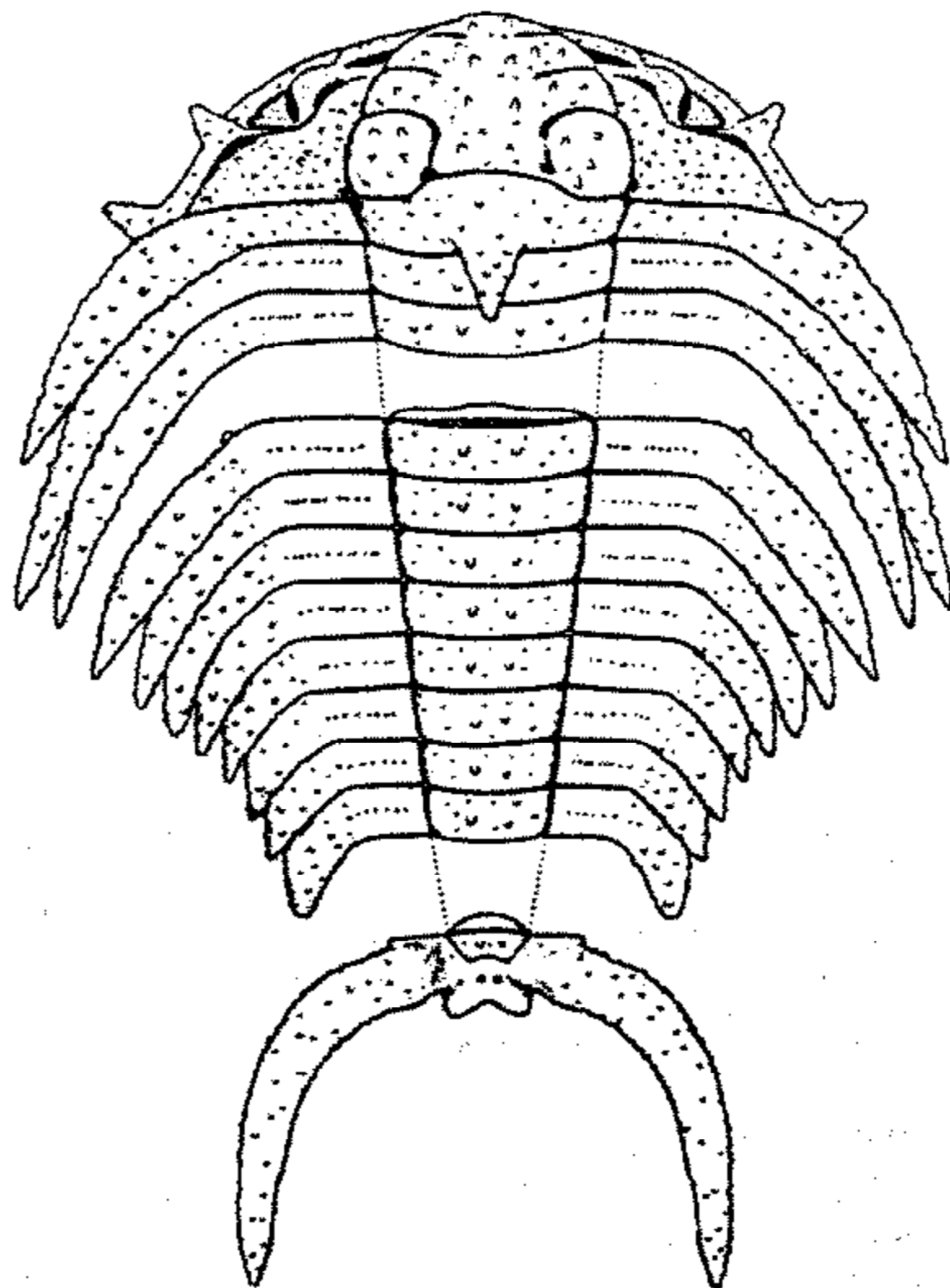
FIG. 340. * Holia secreti WHITTINGTON & EVITT (Cheiruridae), M.Ord., Va.; incompl. exoskel. (reconstr.), \times 8.5 (359).
