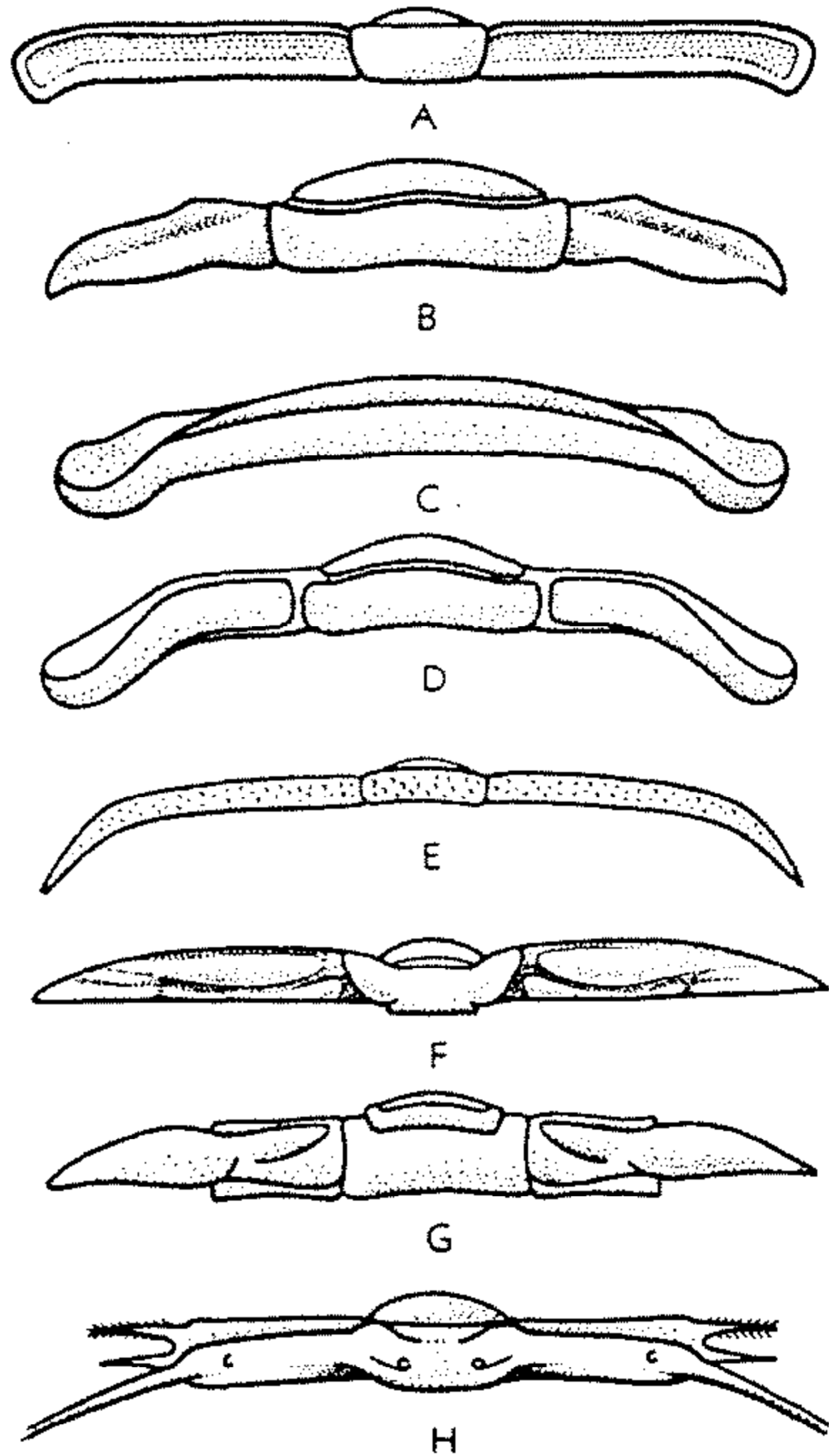
FIG. 51. Different types of thoracic segments.—A. Hapalopleura clavata HARRINGTON & LEANZA, L. Ord., S.Am.(Arg.), \times 10.6 (after 19).—B. Peltura scarabaeoides (WAHLENBERG) MILNE EDWARDS, U.Cam., Swed., \times 2.33 (after 97, 1923).—C. Trimerus delphinocephalus GREEN, M.Sil., USA(N.Y.), \times 0.8 (after 17).—D. Pliomera fischeri (EICHWALD) ANGELIN, M.Ord., Estonia, \times 2.8 (after 34).—E. Nieszkowskia capitalis ÖPIK, Ord., Estonia, \times 0.3 (after 34).—F. Dichelepyge pascuali HARRINGTON & LEANZA, L.Ord., E.Am.(Arg.), \times 8.3 (after 19).—G. Ceraurus aculeatus EICHWALD, Ord. Estonia, \times 2.4 (after 34).—H. Miraspis miru (BARRANDE) RICHTER & RICHTER, M.Sil., Bohemia, \times 3.75 (after 99, 1956).
