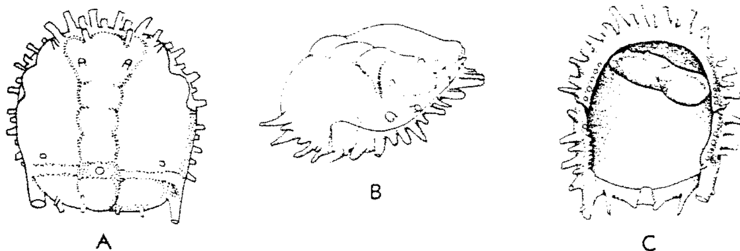
FIG. 94. Phacopid protaspis, L.Dev., E.U.S.A.(N.Y.); A-C, dorsal, anterolateral, ventral views (C with immature ostracode carapace adhering to specimen), \times 30 (+1n; 3+*).
