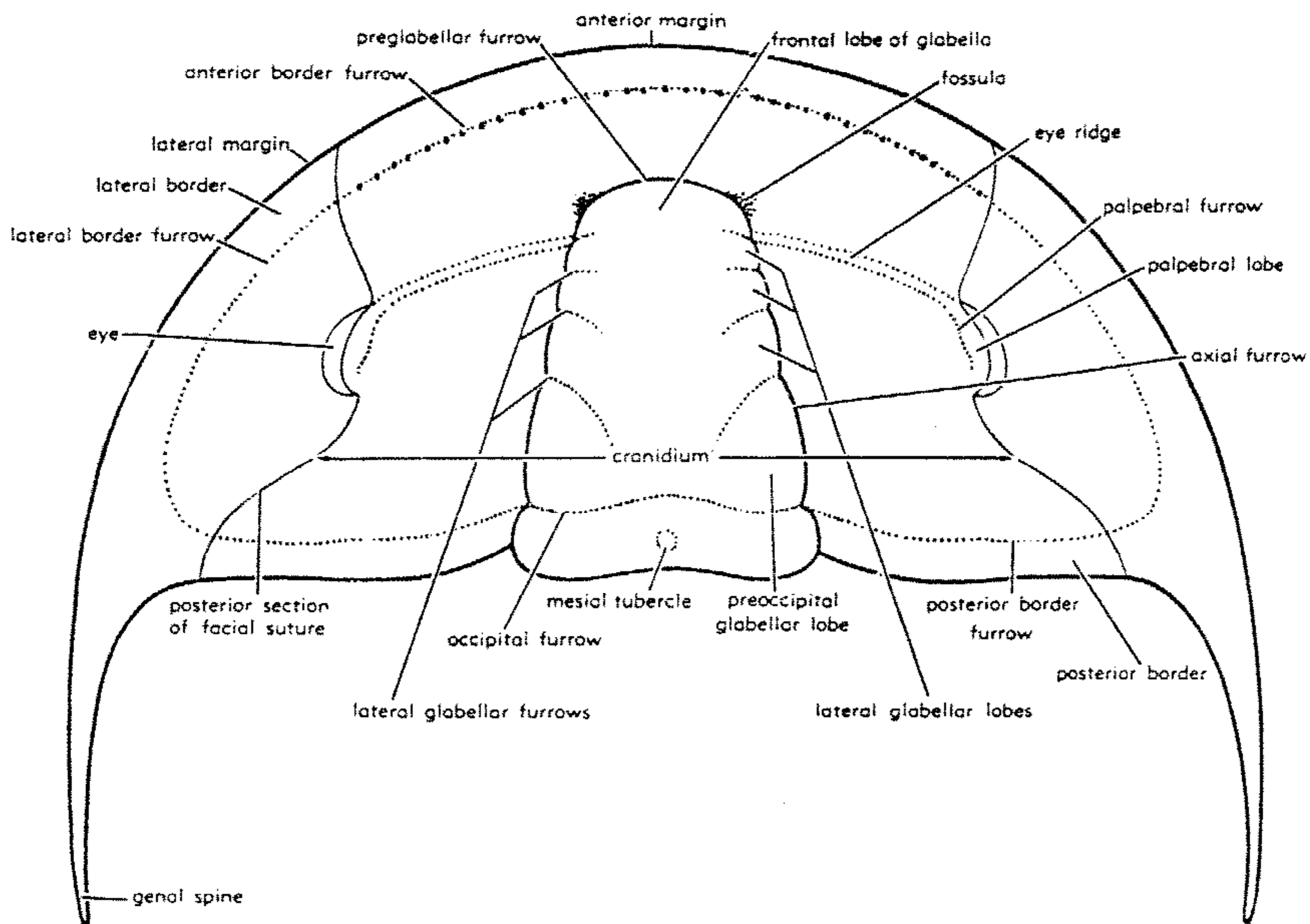
FIG. 30. Cephalic nomenclature of a typical psychopariid trilobite.
