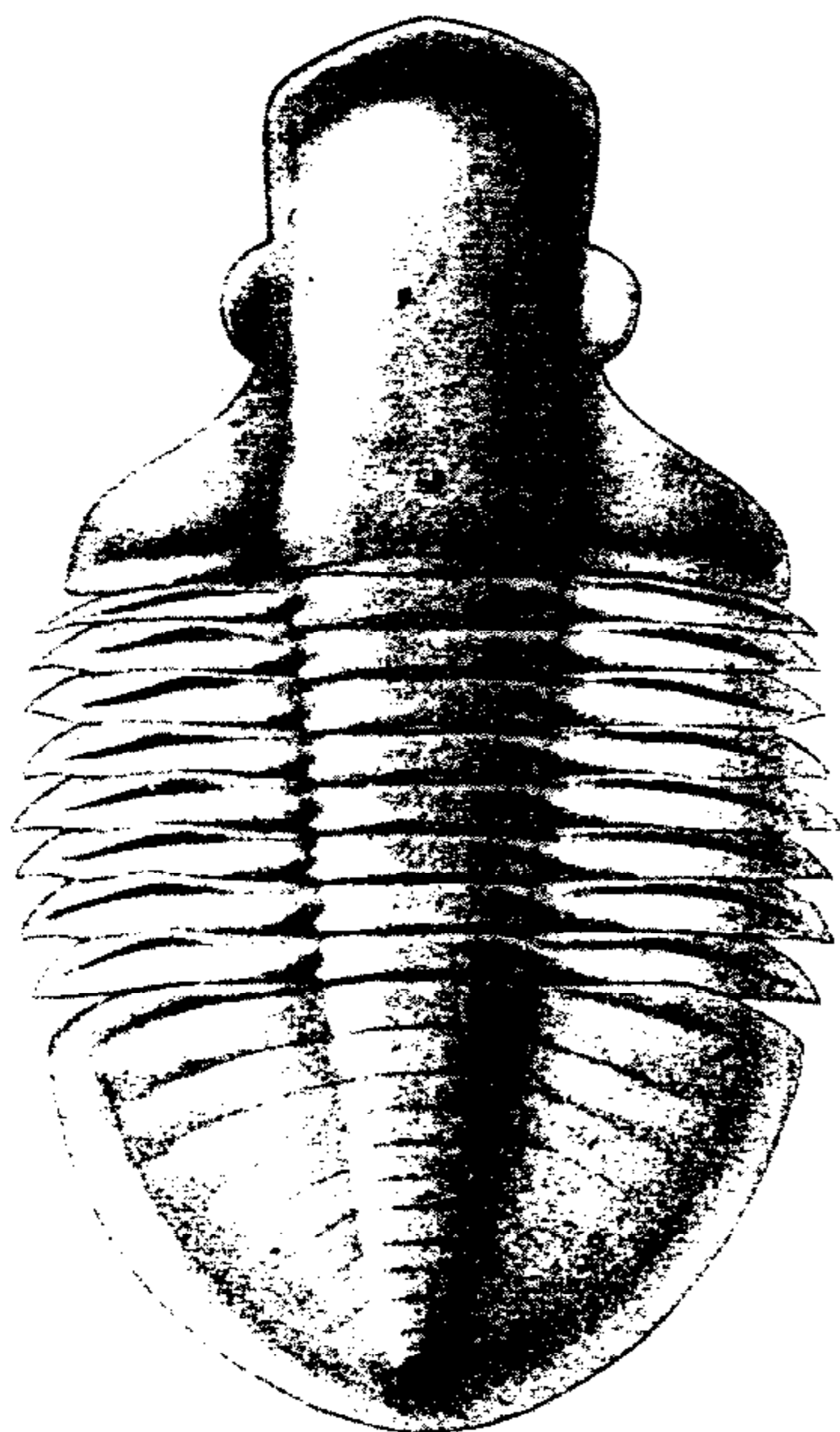
FIG. 257. * Megalaspidella (Megalaspidella) kayseri KOBAYASHI (Asaphidae), L.Ord.(Arenig.), Arg.; carapace lacking librigenae (reconstr.), \times 1.7 (59*).
