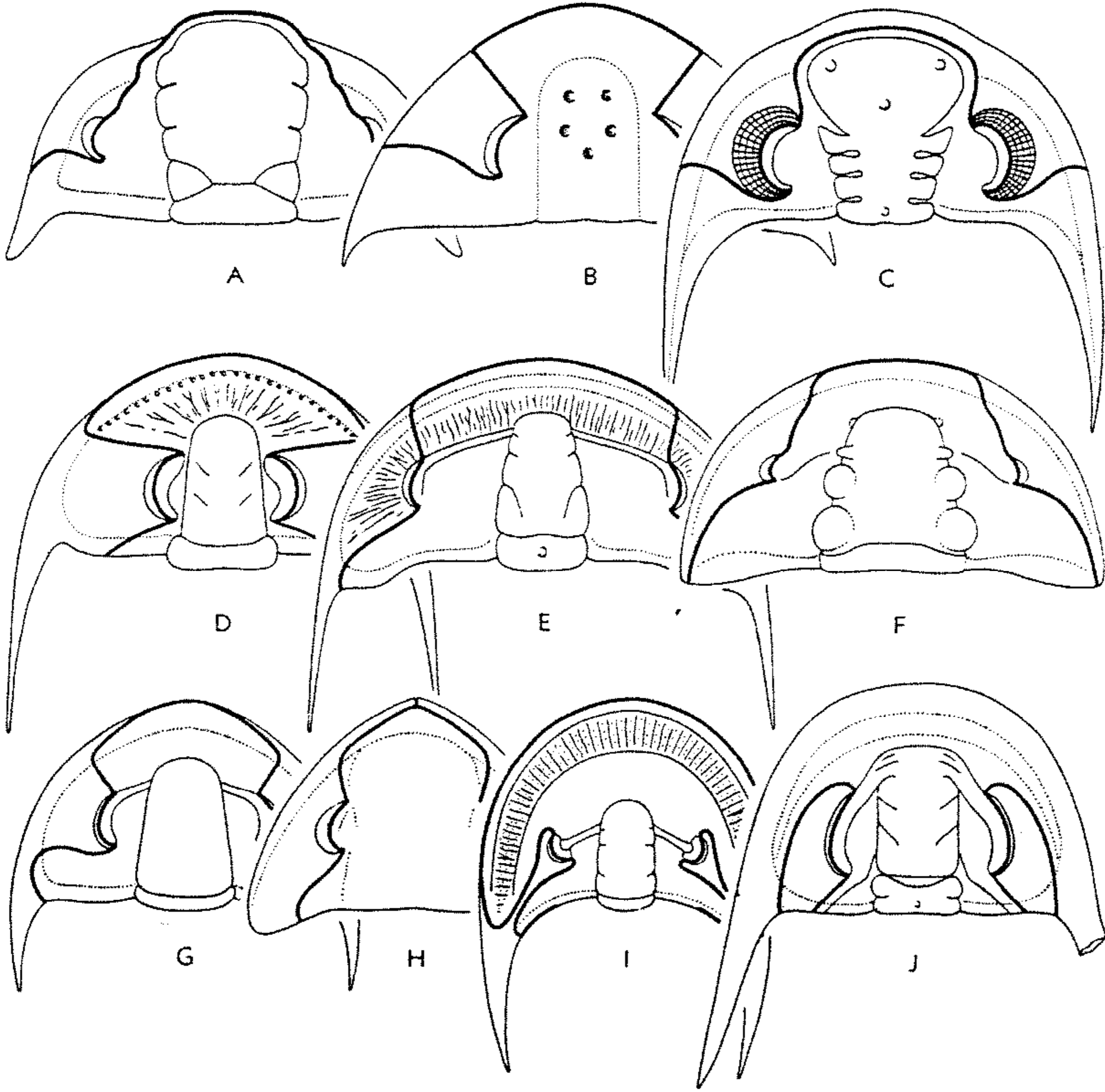
FIG. 45. Types of facial sutures.—A-C. Proparian sutures; A, cheirurid type, Ceraurinella typa B. N. COOPER, M.Ord., USA (Virginia), \times 3.5 (after 71); B, burlingiiform type, Burlingia hectori WALCOTT, M. Cam., Can., \times 9.3 (after 96, 1908); C, dalmanitiform type, Odontochile hausmanni (BRONGNIART) HAWLE & CORDA, Dev., Boh., \times 1 (after 2).—F. Gonatoparian suture; Flexicalymene senaria (CONRAD) WHITTINGTON, M.Ord., USA (N.Y.), \times 3.5 (after 70).—D, E, G-I. Opisthoparian sutures; D, kainelliform type, Kainella meridionalis KOBAYASHI, L.Ord., S. Am. (Arg.), \times 0.73 (after 19); E, ptychopariid type, Ptychoparia striata (EMMRICH) HAWLE & CORDA, L.Ord., Boh., \times 1 (after 2); G, cedariiform type, Cedaria prolifica WALCOTT, U. Cam., USA (Ala.), \times 1.6 (after 81, 1948); H, isoteliform type, Isotelus gigas DEKAY, M.Ord., Can., \times 1.2 (after 84, 1912); I, entomaspidiform type, Entomaspis radiatus ULRICH, U. Cam., USA (Mo.), \times 5.6 (after 48, 1952).—J. Metaparian sutures; Fallotaspis taxemmourtsensis HUPÉ, L. Cam., Afr. (Morocco), \times 1.33 (after 24).
