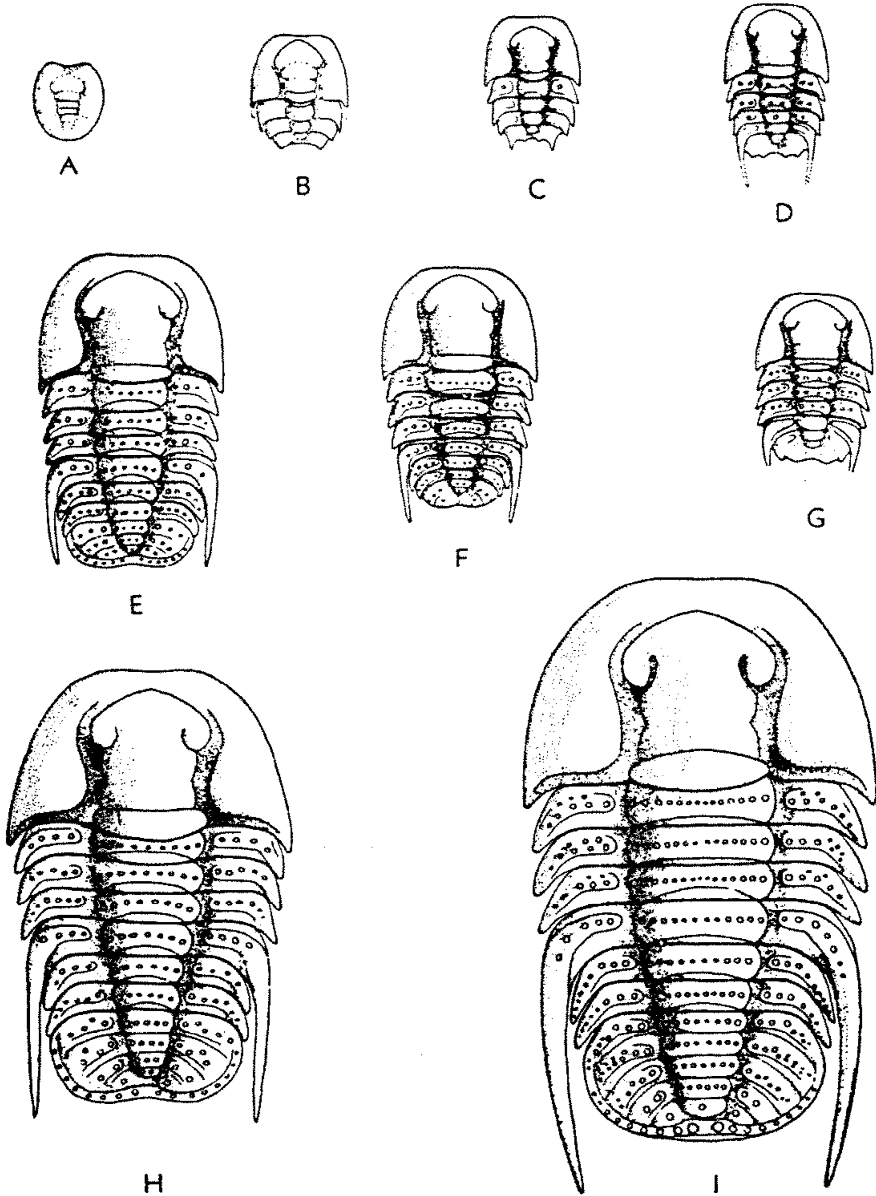
FIG. 87. Ontogenetic stages of Shumardia pusilla (SARS), L.Ord.(Tremadoc.), Eng.; A, protaspis, X40; B, meraspis, "degree" 0, X40; C-G, meraspis, "degrees" 1-5, X30; H, holaspis, X30; I, larger holaspis with additional segment in pygidium, X20 (25*).
