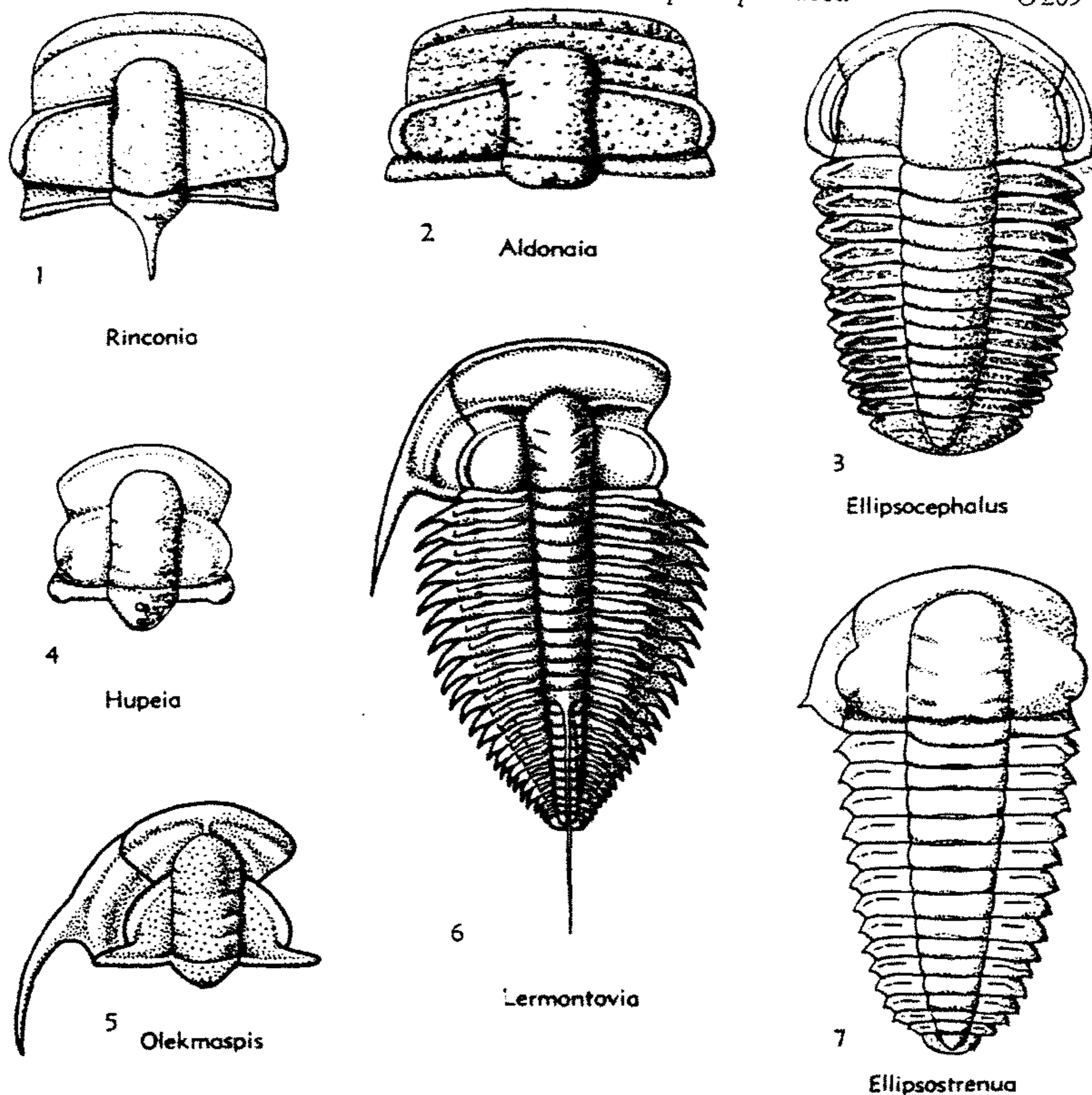
FIG. 150. Ellipsocephalidae (Ellipsocephalinae), Protolenidae (Protoleninae, Aldonaiinae), Family uncertain (p. O207-O212).
