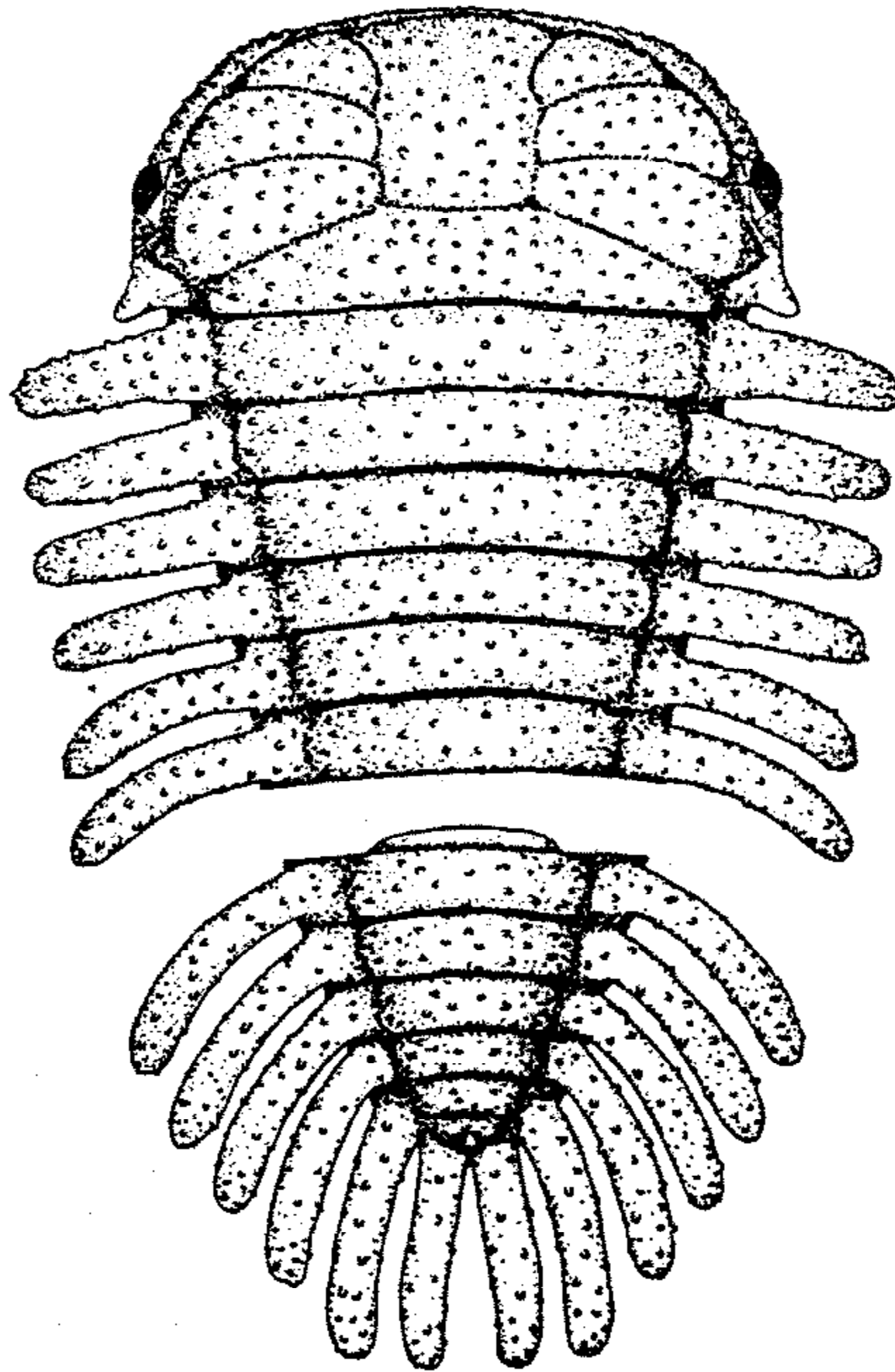
FIG. 343. * Heliomeroides teres EVITT (Cheiruridae), M.Ord., Va.; incompl. exoskel. (reconstr.), \times 4.25 (42).
