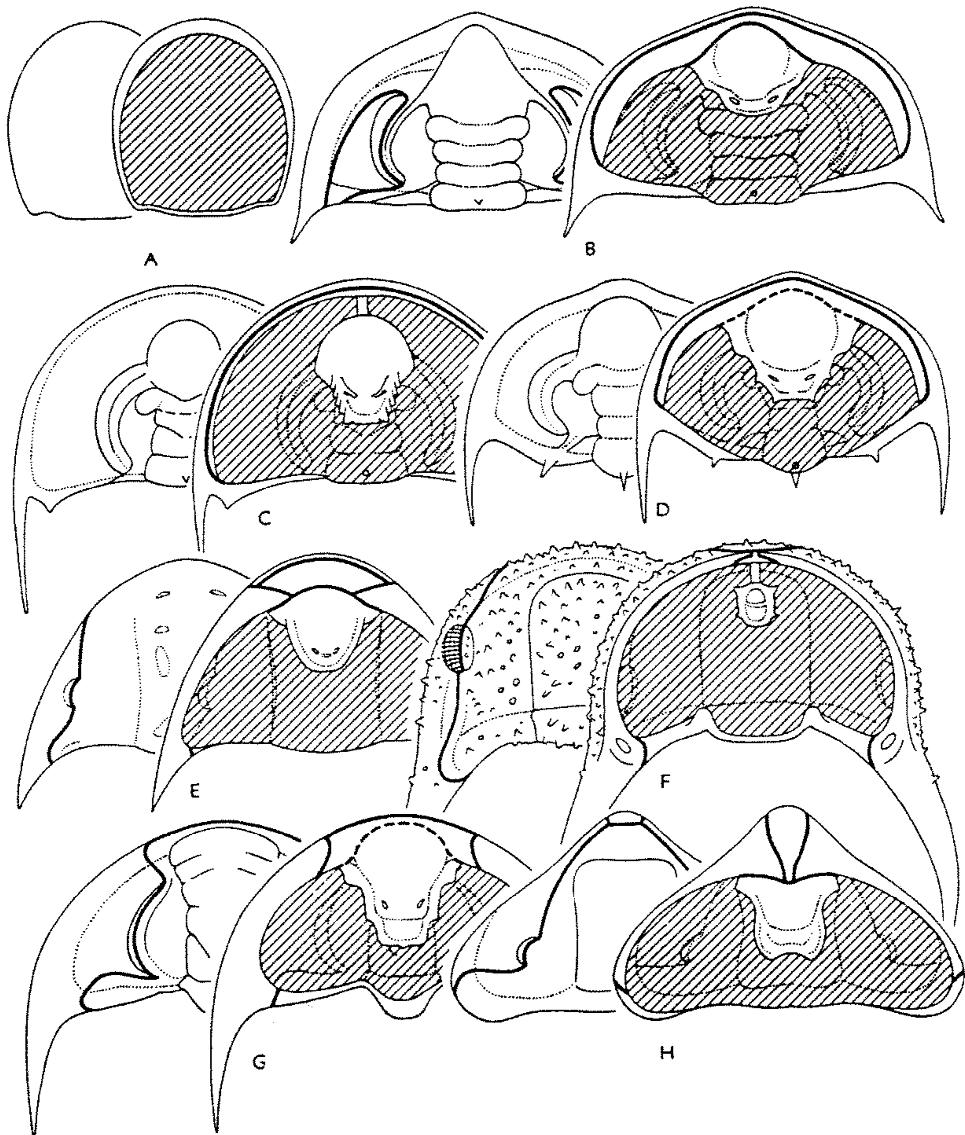
FIG. 48. Cephalic types defined by suture patterns.—A. Agnostid type, Phalacroma glandiforme (ANGELIN) WESTERGÅRD, M.Cam., Swed., \times 3.3 (after 97, 1946).—B. Olenellid type, Kjerulfia lata KIAER, L.Cam., Swed., \times 0.5 (after 28).—C. Paedeumiid type, Paedeumias transitans WALCOTT, L.Cam., USA (Vermont), \times 2.5 (after 64).—D. Holmiid type, Holmia kjerulfi (LINNARSSON) MARCOU, L.Cam., Swed., \times 1.85 (after 28).—E. Ptychopariid type, Dysplanus centrotus (DALMAN) BURMEISTER, L.Ord., Swed., \times 1.2 (after 79, 1954).—F. Dimeropygid type, Dimeropyge virginiensis WHITTINGTON & EVITT, M.Ord., USA (Virginia), \times 21.7 (after 71).—G. Corynexochid type, Fieldaspis jurcata RASETTI, M.Cam., Can. (B.C.), \times 1.3 (after 84, 1951).—H. Homalonotid type, Dipleura dekayi GREEN, M.Dev., USA (N.Y.), (B.C.), \times 1.3 (after 84, 1951).—I. Bathynotid type, Bathynotus holopygus (HALL) HALL, L.Cam., USA (Vermont), \times 0.8 (after 17).—J. Asaphid type, Lachnostoma latucelsum ROSS, L.Ord., USA (Utah), \times 7.45 (after \times 2 (after 81, new)).—K. Nileid type, Nileus armadillo DALMAN, Ord., Swed., \times 1.5 (after 1, 1854, and 2).—L. Phacopid type, Odontochile hausmanni (BRONGNIART) HAWLE & CORDA, Dev., Bohemia, \times 1.25 (after 2).—M. Trinucleid type, Cryptolithus tessellatus GREEN, M.Ord., USA (N.Y.), \times 3 (after 70, and 85, 1930).—N. Harpid type, Paraharpes hornei (REED) WHITTINGTON, U.Ord., Scot., \times 2 (after 99, 1950).
