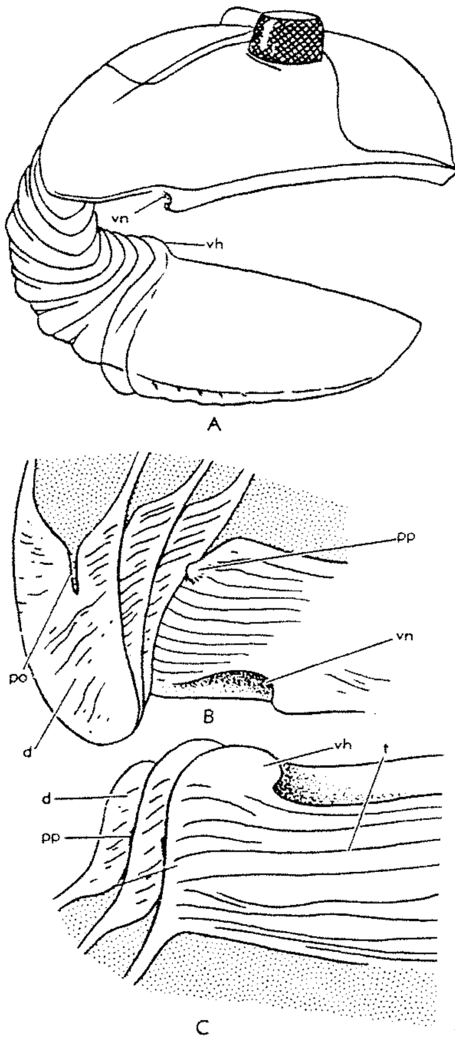
FIG. 78. Vincular notch and hook in Asaphus expansus DALMAN, Ord., Estonia (slightly schematic drawing after 52.)—A. Specimen not completely enrolled, \times 2 ; the thoracic pleural extremities and the anterolateral angle of the pygidium will fit, at completion of enrollment, into cephalic vincular notch.—B. Internal (ventral) view of the posterolateral angle of the cephalon and the anterior 3 overlapping thoracic pleurae, \times 4 .—C. Internal (ventral) view of the anterolateral angle of the pygidium and of the posterior 3 overlapping pleurae, \times 4 . (Explanation: d , doublure; po , panderian opening; pp , panderian protuberance; t , terrace lines; vn , vincular notch; vh , vincular hook.)
