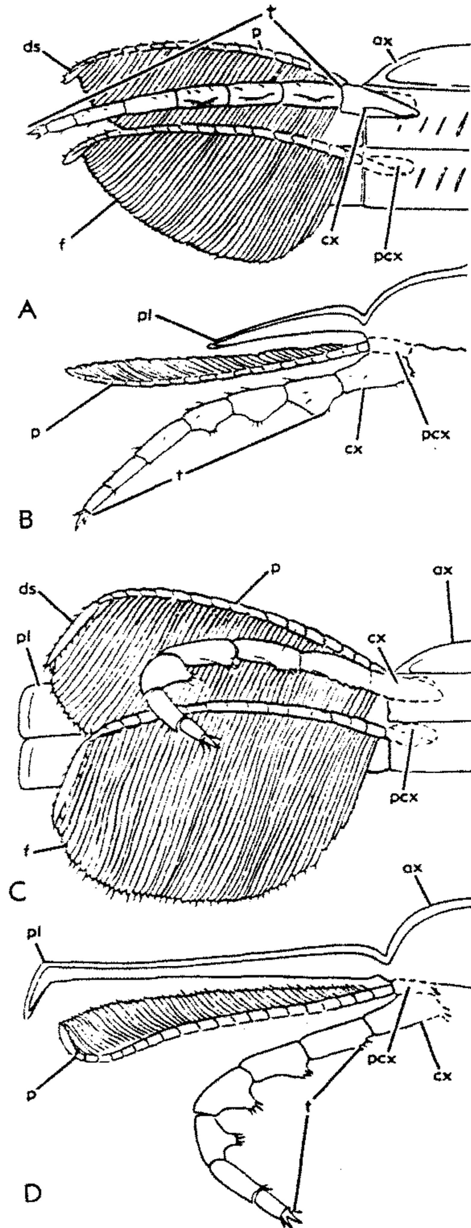
FIG. 55. Diramous appendages of trilobites; reconstructions of the appendages of 2 thoracic segments (after 56).—A,B. Triarthrus eatoni (HALL) RUEDEMANN, M.Ord., USA(N.Y.); A, ventral view; B, anterior view, \times 5 .—C,D. Cryptolithus tessellatus GREEN, M.Ord., USA(N.Y.); C, ventral view; D, anterior view, \times 14 . (Explanation: ax, axis; cx, coxa; ds, distal segment of pre-epipodite; f, filaments; p, pre-epipodite; pex, pre-coxa; pl, pleura; t, telopodite.)
