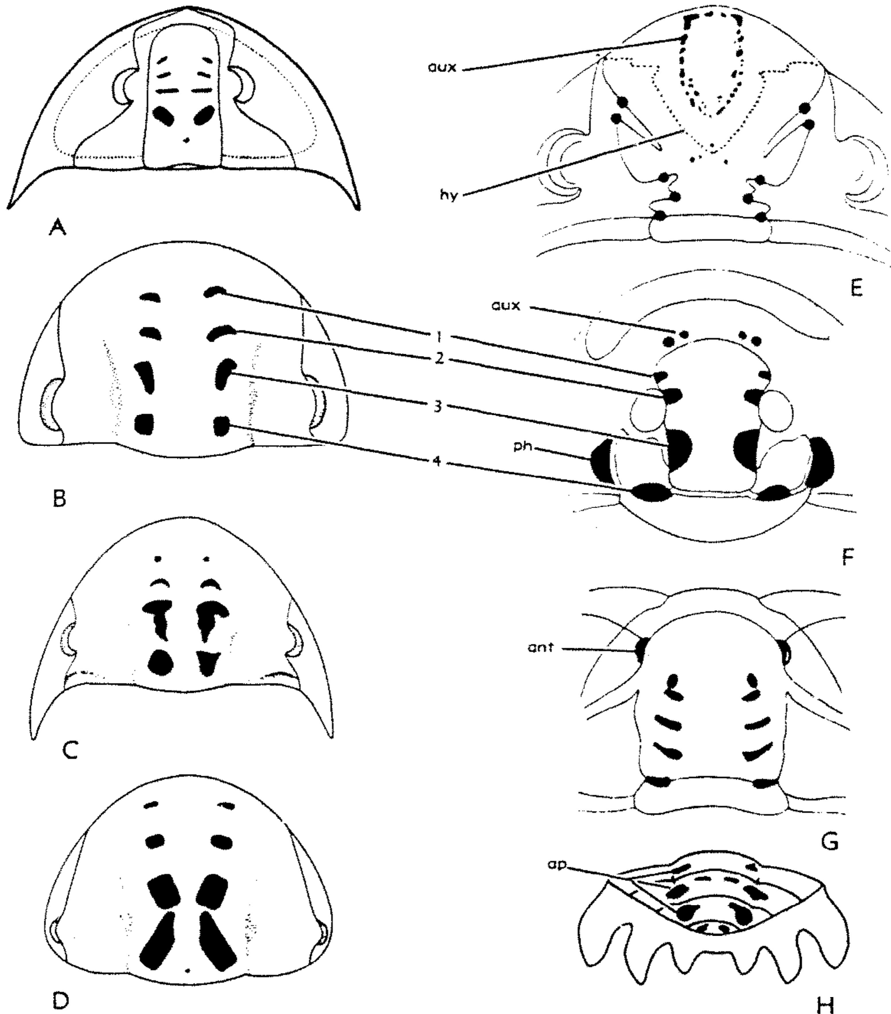
FIG. 69. Areas of muscle attachment.— A , Cephalon of Notopeltis orthometopus (HARRINGTON) HARRINGTON & LEANZA, L.Ord., Arg., \times 2.5 (after 19).— B , Cephalon of Ilaenus dalmani VOLBORTH, Ord., Russia, \times 1.2 (after 79, 1954).— C , Cephalon of Dysplanus centrotus (DALMAN) BURMEISTER, L.Ord., Swed., \times 1.2 (after 79, 1954).— D , Cephalon of Stenopareia oviformis (WARBURG) JAANUSSON, M.Ord., Swed., \times 1.8 (after 79, 1954).— E , Cephalic axial region of Chasmops odini (EICHWALD), M.Ord., Estonia, \times 2 (after 9).— F , Cephalic axial region of Pharostoma nieszowski SCHMIDT, Ord., Estonia, \times 5.75 (after 24).— G , Cephalic axial region of Cybele grewingkii SCHMIDT, Ord., Estonia, \times 1.25 (after 24).— H , Ventral view of pygidium of Reraspis plautini (SCHMIDT) ÖPIK, M.Ord., Estonia, \times 3.95 (after 34). (Explanation: ant , antennary muscle scar; app , appendage muscle scars; aux , auxiliary impressions; hy , outline of the hypostoma; ph , pharostomial scar; 1-4, principal muscle scars of cephalic axis, regarded as places of attachment of ventral appendage muscles.)
