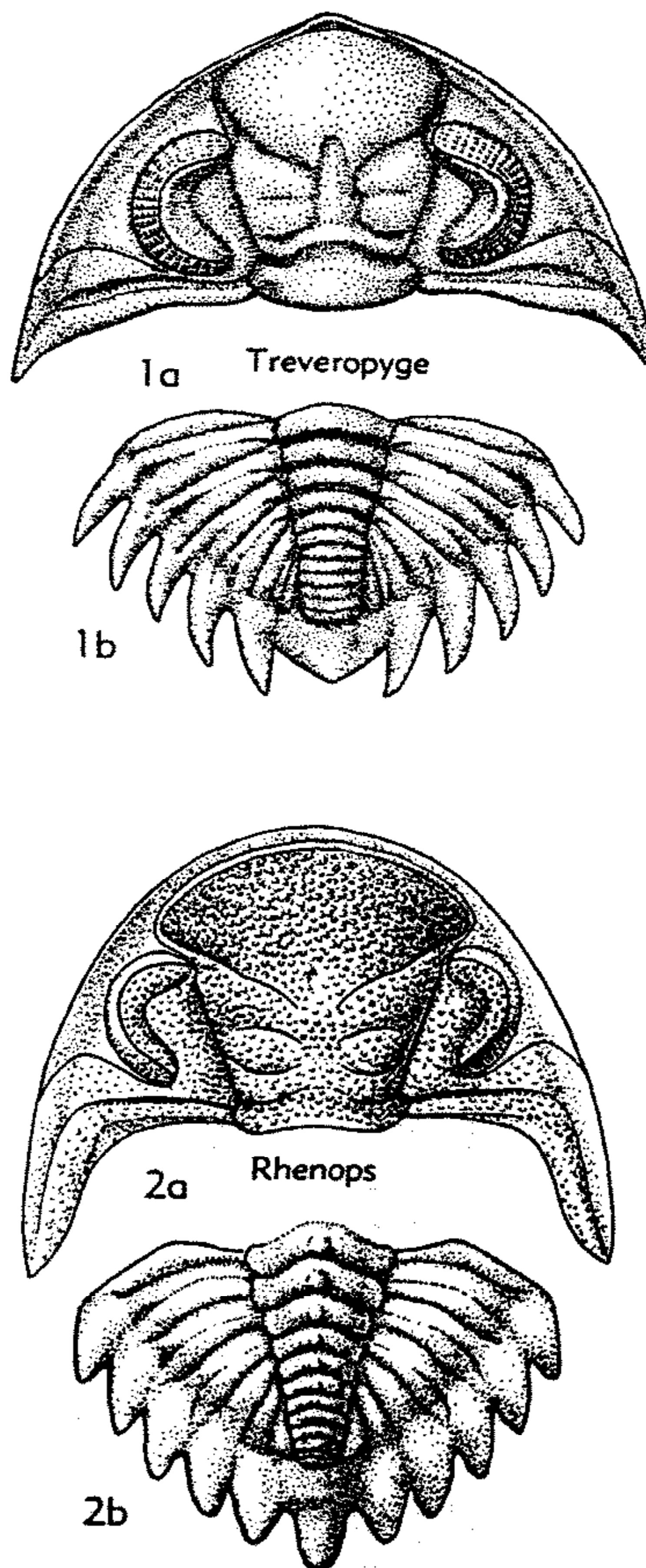
FIG. 382. Dalmanitidae (Asteropyginae (p. 0483)).
