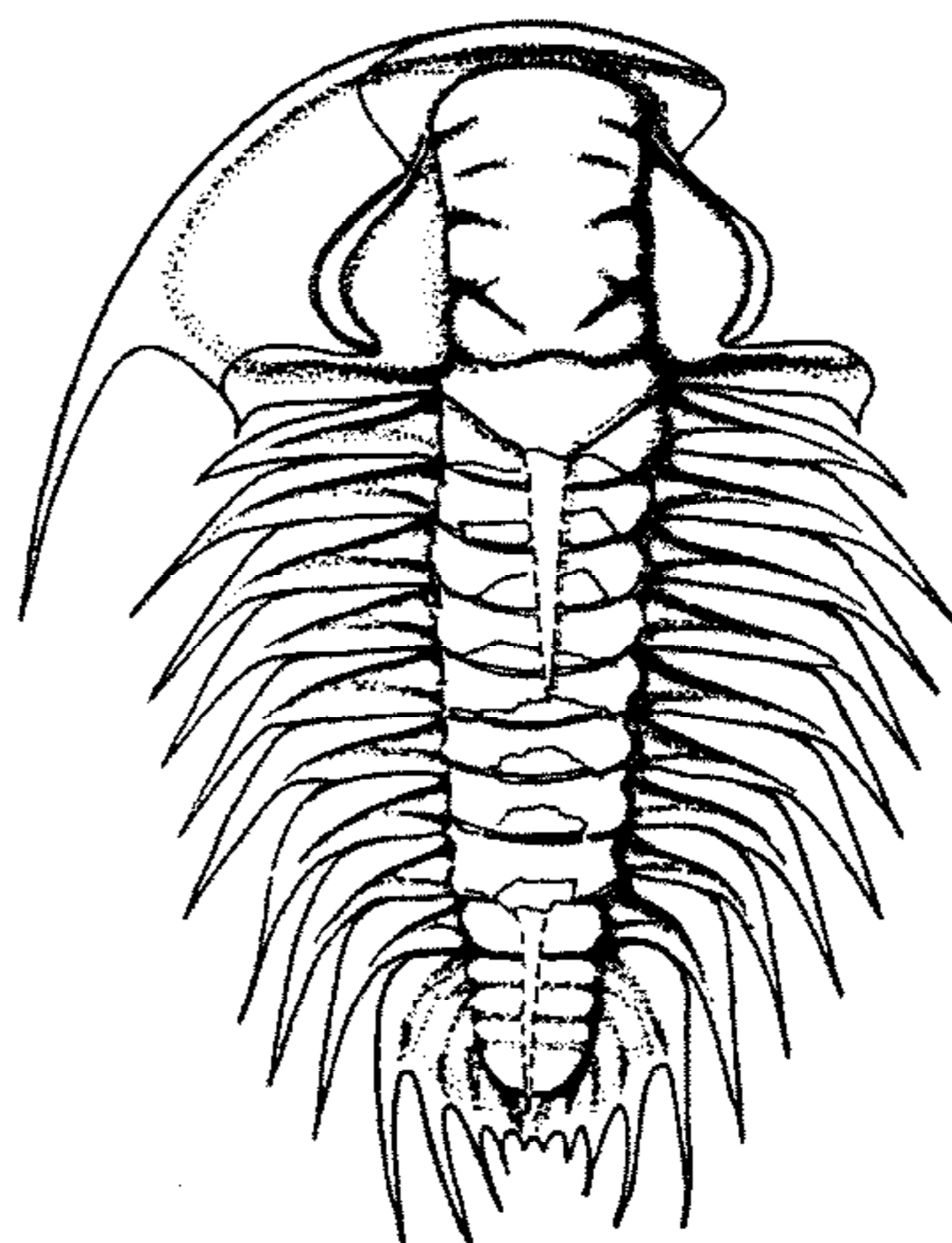
FIG. 166. *Zacanthoides romingeri WALCOTT ( Zacanthoididae ), M. Cam. , W.Can. (B.C.); exoskel., \times 0.6 (448n).
