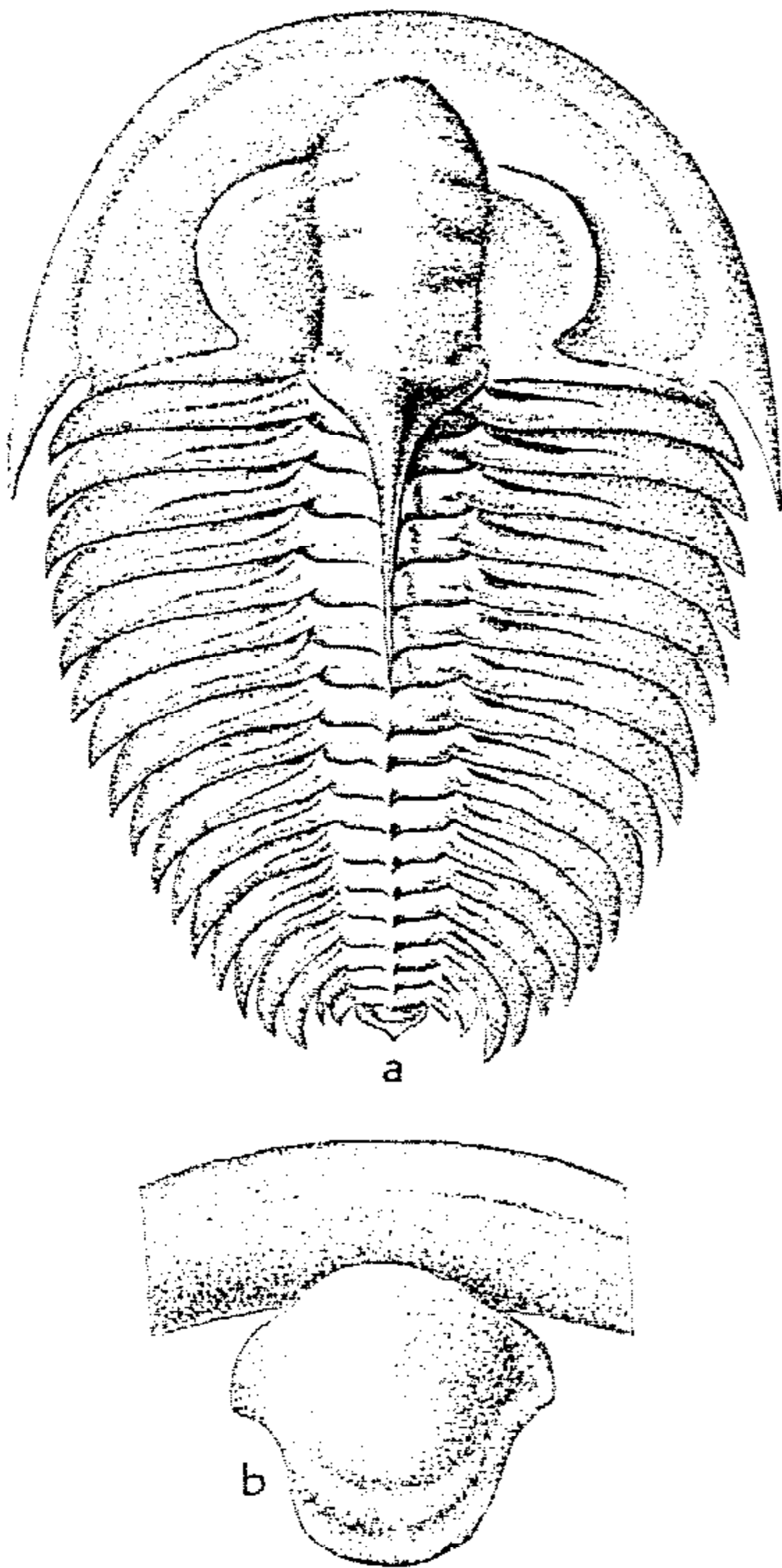
FIG. 136. * Callavia broeggeri (WALCOTT) (Olenellidae, Callaviinae). L.Cam. , Newf.; a , dorsal exoskel., \times 0.4 ; b , hypostoma and part of rostral plate, \times 1.8 (312).
