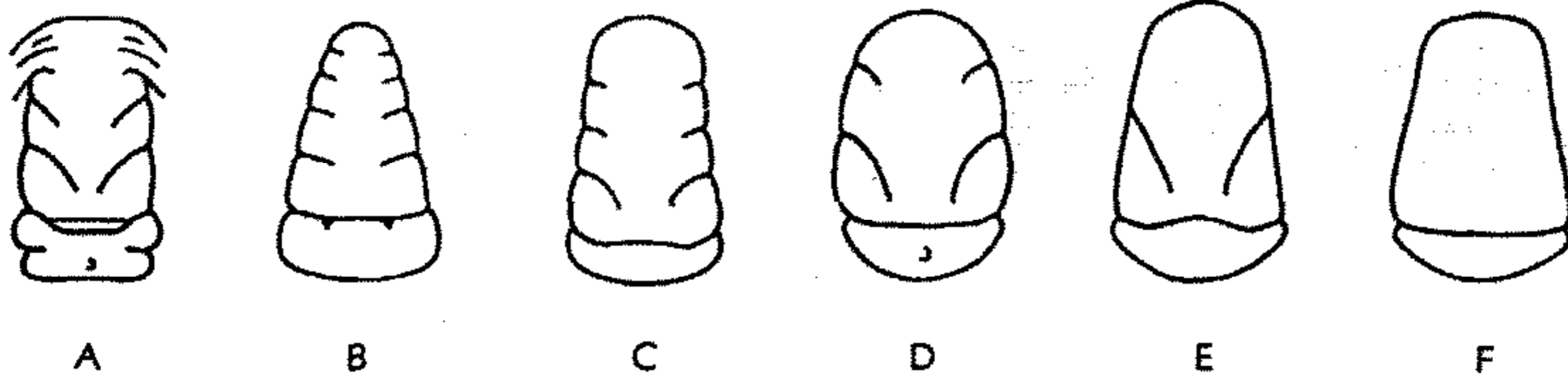
FIG. 33. Glabellar segmentation in different genera, showing decreasing number of lateral glabellar furrows from 5 pairs to none. A , Fallotaspis ; B , Daguinaspis ; C , Latiredlichia ; D , Talbotina ; E , Elrathiella ; F , Plethopeltis .
