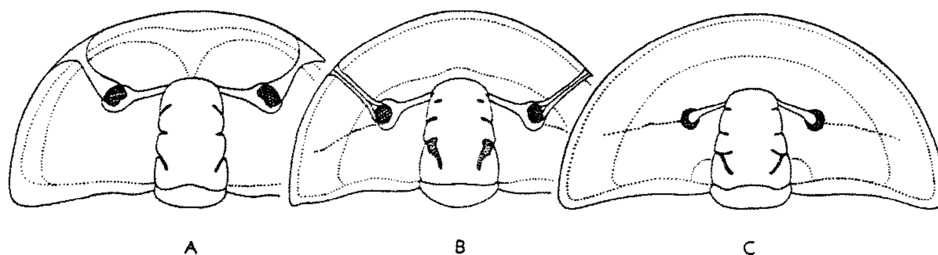
FIG. 46. Evolution of the facial sutures in the Loganopeltid stock of the Harpididae.—A. Loganopeltoides kindlei RASETTI, U.Cam., Can. (Newf.), \times 5.4 .—B. Loganopeltoides zenkeri (BILLINGS) RASETTI, U.Cam., Can.(Que.), \times 4.65 .—C. Loganopeltis depressa RASETTI, L.Ord., Can.(Que.), \times 3.3 (All after 38).
