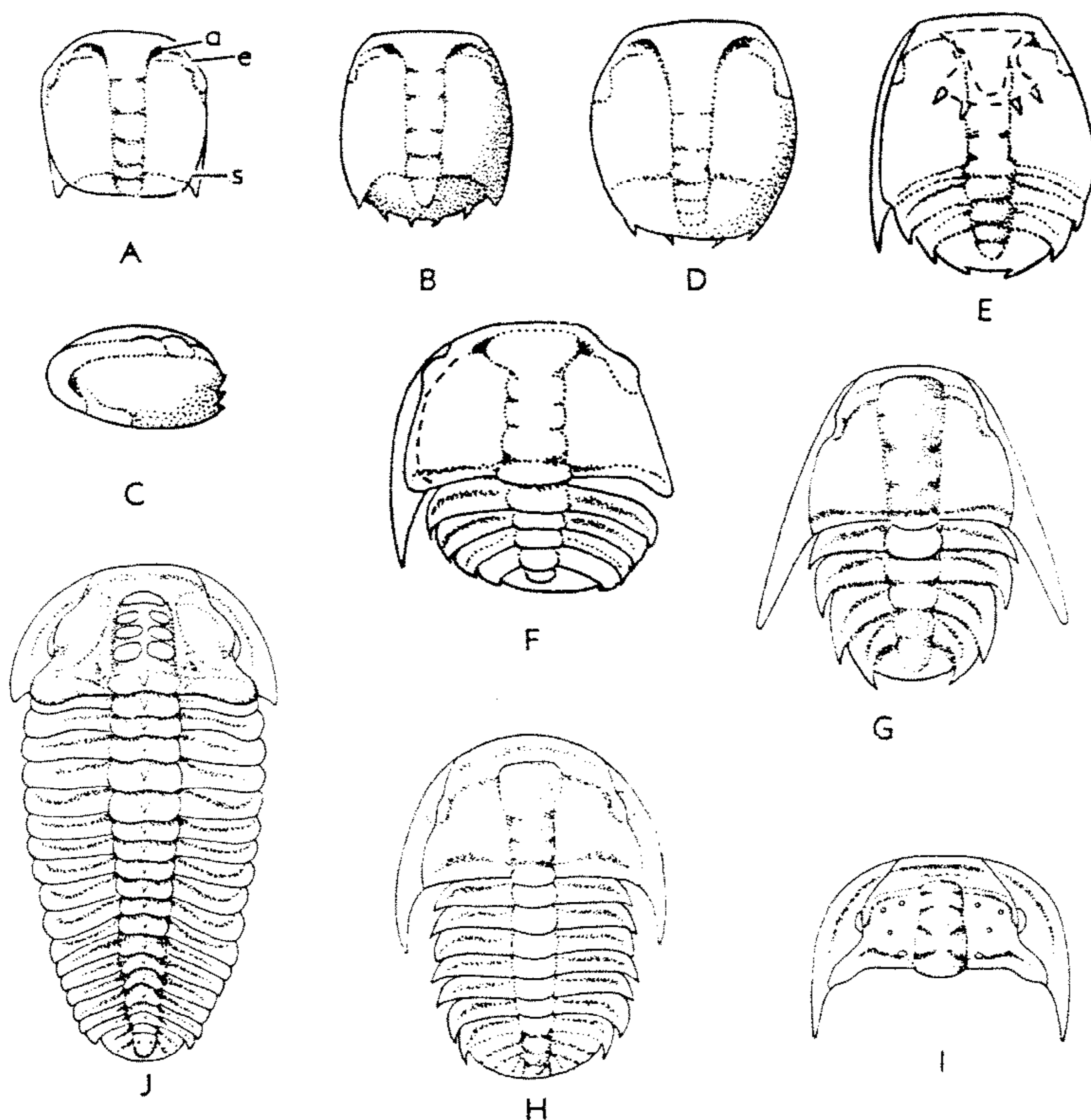
FIG. 88. Ontogenetic stages of Szö hirsuta BARRANDE, M. Cam., Bohemia; A, protaspis with librigena ( a , anterior pit; e , eye ridge; s , suture), \times 30 ; B, C, protaspis lacking librigenae, dorsal and anterolateral views, \times 30 ; D, protaspis, \times 30 ; E, protaspis with left librigena and hypostoma shown by dashed outline, \times 30 ; F, "degree" 0 with left librigena, dashed line showing inner edge of doublure, \times 30 ; G, "degree" 1, \times 30 ; H, "degree" 6, \times 15 ; I, "degree" 12 cephalon, \times 7 ; J, holaspisid exoskeleton, \times 2 (4In).
