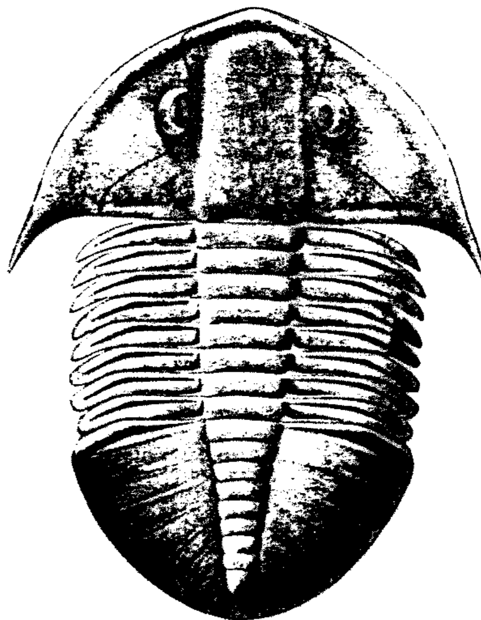
FIG. 261. * Notopeltis orthometopa (HARRINGTON) (Asaphidae), L.Ord.(U.Tremadoc.), Arg.; carapace (reconstr.), \times 2.8 (59*).
