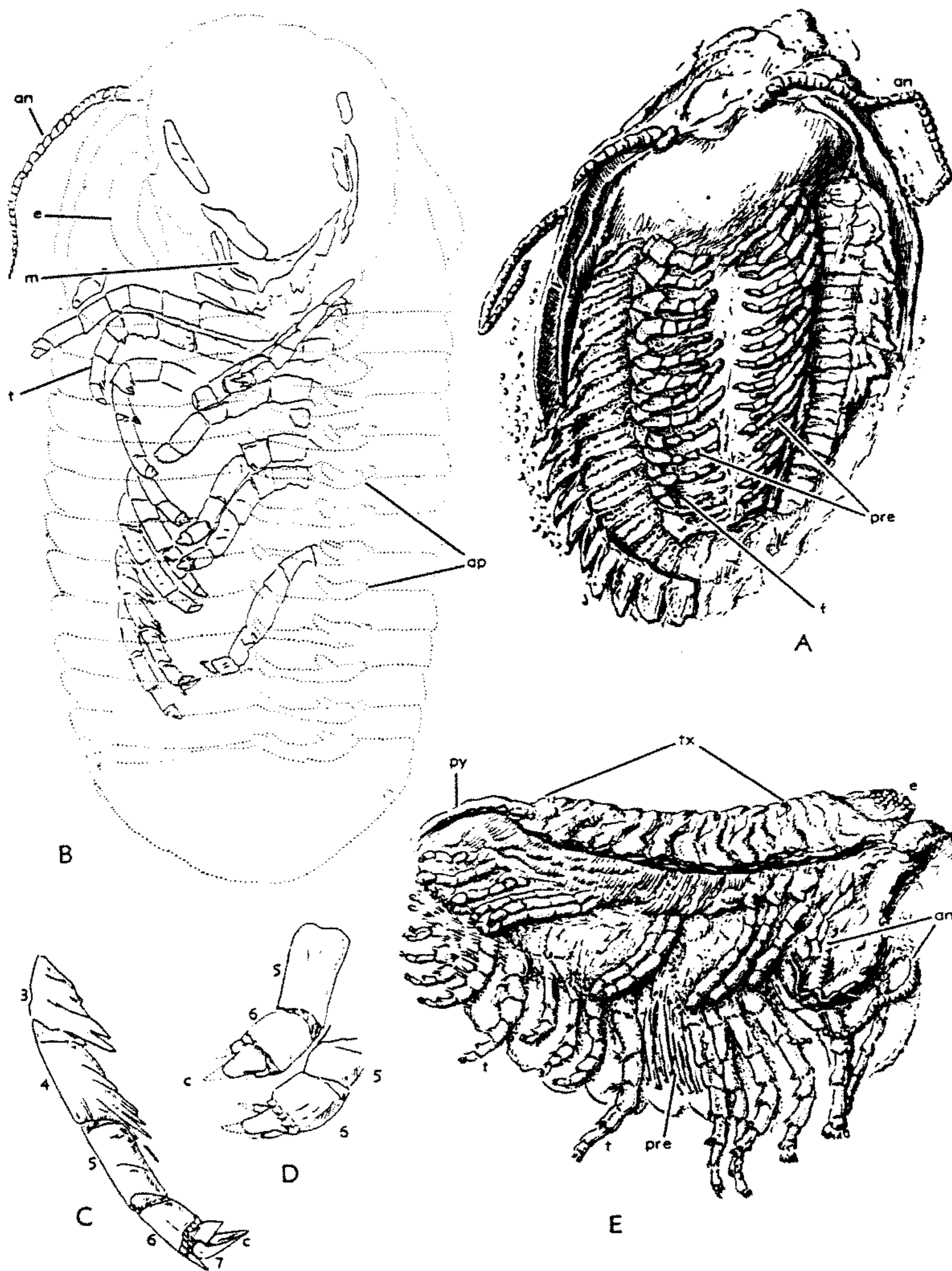
FIG. 57. Ventral appendages of trilobites.— A. Asteropyge sp., L.Dev., Ger., X2; ventral view of specimen lacking cephalic biramous appendages (after 72).— B-E. Phacops sp., L.Dev., Ger.; B , ventral view of specimen retaining several telopodites, right antenna, and metastoma, X1.33; C-E , enlargement of fragmentary telopodites, showing distal claw, X3.7 (after 55); F , lateral view of specimen showing biramous appendages and antennae, X0.75 (after 72). (Explanation: an , antenna; ap , apodeme; c , claw; e , eye; f , filaments; m , metastoma; p , pre-epipodite; py , pygidium; t , telopodite; tx , thorax; 3-7, segments of telopodite.)
