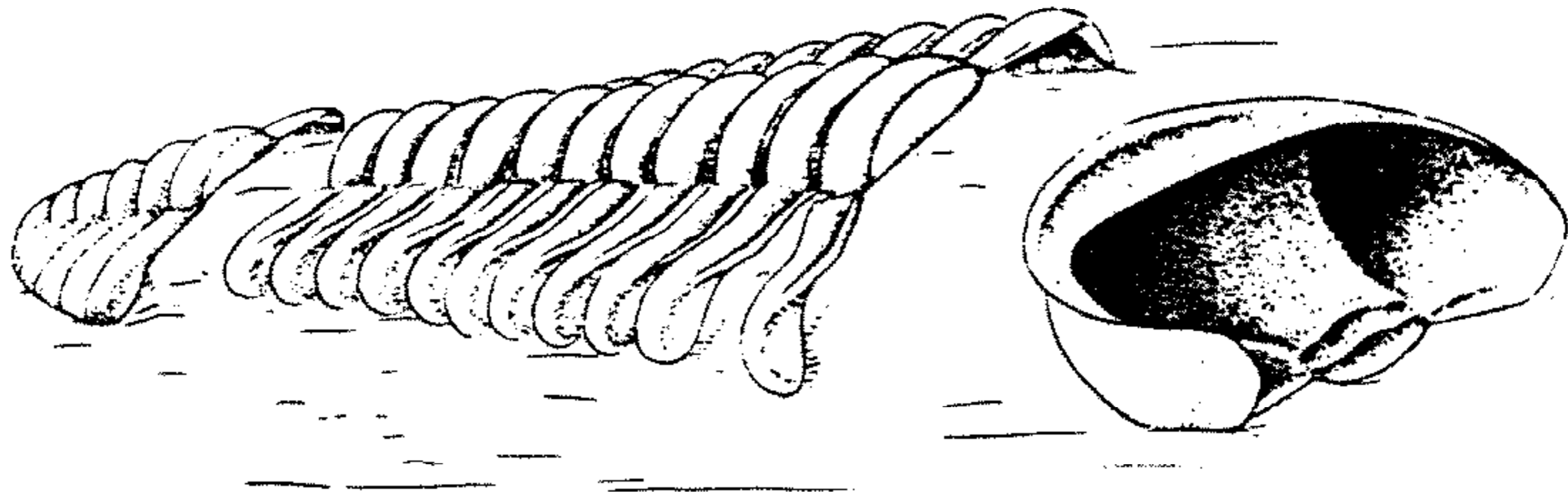
FIG. 83. Phacopid mode of ecdysis. Exuviae of Nephranops sp., U.Dev., Ger., showing thoracic and pygidial parts in normal position (ventral face downward), whereas the cephalon has rotated backward about 180° and lies upside down; as the facial sutures are nonfunctional, the librigenae remain attached to the cranidium (after 46).
