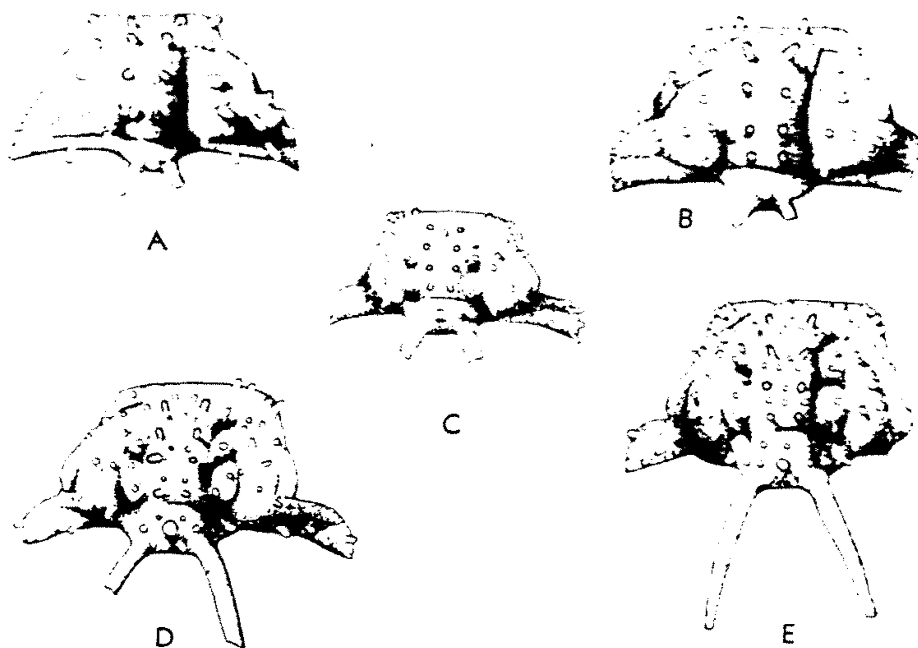
FIG. 103. Cranidia of Diacanthaspis cooperi WHITTINGTON, M.Ord., E.U.S.A. (Virginia); A-E, series showing growth stages, A, B, \times 50 , C-E, \times 25 (33*).
