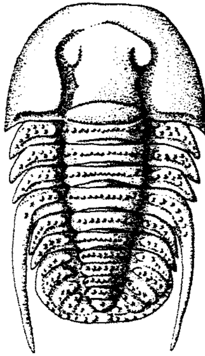
FIG. 183. Shumardia pusilla (SARS) (Shumardiidae), ?L.Ord.(Tremadoc.), Eng.; exoskel (reconstr.), \times 22.5 (475).
