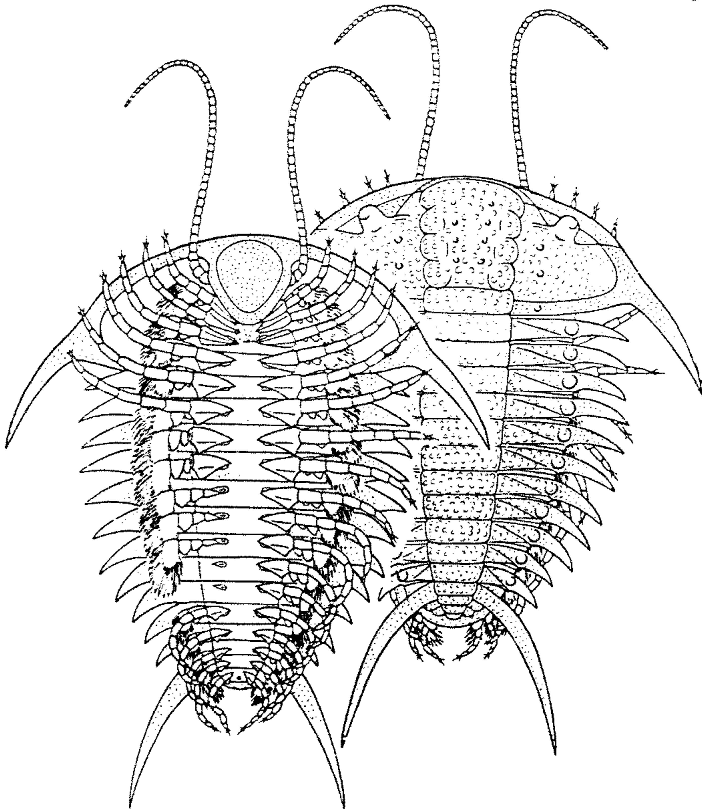
FIG. 61. Reconstruction of Ceraurus pleurexanthemus GREEN, M.Ord., USA(N.Y.), \times 2.15 (after 60).
