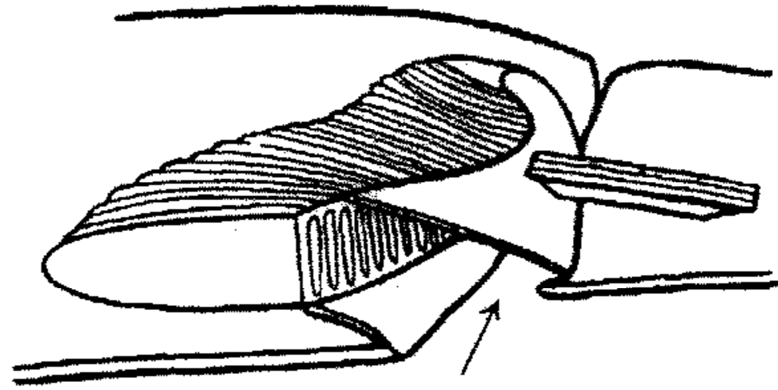
FIG. 9. Lung books of an arachnid (Phrynichida). (After Kästner.)
