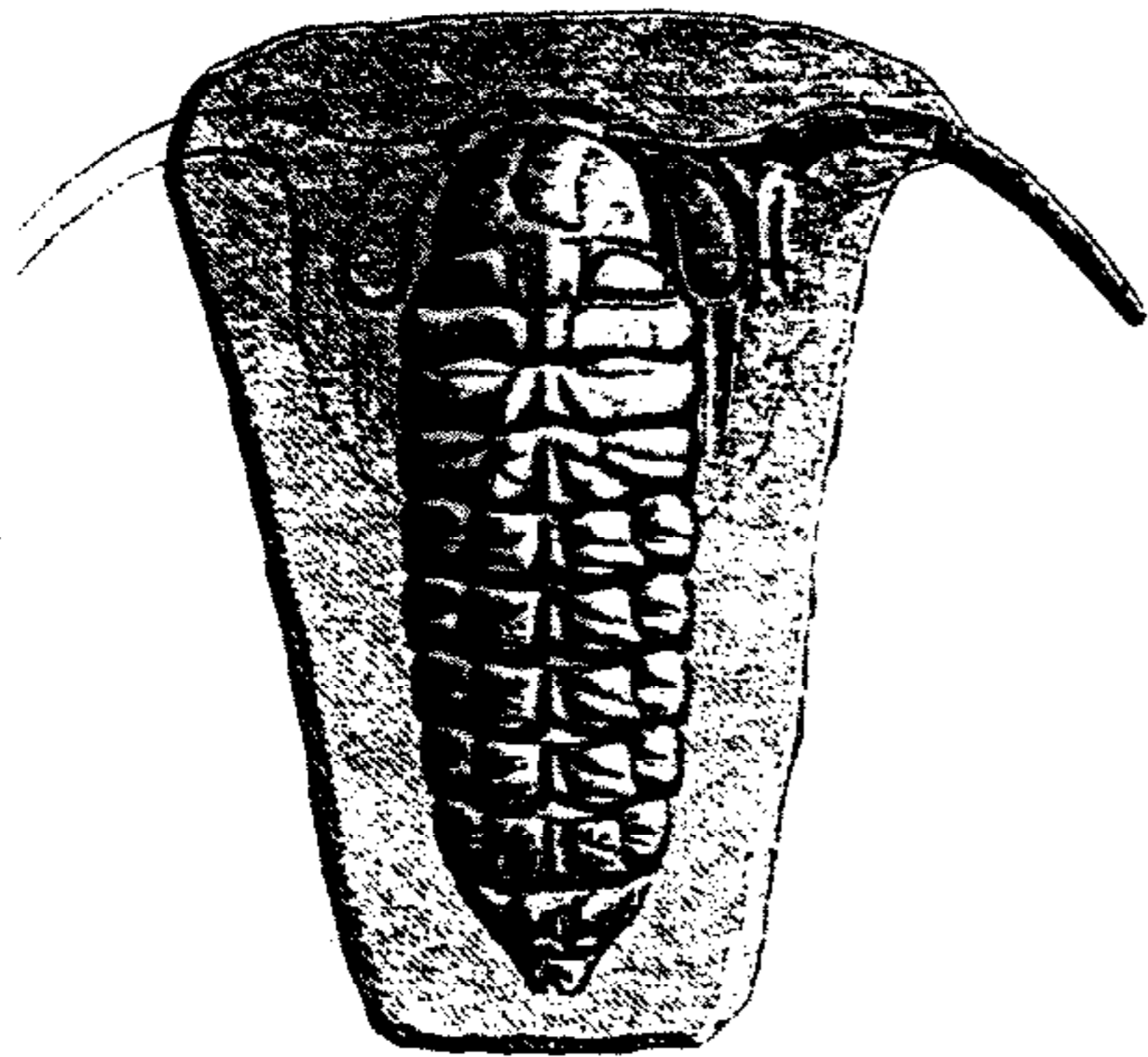
FIG. 415. * Bohemilla stupenda BARRANDE (Bohemilidae), Ord. (D gamma 2), St. Benigna, Boh.; exoskel. (restored), \times 3 (4).
