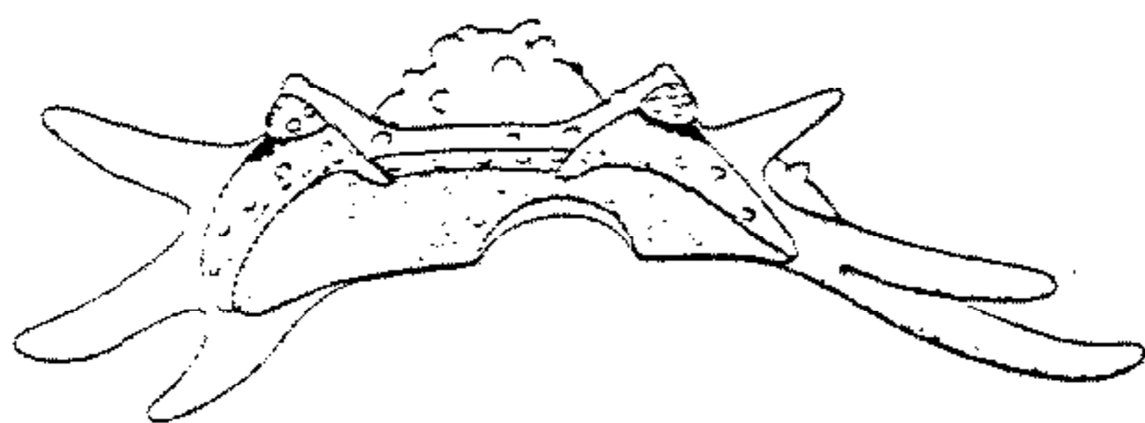
FIG. 106. Cranidium of Acanthoparypha chiropyga WHITTINGTON & EVITT, M.Ord., E.USA (Virginia); specimen showing librigenae and rostral plate, \times 65 (37*).
