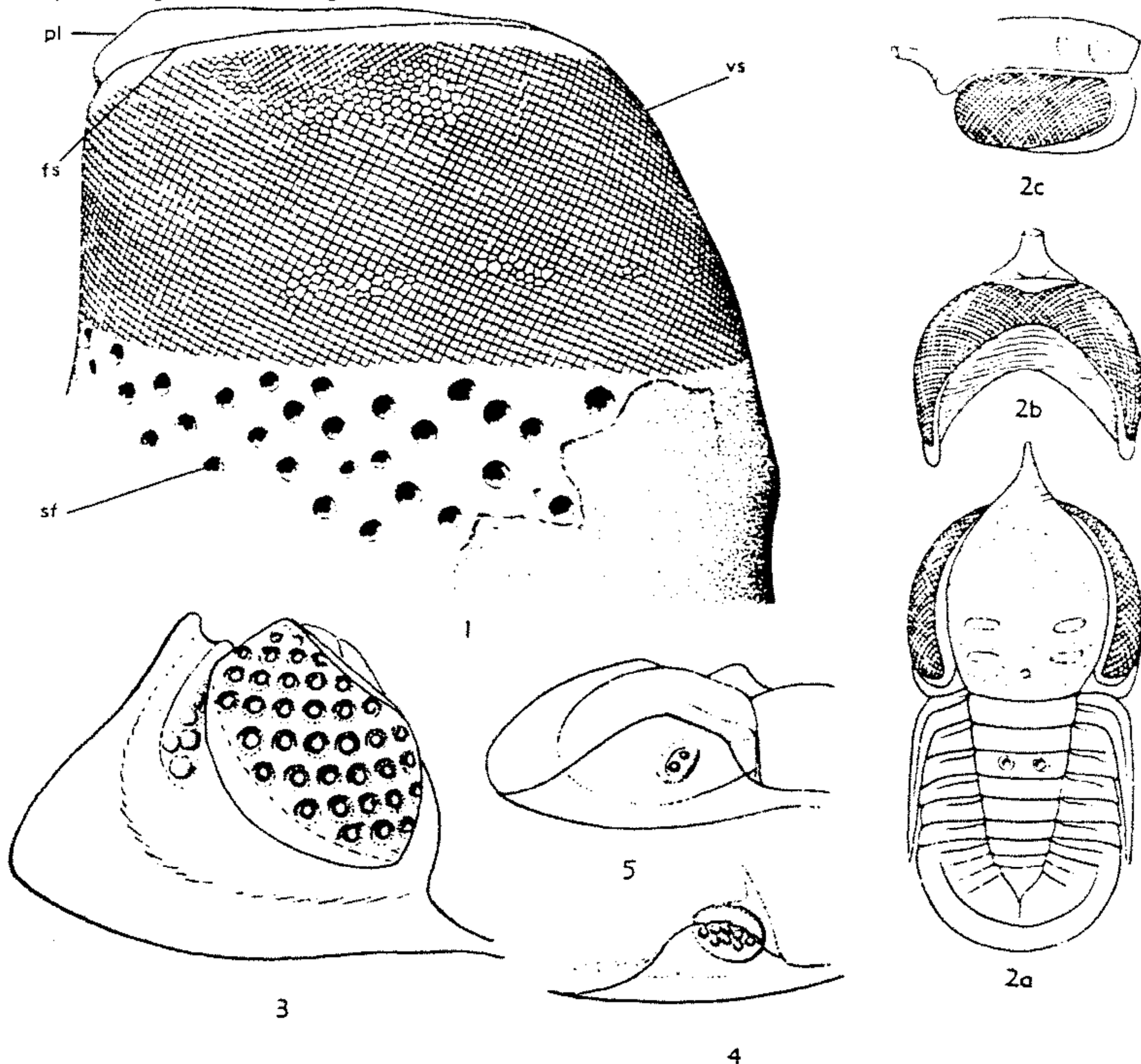
FIG. 64. Eyes of trilobites.—1. Holochroal eye of Asaphus cornutus PANDER, Ord., Russia, X25 (after 24). (Explanation: fs , facial suture; sf , sensorial fossette; pl , palpebral lobe; vs , visual surface.)—2. Confluent eyes of Symphysops subarmatus (REED) RAYMOND, U.Ord., G.Brit., X1.2; 2a, dorsal view of carapace; 2b, ventral view of cephalon; 2c, lateral view of cephalon (after 26).—3. Right eye of Phacops latifrons (BRONN), M.Dev., Ger., X2.5 (after 45).—4. Right eye of Cryphops cryptophthalmus (EMMIRICH), U. Dev., Ger., X7 (after 45).—5. Left eye of Nephranops incisus incisus (ROEMER), U.Dev., Ger., X2 (after 45).
