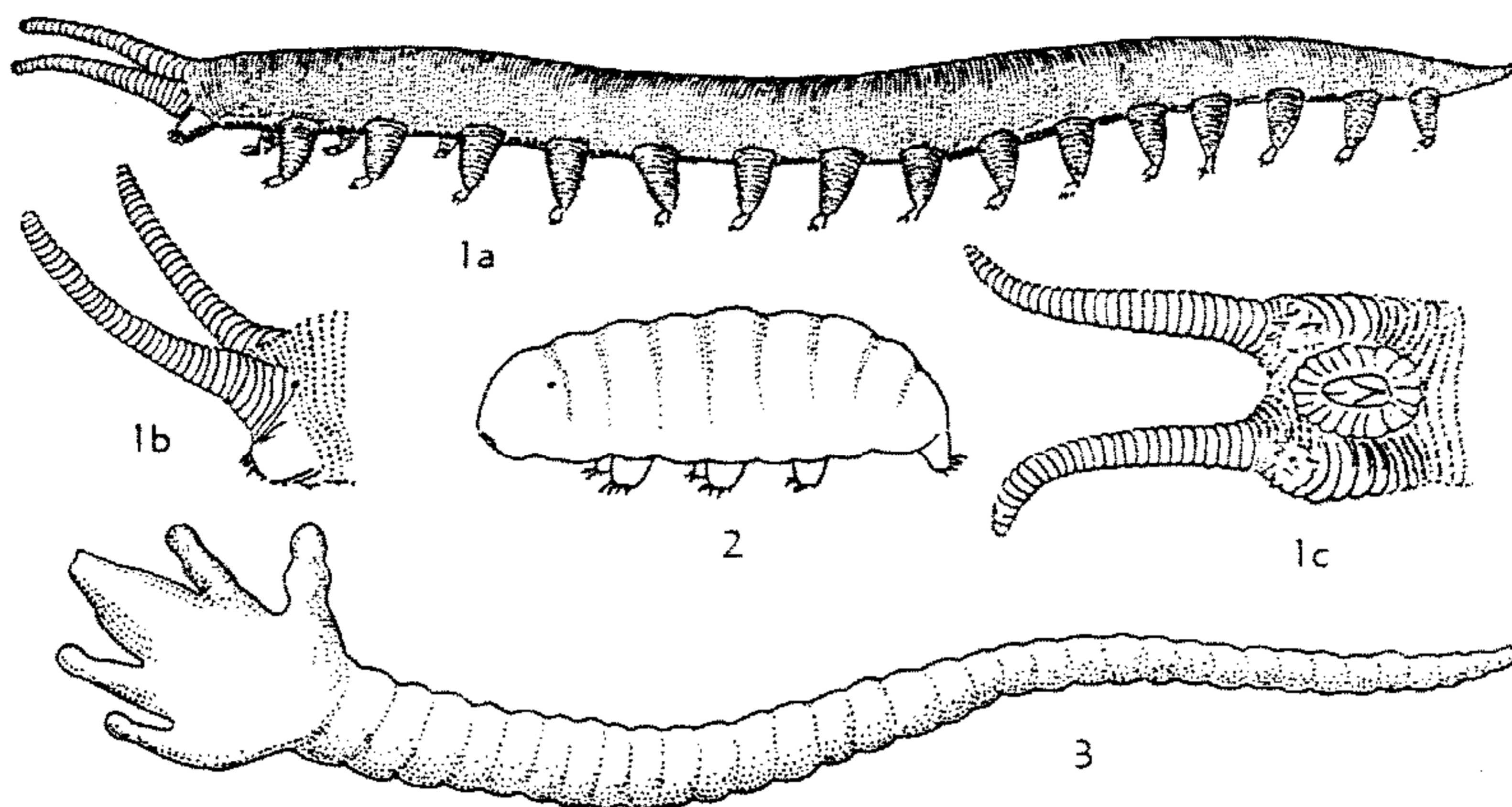
FIG. 11. Types of living Pararthropoda.—1. Onychophora; 1a, Peripatus , from South Africa, side view of whole animal, \times 2 ; 1b,c, side and ventral views of same, \times 2.5 (Mod. from Snodgrass).—2. Tardigrada; Macrobiotus from side, a cosmopolitan genus, \times 60 (Mod. from Cuenot).—3. Pentastomida; Cephalobuena , parasite in lungs of snakes, \times 4 (Mod. from Heymons).
