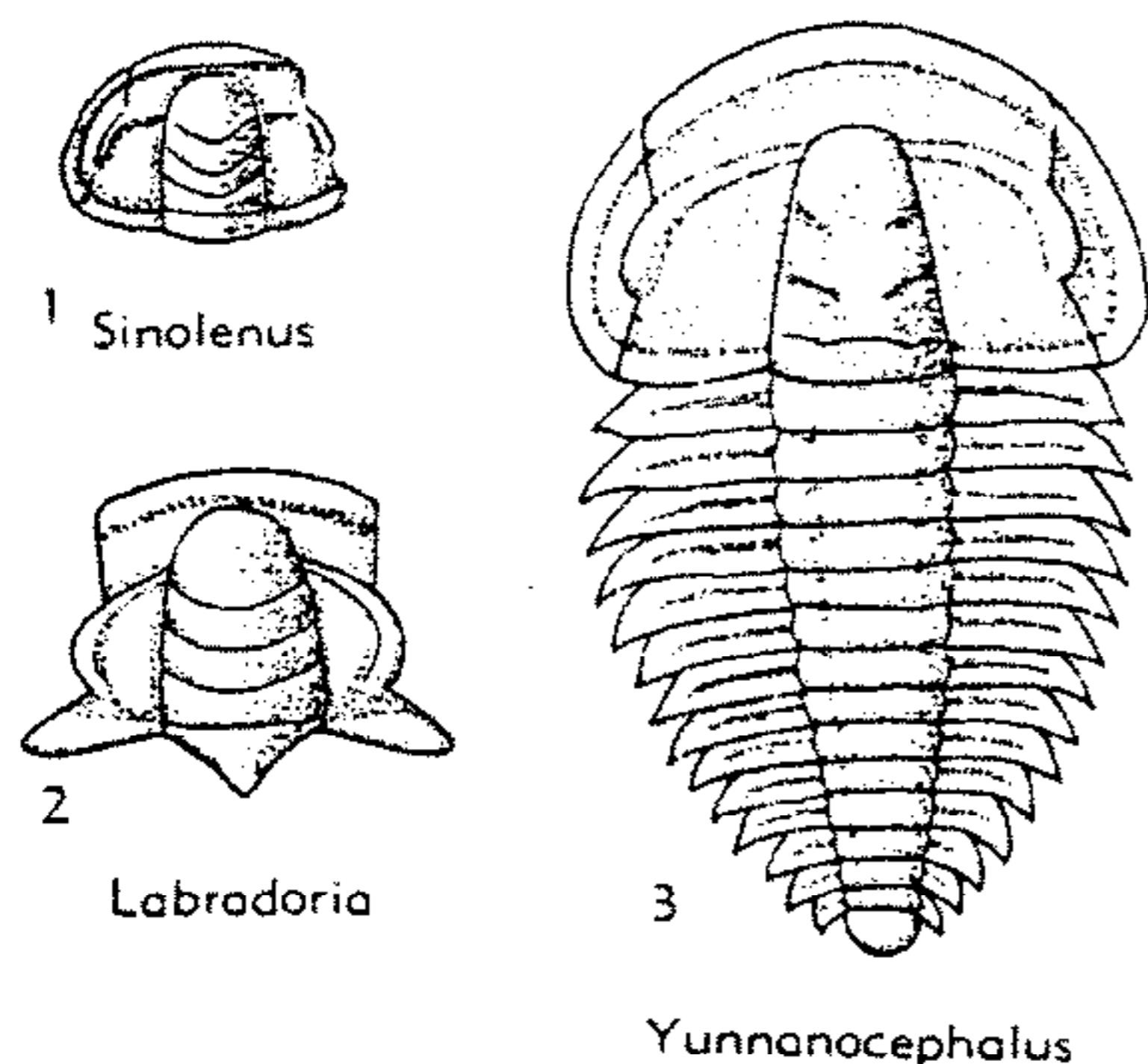
FIG. 152. Yunnanocephalidae, Ellipsocephalacea (Family uncertain) (p. 0212).
