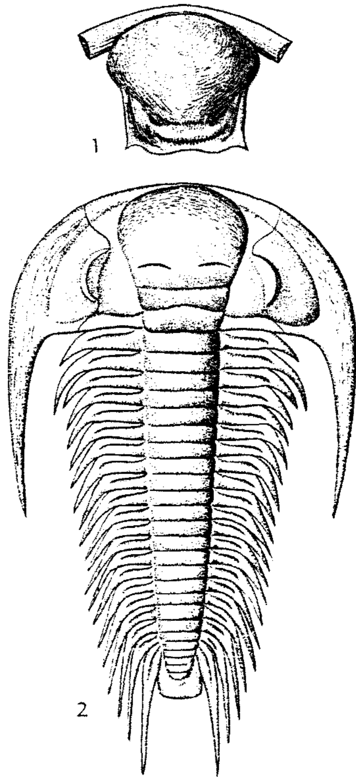
FIG. 153. Paradoxides (Paradoxididae, Paradoxidinae), M.Cam. —1. P. minor (BOECK), Bohemia; rostral plate with hypostoma, \times 3 (3).—2. * P. paradoxissimus (WAHLENBERG), Swed.; exoskel., \times 0.5 (1).
