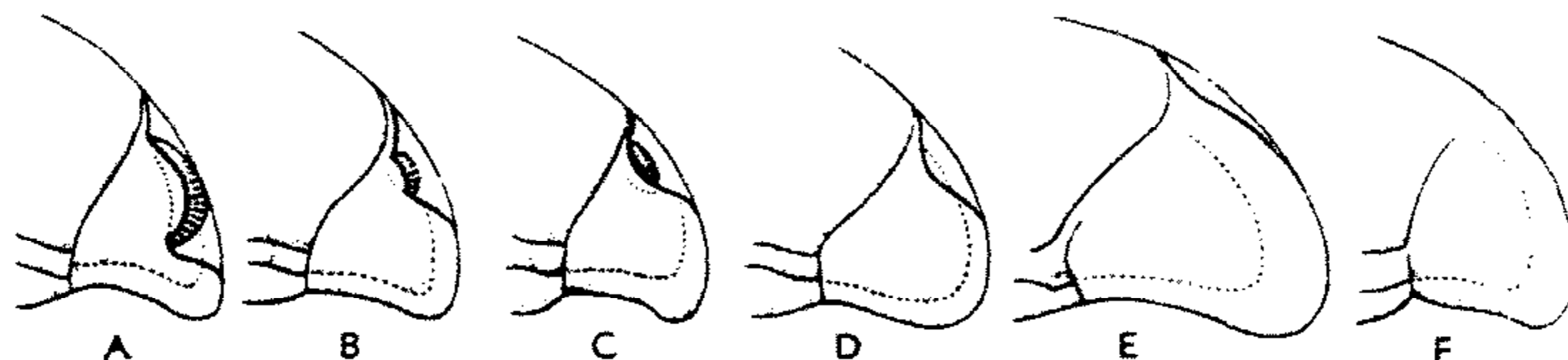
FIG. 47. Lateral migration of the facial sutures accompanying migration, reduction, and disappearance of the eyes in the Phacopidae.—A. Phacops circumspectans PORTLOCK, U.Dev., Ger.—B. Phacops wedekindi RICHTER & RICHTER, U.Dev., Ger.—C. Cryphops? ensae (RICHTER & RICHTER), U.Dev., Ger.—D. Trimerocephalus mastophthalmus (REINH. RICHTER), U.Dev., Ger.—E. Dianops limbata (REINH. RICHTER), U.Dev., Ger.—F. Ductina ductifrons (RICHTER & RICHTER), U.Dev., Ger. (All after 47.)
