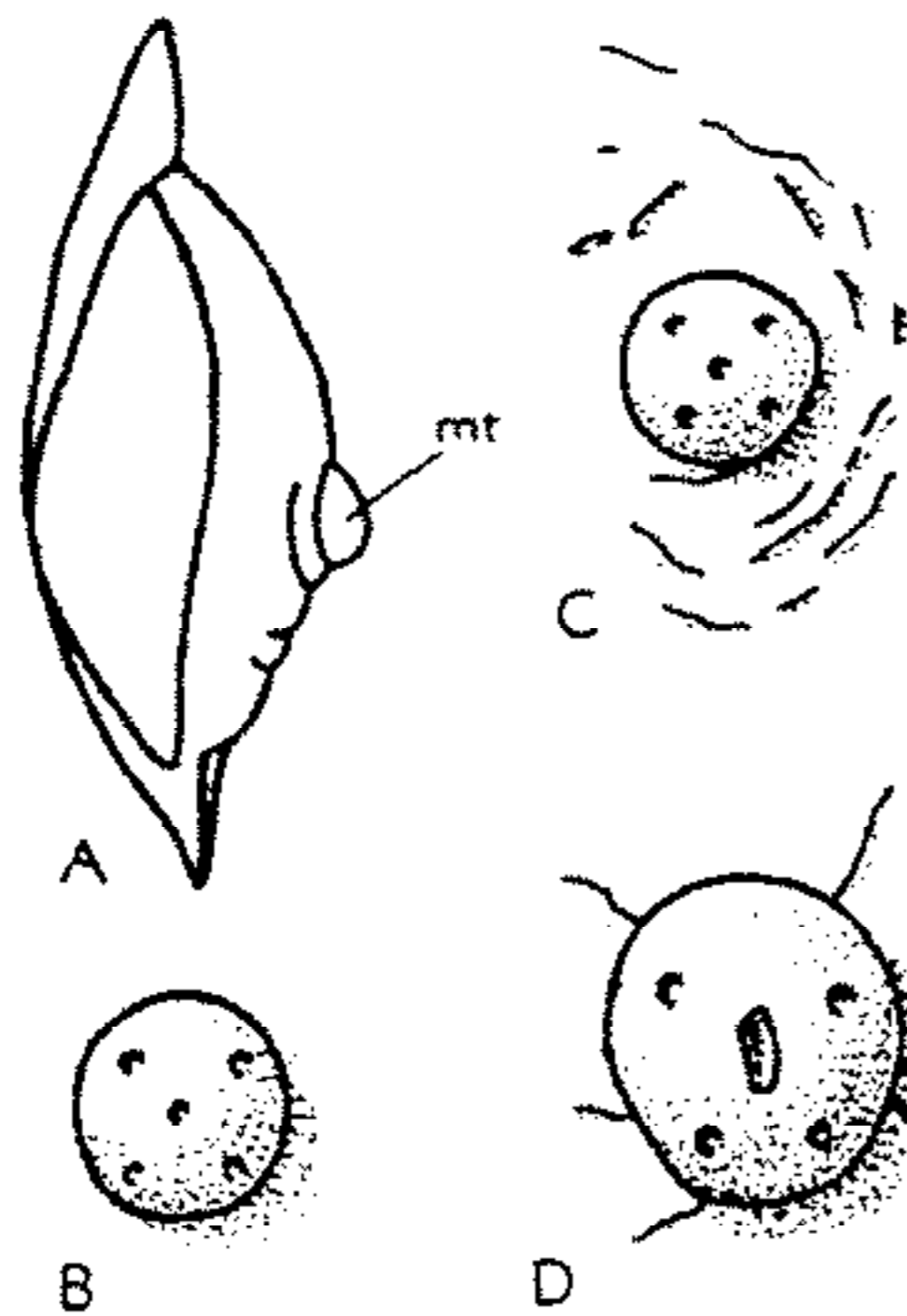
FIG. 67. Median glabellar tubercle of Tretaspis seticornis (HISINGER) STØRMER, Ord., Norway (after 55). A, Lateral view of meraspid cephalon (stage II) showing median tubercle ( mt ), \times 36 ; B, dorsal view of median tubercle of same cephalon, \times 80 ; C, D, dorsal views of median tubercle of 2 holaspid cephalata, \times 50 .
