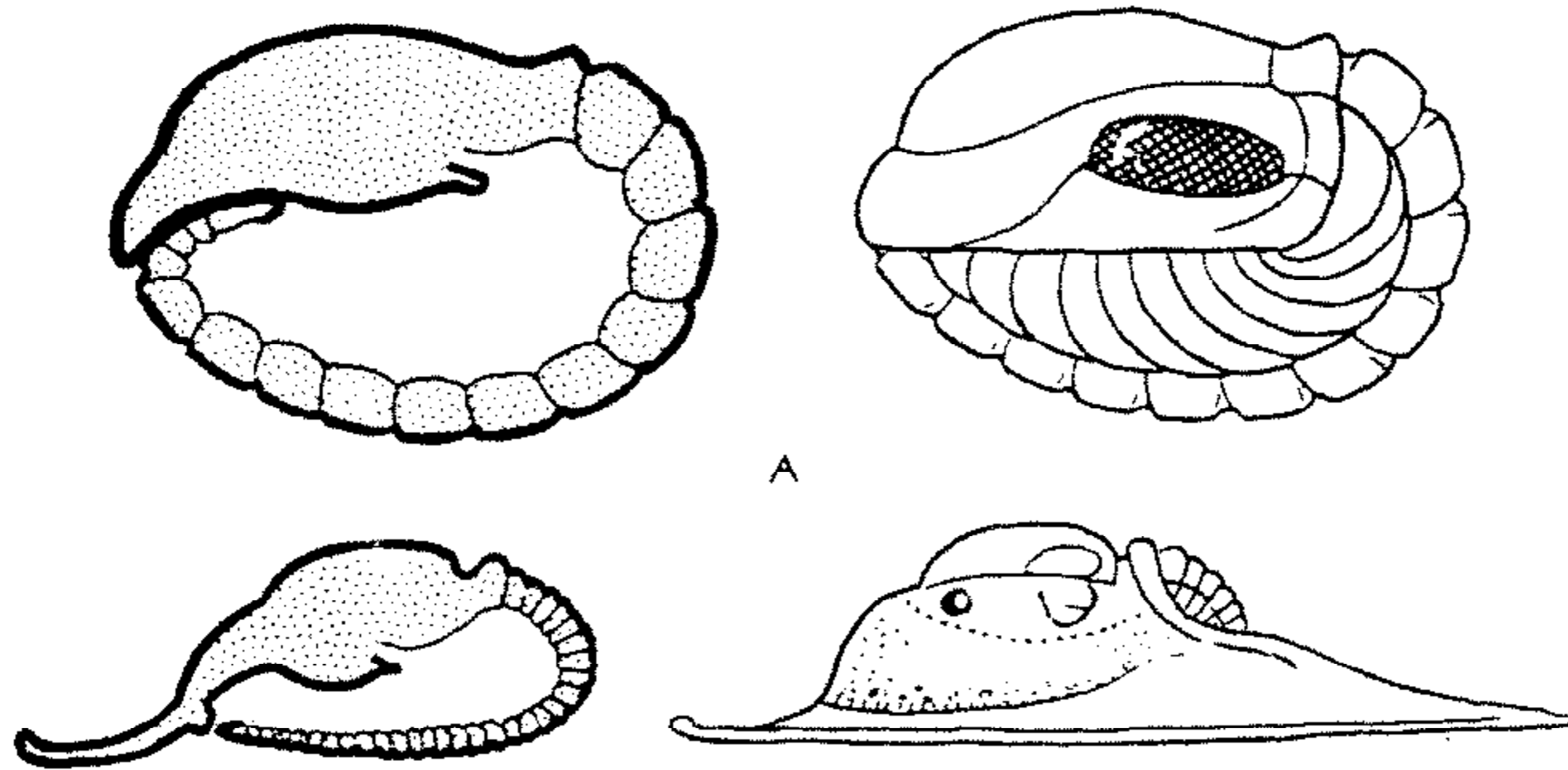
FIG. 76. Double and discoidal enrollment; right side, lateral view of enrolled specimens; left side, sagittal section of enrolled specimens.—Double enrollment (above), Ellipsocephalus polytomus LINNARSSON, M. Cam., Swed., \times 8.25 (data from 68).—Discoidal enrollment (below), Harpes macrocephalus GOLDFUSS, M.Dev., Ger., \times 1.25 (right side, after 86, 1921).
