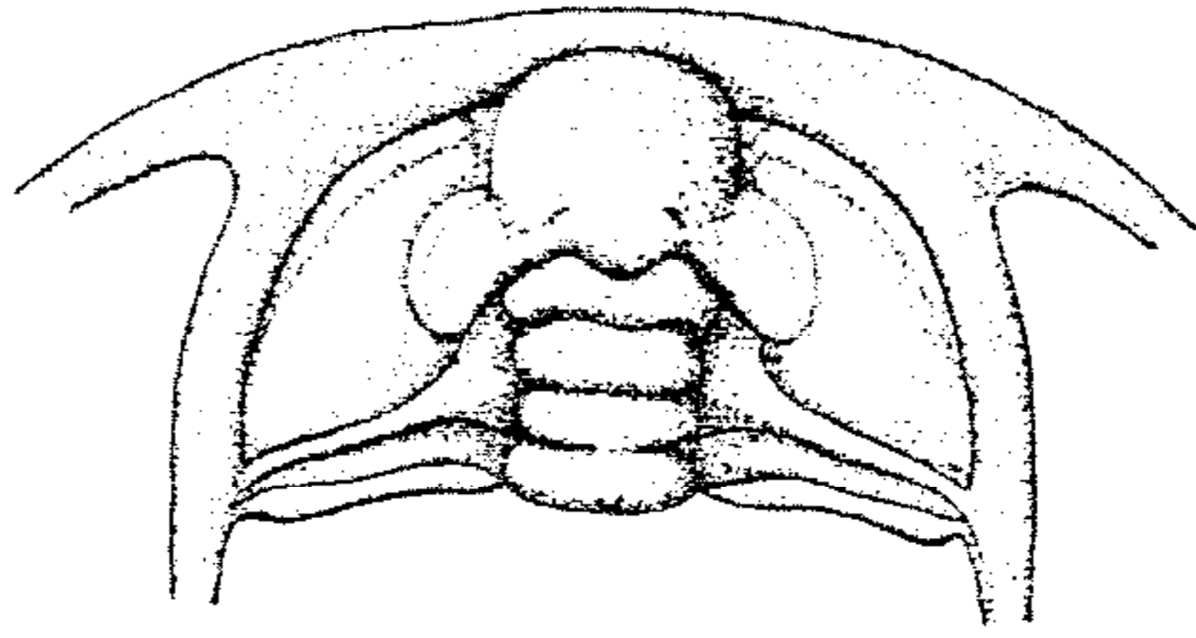
FIG. 134. *Laudonia bispinata HARRINGTON (Olenellinae), L.Cam. , W. Can. (B.C.); cephalon, \times 3 (56).
