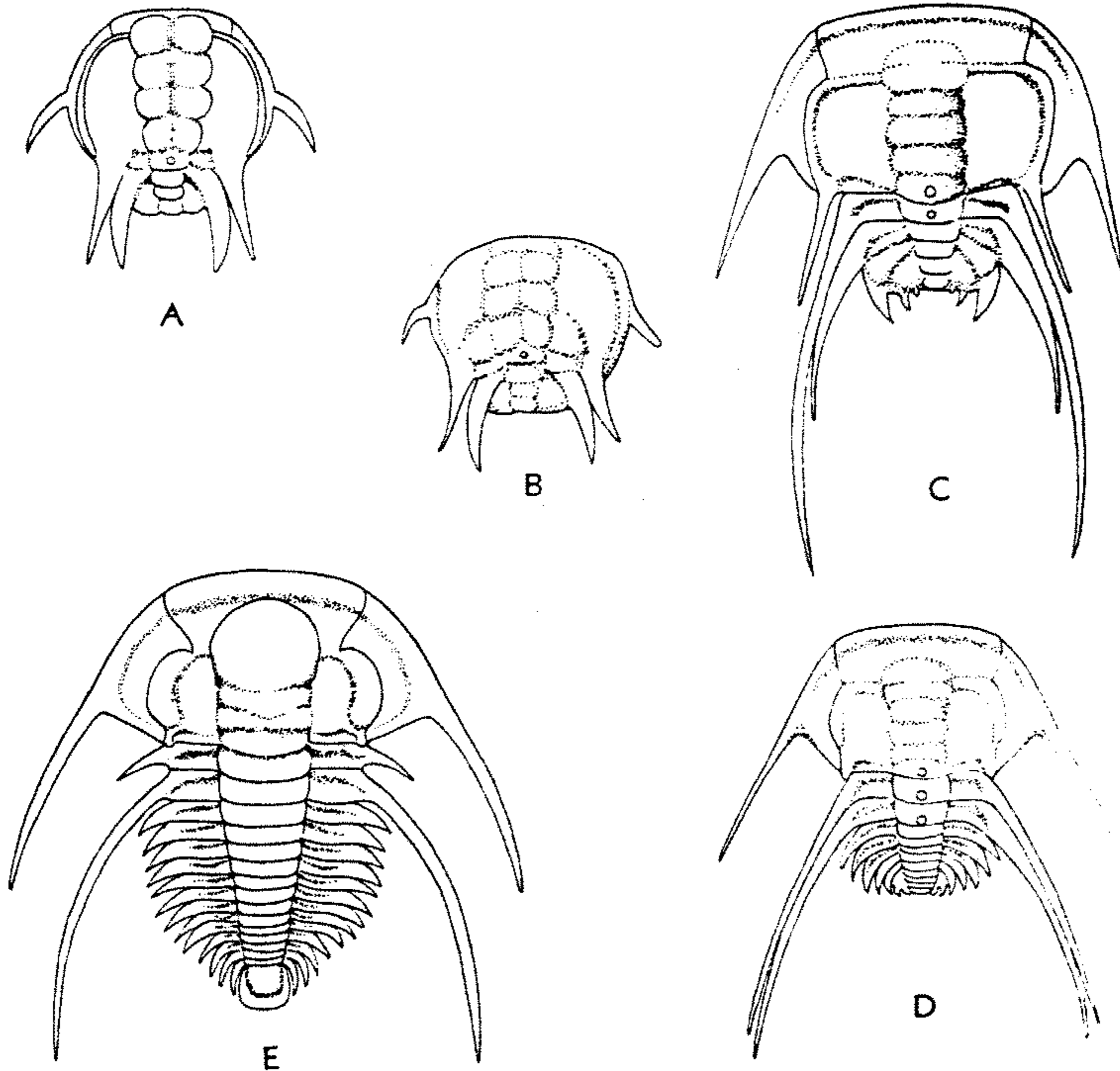
FIG. 93. Ontogenetic stages of Paradoxides pinus HOLM, M.Cam., Swed.; A, B, protaspides (A, reconstr.), \times 20 ; C-E, meraspid "degree" 1, \times 20 ; "degree" 4, \times 10 , "degree" 15, \times 5.4 (30).
