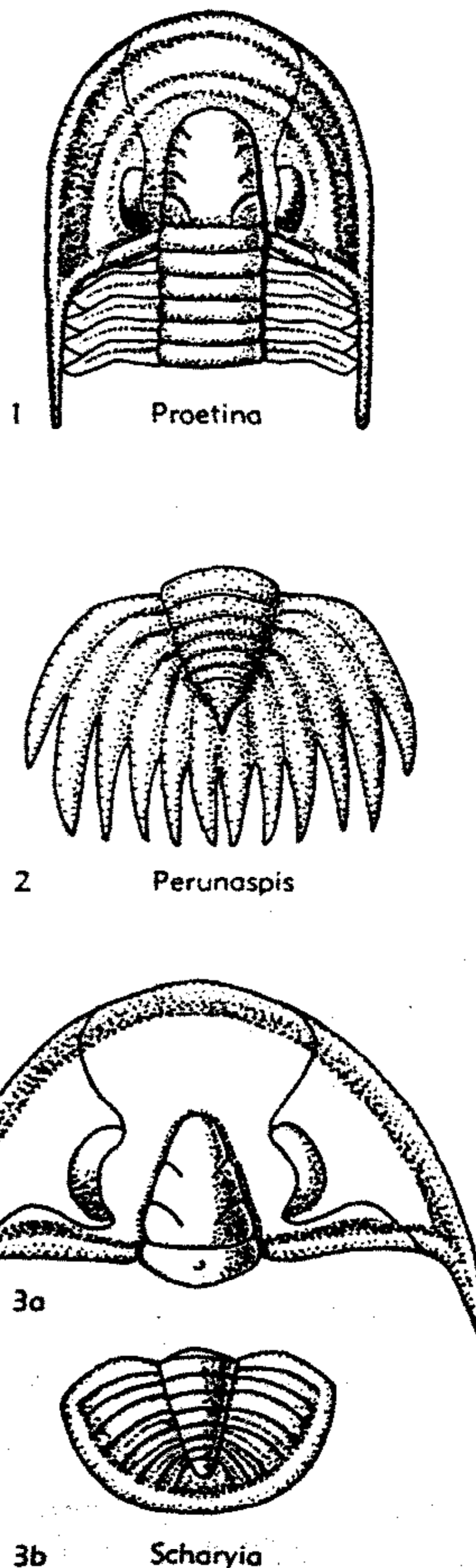
FIG. 317. Proetacea (Family Uncertain) (p. 0413, 0415).
