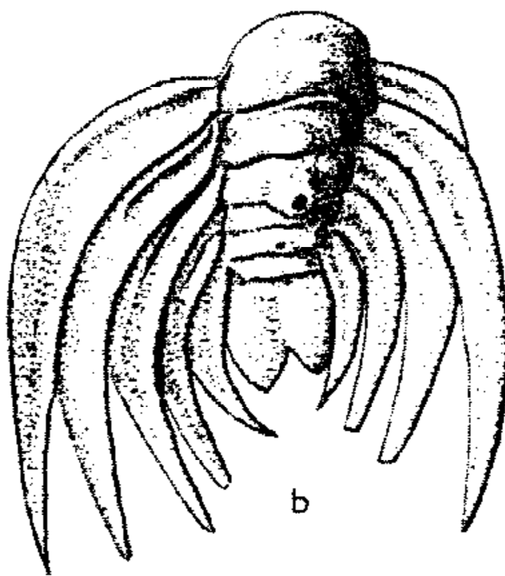
FIG. 139. *Wanneria walcottana (WANNER) (Olenellidae, Wanneriinae), L. Cam. , E. USA (Pa.); a , dorsal exoskel., \times 0.7 ; b , pyg. and part of thorax, \times 2 ; c , posterolateral part of hypostoma, \times 6 (312).
