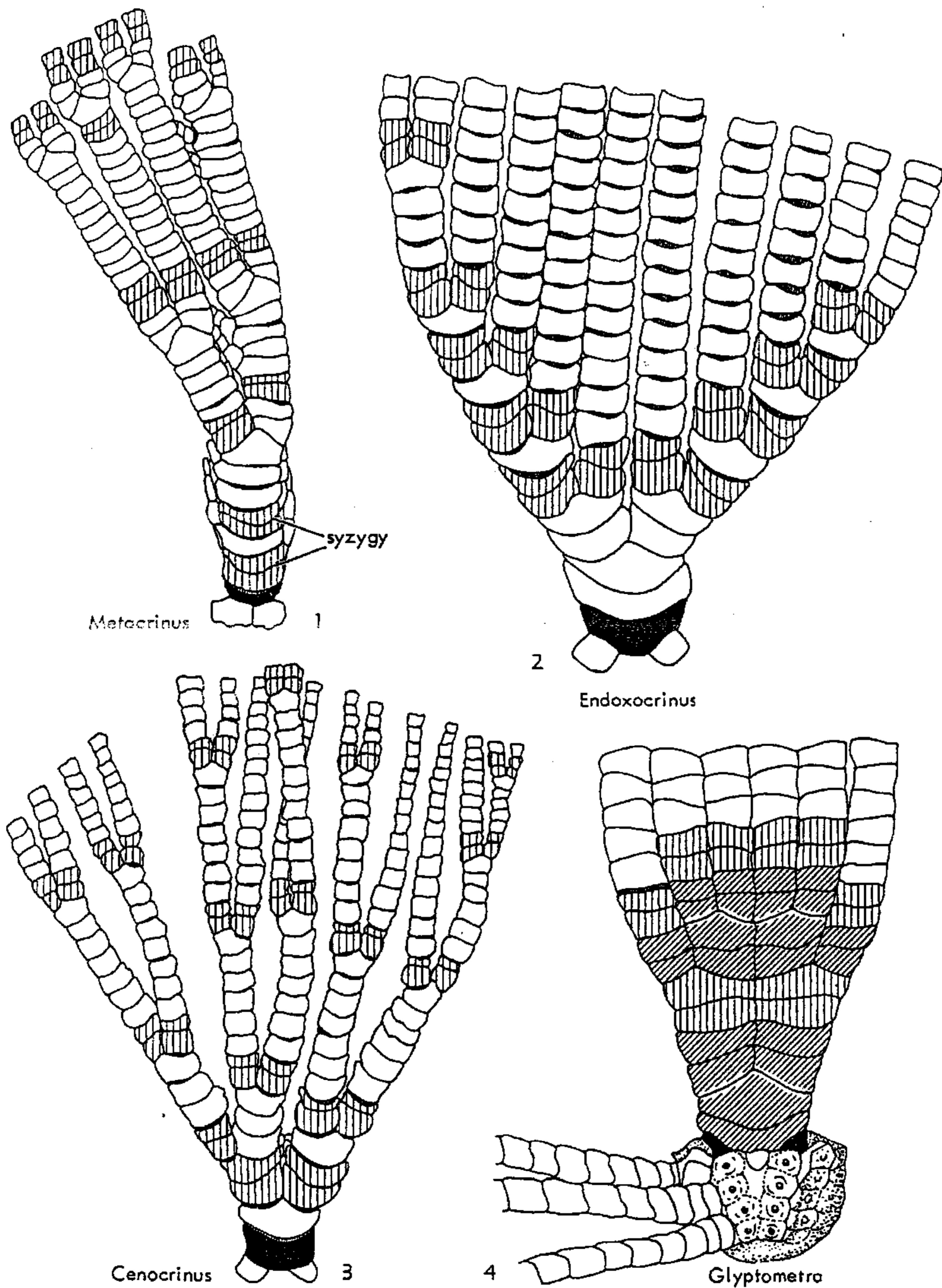
FIG. 20. Types of arm ramification in recent crinoids with distribution of synarthrial (oblique ruled) and syzygial (vertical ruled) brachial pairs.
