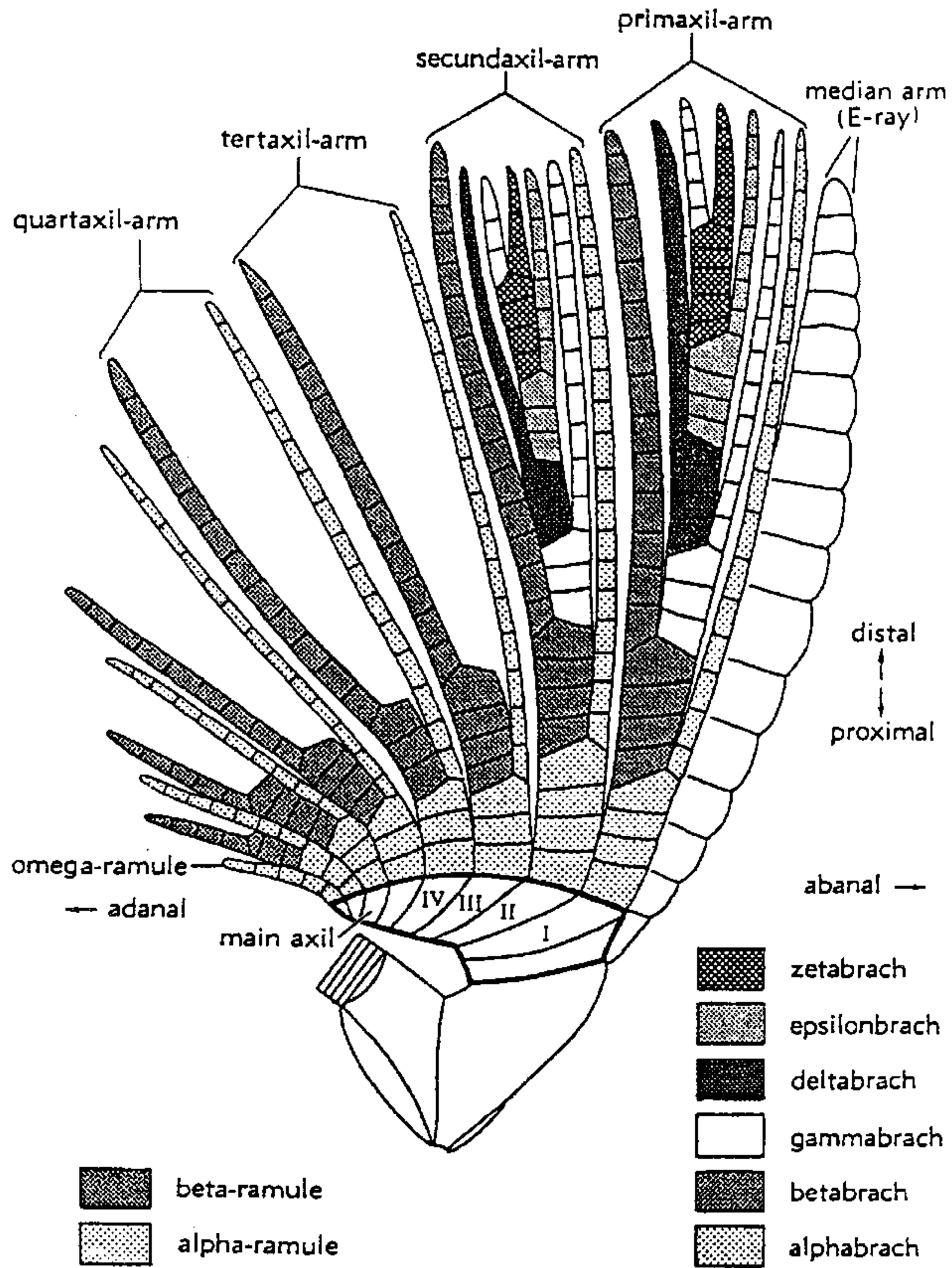
FIG. 121. Nomenclature applied to arm branching in lateral (A and D) rays of Calceocrinidae (Moore, 1962a).
