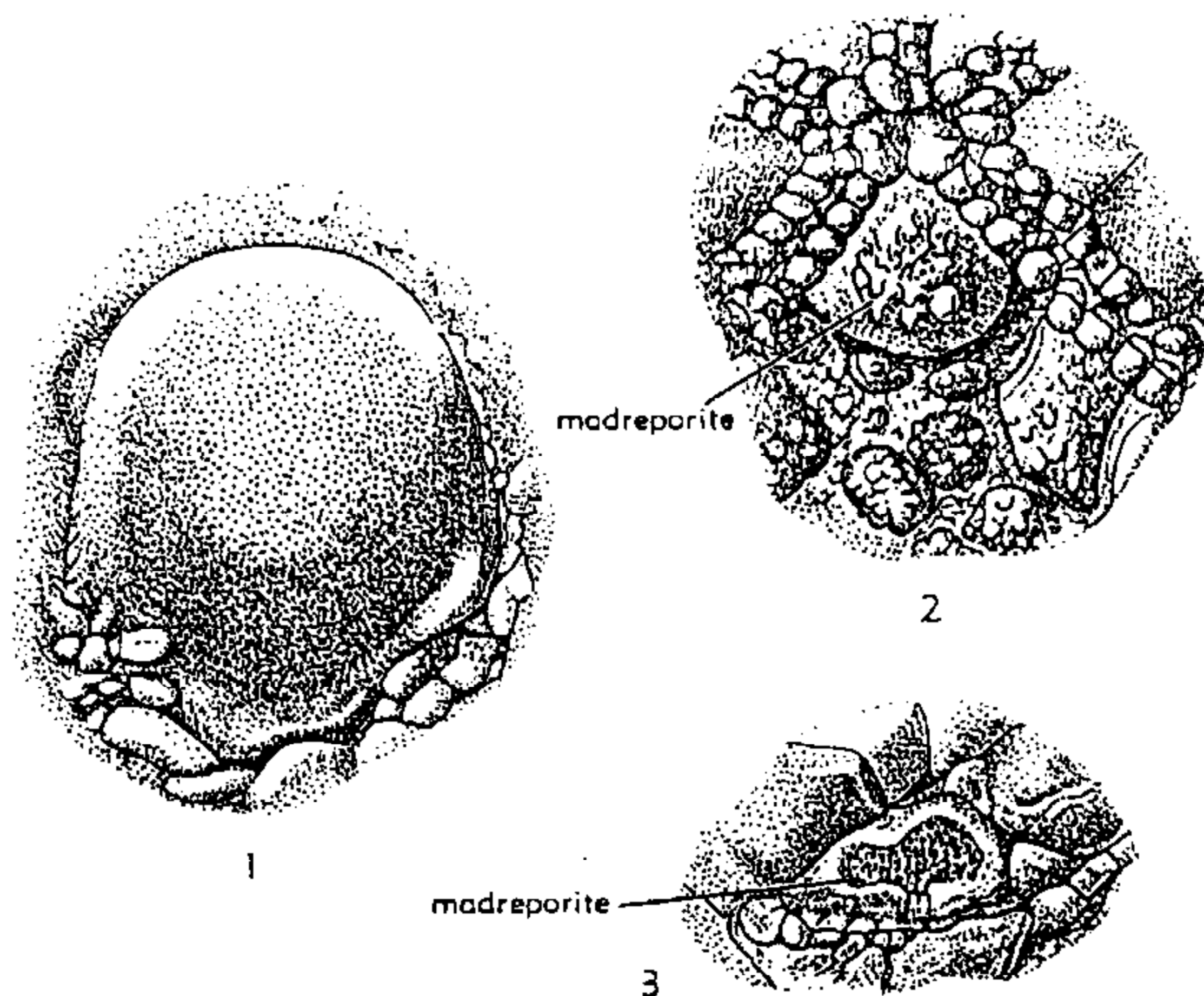
FIG. 165. Morphology of the madreporite.—1. Aexitrochocrinus jaekeli MOORE & PLUMMER, L. Carb., Scot., USSR; \times 6 (Springer, 1920).—2. Gissocrinus incurvatus (ANGELIN), U.Sil., Gotl.; \times 6 (Bather, 1893a).—3. Euspirocrinus spiralis ANGELIN, U.Sil., Gotl.; \times 6 (Bather, 1893a).
