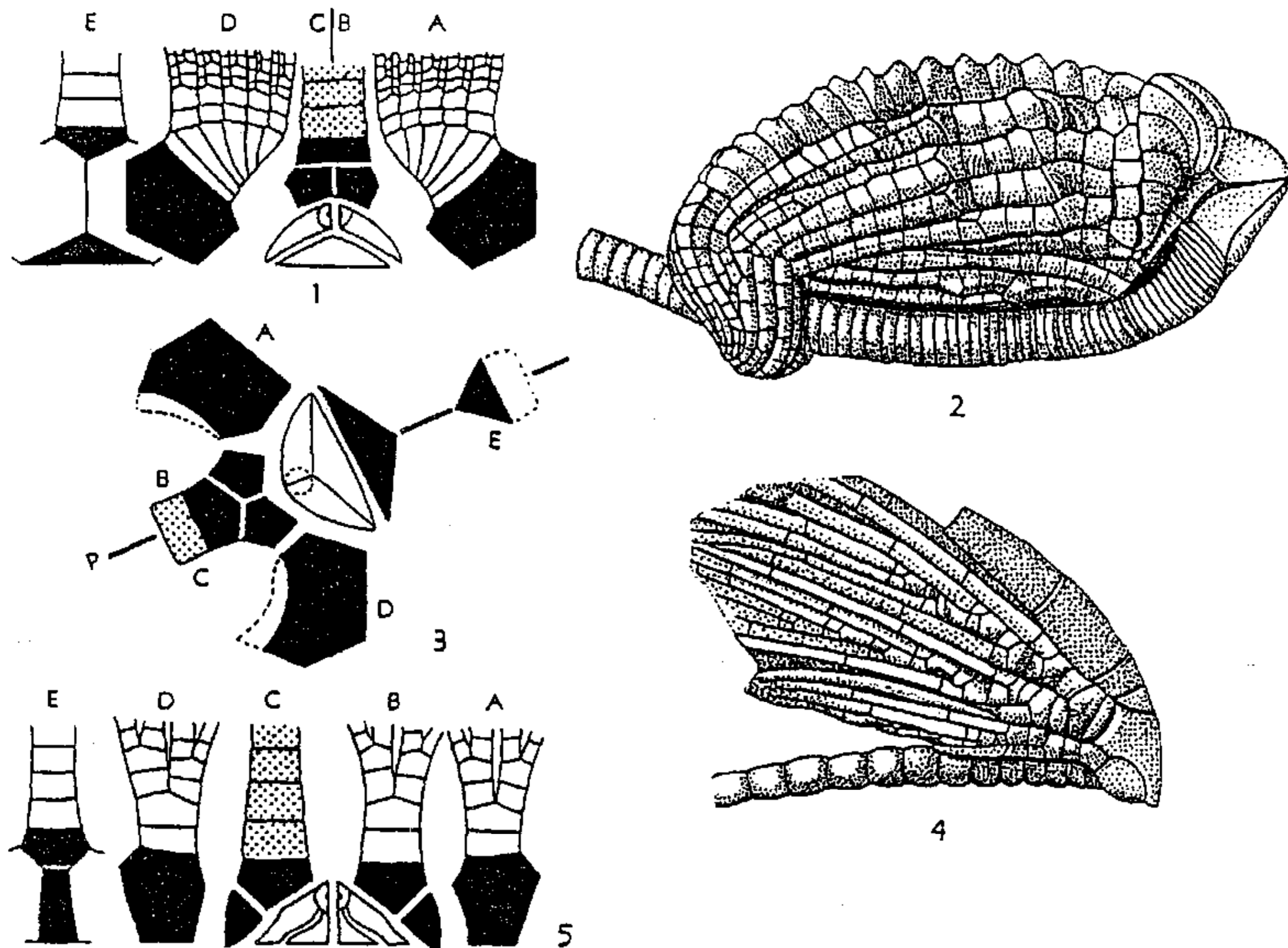
FIG. 87. Inequality of radials in relation to unequal arms in Calceocrinidae (Disparida). [Explanation: P, plane of bilateral symmetry; radials and biradials black; anal plates stippled; rays identified by letter symbols of CARPENTER system.]
