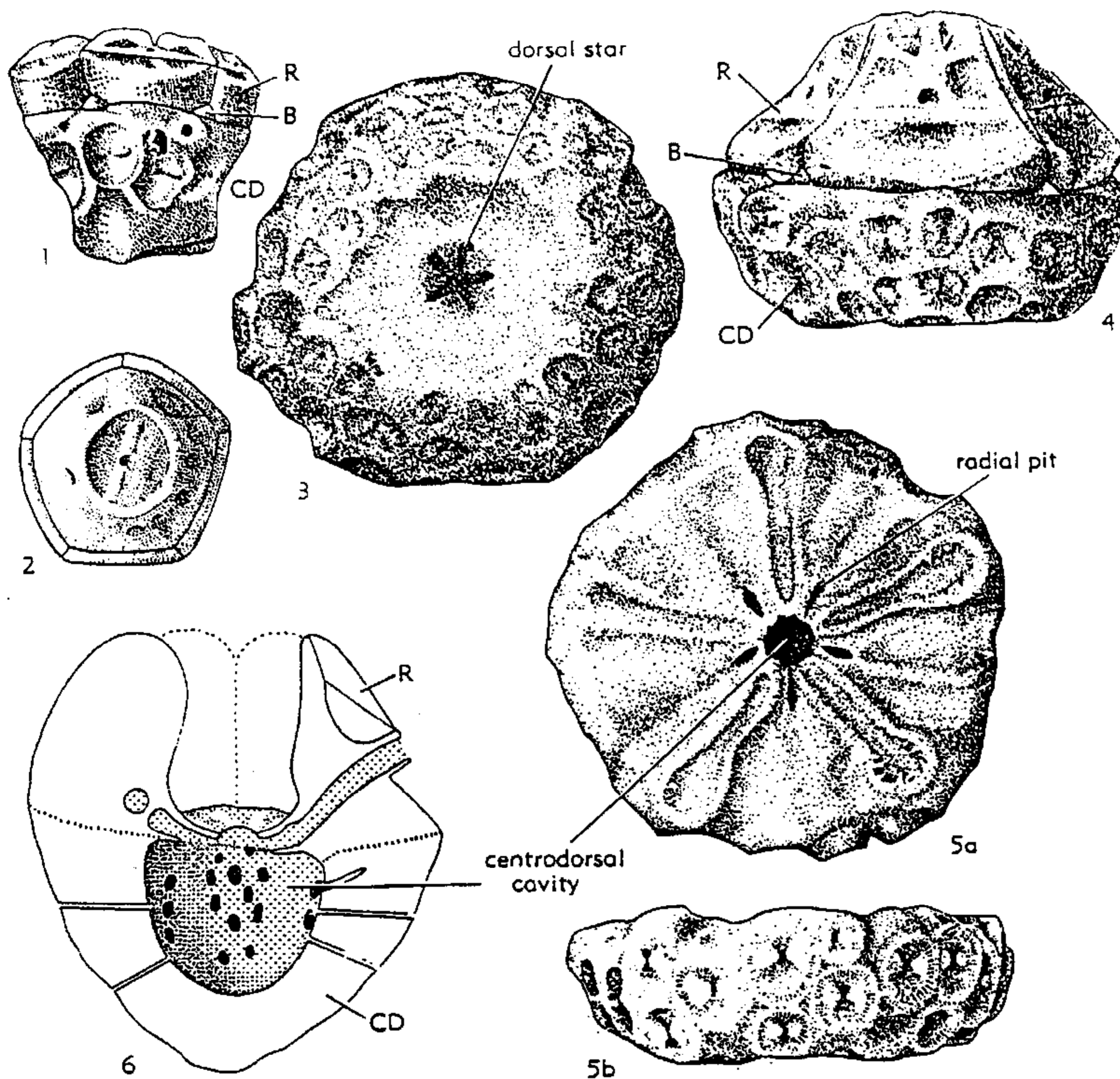
FIG. 52. Morphology of centrodorsal. [Explanation: B, basal; CD, centrodorsal; R, radial.]
