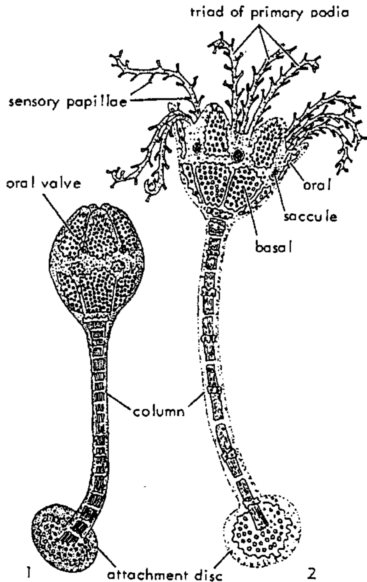
FIG. 39. Morphogenesis of cystidean stages in Antedon .—1. Early growth stage (after Thomson, 1865).—2. Late growth stage (after Clark, 1921).
