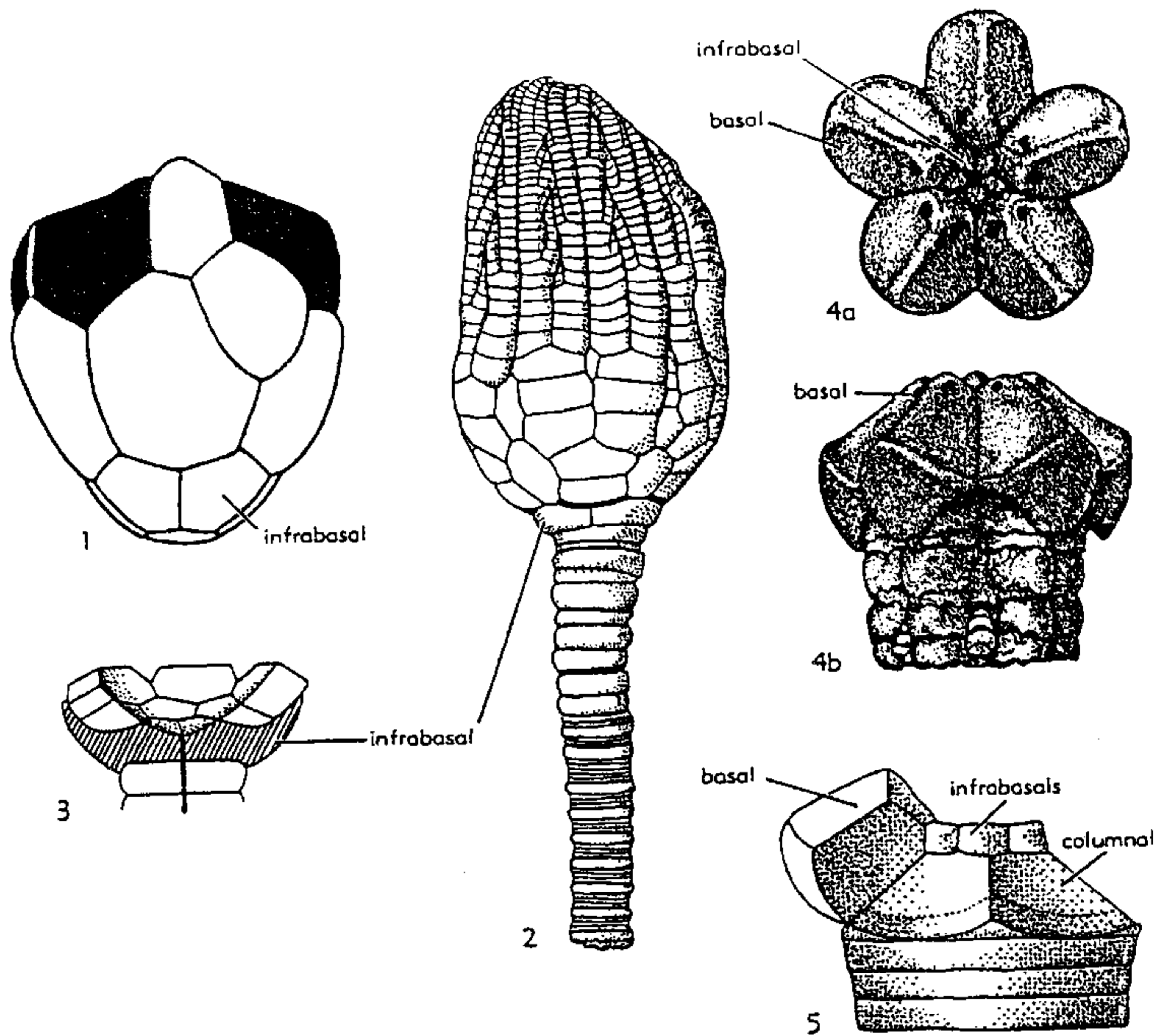
FIG. 73. Morphology of infrabasals. [Explanation: radials black.]
