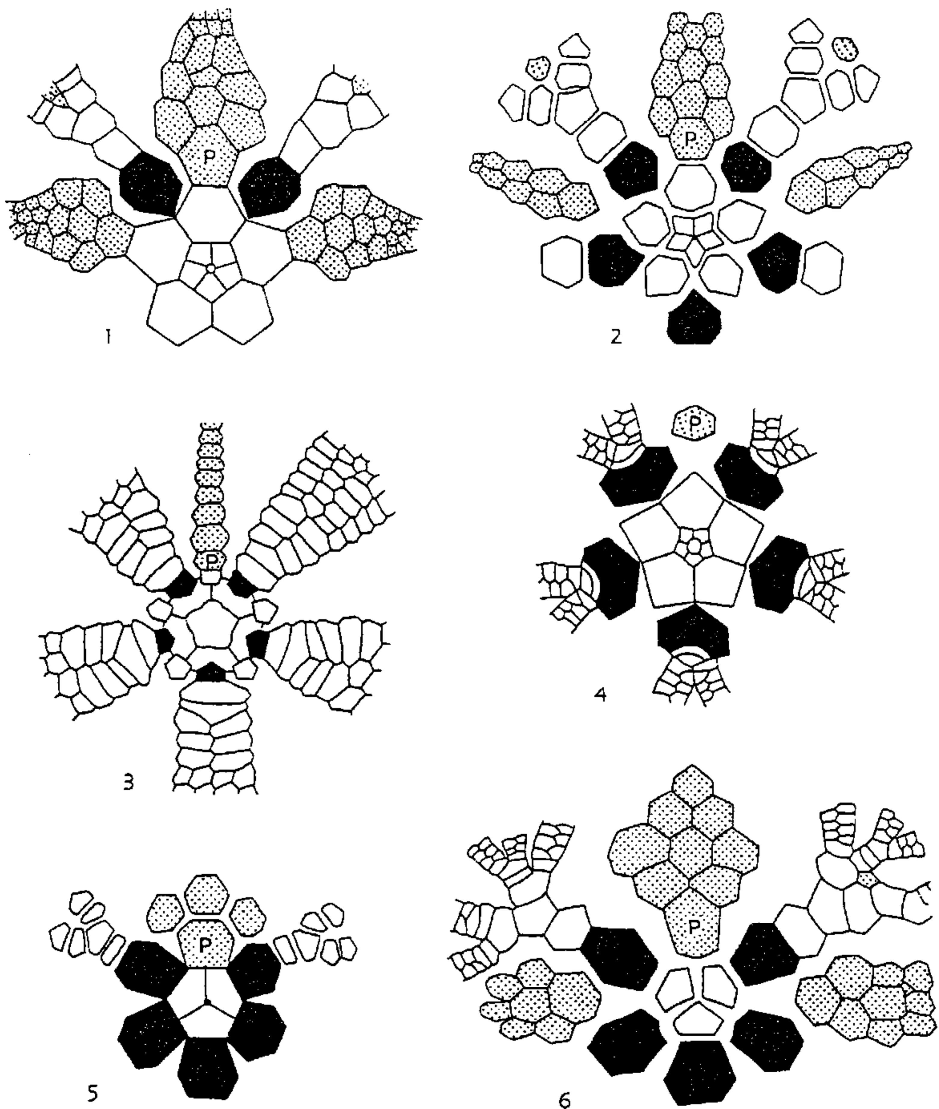
FIG. 99. Relations of primanal in camerates shown by plate diagrams (Ubaghs, n). [Explanation: radials black; anal plates, interbranchials stippled; P, primanal.]
