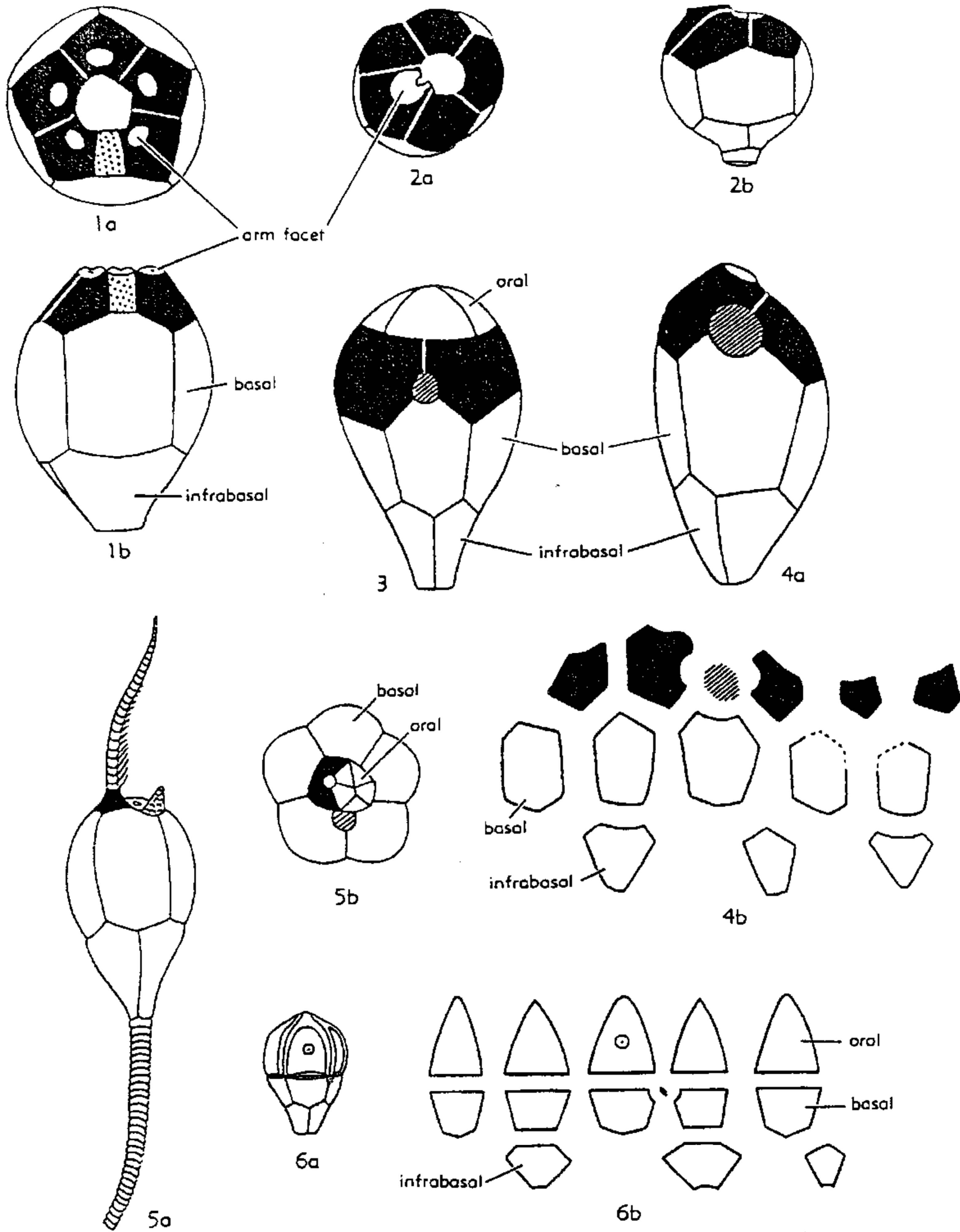
FIG. 86. Reduction of arms and radials in some Codiocrinacea. [Explanation: radials black, anal plate stippled; anus obliquely ruled. Circle with central dot in 6a,b represents the hydropore, the gonopore, or a common hydropore-gonopore.]
