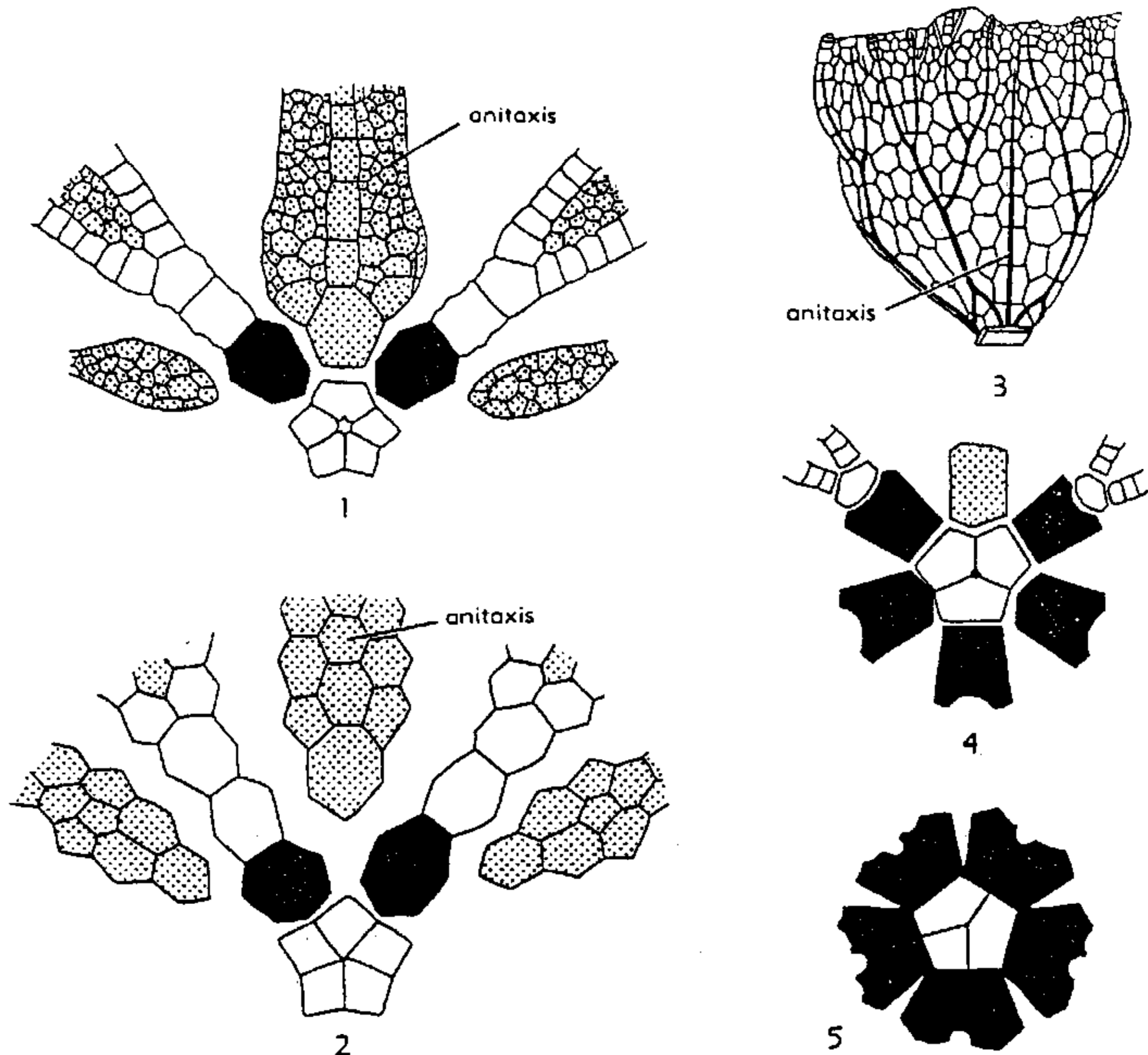
FIG. 98. Anal plate structure of camerates (Ubaghs, n). [Explanation: radials black; anals, interbranchials stippled.]
