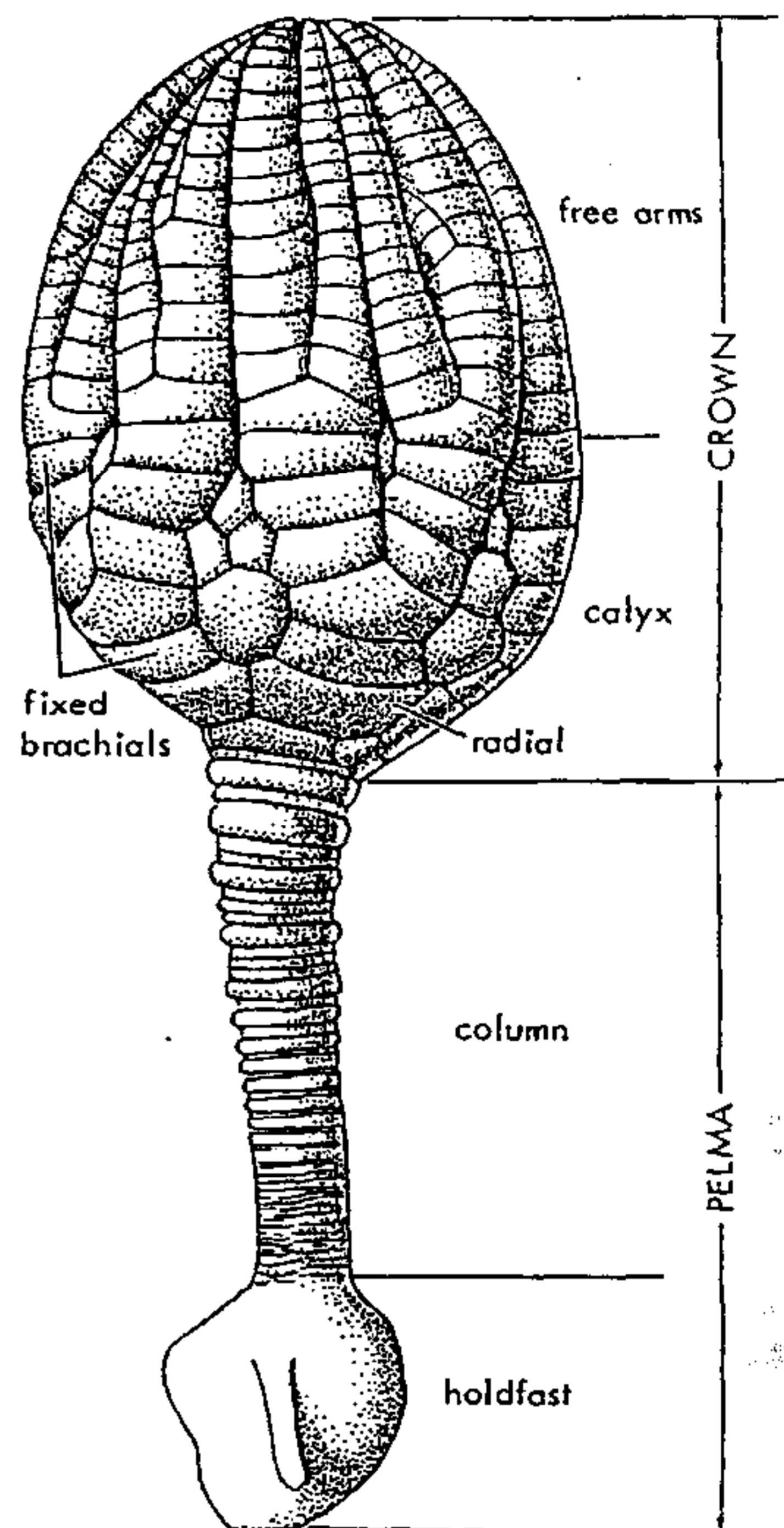
FIG. 41. Calpiocrinus intermedius SPRINGER, M. Sil., Eng., complete specimen of flexible crinoid, \times 3 (Springer, 1920).
