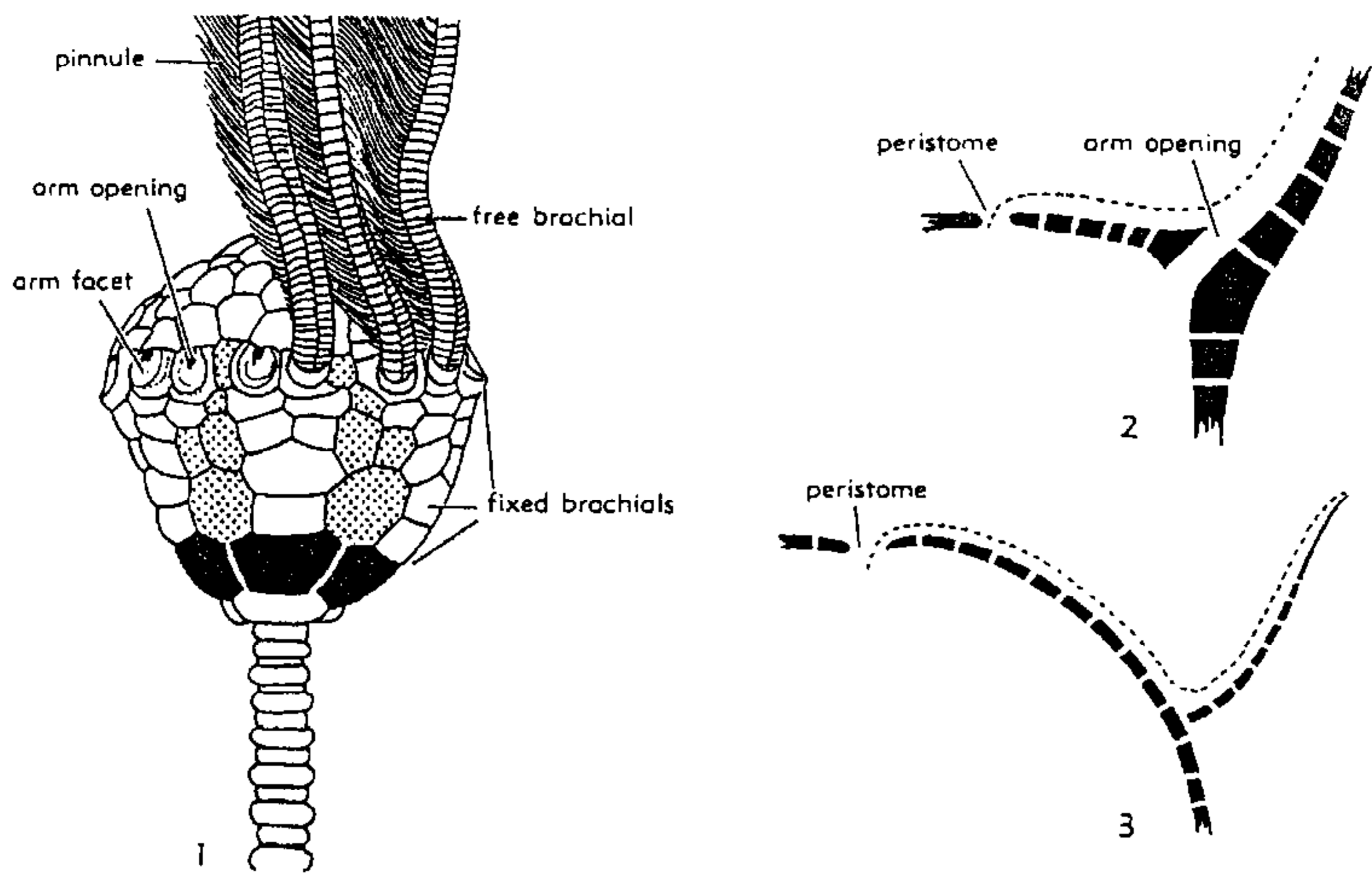
FIG. 105. Relationship of free arms with theca.—1. Uperocrinus longirostris (HALL), Miss., USA; theca with parts of free arms and column, \times 1.3 (Ubaghs, n). [Explanation: radials black; interbrachials stippled.]—2,3. Diagrammatic vertical sections of parts of theca and arm or armlike appendage in a crinoid (2) and a noncrinoid pelmatozoan echinoderm (3) (mod. from Jaekel, 1898a).
