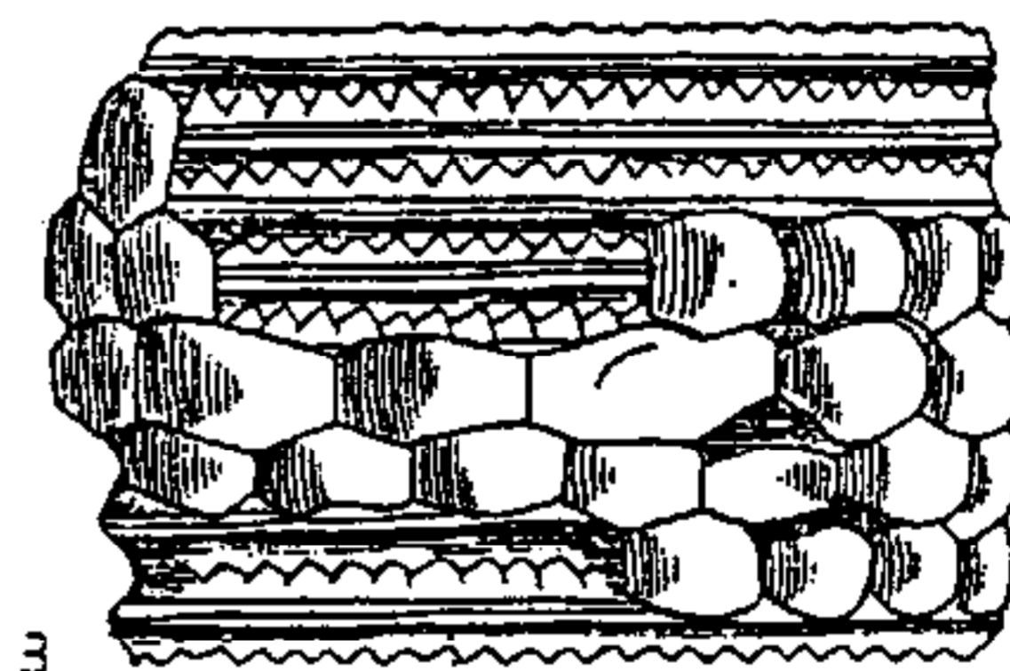
FIG. 63. Pseudocirri and structures of uncertain nature carried on latera of columnals.—1. Hyperexochus immodiscus MOORE & JEFFORDS, L.Dev., USA (Tenn.), facetal view of columnal provided with pseudocirri, \times 2.8 (Moore & Jeffords, 1968).—2. Polypeltes granulatus ANGELIN, U.Sil., Gotl., lateral view of pluricolumnal showing pimplelike ossicles and concave nonperforated scars, \times 6.6 (Ubaghs, 1956).—3. Musivocrinus sp. TERMIER & TERMIER, Perm., Tunisia, lateral view of pluricolumnal with partially preserved covering of small platelike ossicles (Termier & Termier, 1949).
