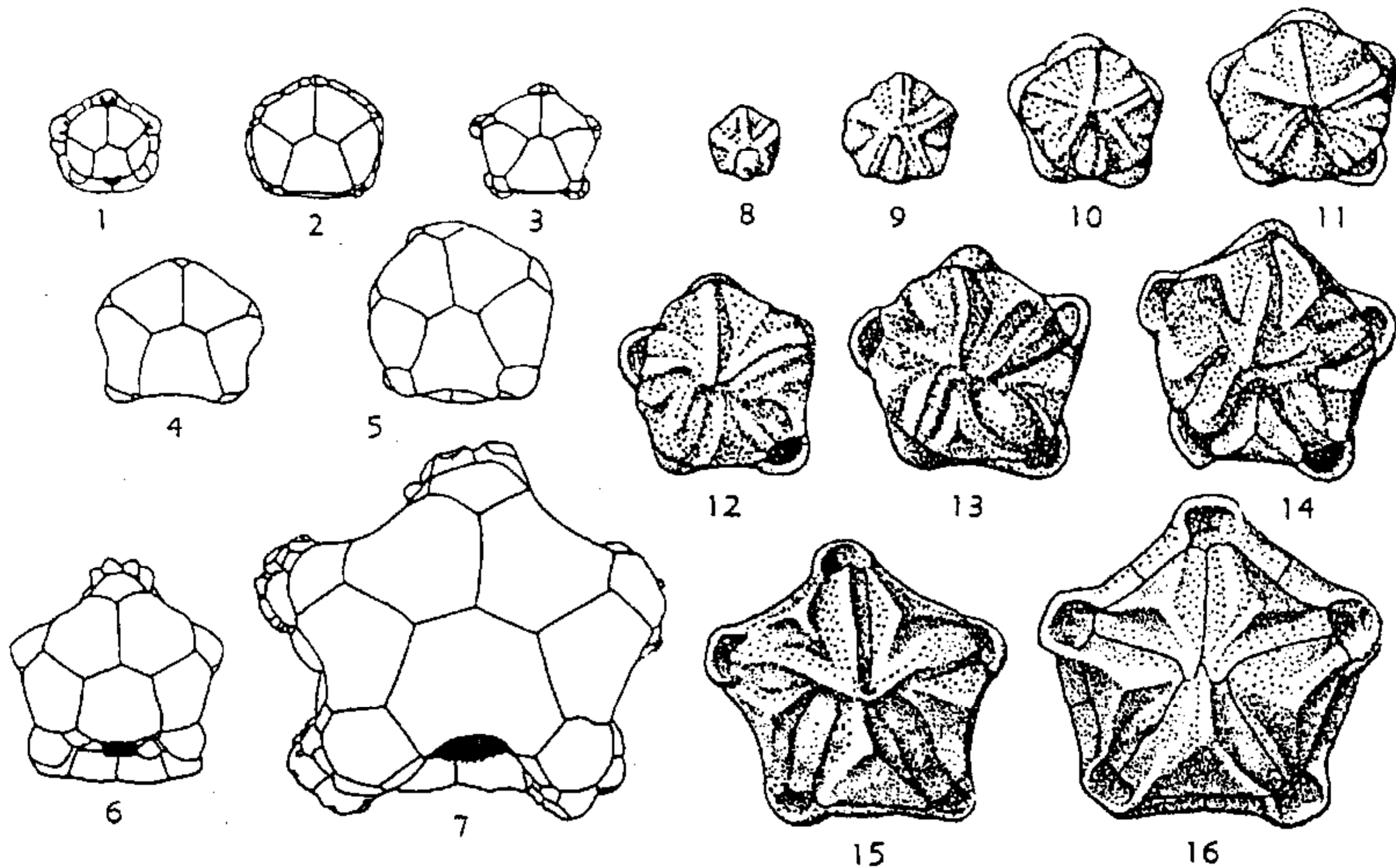
FIG. 150. Growth series of oral plates in a platycrinid (1-7) and a hapalocrinid camerate (8-16).—1-7. Neoplatycrinus dilatatus WANNER, Perm., Timor; \times 1 (Wanner, 1937).—8-16. Cyttarocrinus eriensis (HALL), M.Dev., USA (N.Y.); \times 15 (Koenig, 1965).
