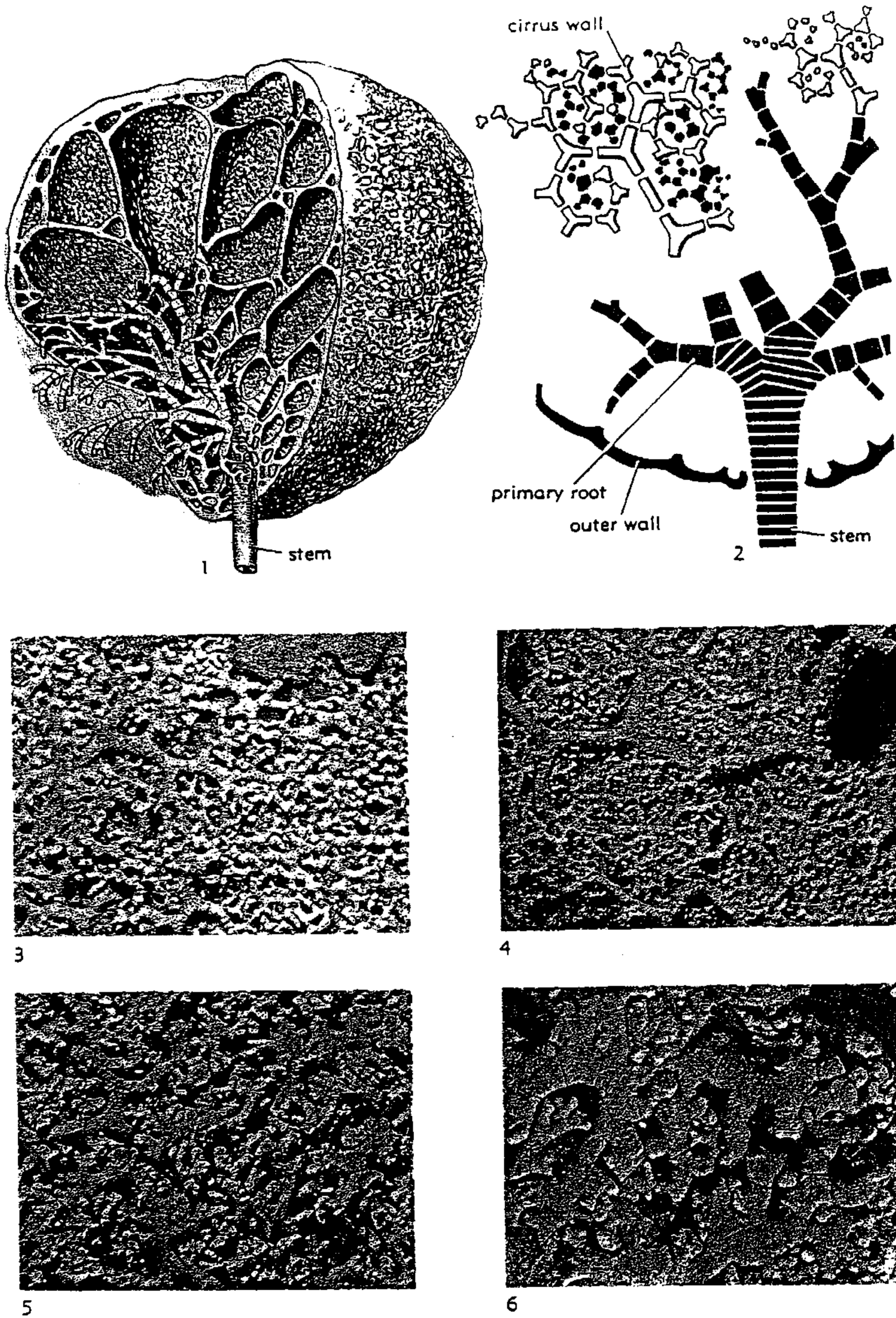
FIG. 67. Morphology of the cirrus type of the bulbous holdfast called Camarocrinus (all from Haude, 1972, modified in 1 and 2).
