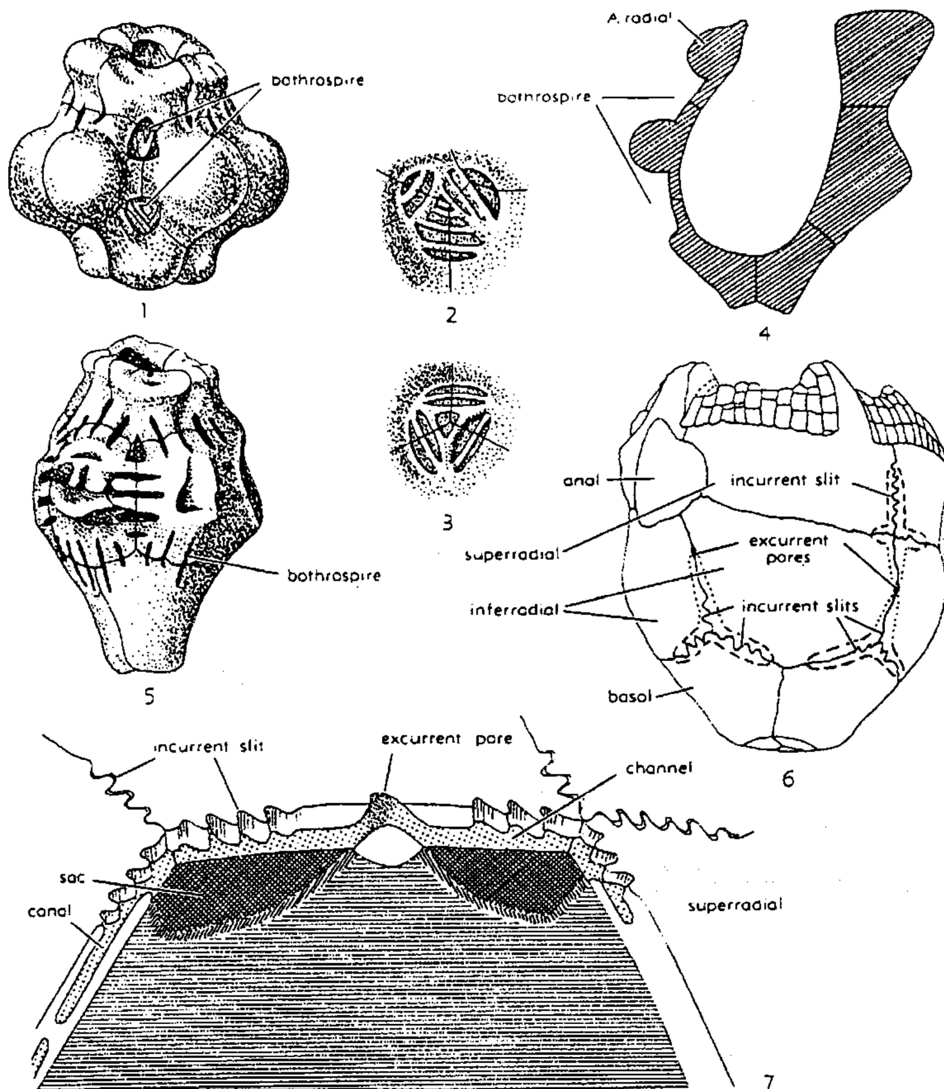
FIG. 183. Morphology of some endospire structures.
