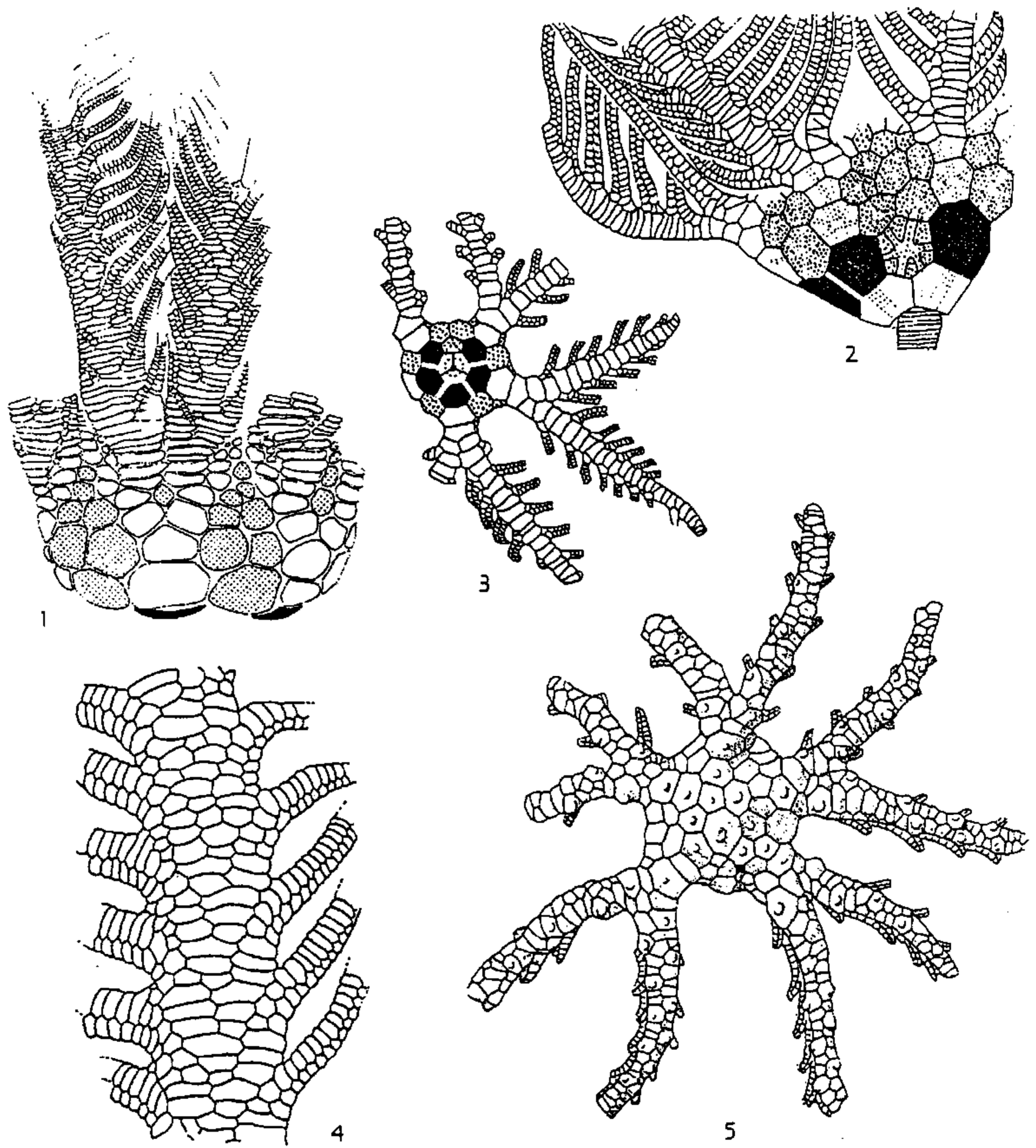
FIG. 116. Arm trunks in camerates.—1. Rhipidocrinus sp. cf. R. perloricatus W. E. SCHMIDT, M.Dev., Ger.; calyx and arm trunks of E ray, ca. \times 1 (Breimer, 1960).—2. Cyidocrinus sculptus (HALL), Miss., N.Am.; calyx and proximal portions of arm trunks, in CD-interray view, \times 1 (Kirk, 1943a).—3. Steganocrinus pentagonus (HALL), Miss., N.Am.; calyx and parts of arm trunks, aboral view, \times 1 (Kirk, 1943a).—4. Trybliocrinus flatheanus GEINITZ, L.Dev., Spain; part of an arm trunk, \times 3.3 (Breimer, 1962).—5. Eucladocrinus millebrachiatus immaturus WACHSMUTH & SPRINGER, Miss., USA(Ia.); adoral side of theca and arm trunks, \times 1 (Wachsmuth & Springer, 1897). [Explanation: interbrachials and anals stippled; radials black.]
