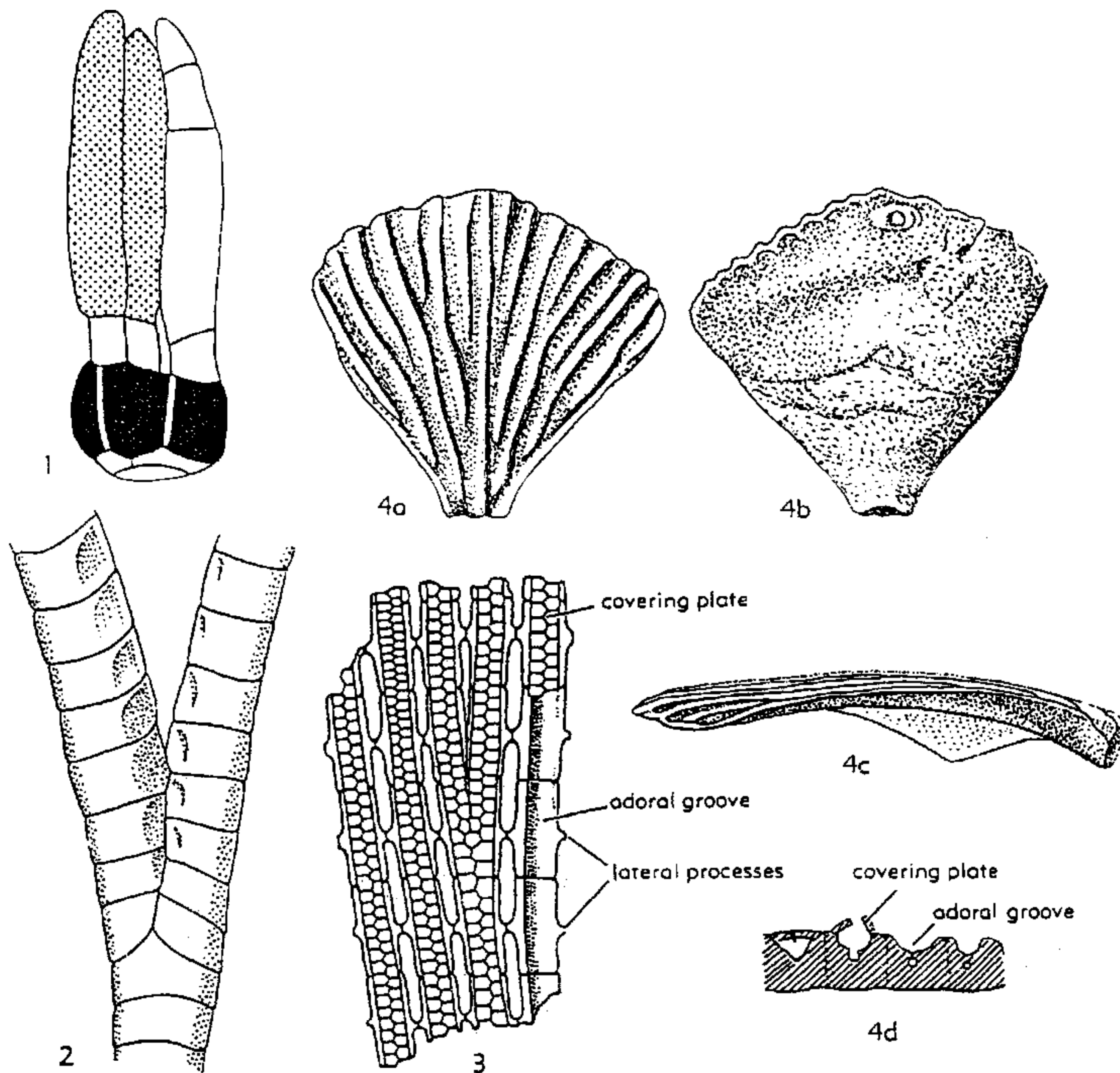
FIG. 124. Fusion of brachials.
