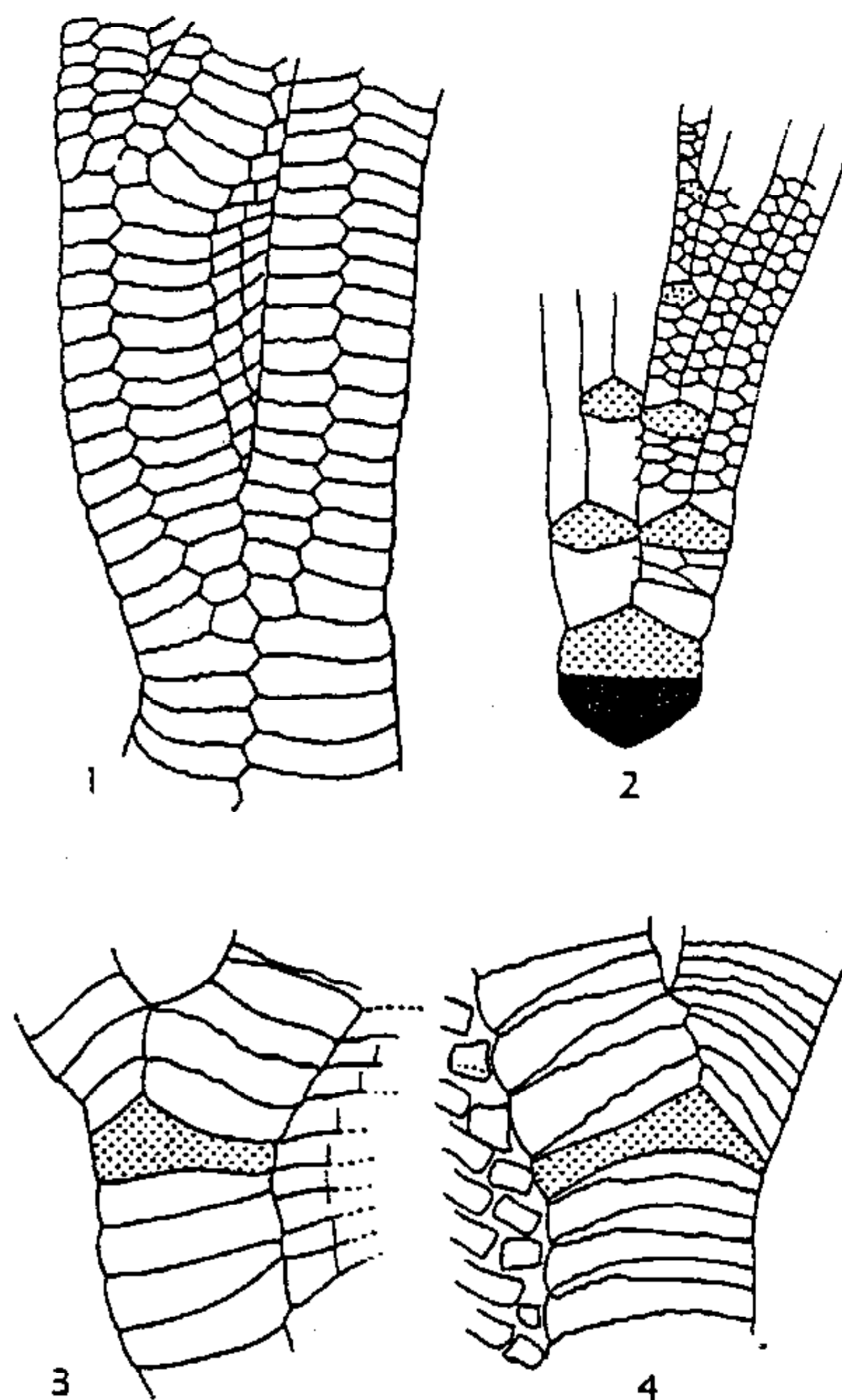
FIG. 120. Bifurcation of arms in camerates (1, 3, 4) and inadunates (2) (axillaries stippled; radial black).—1. Abacocrinus sp., U.Sil., Gotl.; no distinct axillaries, \times 5 (Ubaghs, n).—2. Hydreionocrinus goniodactylus (DE KONINCK & WOOD), U.Carb., Eng.; conspicuous axillaries present, \times 1 (Bather, 1911-12).—3,4. Scyphocrinites sp., U.Sil., Alg.; pinnule-bearing axillaries, \times 7 (Ubaghs, n).
