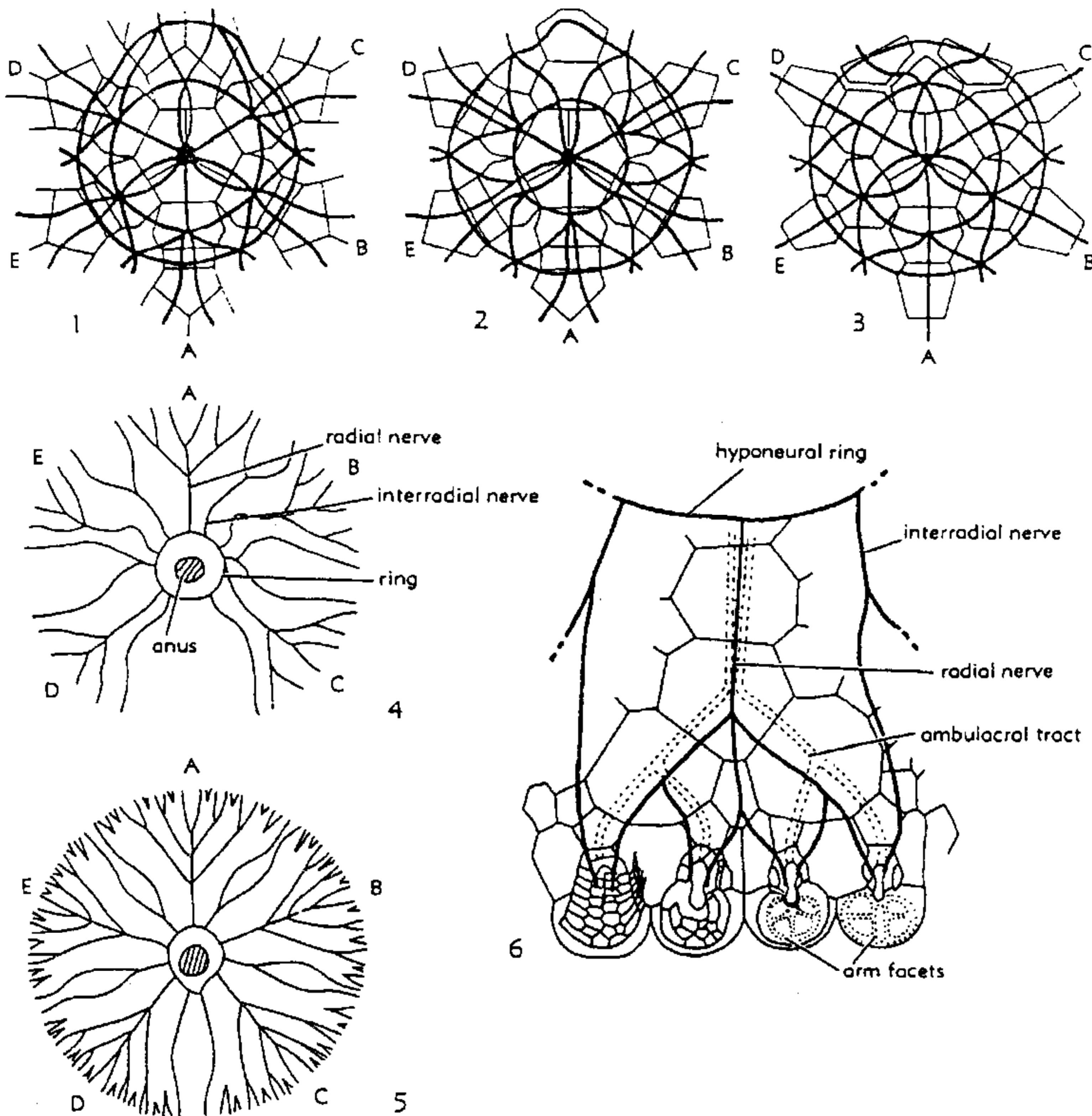
FIG. 164. Diagrammatic plan of the entoneural (1-3) and hyponeural (4-6) systems in some camerate crinoids (all figures from Haugh, 1975b, slightly mod.). [Explanation: A, B, C, D, E, letters designate rays according to CARPENTER.]—1. Batocrinus icosidactylus CASSEDAY, Miss., USA.—2. Dorycrinus quinquelobus (HALL), Miss., USA.—3. Steganocrinus pentagonus (HALL), Miss., USA.—5. Teleocrinus rudis (HALL), Miss., USA.—6. View from exterior of a part of a tegmen as if it were transparent in order to show the course of the hyponeural nerves in a single ray and adjacent interrays. (From Paleobiology , v. 1, no. 3, Summer, 1975, courtesy of The Paleontological Society and Bruce N. Haugh.)
