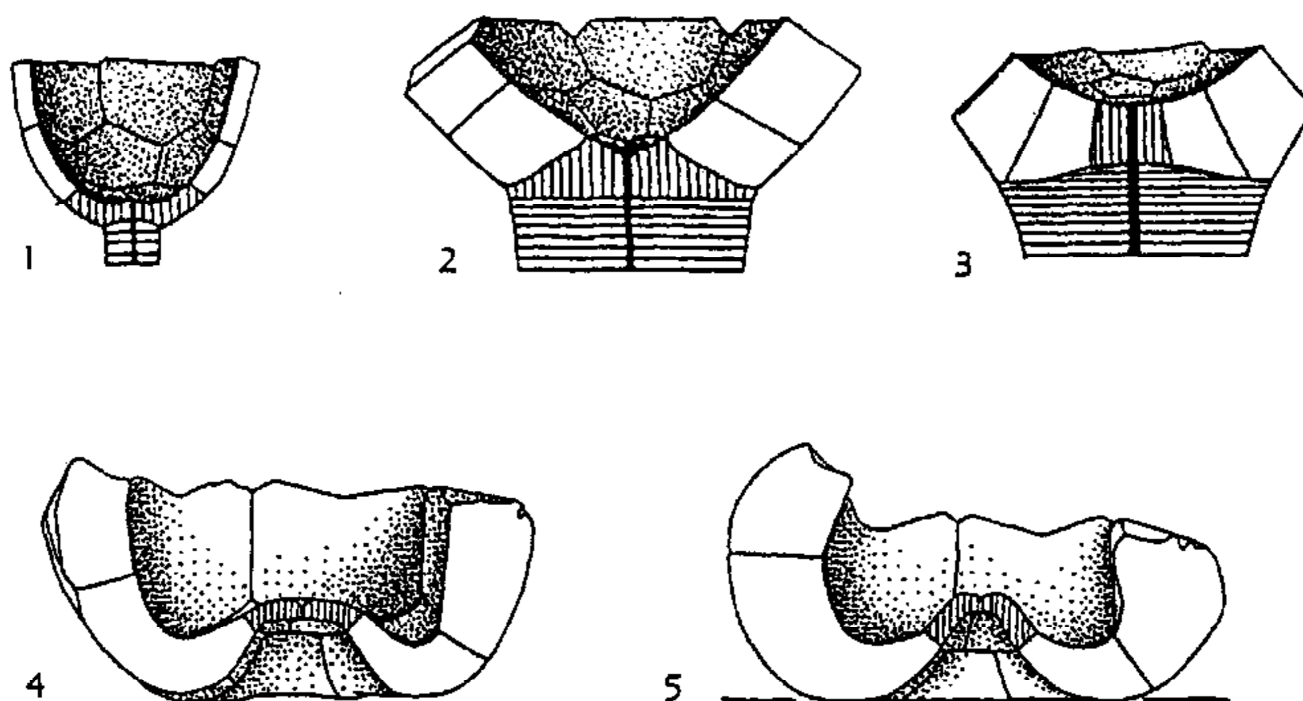
FIG. 74. Diagrammatic vertical sections of cups (1,4,5) and patinas of calyces (2,3) illustrating various conditions of infrabasals. [Explanation: infrabasals ruled vertically.]
