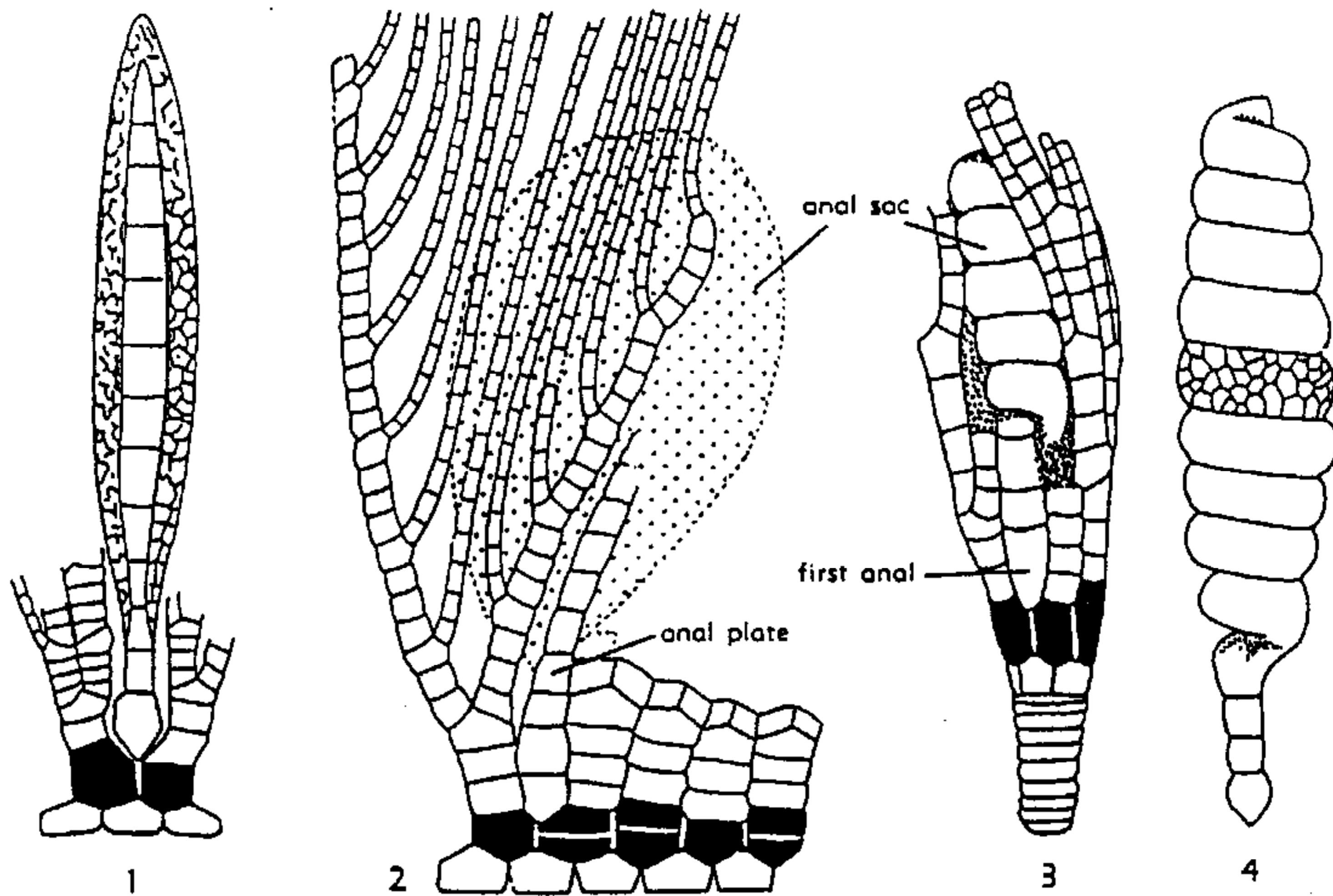
FIG. 156. Morphology of anal tube or sac in disparid inadunates. [Explanation: radials and biradials black.]—1. Dystactocrinus constrictus (HALL), U.Ord., USA (Ohio); diagram of part of crown and anal sac (adapted from Ulrich, 1925).—2. Daedalocrinus kirki ULRICH, Ord., Can. (Ont.); diagram of part of crown and anal sac (Ulrich, 1925).—3. Ohioocrinus brauni ULRICH, U.Ord., USA (Ind.); CD-interray view of crown, \times 4.5 (redrawn from Ulrich, 1925).—4. Ohioocrinus laxus (HALL), U.Ord., USA (Ohio); anal series and spiral anal sac, enl. (Ulrich, 1925).
