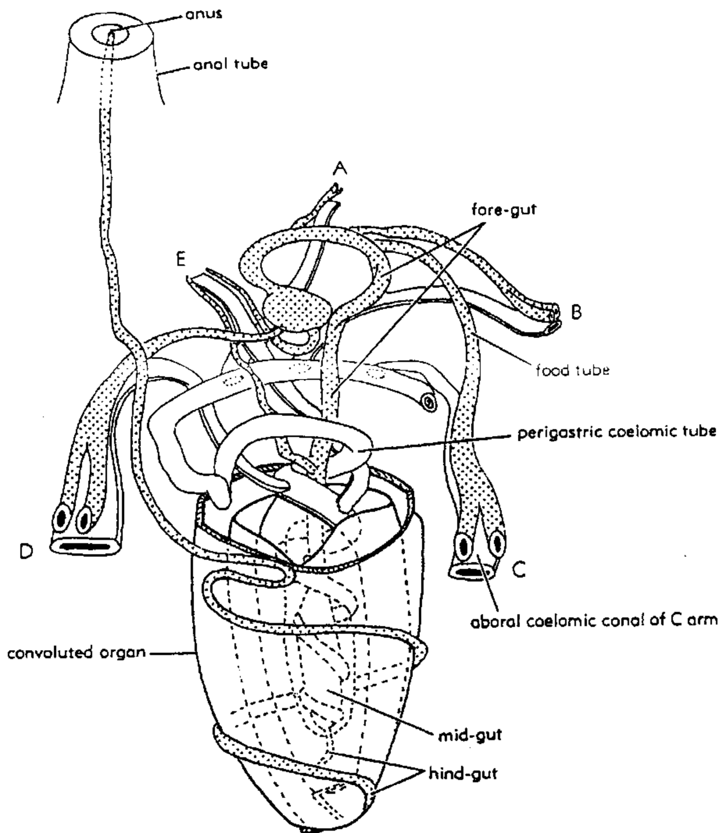
FIG. 169. Diagrammatic reconstruction of the digestive system and part of the coelomic system of camerate crinoids. [Explanation: food tubes and digestive tube stippled. Rays identified by symbol letters of CARPENTER system] (mod. from Haugh, 1975a). (From Journal of Paleontology , v. 49, no. 3, May, 1975, courtesy of The Paleontological Society and Bruce N. Haugh.)
