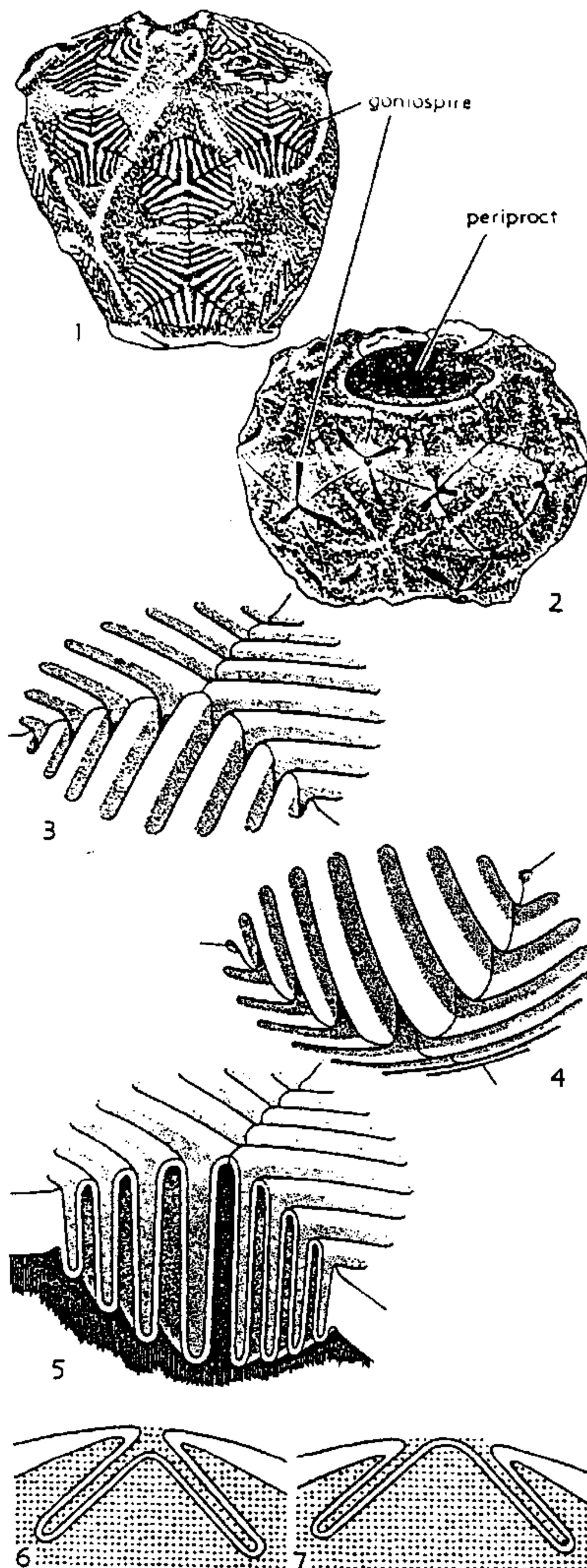
FIG. 180. Morphology of goniospires.—1. Porocrinus shawi SCHUCHERT, M.Ord., Can.; A-ray view, \times 4 (Kesling & Paul, 1968).—2. Triboloporus cryptoplicatus KESLING & PAUL, M.Ord., USA (Va.); CD-interray view, \times 5 (Kesling & Paul, 1968).—3-5. Diagram. representation of gonio-
