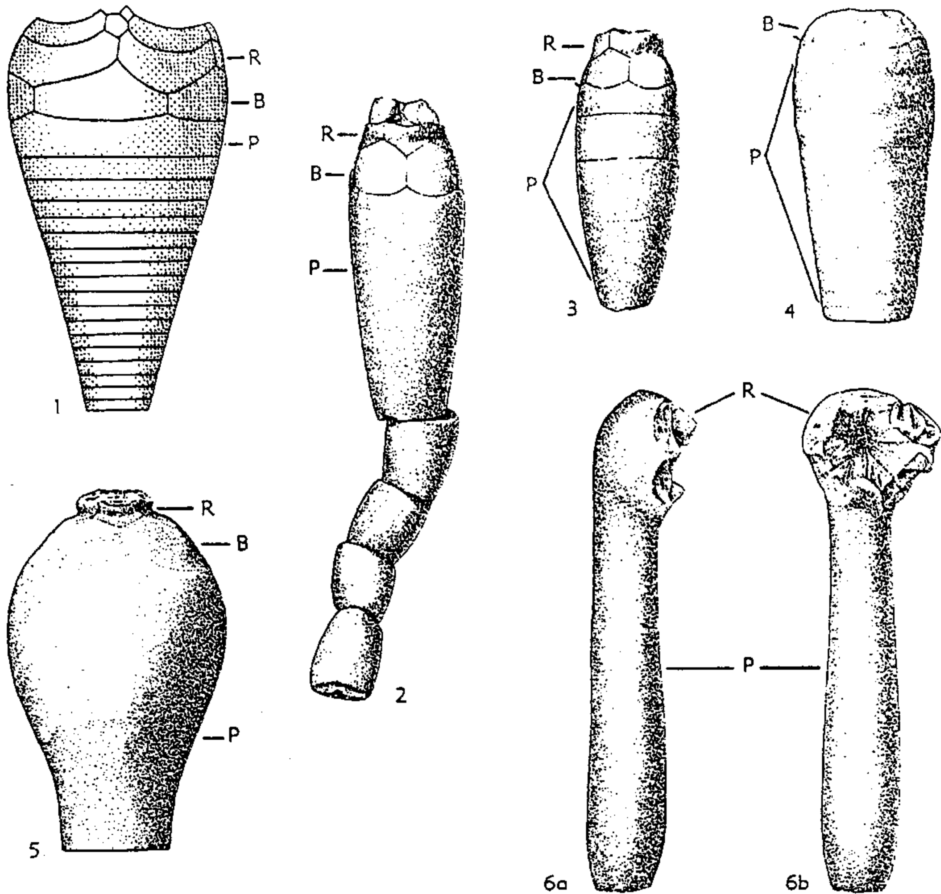
FIG. 51. Morphology of proximale. [Explanation: B , basal; P , proximale; R , radial.] (All Rasmussen, 1961, except 1, from de Loriol, 1882-84.)
