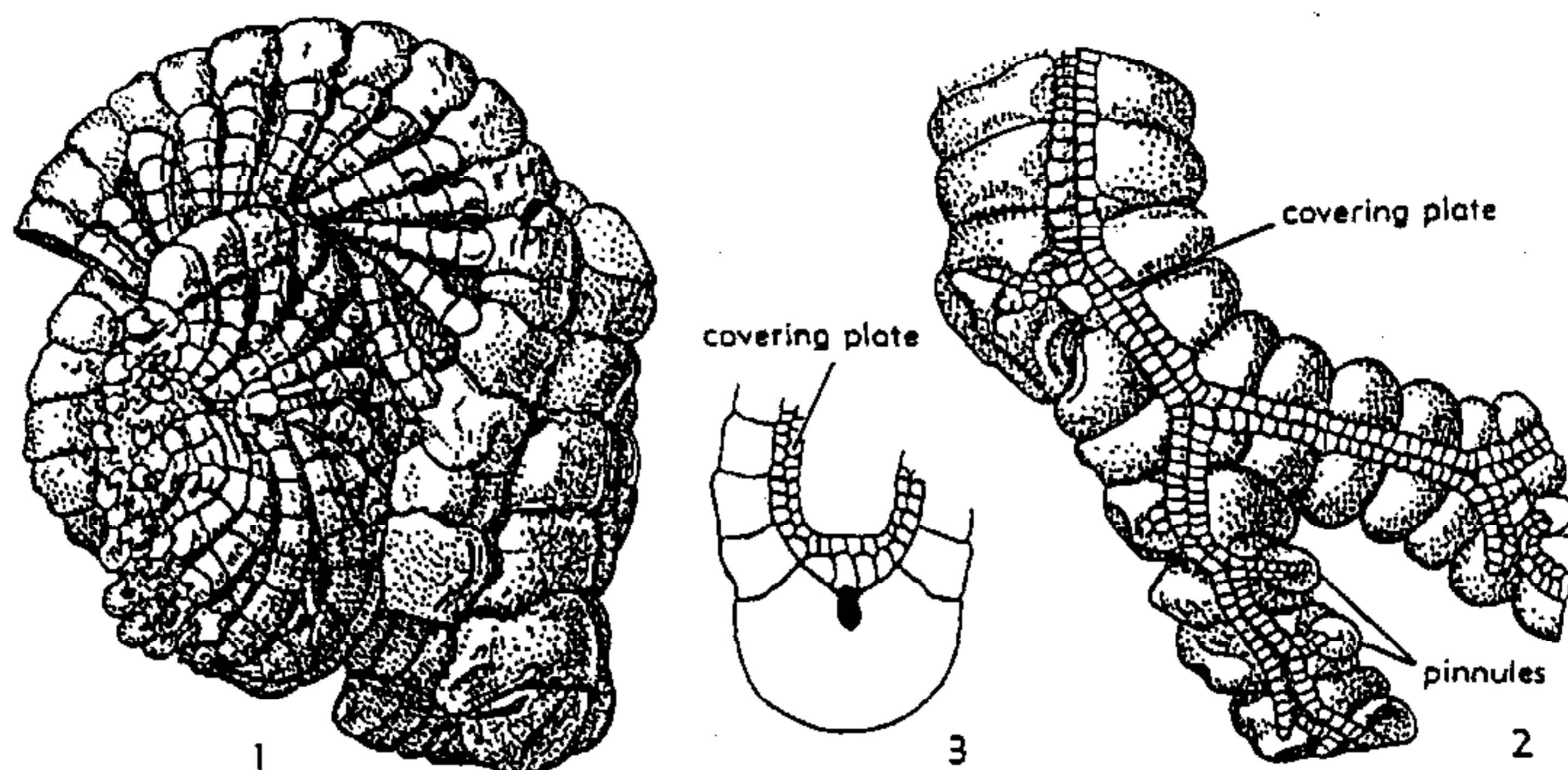
FIG. 132. Cyliocrinus scolopendra (BATHER), U.Sil., Gotl. (redrawn from Bather, 1893a).—1. Lat. view of arm, \times 3 .—2. Adoral aspect of part of arm, in which only the bases of the pinnules are preserved, \times 3 .—3. Transverse section of a brachial with two pinnules, \times 3 .
