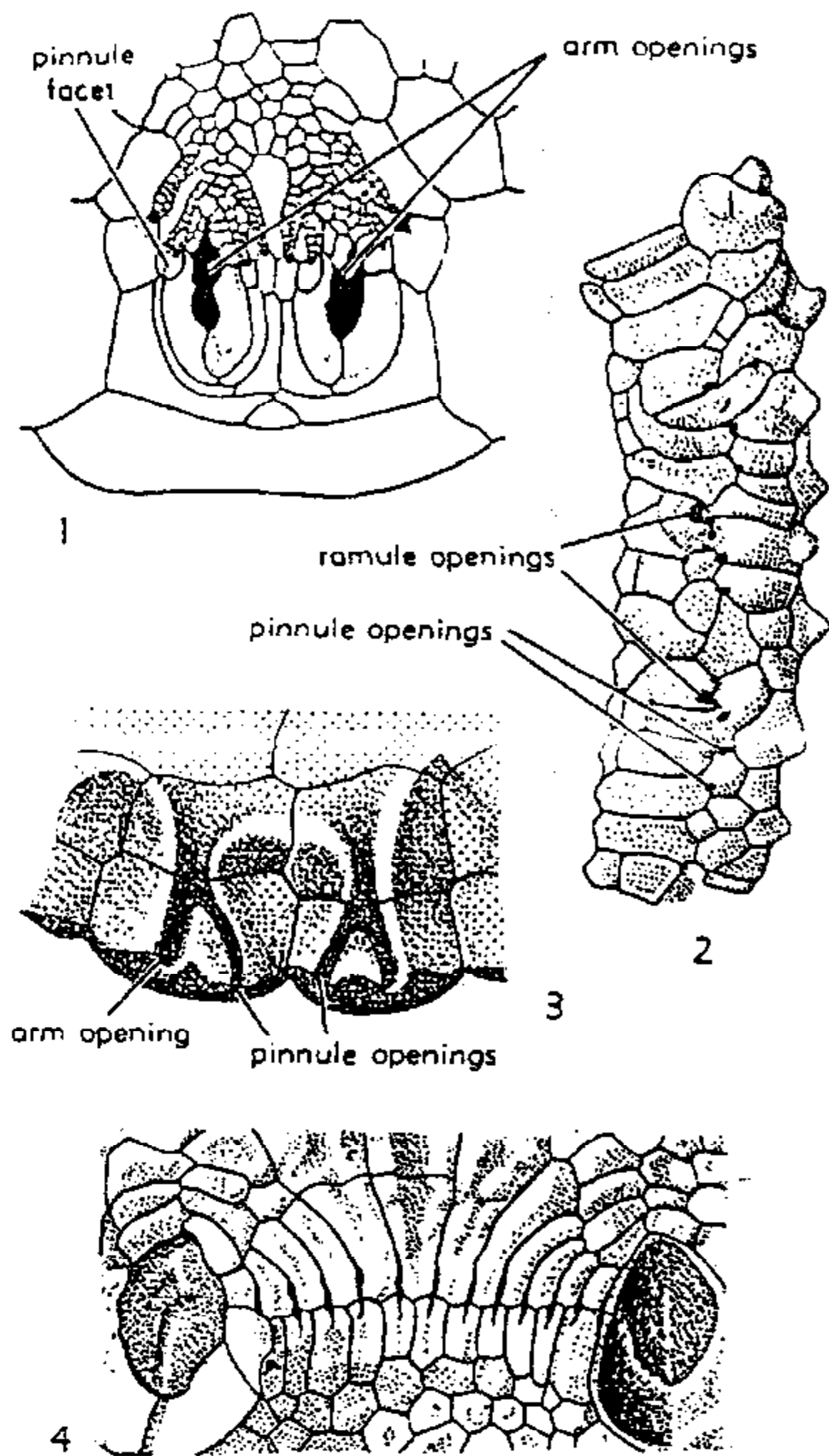
FIG. 184. Pinnule openings in camerates.— 1. Marsupiocrinus inflatus (TROOST), Sil., USA; part of ray showing pinnule openings and ambulacral tracts leading to them, \times 1.5 (Springer, 1917).—2. Eucladocrinus millebrachiatus WACHSMUTH & SPRINGER, Miss., USA (Iowa-Ill.); part of arm trunk, lat. view, \times 1.5 (Wachsmuth & Springer, 1897).—3. Abatocrinus clypeatus (HALL), Miss., USA; transv. sec. of theca at arm-opening level, plates separated at sutures, \times 4 (Springer, 1917).—4. Dolatocrinus grandis MILLER & GURLEY, M.Dev., USA (Ky.); part of interray with 12 slitlike pinnule openings, \times 2 (Springer, 1921a).
