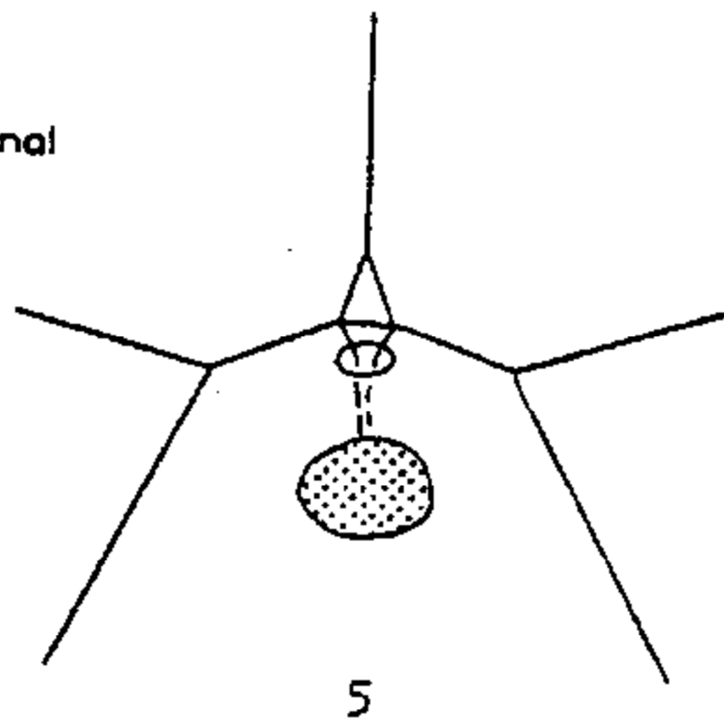
FIG. 166. Structures related to water-vascular system in camerates.
