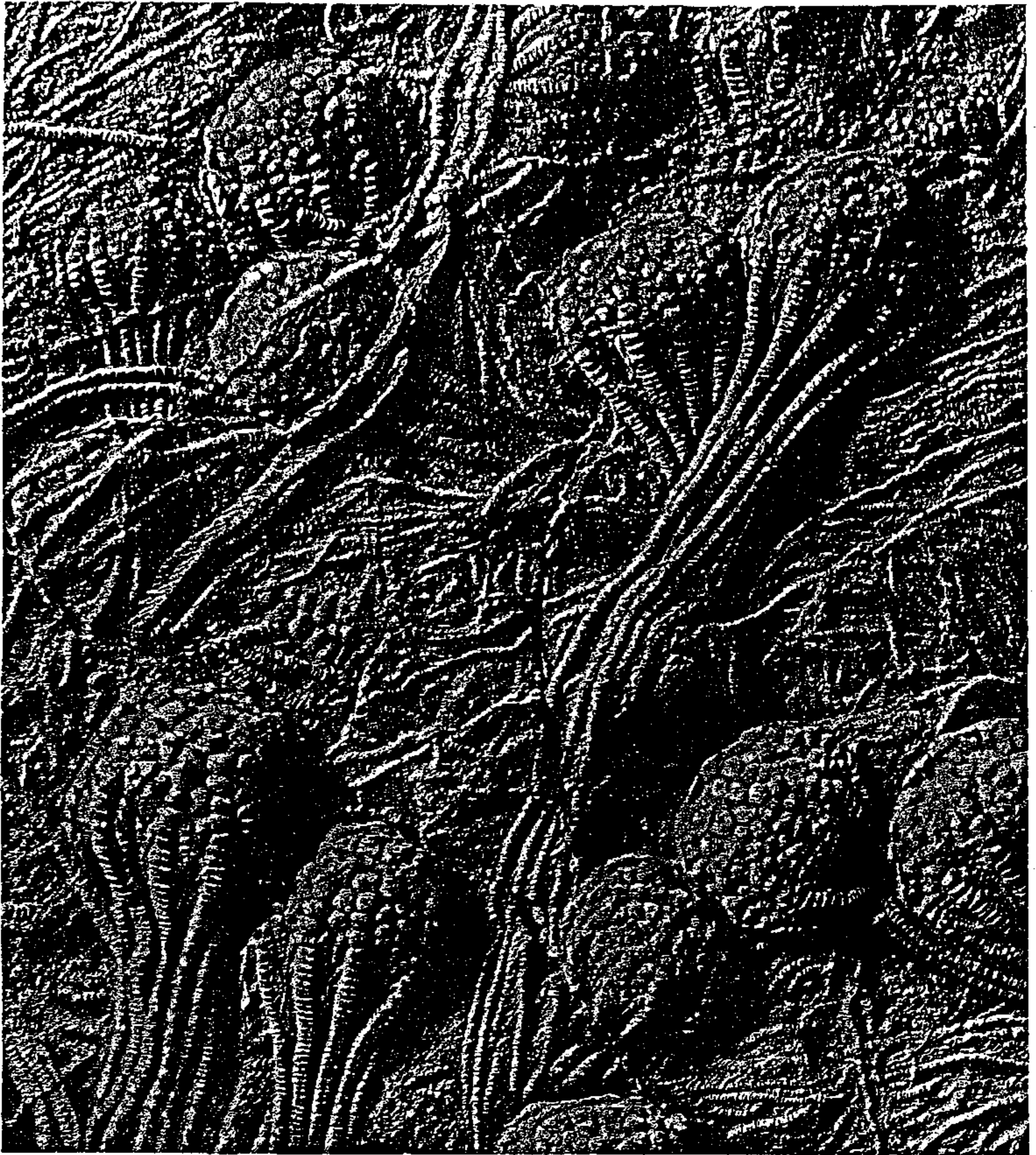
FIG. 216. Specimens of free-swimming crinoid Urintacrinus clustered on a slab of thin limestone found interbedded with chalk of Cretaceous age in western Kansas (about two-fifths natural size) (from Historical Geology , by R. C. Moore, copyright 1933, McGraw-Hill Book Company; used with permission of McGraw-Hill Book Company and University of Kansas Museum of Natural History). [For detailed discussion of this occurrence see STRUVE, 1957.—Eds.]
