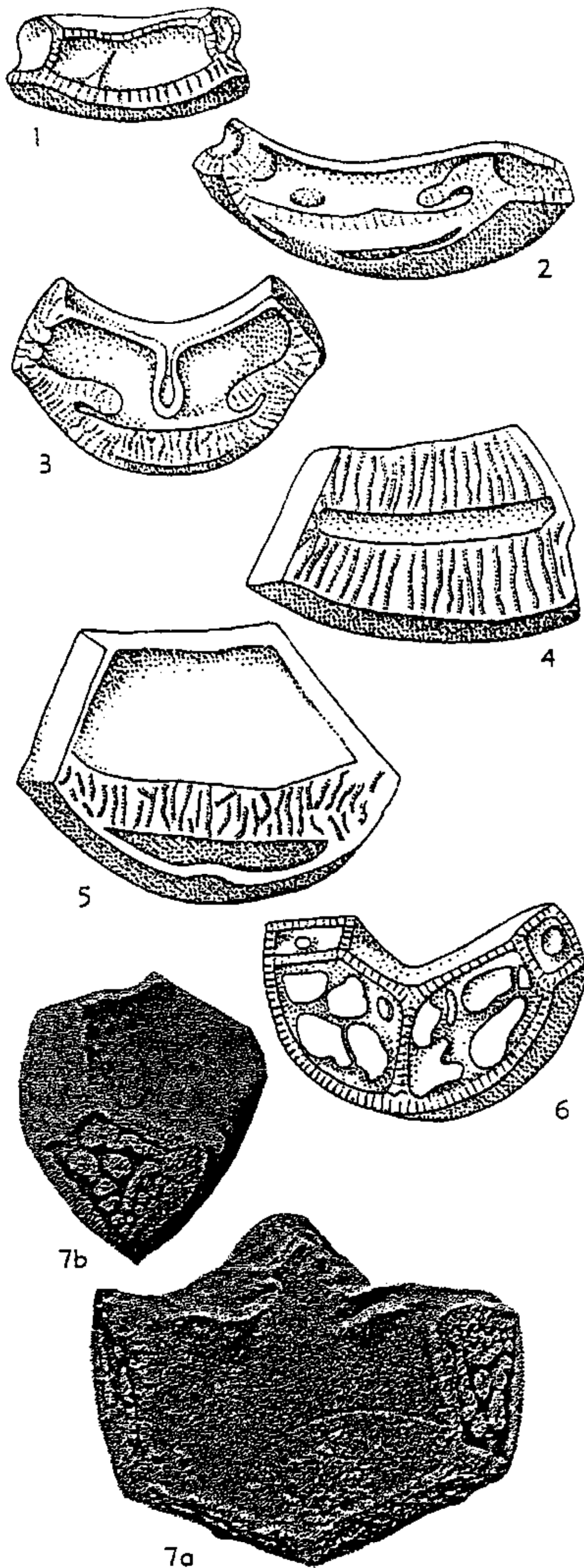
FIG. 102. Articular on selected calycinal plates of flexible (1-6) and inadunate (7) crinoids. [Explanation: aboral (outer) side of each ossicle directed downward.]—1-3. Forbesiocrinus nobilis DE KONINCK & LE HON, L.Carb., Belg.; 1, proximal face of basal; 2, distal face of radial; 3, distal face
