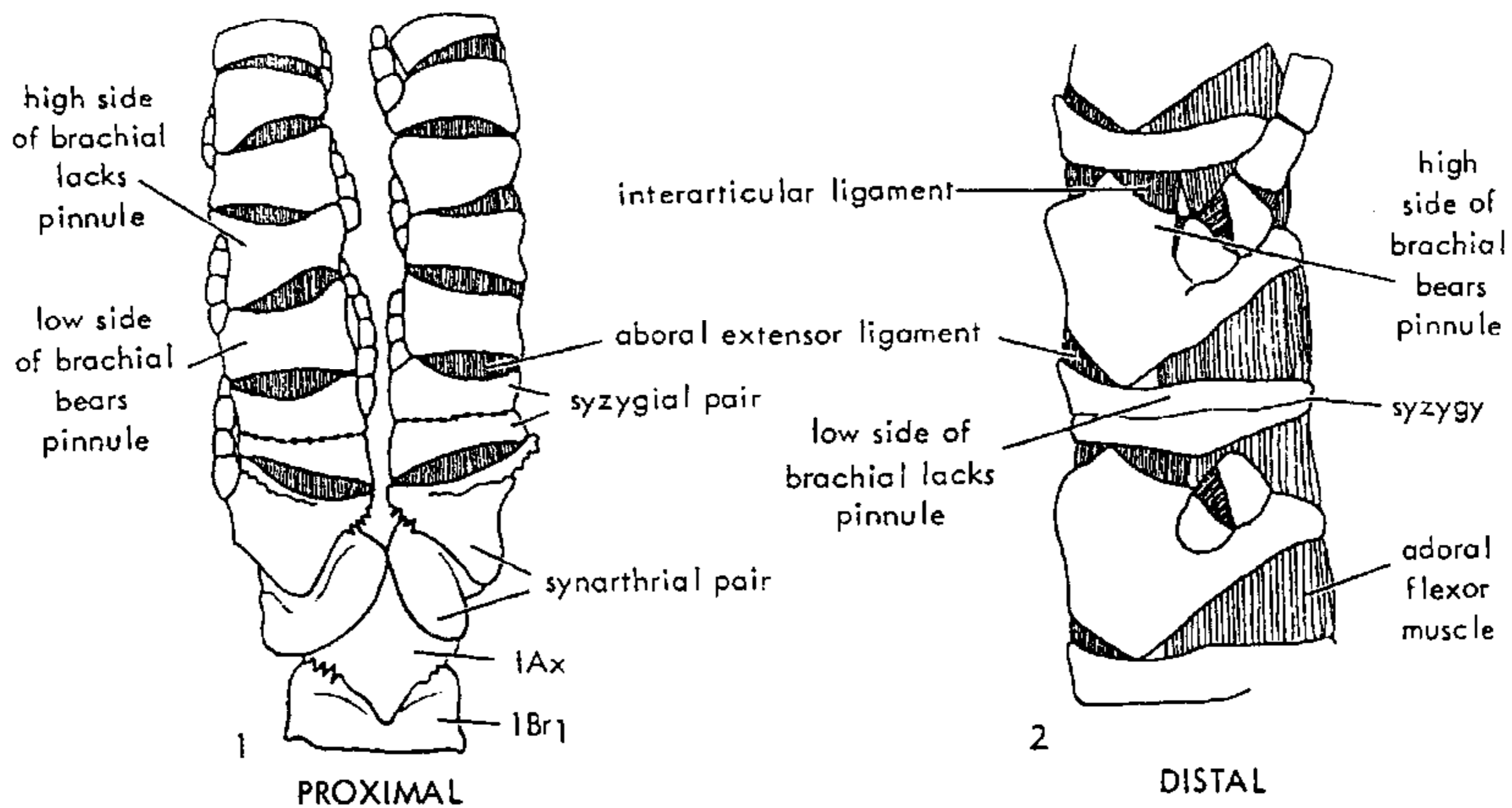
FIG. 22. External obliqueness of brachials and the reversion phenomenon in Florometra serratissima (Breimer, n).
