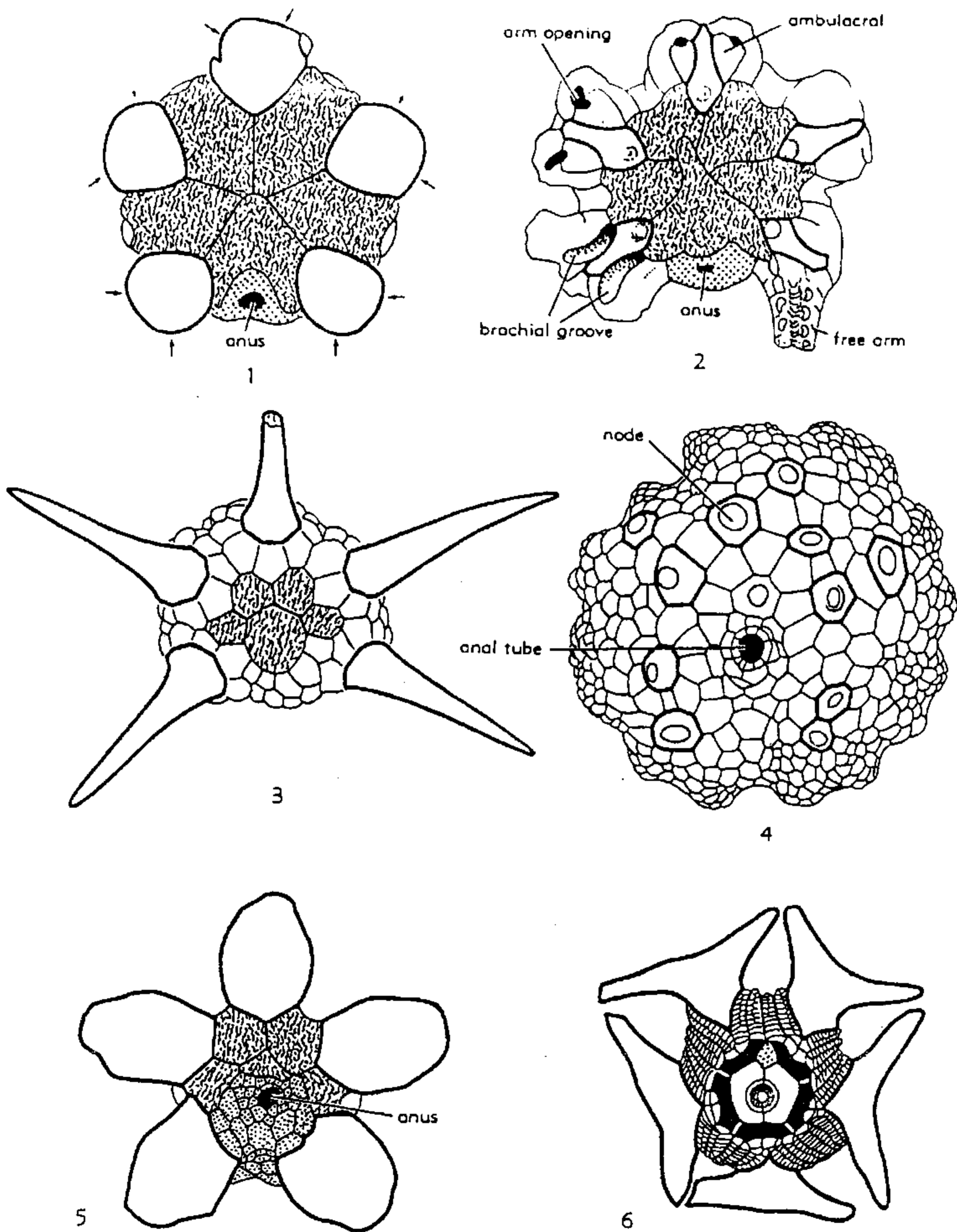
FIG. 154. Axillary ambulacrals and radial dome plates in camerates. [Explanation: radials black; anals stippled; orals shaded; axillary ambulacrals and radial dome plates with heavy outlines.] 1. Oenochoacrinus pileatus BREIMER, M.Dev., Spain; arrows indicate positions of arm facets, X3 (Breimer, 1962). 2. Oenochoacrinus princeps BREIMER, Dev., Spain; X3 (Breimer, 1962). 3. Pterocrinus missouriensis (SPRINGER), Miss., USA (Iowa-Mo.); X1 (redrawn from Wachsmuth & Springer, 1897). 4. Megistocrinus nodosus BARRIS, M.Dev., USA (Iowa-Mich.); X1 (redrawn from Wachsmuth & Springer, 1897). 5. Pterocrinus coronarius (LYON), Miss., USA (Ky.); adoral view, X1 (Springer, 1926b). 6. Pterocrinus bifurcatus WETHERBY, Miss., USA (Ky.); aboral view, X1 (redrawn from Springer, 1926b).
