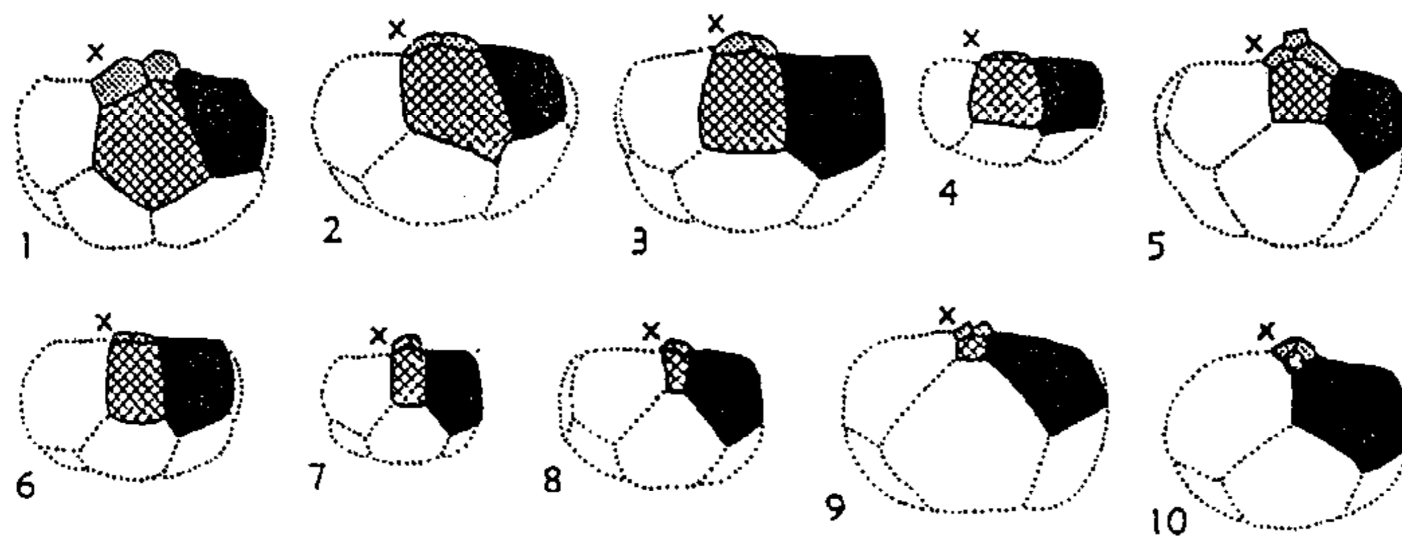
FIG. 96. Variations of the radianal in specimens of Cadocrinus variabilis (WANNER) (Cladida), Perm., Timor; 1-10, selected specimens, post. view, \times 0.87 (Moore, 1962b). [Explanation: C radial black; radianal cross ruled; anal X and other anal plates stippled.]
