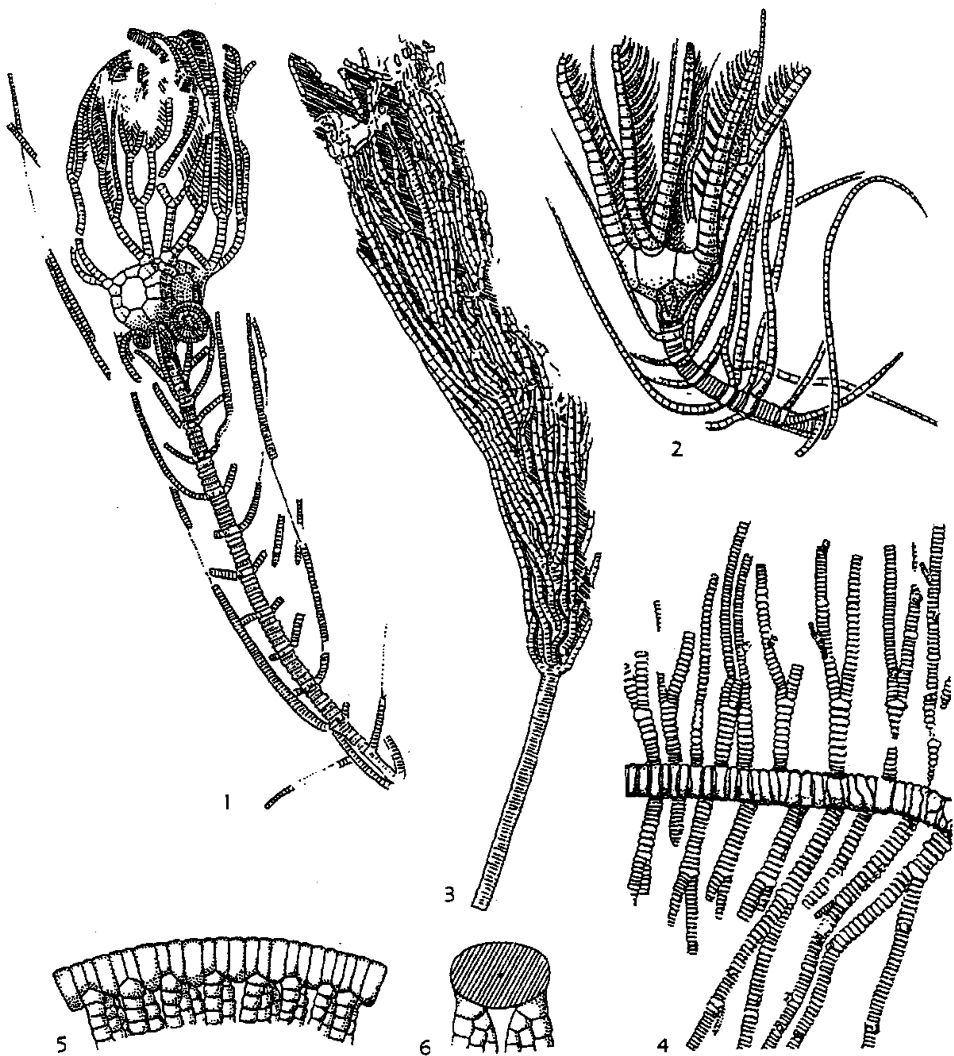
FIG. 62. Morphology of cirri in some Paleozoic crinoids.
