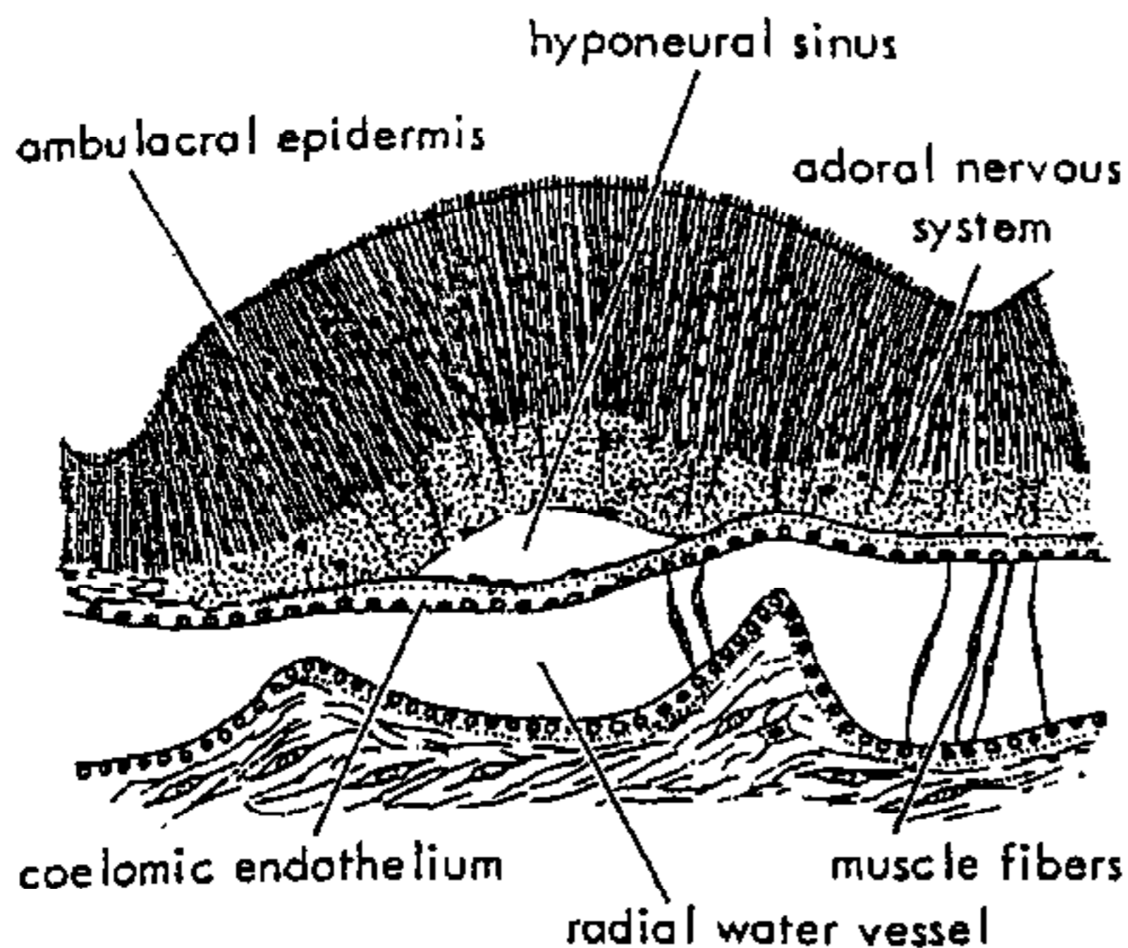
FIG. 6. Transverse section through ambulacrum (after Hamann, 1889).
