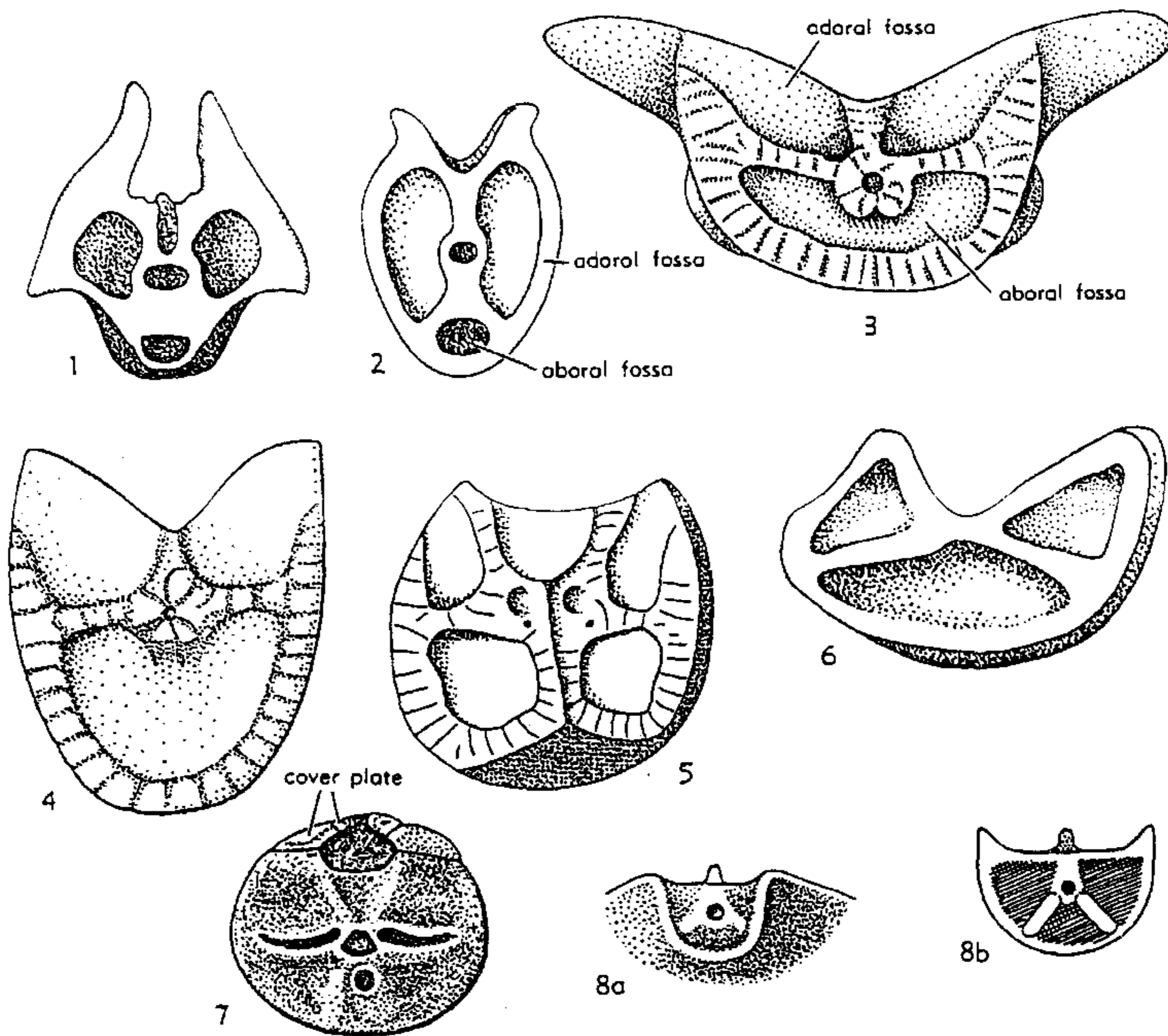
FIG. 139. Trifascial articulations.
