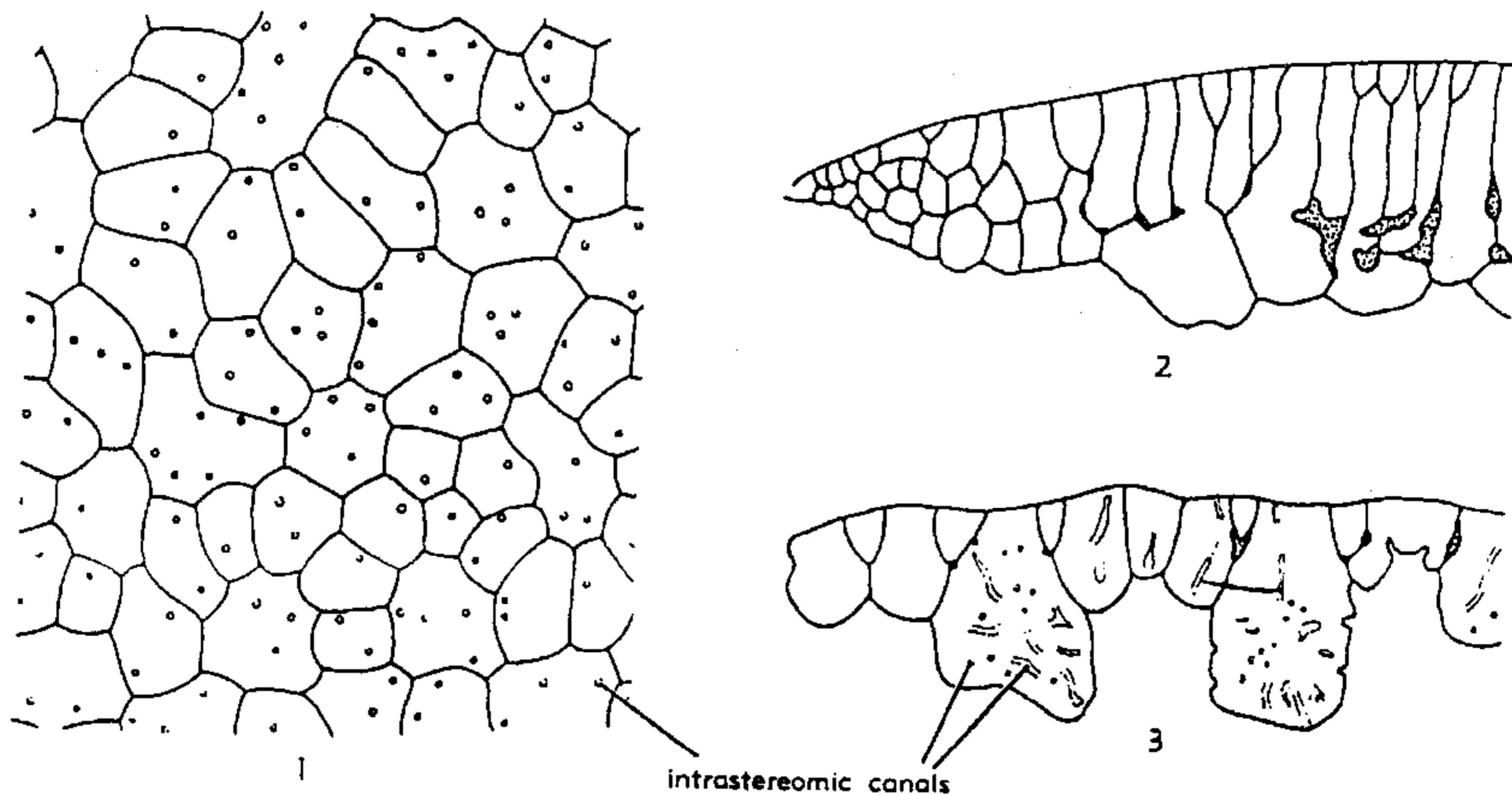
FIG. 179. Trybliocrinus flatheanus (GEINITZ), L.Dev., Spain; morphology of tegmen, ca. \times 3 (Breimer, 1962).—1. External view of slightly weathered surface, showing canal system within plates.—2. Section through tegmen, with stratified margin at left, and lacunae between plates at right (stippled).—3. Section through tegmen, with inner expansions and canal system within plates.
