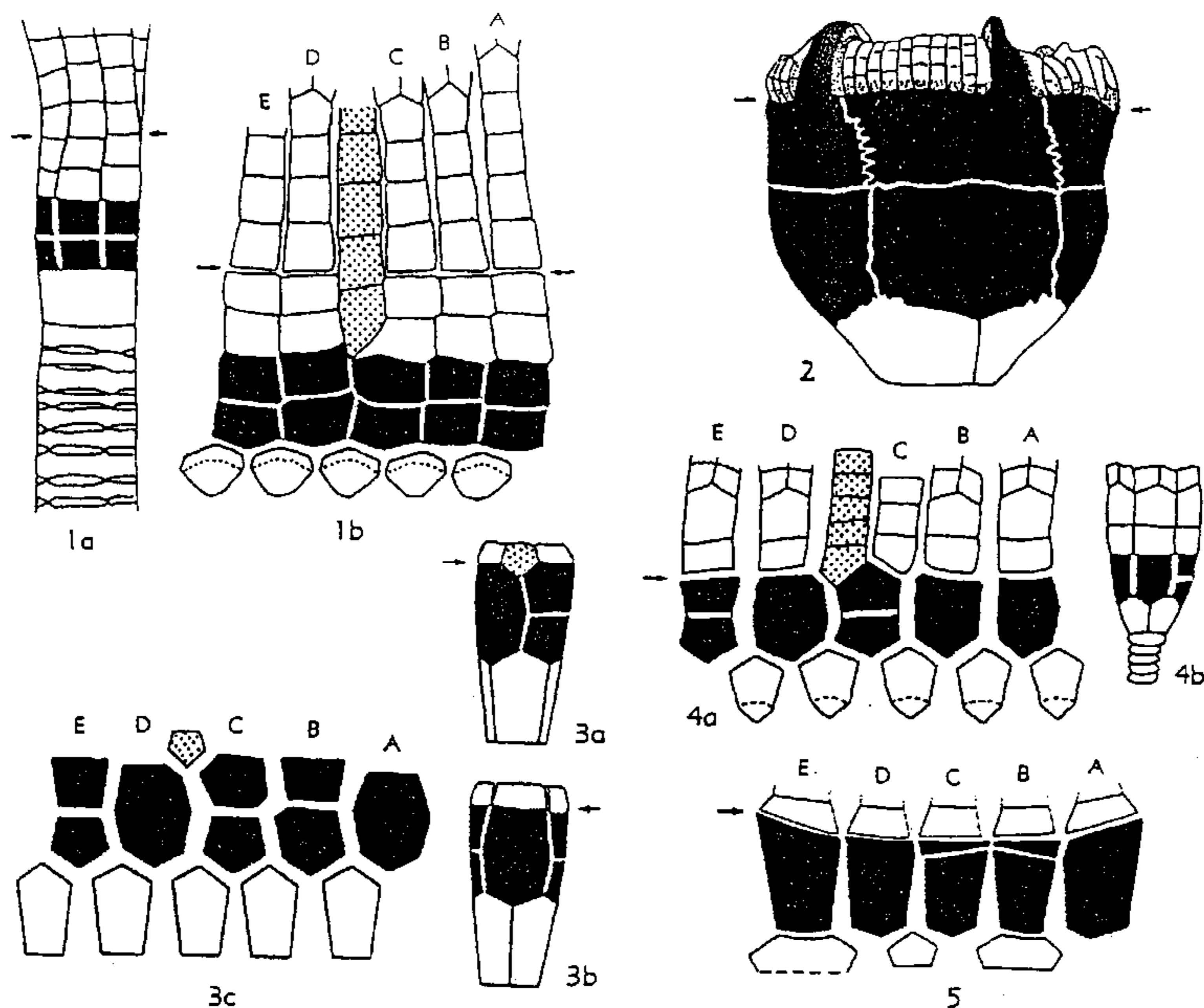
FIG. 88. Selected examples of disparid inadunates with biradials. [Explanation: radials and biradials black; anal plates stippled; top of calyx marked by small arrows; rays identified by letter symbols of CARPENTER system.]
