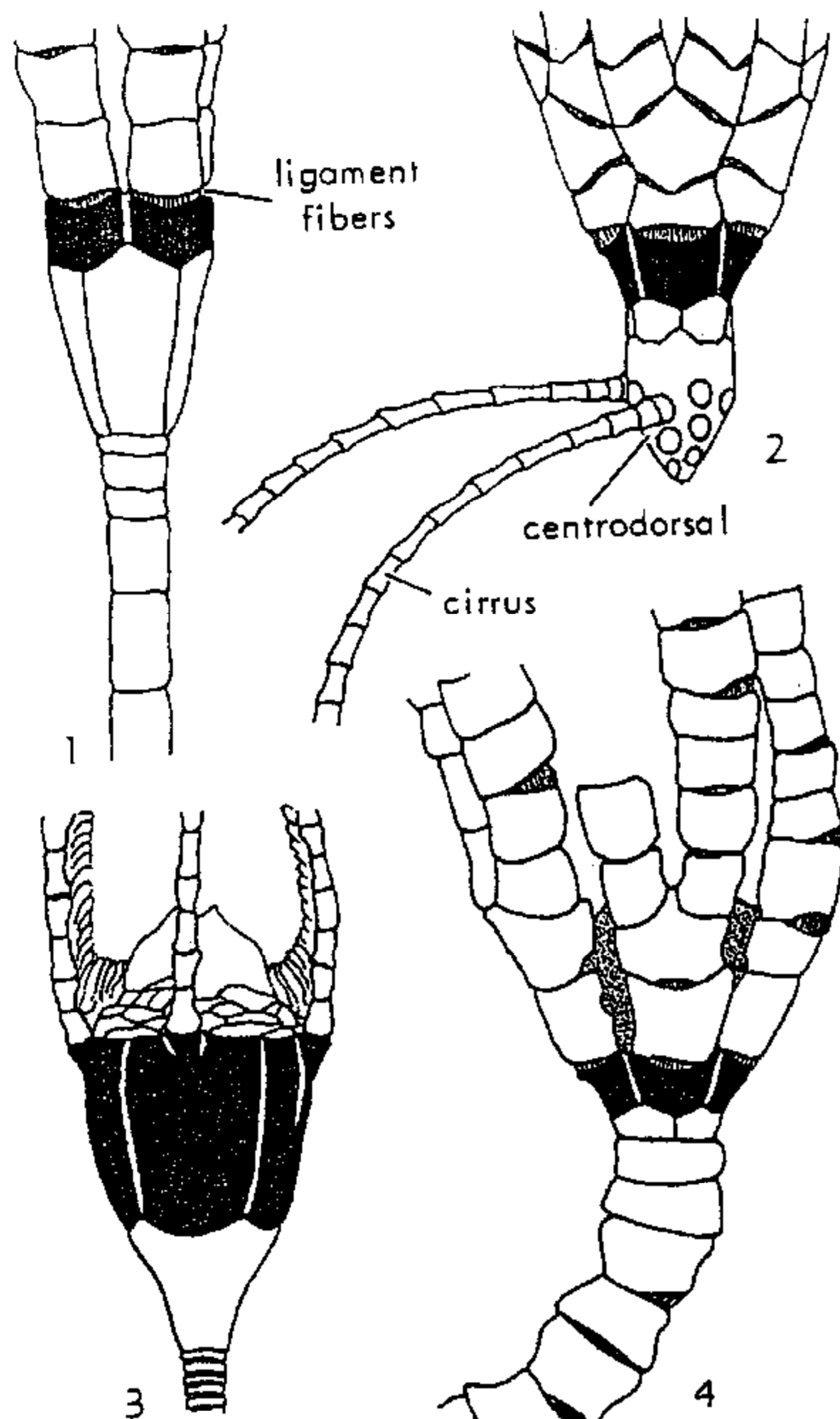
FIG. 13. Radial and basal circlets in various recent crinoids (radials solid black).—1. Democrinus conifer (Breimer, n).—2. Atelecrinus anomalus (after Clark, 1915a).—3. Hyocrinus bethellianus (after Carpenter, 1884a).—4. Presumed Zeuctocrinus from Antarctic (Breimer, n).
