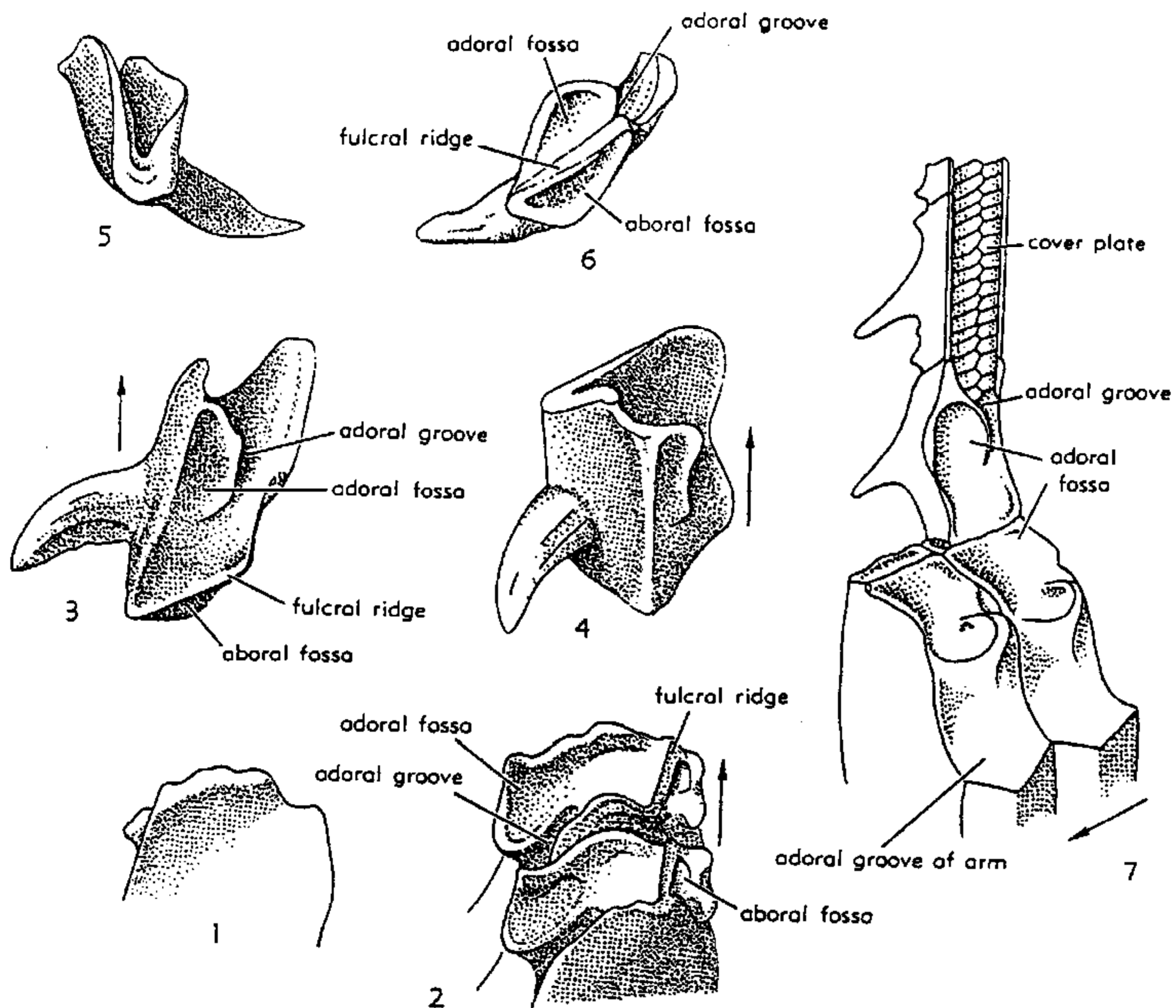
FIG. 136. Pinnule facet and first pinnular of an actinocrinitid camerate, Actinocrinites sp., L. Carb., Belg.; all figures \times 20 (Ubaghs, n). [Explanation: arrows indicate distal direction.]—1-2. Pinnule facet in 1) proximal lateral view, 2) oblique adoral aspect.—3-6. First pinnular seen from 3) adoral face, 4) ext. lat. face, 5) distal face, 6) proximal face.—7. Diagram. reconstr. of adoral aspect of two brachials with proximal part of a pinnule.
