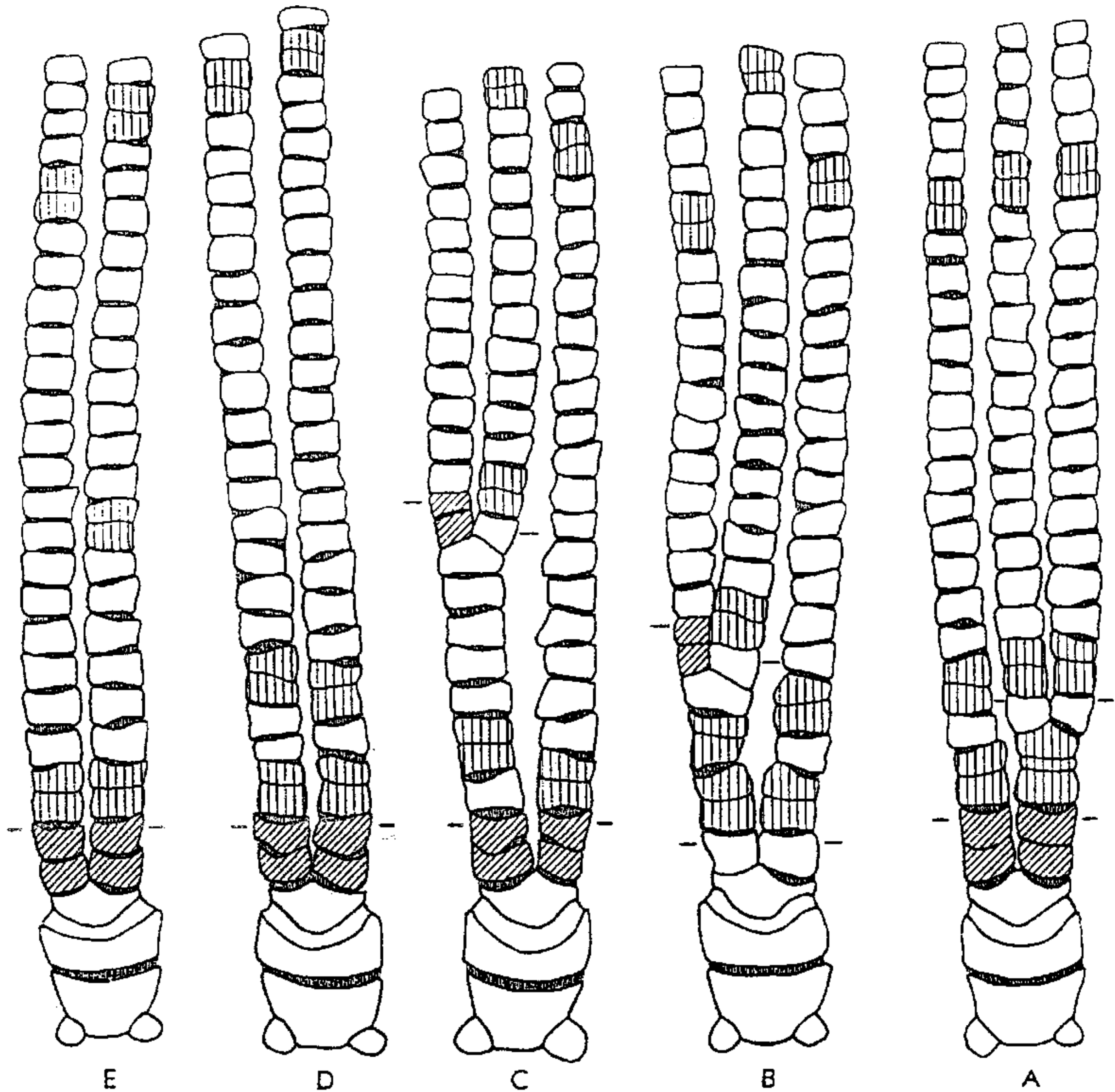
FIG. 27. Semidiagrammatic representation of arm ramification and distribution of synarthrial (oblique ruled) and syzygial (vertical ruled) pairs of brachials in a specimen of Neocrinus decorus (Breimer, n).
