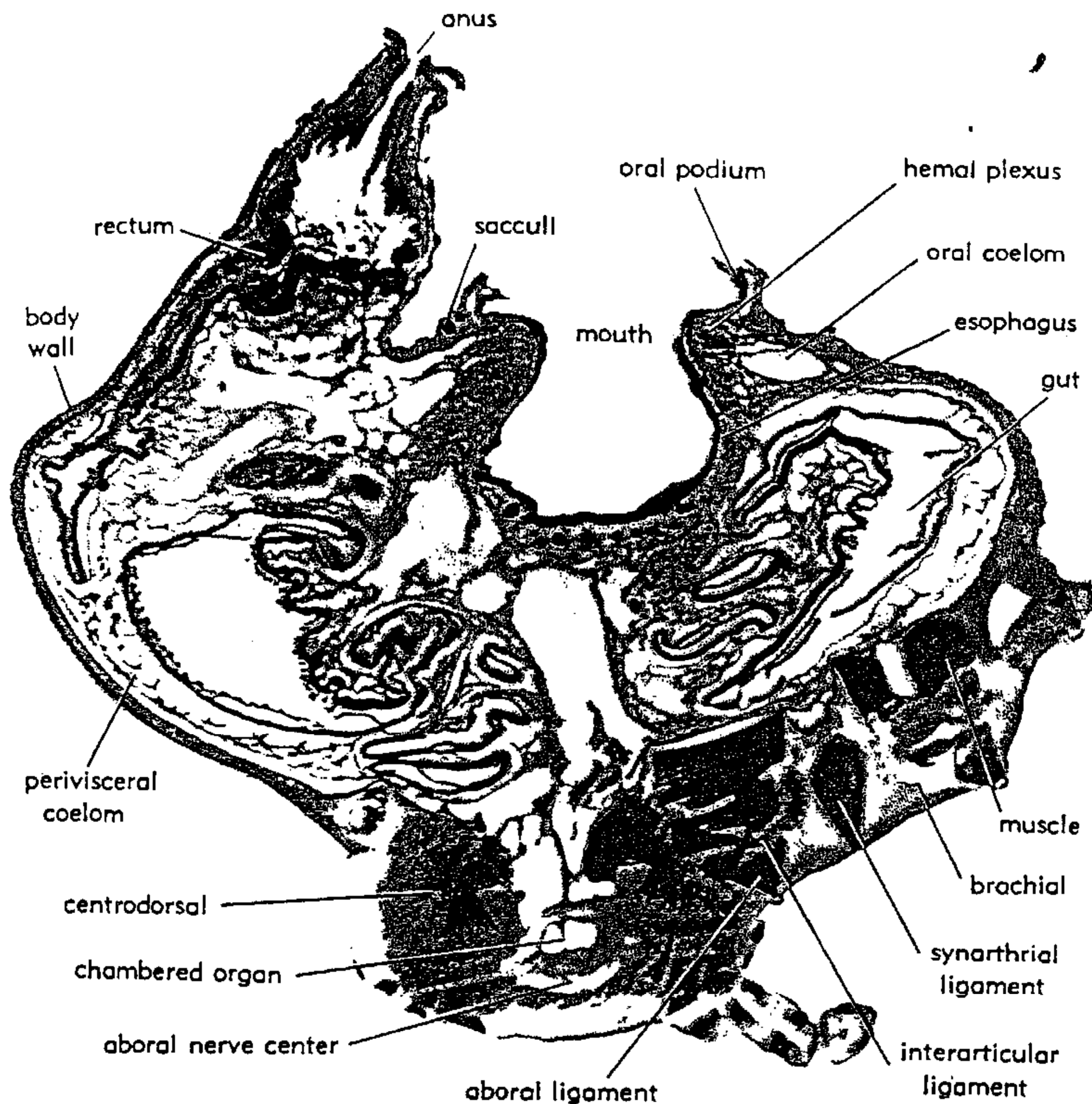
FIG. 1. Vertical sagittal section through theca of Antedon bifida [from preparations in the British Museum (Natural History), London] (Breimer, n).
