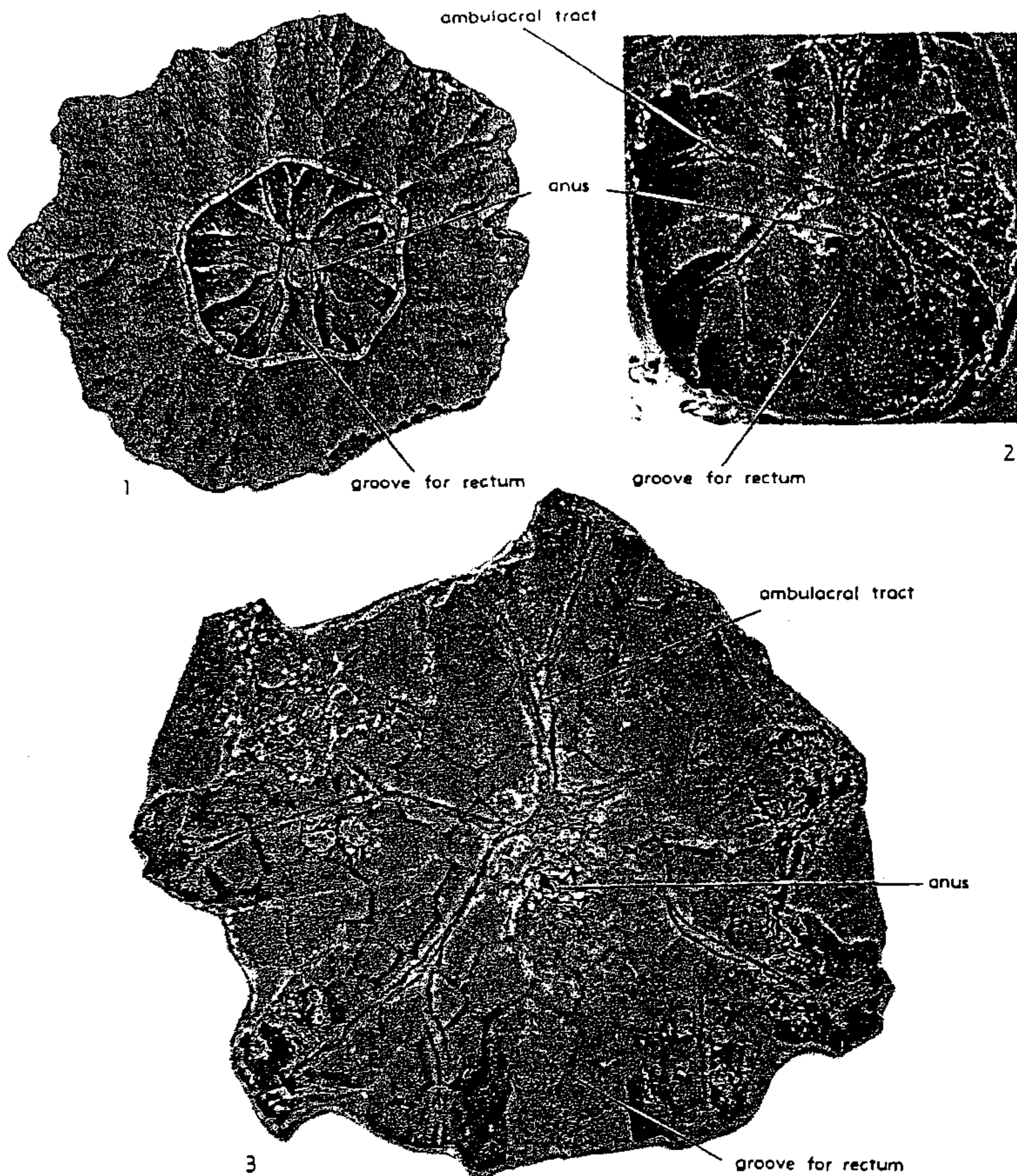
FIG. 167. Inner tegmental structures in camerates.—1. Strotocrinus regalis (HALL), Miss., USA (Iowa-Mo.); theca in aboral view, with part of aboral cup broken away, exposing subtegminal galleries and grooves for rectum and ambulacral tracts, \times 0.67 (Wachsmuth & Springer, 1897).—2. Physetocrinus ornatus (HALL), Miss., USA (Mo.); inner view of tegmen, latex cast, USNM S 1259, \times 2 (Ubaghs, n).—3. Strotocrinus regalis (HALL), Miss., USA (Mo.); inner view of tegmen, latex cast, USNM S 1275, \times 3 (Ubaghs, n).
