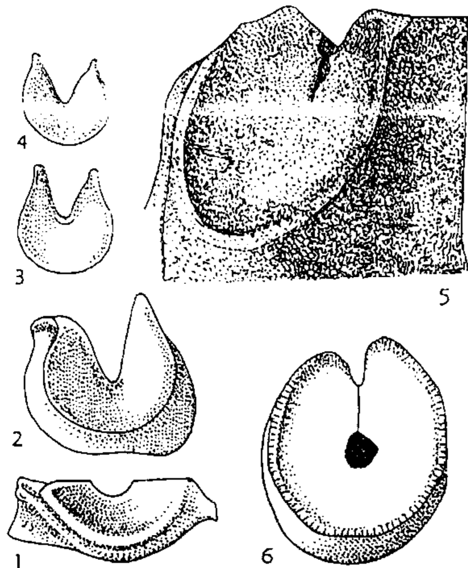
FIG. 143. Synostosial articulations.—1-4. Aethocrinus moorei UBAGHS, L.Ord., France; distal facets of second fixed primibrach, of a free primibrach, and of two secundibrachs, \times 10 (Ubaghs, 1969).—5. Thetidocrinus piriformis WANNER, Perm., Timor; a radial facet in oblique view, \times 3 (Wanner, 1937).—6. Barycrinus hoveyi (HALL), Miss., USA (Ind.); distal facet of third primibrach, \times 3 (Van Sant in Van Sant & Lane, 1964).
