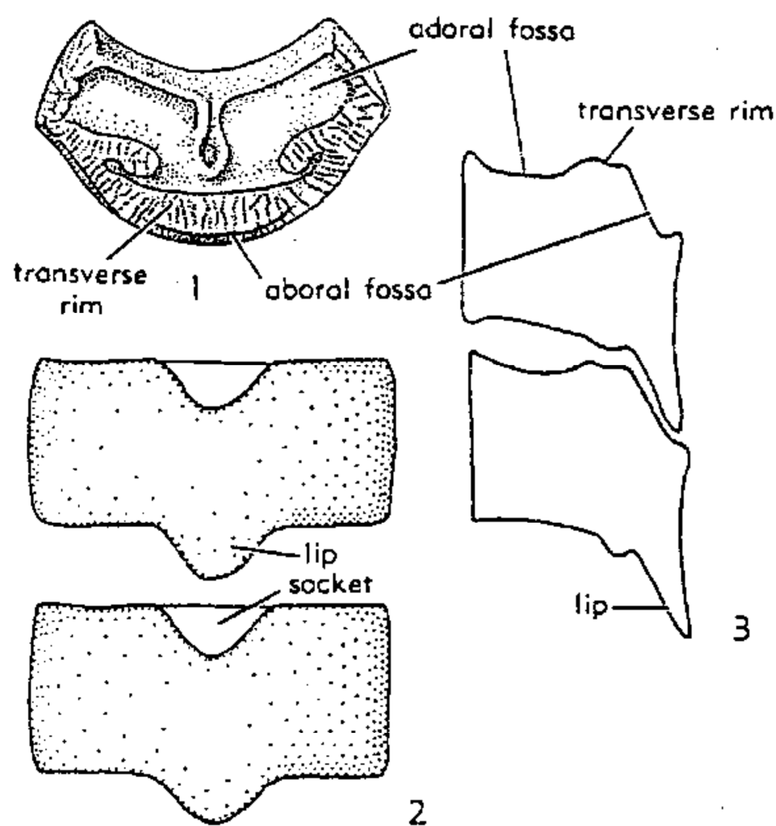
FIG. 141. Forbesiocrinus nobilis DE KONINCK & LE HON, L.Carb., Belg. (Springer, 1920).—1. Distal facet of second primibrach, \times 2.8 .—2,3. Diagrammatic representation of a pair of brachials, from aboral side and in long. median section.
