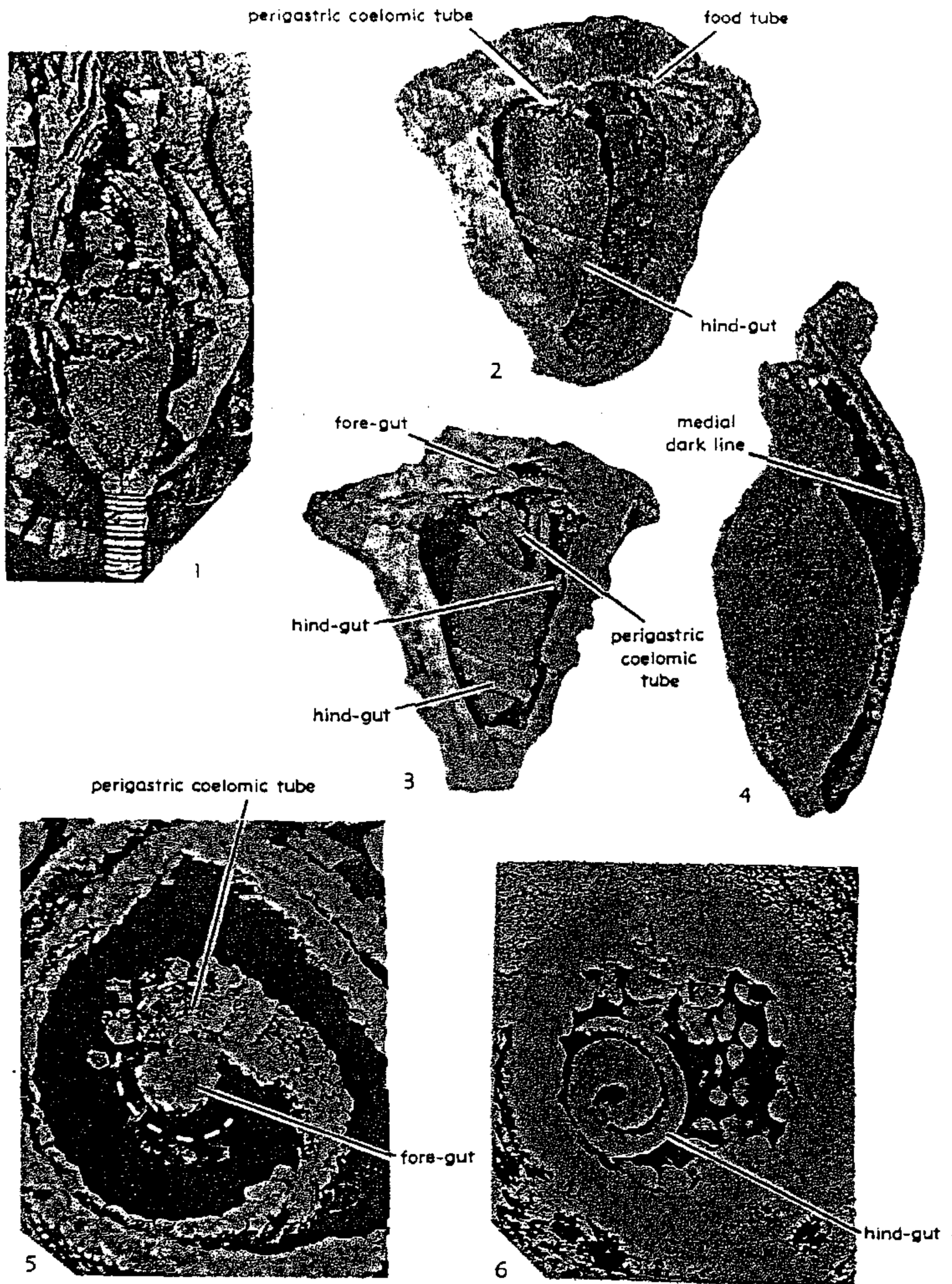
FIG. 170. Convoluted organ of camerate crinoids (2-6, from Journal of Paleontology, v. 49, no. 3, May, 1975, courtesy of The Paleontological Society and Bruce N. Haugh). 1. Ptychocrinus fimbriatus (SHUMARD), M.Ord., USA(Mo.); theca open showing convoluted organ (lat. view), \times 4 (Brower, 1973). 2. Teleiocrinus umbrosus (HALL), L.Miss., USA (Iowa); theca open with whole convoluted organ, \times 1.1 (Haugh, 1975a). 3. Teleiocrinus liratus (HALL), L.Miss., USA (Iowa); theca open with convoluted organ partly broken, \times 0.8 (Haugh, 1975a). 4. Actinocrinites verrucosus (HALL), Miss., USA (Ind.); central part of convoluted organ (Haugh, 1975a).
