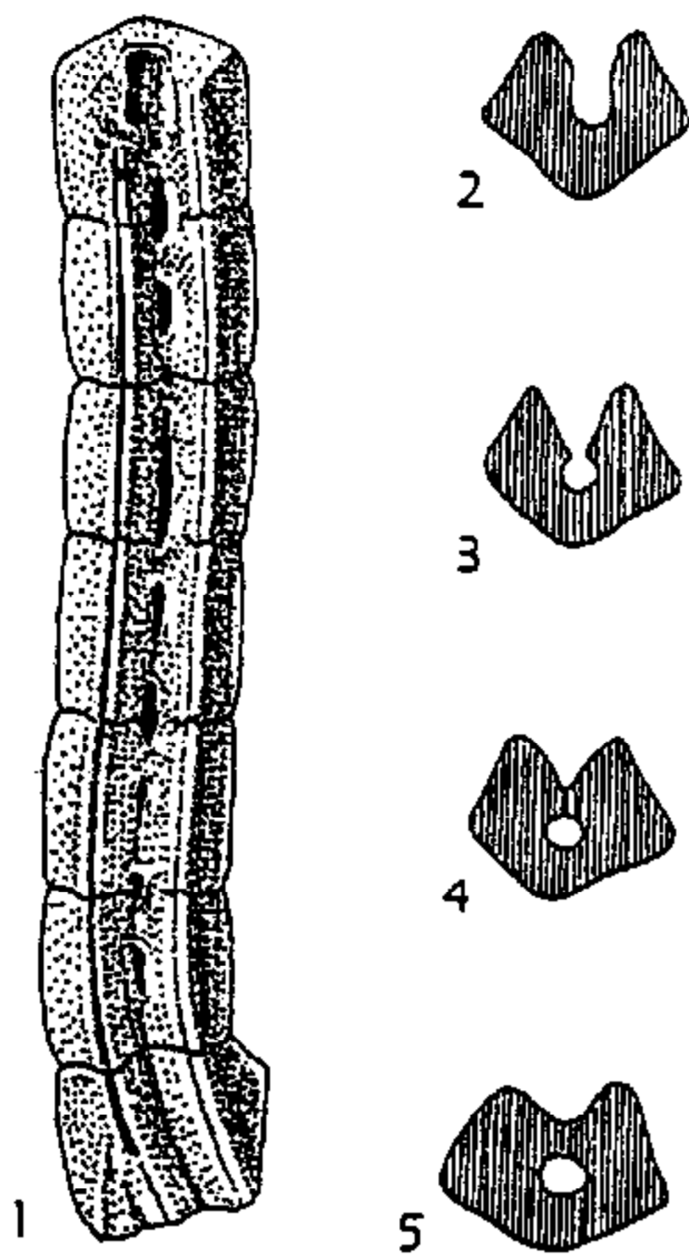
FIG. 107. Differentiation of axial canal from ventral groove.—1. Gissocrinus sp. cf. G. goniodactylus (PHILLIPS), Sil., Gotl., part of an arm in adoral view, showing axial canal still partly confluent with ventral groove, X6 (Bather, 1893a).—2-5. Gissocrinus goniodactylus (PHILLIPS), Sil., Eng., Gotl.; stages in separation of an axial canal, X8 (Bather, 1900a).
