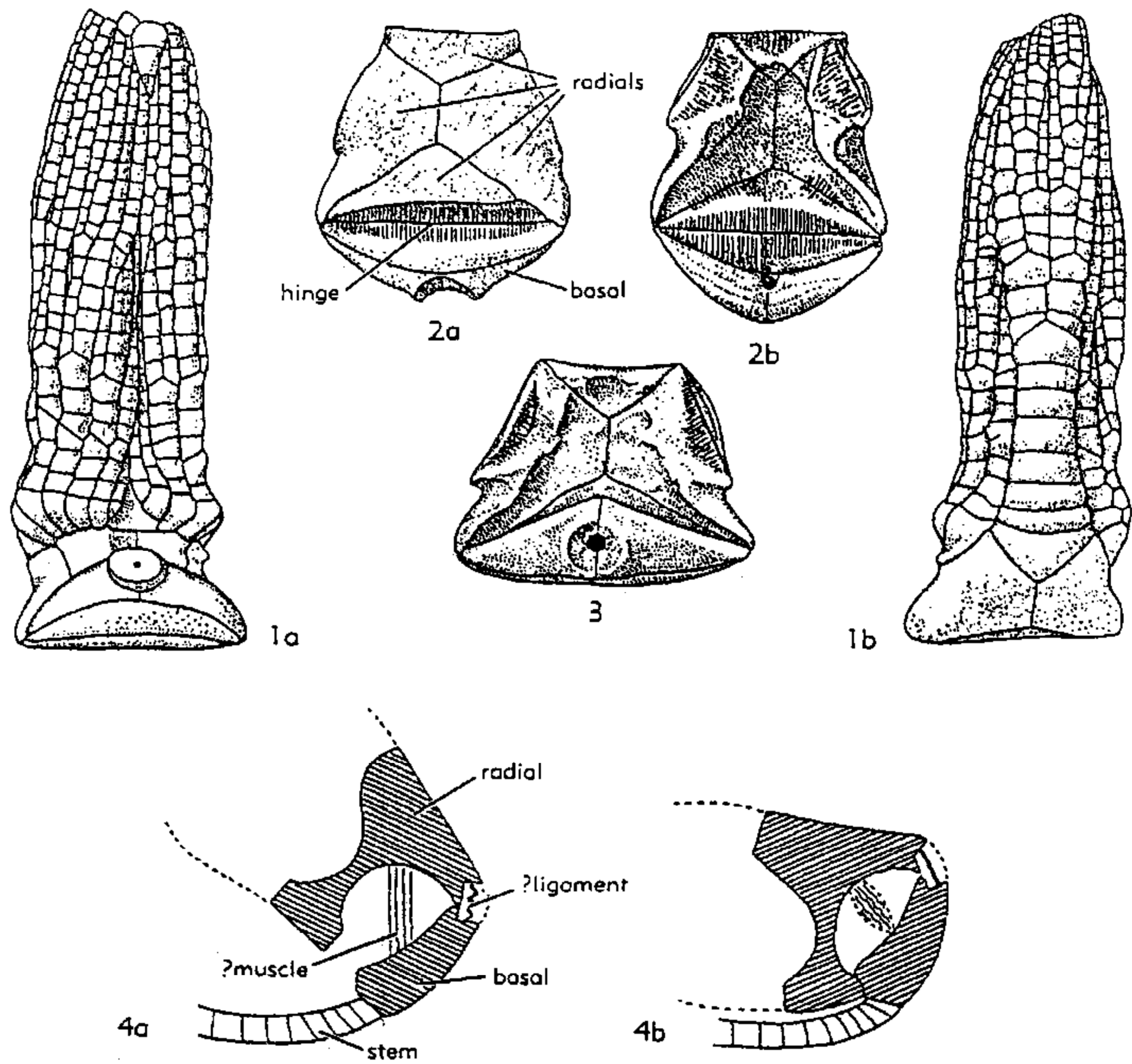
FIG. 104. Hingement in cup of calceocrinid inadunates.
