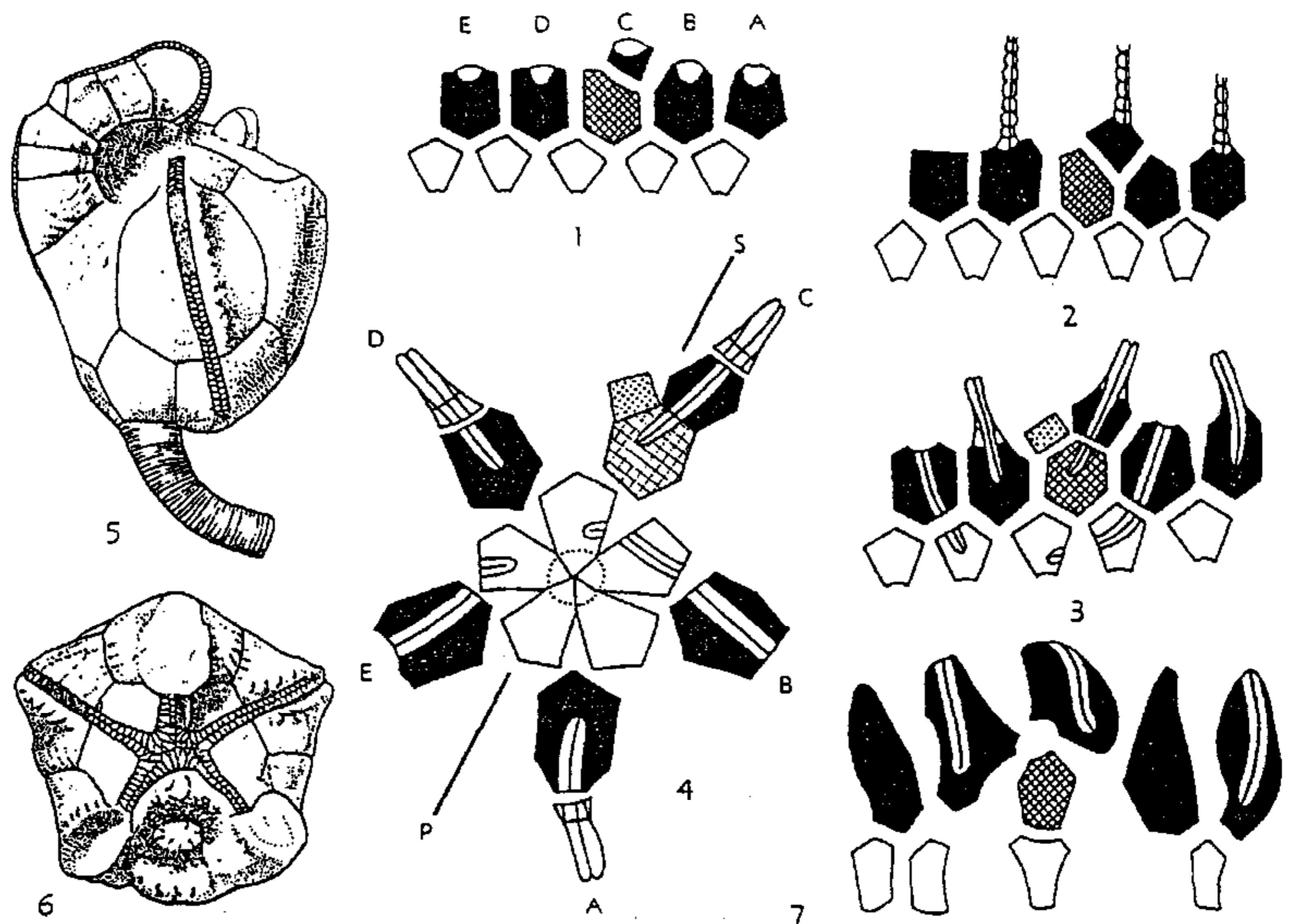
FIG. 109. Reduction of numbers of arms illustrated by hybocrinid inadunates. [Explanation: P-S, plane of bilateral symmetry; rays identified by letter symbols of the CARPENTER system; anal X stippled; radials black; radial cross ruled.]
