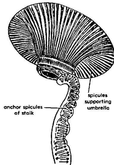
FIG. 162. Umbrella tube foot of Micropyga (from 4, after Döderlein).
