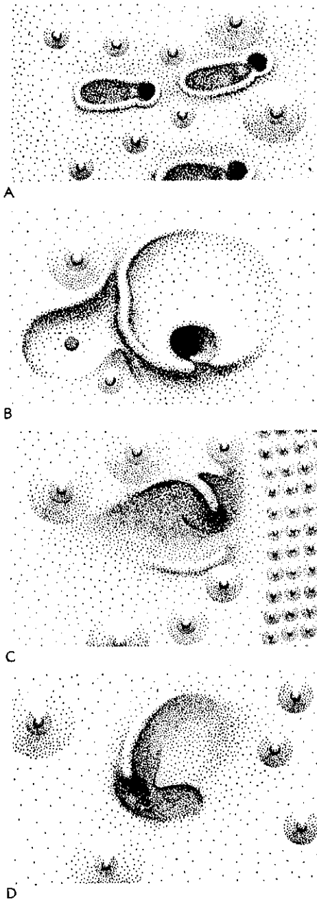
FIG. 207. Pores in test of Echinocardium cordatum for various types of tube feet (4).—A. Pores for funnel-building tube feet in ambulacrum III, with inner fasciole.—B. Pores for oral food-gathering. (Continued at right.)
