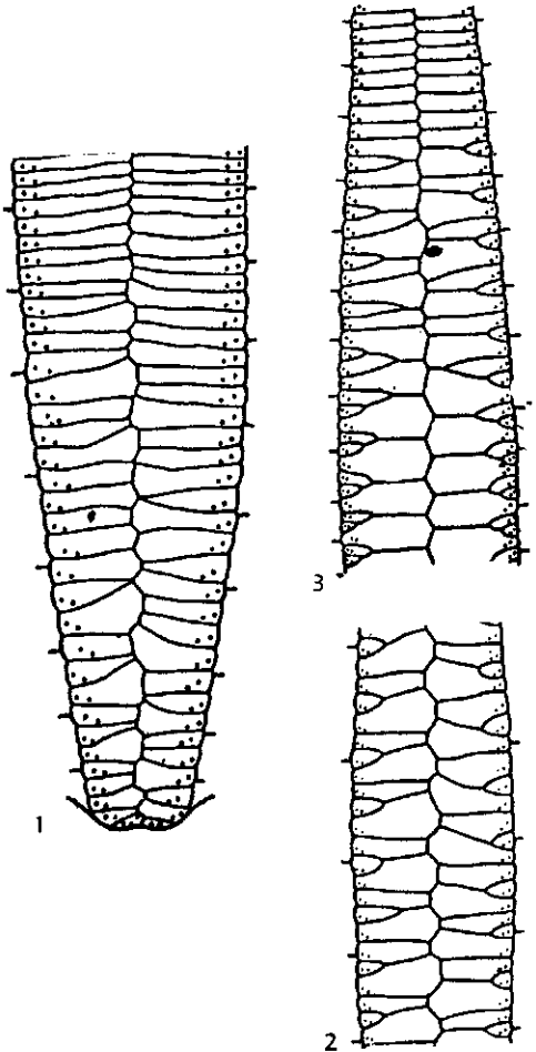
FIG. 177. Types of ambulacral structures in echinoids (6).—1. Pleisichinoid type in adoral half of ambulacrum of Plesiechinus .—2. Pyrinid type in medial part of ambulacrum of Conulus .—3. Discodeid type in medial part of ambulacrum of Camerogalerus .
