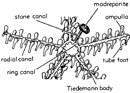
FIG. 2. Diagram of parts of starfish water-vessel system (104).
