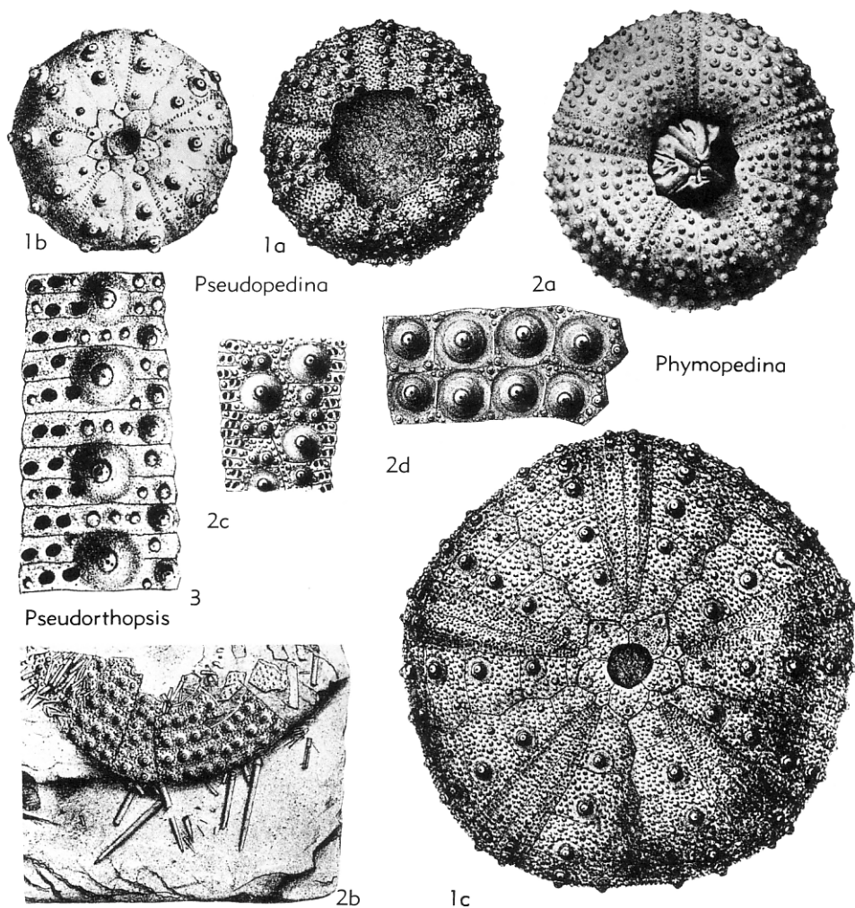
FIG. 268. Pedinidae (p. U362-U365).
