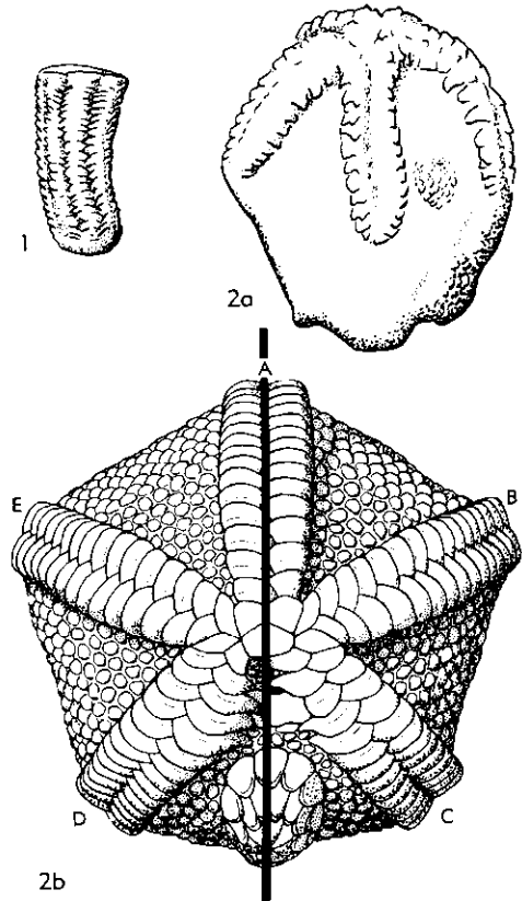
FIG. 102. Edrioasteroids, showing side view of cylindrical form (1) and D -ray side view and oral view (2a,b) of globose form, anteroposterior plane of bilateral symmetry strongly defined in all, not to scale (1, from Aurivillius; 2a, from Jaekel; 2b, from Kesling).
