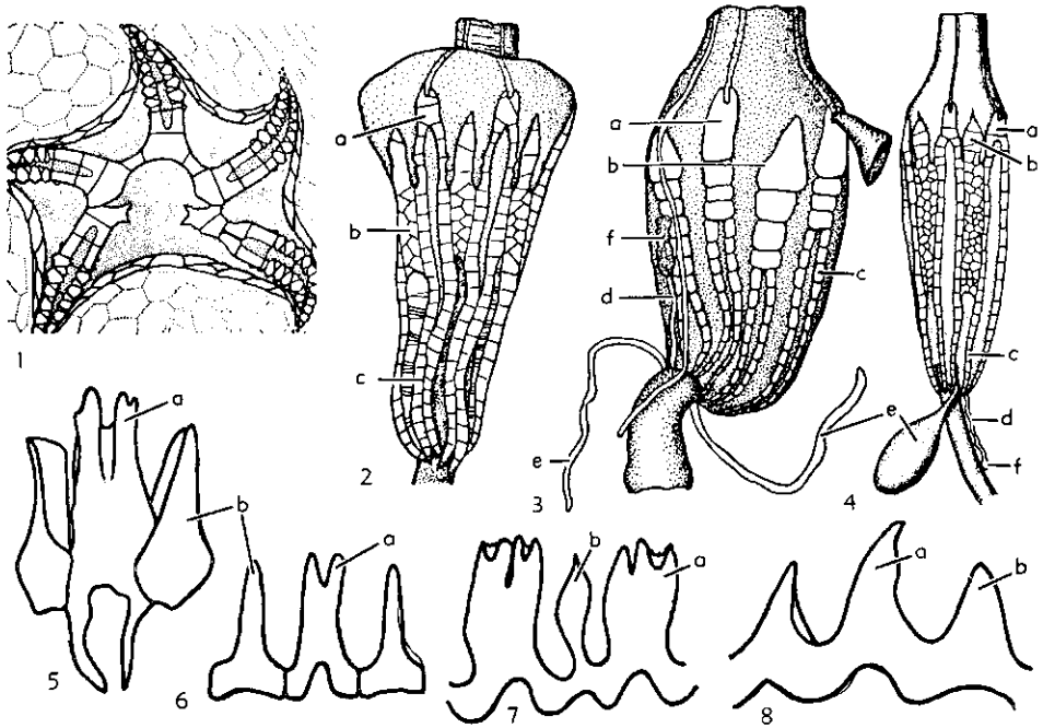
FIG. 95. Calcareous rings of edrioasteroid and holothurians.—1. Oral side of Isorophus , U.Ord. edrioasteroid, showing calcareous ring and associated ambulacral plates (10).—2-4. Side views of pharyngeal region of dendrochirotidan holothurians Pentadactyla , Placothuria , and Neothyonidium , showing calcareous rings and associated structures, all Rec. (Pawson).—5-8. Diagrammatic outlines of part of calcareous rings of Euthyonidiella , Psolus , Thyonidium , and Mitsukurietta , from side (all Rec. dendrochirotidan holothurians) (5,7,8, from Hedling & Panning, 1954; 6, Pawson). [Explanation: a , radial piece of calcareous ring; b , interradial piece; c , posterior process of radial; d , madreporic duct (or stone canal); e , Polian vesicle; f , madreporite.]
