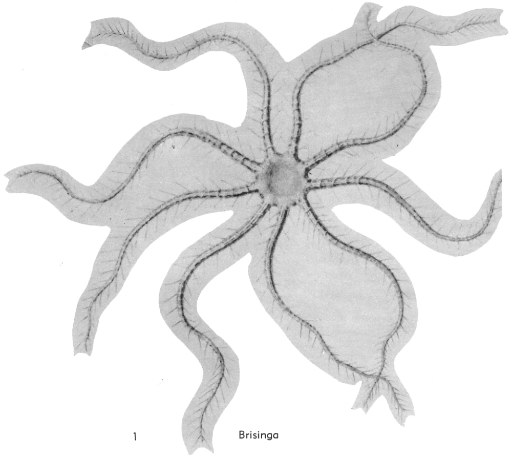
FIG. 67. Brisingidae (p. U77).
