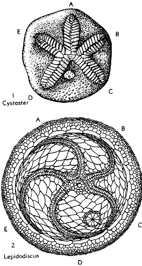
FIG. 114. Edrioasteroids with straight and curved ambulacra.—1. Cystaster granulatus HALL., U. Ord., USA (Ohio), a simple type characterized by relatively wide, short, and straight rays, \times 4.5 (20).—2. Lepidodiscus ephraemovianus (BOGOLUBOV), U.Dev. (Famenn.), USSR, showing contrasolar curvature of long, narrow ambulacra in all rays except C, which is solar, \times 2.8 (18).
