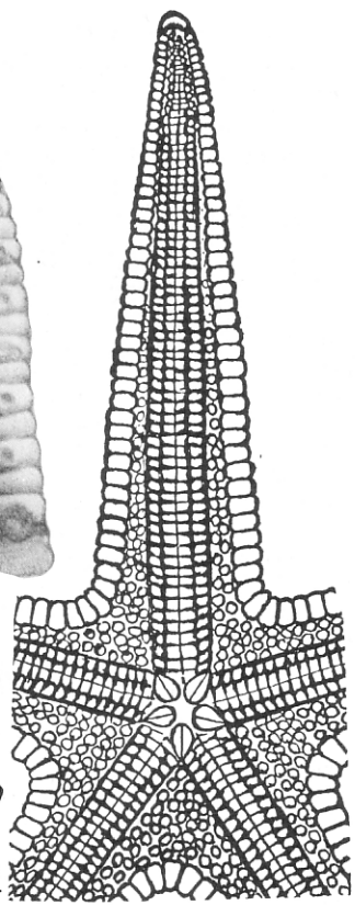
FIG. 44. Astropectinidae (Astropectininae) (p. U45-U46).
