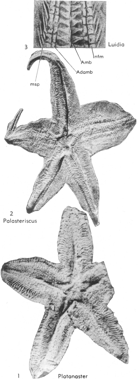
FIG. 42. Palasteriscidae (1,2); Luidiidae (3). [Explanation: Adamb , adambulacrum; Amb , ambulacrum; Injm , inferomarginal; MAP , mouth-angle plate; msp , marginal spine.] (p. U42-U43).
