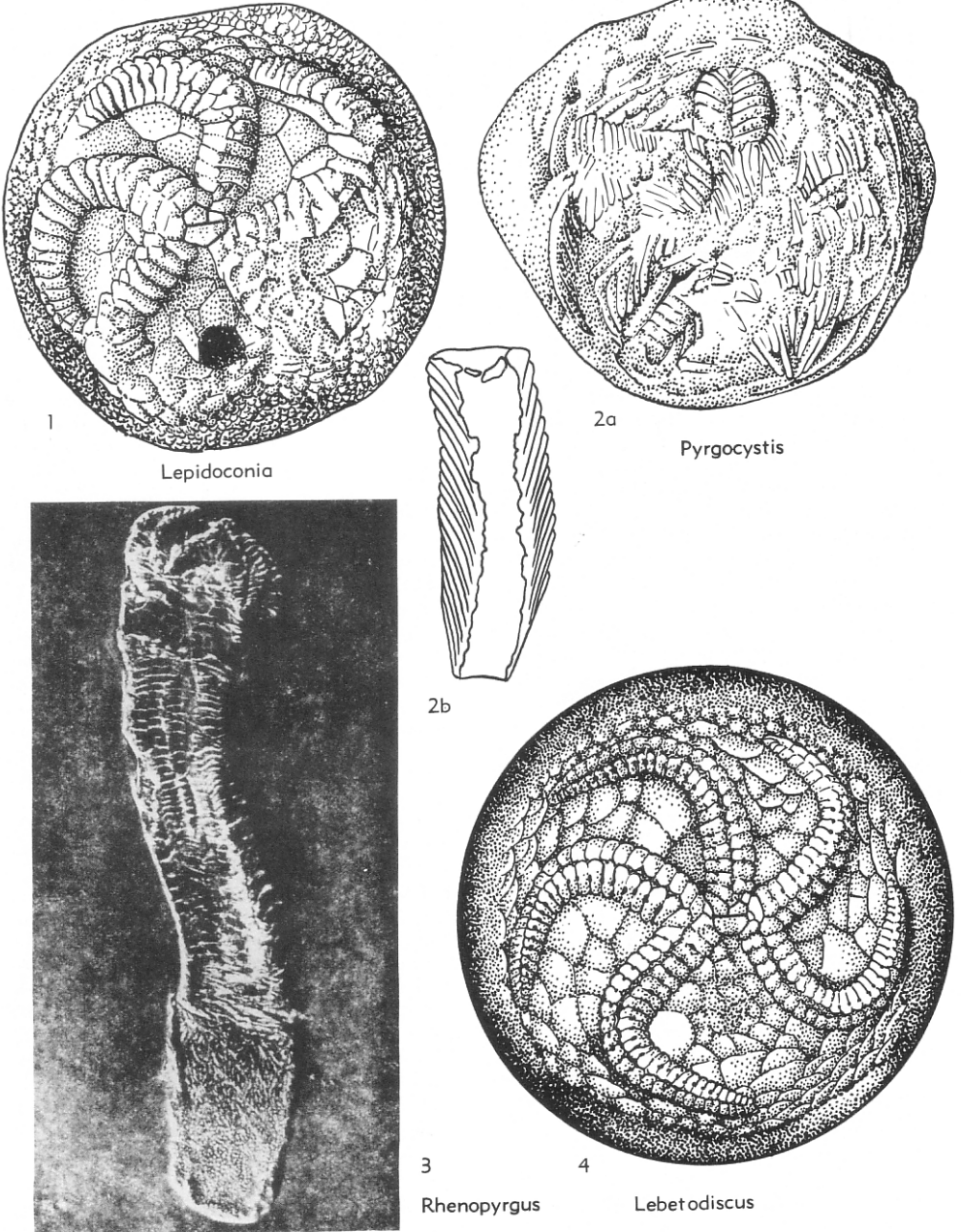
FIG. 127. Hemicystitidae (p. U165-U167).
