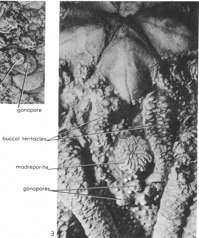
FIG. 137. Sollasina and Eucladia , U.Sil.(L.Ludlov.), Eng.; 1,2, S. woodwardi (SOLLAS), features of oral side, \times 5 ; 3, E. johnsoni WOODWARD, part of oral side, \times 5 (all Ubaghs, n).
