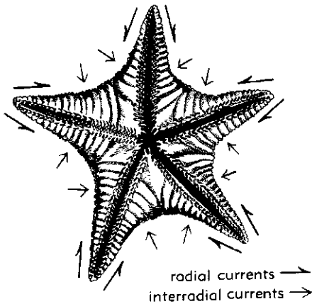
FIG. 15. Oral surface of recent asteroid Porania , showing large interradia and ciliate grooves; arrows indicate direction of flow of water currents (111).
