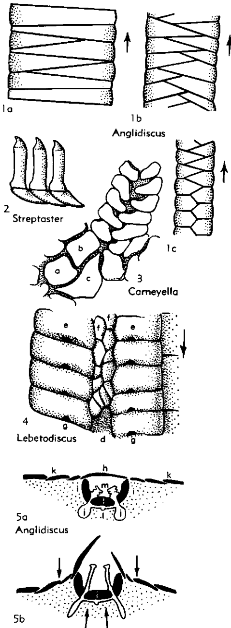
FIG. 117. Form and relationships of edrioasteroid cover plates.—1. Anglidiscus fistulosus (ANDERSON), I. Carb., Eng., showing development of cover plates in different parts of single ambulacrum, arrows pointing toward mouth, \times 28 (1); 1a-c, proximal, medial, distal.—2. Streptaster septembra-chiatus MILLER & DYER, U.Ord., USA (Ohio), 3 vertically disposed palisade-like cover plates borne
