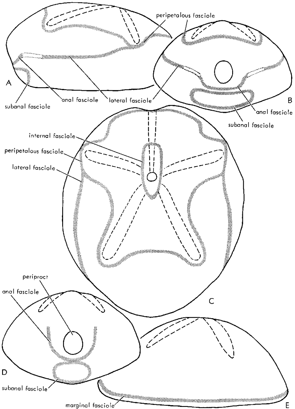
FIG. 185. Fascioles of spatangoid tests (diagram.) (Durham, n).—A. Side view of test showing lateral and other fascioles (termed lateroanal fasciole if lateral and anal fascioles are continuous).—B. Posterior view of test showing subanal and other fascioles.—C. Aboral view of test showing peripetalous and other fascioles.—D. Posterior view of test showing anal and subanal fascioles.—E. Side view of test showing marginal fasciole.
