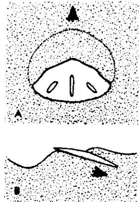
FIG. 208. Sand dollar Mellita lata burrowing, (A) seen from above, (B) side view (2, courtesy Trustees, British Museum, Natural History).
