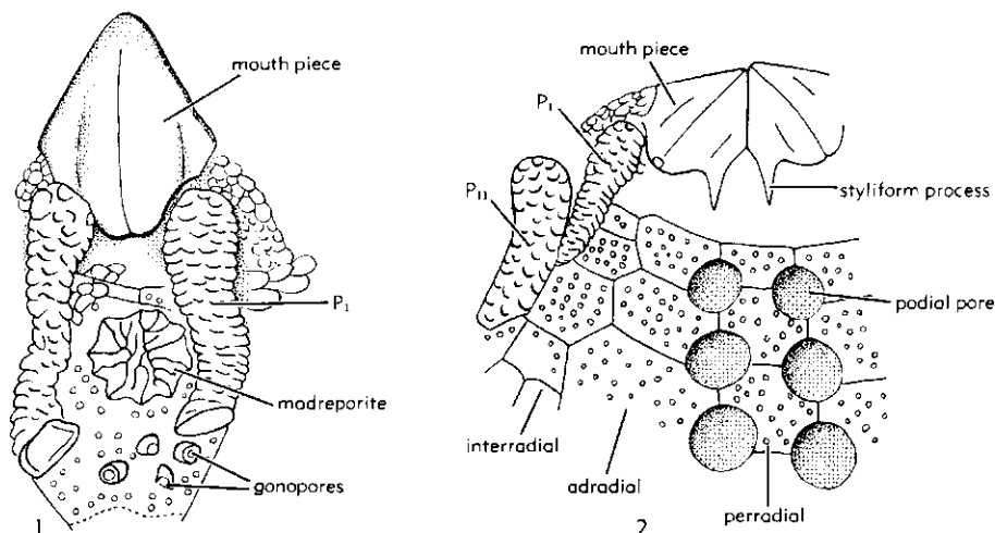
FIG. 136. Eucladia johnsoni WOODWARD, U.Sil.(L.Ludlov.), Eng.; 1, part of B ray and BC interray, \times 2 (4); 2, part of CD interray, \times 2.7 (4). [Explanation: P 1 , P 11 , 1st, 2nd pairs of podia.]
