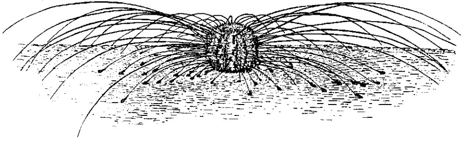
FIG. 200. Diademate echinoid Plesiadiadema indicum (DÖDERLEIN), showing exceptionally long curved slender spines, \times 0.35 (Mortensen, 1923).
