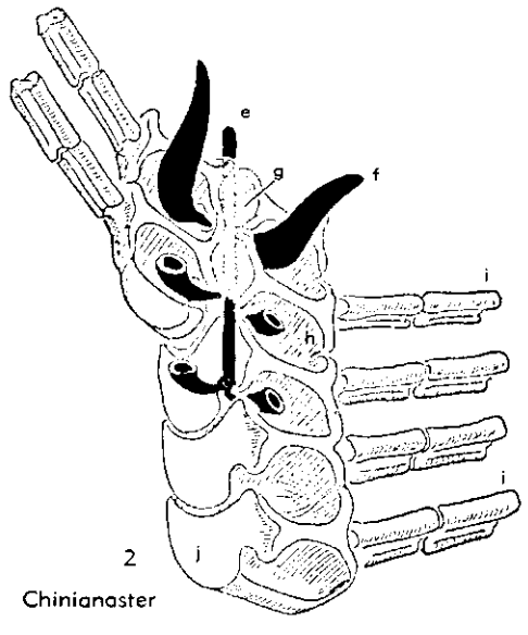
FIG. 8. Axial structures and tube feet of primitive somasteroids (108).—1. Villebrunaster thorali SPENCER, L.Ord., Fr.; 1a, arm skeleton near tip, \times 6 ; 1b, interpretation of mid-arm structure, \times 10 .—2. Chinianaster levyi THORAL, L.Ord., Fr. [Explanation: a, capitulum of ambulacral; b, adambulacral virgal; c, shelf of cupule (basin for tube foot); d, passage from cupule to arm interior; e, radial water vessel; f, tube foot; g, adductor muscle; h, cupule; i, virgal; j, ambulacral.]
