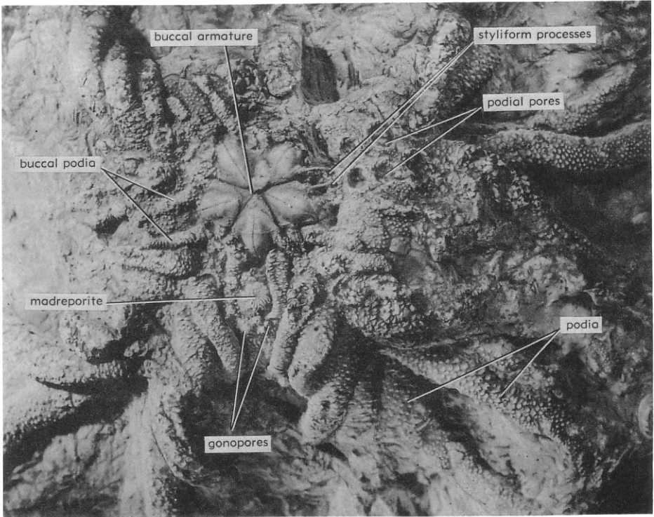
FIG. 132. Eucladia johnsoni WOODWARD, U.Sil.(L.Ludlov.), Eng.; part of oral surface showing morphological features, \times 1.3 (Übaghs, n).
