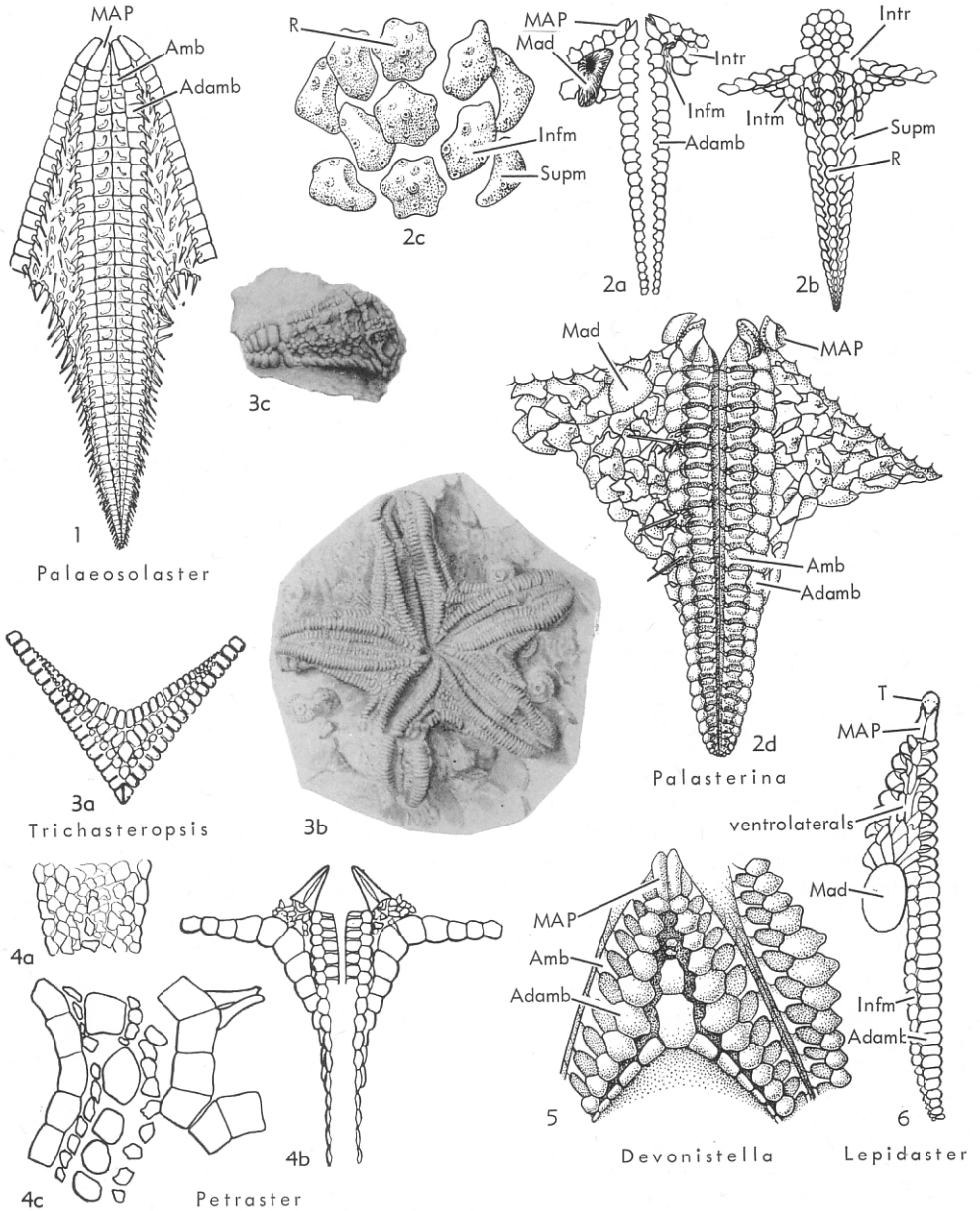
FIG. 43. Petrasteridae (4); Lepidasteridae (5,6); Palasterinidae (1-3). [Explanation: Adamb , adambulacral; Amb , ambulacral; Infm , inferomarginal; Intr , intermarginal; Intr , interradial; Mad , madreporite, MAP , mouth-angle plate; R , radial; Supm , superomarginal; T , torus.] (p. U43-U45).
