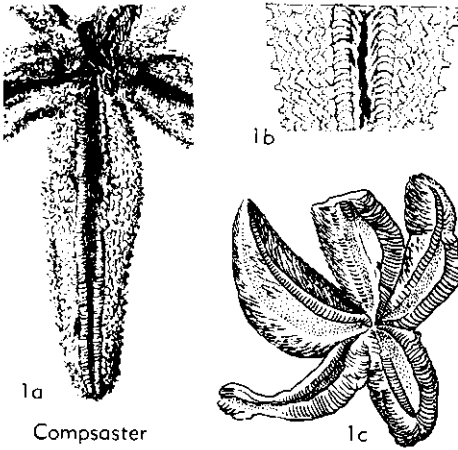
FIG. 65. Compasteridae (p. U74).
