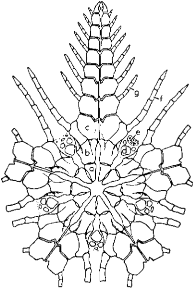
FIG. 13. Chinianaster levyi THORAL, L.Ord., Fr.; oral side of juvenile specimen, \times 6.3 (108). [Explanation: a-c, 1st, 2nd, 3rd ambulacra, b and c united syzygially; d, tegmental; e, inferred madreporite; f, oral pinnule; g, 4th metapinnule.]
