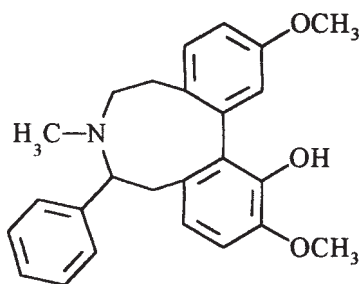
phenyldihydrothebaine
