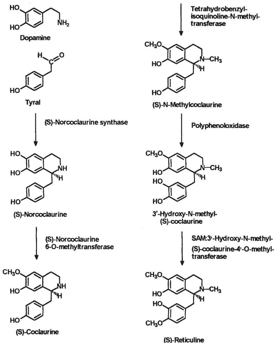
Figure 6 The biosynthetic pathway of (S)-reticuline
