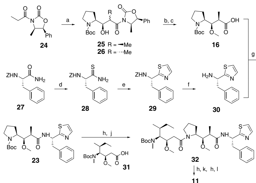
Scheme 15.3. Shioiri-Hamada synthesis of dolastatin 10. (a) \text{Et}_3\text{N} , n -Bu 3 BOTf, 12 , \text{H}_2\text{O}_2 , 99%. (b) 25 , LiOH, \text{H}_2\text{O} , 98%. (c) NaH, \text{CH}_2\text{I}_2 , 89%. (d) Lawesson's reagent, 97%. (e) (1) \text{BrCH}_2\text{CHO} , \text{K}_2\text{CO}_3 , (2) (\text{CF}_3\text{CO})_2\text{O} , 66%, 2 steps. (f) (1) 25% HBr/AcOH, (2) aq. \text{NaHCO}_3 , 99%. (g) DEPC, \text{Et}_3\text{N} , 97%. (h) TFA. (j) 31 , DEPC, \text{Et}_3\text{N} , 99%. (k) Boc-Val, Bop-Cl, \text{Et}_3\text{N} , 59%. (l) Dov, DEPC, NMM, 90%
