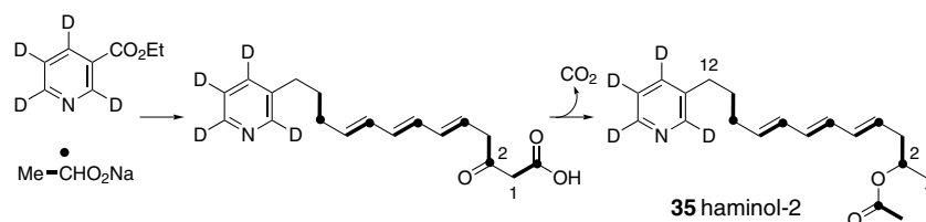
Fig. 14.5. Incorporation of \text{d}_4 -nicotinic acid ethyl ester, [\text{1-}^{13}\text{C}] -acetate and [\text{1,2-}^{13}\text{C}_2] -acetate into haminol-2 (35)
