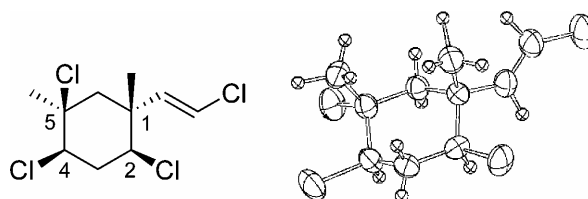
aplysiaterpenoid A ( 5 )
