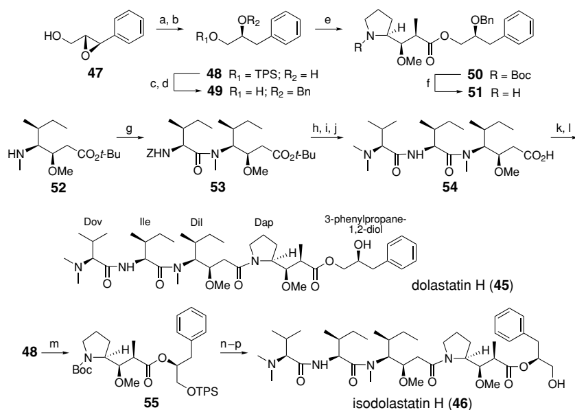
Scheme 15.7. Yamada synthesis of dolastatin H and isodolastatin H. (a) DIBAL, 62%. (b) TPSCl, imidazole, 78%. (c) BnBr, LiN(SiMe 3 ) 2 , 75%. (d) HF, 97%. (e) 16 , DCC, DMAP, CSA, 86%. (f) TFA. (g) Z-Ile, PyBOP, DIPEA, 83%. (h) H 2 , Pd/C. (i) Dov, DEPC, Et 3 N, 95%, 2 steps. (j) TFA. (k) 51 , DEPC, Et 3 N, 87%, 2 steps. (l) H 2 , Pd/C, AcOH, 77%. (m) 16 , DCC, DMAP, CSA, 85%. (n) TFA. (o) 54 , DEPC, Et 3 N, 52%, 2 steps. (p) HF, 87%
