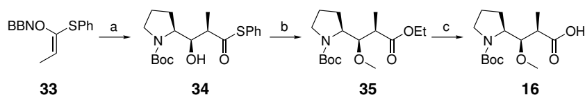
Scheme 15.4. Koga Boc-Dap preparation. (a) 12 , 64%. (b) (1) \text{K}_2\text{CO}_3 , 88%, (2) LHMDS, MeOTf, 83%. (c) LiOH, 91%
