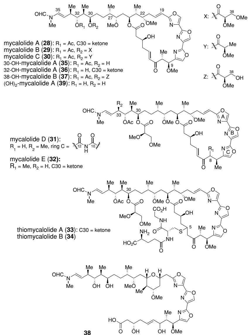
Fig. 11.4. Structures of mycalolides and their degradation products
