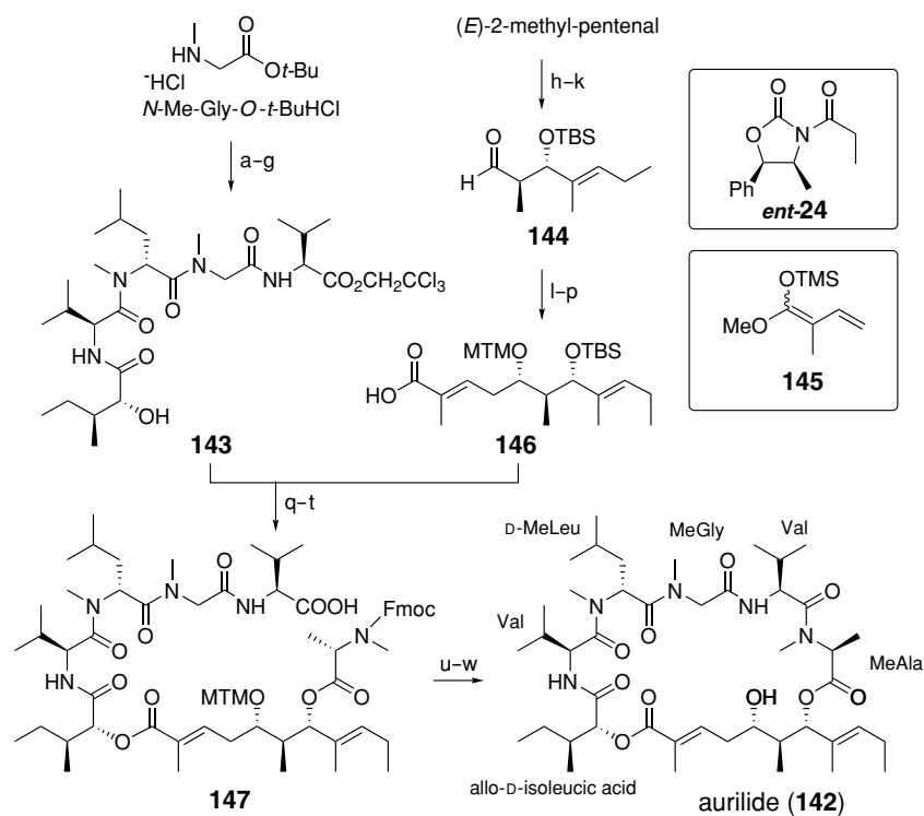
Scheme 15.20. Yamada synthesis of aurilide. (a) Z-D-Me-Leu, DEPC. (b) H 2 , Pd/C. (c) Z-L-Val, PyBOP, i -Pr 2 EtN. (d) H 2 , Pd/C. (e) allo -D-isoleucic acid Na salt, EDCI-HCl, HOBT. (f) TMSOTf, 2,6-lutidine. (g) L-Val-OCH 2 CCl 3 , EDCI-HCl, HOBT, 84%, 7 steps. (h) Bu 2 BOTf, i -Pr 2 EtN, ent -24. (i) Me 2 AlN(Me)OMe. (j) TBSCl. (k) DIBAL, 78%, 4 steps. (l) 145 , BF 3 ·Et 2 O. (m) Dess-Martin oxid. (n) NaBH 4 . (o) DMSO, Ac 2 O, AcOH. (p) LiOH, 44%, 5 steps. (q) EDCI-HCl, DMAP. (r) HF-Py, Py. (s) Fmoc-L-Me-Ala, EDCI-HCl, DMAP. (t) Zn, NH 4 OAc, 83%, 3 steps. (u) Et 3 NH. (v) EDCI-HCl, HOAt. (w) AgNO 3 , 2,6-lutidine, 62%, 3 steps
