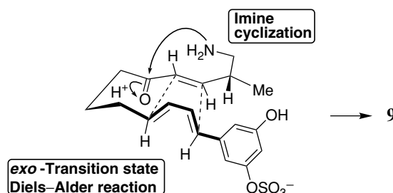
Fig. 2.4. Proposed biogenesis of symbioimine ( 9 )
