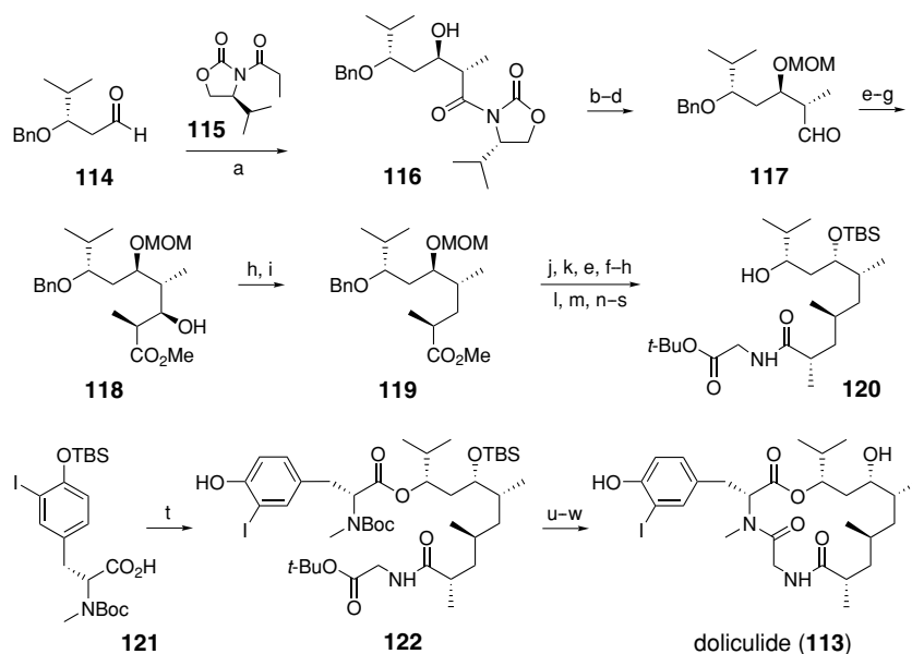
Scheme 15.17. Yamada synthesis of dolicolide. (a) 115 , \text{Bu}_2\text{BOTf} , \text{Et}_3\text{N} , 95%. (b) \text{Me}(\text{MeO})\text{NH}\cdot\text{HCl} , \text{Me}_3\text{Al} . (c) \text{MeOCH}_2\text{Cl} , i\text{-Pr}_2\text{NEt} . (d) DIBAL, 80%, 3 steps. (e) 115 , \text{Bu}_2\text{BOTf} , \text{Et}_3\text{N} . (f) \text{LiOH} , \text{H}_2\text{O}_2 . (g) \text{CH}_2\text{N}_2 , 85%, 3 steps. (h) \text{Im}_2\text{CS} , THF. (i) \text{Bu}_3\text{SnH} , 73%, 2 steps. (j) \text{LiAlH}_4 . (k) DMSO, (\text{COCl})_2 , \text{Et}_3\text{N} . (l) \text{Bu}_3\text{SnH} , 55%, 7 steps. (m) HCl. (n) \text{Ph}_3\text{P} , p\text{-NO}_2\text{C}_6\text{H}_4\text{COOH} , (\text{EtOOCN})_2 , 69%. (o) NaOH. (p) TBSOTf, \text{Et}_3\text{N} . (q) \text{K}_2\text{CO}_3 , 99%, 3 steps. (r) Gly- O - t -Bu-HCl, DEPC, \text{Et}_3\text{N} , 93%. (s) \text{H}_2 , \text{Pd}(\text{OH})_2/\text{C} . (t) 120 , DCC, DMAP, 94%. (u) TFA. (v) BOP-Cl, \text{Et}_3\text{N} , 74%. (w) \text{Bu}_4\text{NF} , 99%
