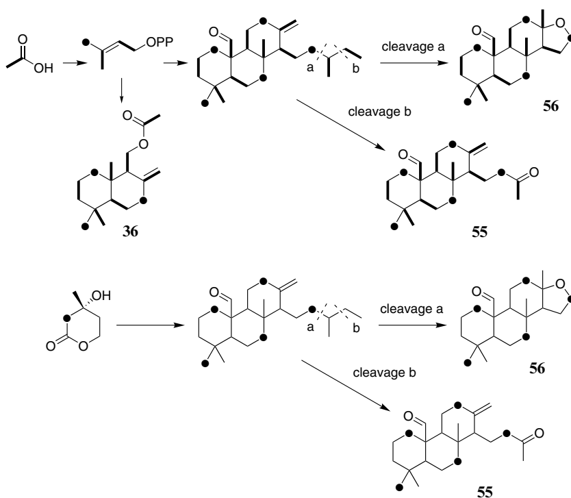
Scheme 13.2. Proposed biogenesis of albicanyl acetate ( 36 ), luteone ( 55 ), and cadlinaldehyde ( 56 ) that accounts for the observed labeling patterns resulting from feeding [1,2- 13 C 2 ] acetate and [2- 13 C] mevalonolactone
