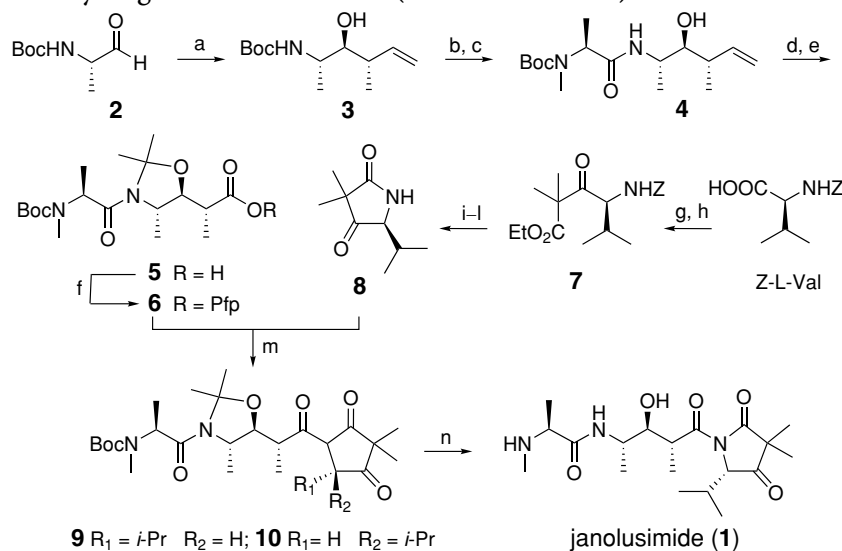
Scheme 15.1. Sodano synthesis of janolusimide. (a) (-) -Ipc 2 B-( E )-crotyl, 72%. (b) HCl. (c) N -Boc- N -Me-L-Ala, EDC, DMAP, 38%, 2 steps. (d) (\text{CH}_3)_2\text{C}(\text{OCH}_3)_2 , p -TsOH (cat.). (e) \text{NaIO}_4 , \text{RuCl}_2 , 36%, 2 steps. (f) \text{C}_6\text{F}_5\text{OH} , DCC, DMAP, 89%. (g) CDI, then \text{LiCH}_2\text{COOEt} . (h) \text{K}_2\text{CO}_3 , MeI. (i) \text{NaBH}_4 , 44%, 3 steps. (j) \text{H}_2 , Pd/C. (k) \text{NaOEt} . (l) PDC, 86%, 3 steps. (m) n -BuLi, 63%. (n) p -TsOH, 59%
