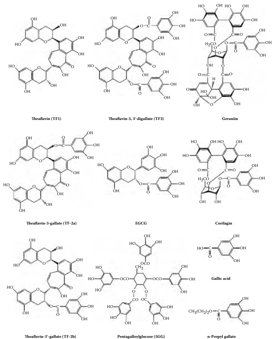
FIGURE 11.1 Chemical structures of selected polyphenols.
