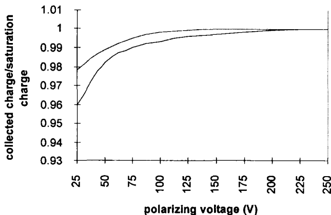
Fig.(7.9) The reduction in efficiency of a parallel plate ionization chamber at low polarizing voltage due to recombination. Top curve, 4 MeV electrons : Bottom curve, 18 MeV electrons. Data adapted from [5].
