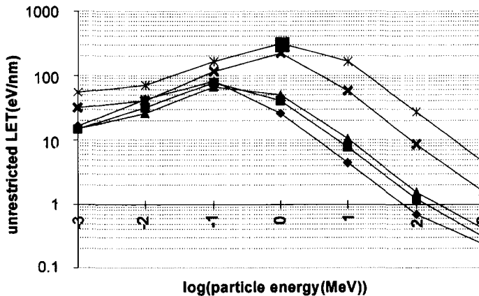
Fig.(9.37) Mass Stopping Powers of spallation products from Fig.(9.35) in water. ♦ protons : ■ deuterons : ▲ tritons : × He nuclei : ∗ Li nuclei. Note that the peak in the stopping power shifts to higher values and occurs at higher energies as the ions become heavier. Data taken from [33].
