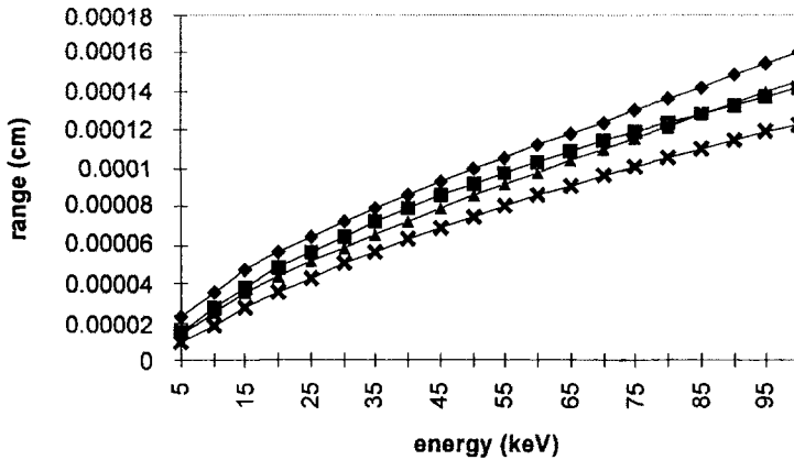
Fig.(2.2) The csda range r_o and mean penetration depth z_{av} in liquid water as a function of particle energy. Data taken from [3].
