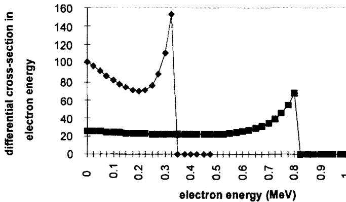
Fig.(3.11) Compton cross-section differential in electron energy Eq.(3.23) for incident photon energies 0.5 MeV (◆) and 1.0 MeV (■). The ordinate axis is in units of \text{m}^2 \text{electron}^{-1} \text{MeV}^{-1} \times 10^{-30} . The maximum electron energies in the two cases are 0.331 MeV and 0.796 MeV respectively, Eq.(3.15). The above curves do not show an infinitely sharp edge (the Compton edge) at these energies because of the finite energy increments taken along the abscissa axis.
