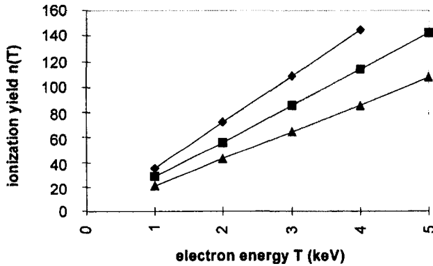
Fig.(2.28) High energy ionization yield n_n(T) versus electron energy. ◆ \text{CH}_4 ; ■ \text{N}_2 ; ▲ He. Data taken from [18], [19], [20].
