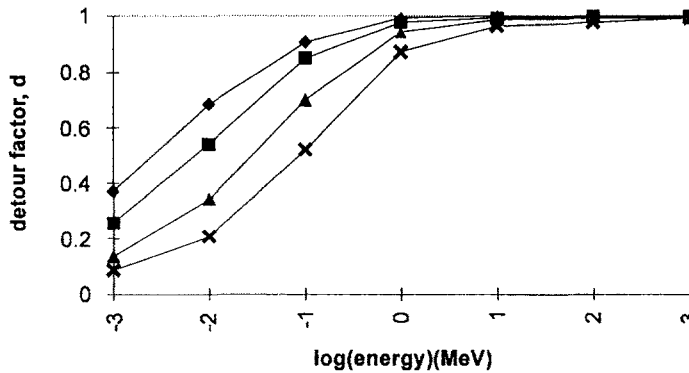
Fig.(2.3) Detour factor, d , versus proton energy (MeV) in various materials. \blacklozenge carbon : \blacksquare aluminium : \blacktriangle copper : \times tungsten, [3].
