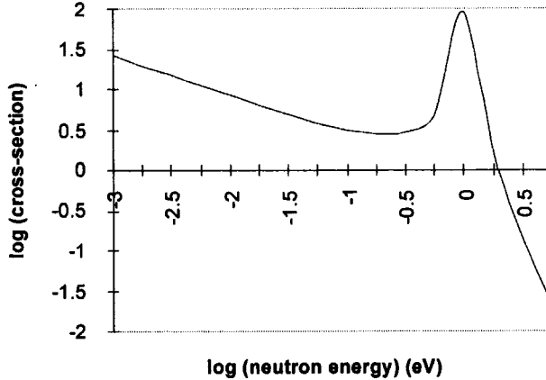
Fig.(4.3) The radiative capture cross-section, in arbitrary units, as given by the Breit-Wigner formula for energies below a single resonance at E_R = 1.0 eV having width \Gamma = 0.07 eV. The 1/v dependence at low energies is evident.
