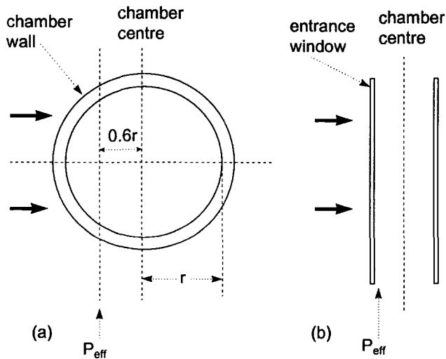
Fig.(7.13) Effective point of measurement, P_{\text{eff}} , for (a) cylindrical and (b) parallel-plate chambers. For all electron measurements, P_{\text{eff}} must be placed at the depth of interest, [5].
