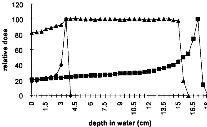
Fig.(9.30) Relative proton dose versus depth in water : \blacklozenge unmodulated 72 MeV [22] ; \blacksquare unmodulated 158.6 MeV [23] ; \blacktriangle Spread-Out-Bragg-Peak (SOBP) 158.6 MeV [23].
