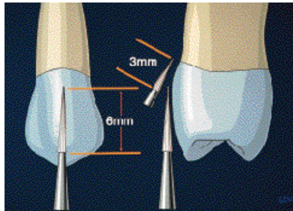
Figure 13-19C: This drawing shows the proper length and shape burs to use for contouring and finishing of posterior restorations.
