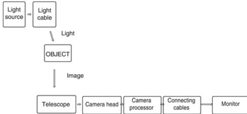
Fig. 2.3 Imaging chain. A clear understanding of this interlinked chain would allow trouble-shooting when the displayed image is absent or poor
