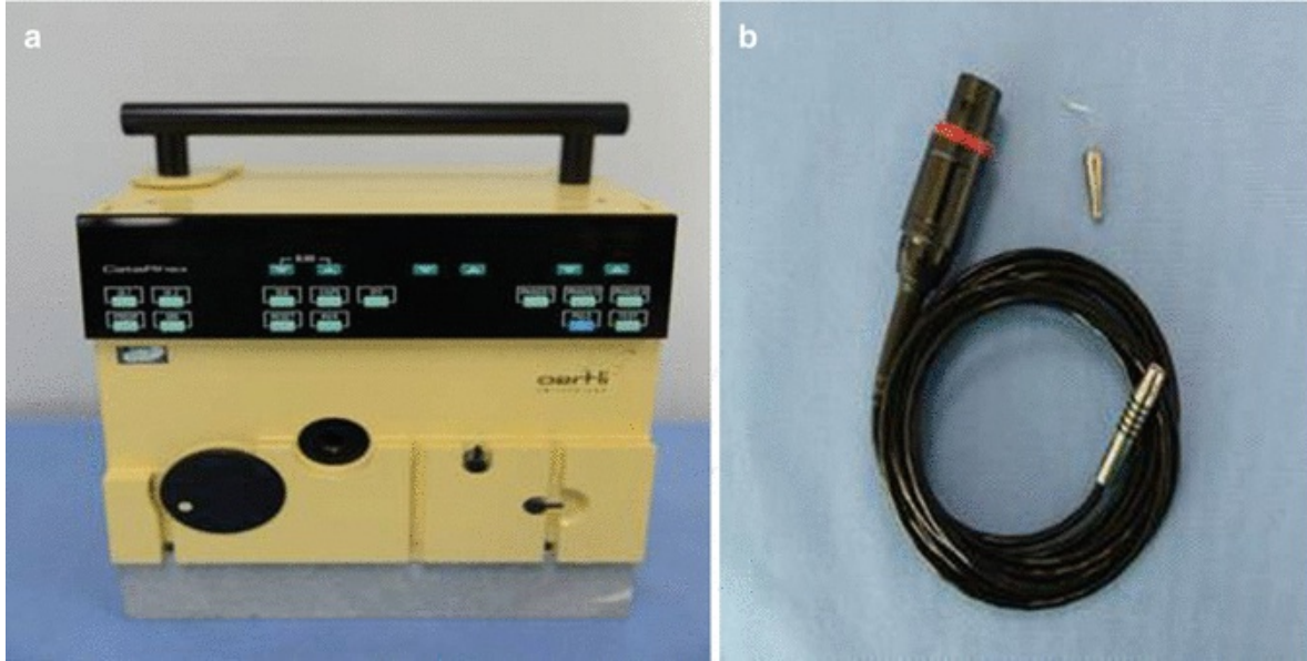
Fig. 11.4 (a) Radiofrequency diathermy device for capsulorhexis; (b) needle and wire for capsulorhexis with radiofrequency diathermy
