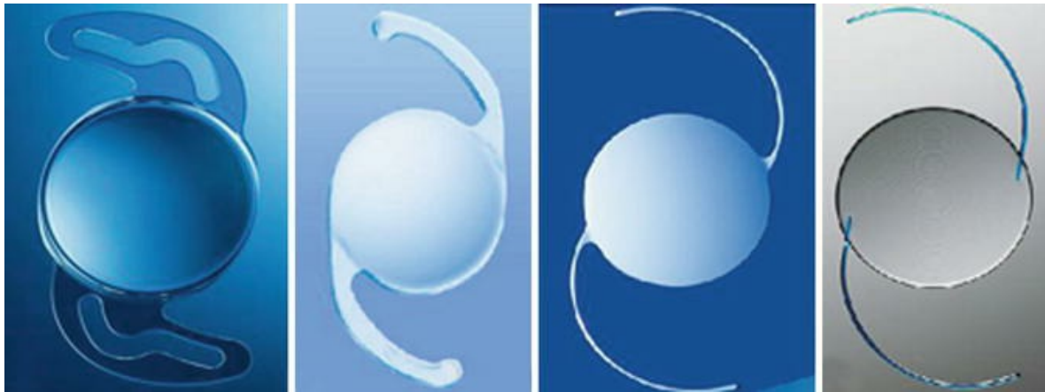
Fig. 14.2 PC-IOLs. (a) Single-piece IOL with anti-vaulting haptics (AVH TM ); (b) single-piece IOL with J-shaped haptics; (c) and (d) three-piece IOL with C-shaped haptics
