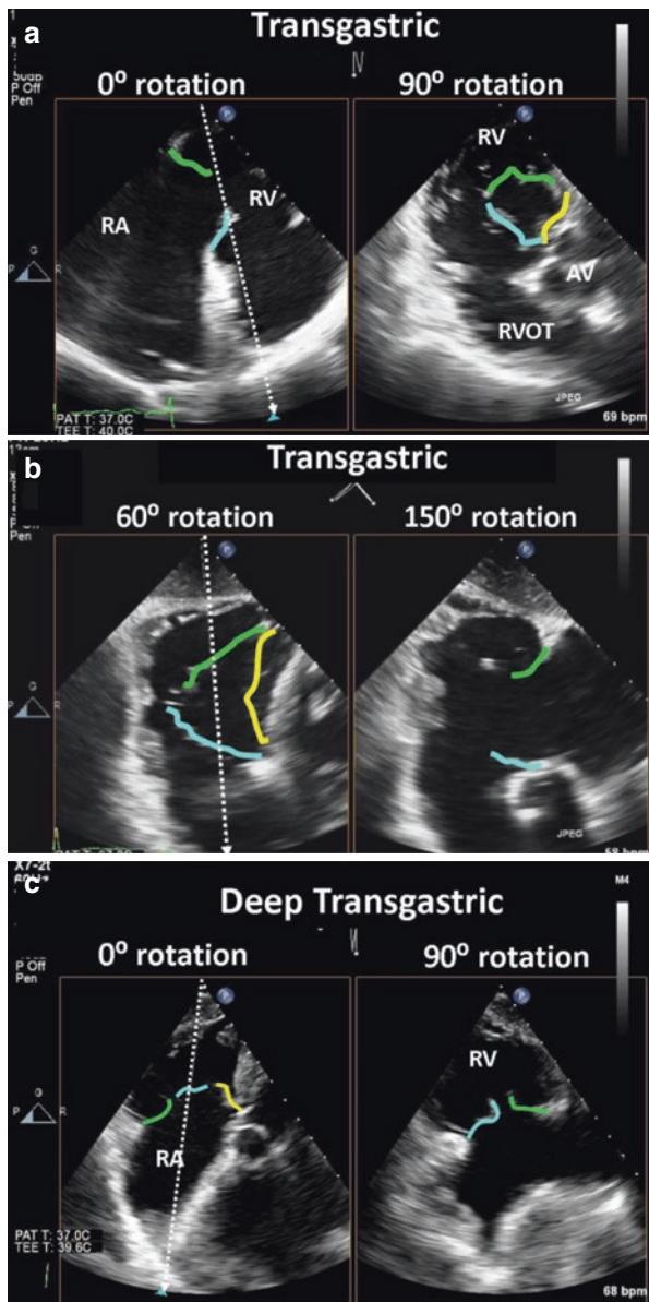
Fig. 6.3 Simultaneous biplane imaging from transgastric views with right and antelexion, the inflow-outflow view of the right heart (panel a) images the anterior (blue line) and posterior leaflet (green line) at 0 degrees. The orthogonal view shows all three tricuspid valve leaflets. This short-axis view of the tricuspid valve can also be imaged between 60 and 90 degrees (panel b) with the simultaneous multiplane imaging plane used to image all three leaflet tips. Deep transgastric views of the tricuspid valve (panel c), may align the insonation beam with the flow across the tricuspid valve for Doppler assessment
