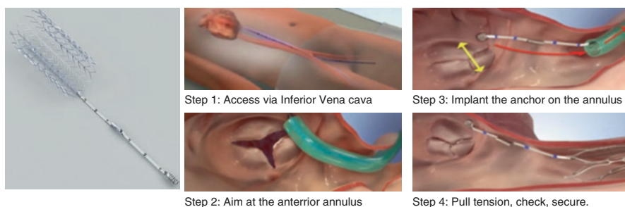
Fig. 15.11 The TriCinch System. The TriCinch System is composed of a corkscrew anchor, a self-expanding stent, and a Dacron band connecting them ( left ). Images show the step-by-step procedure for implantation of the TriCinch System ( right ). Reprinted with permission from Latib et al. [43]
