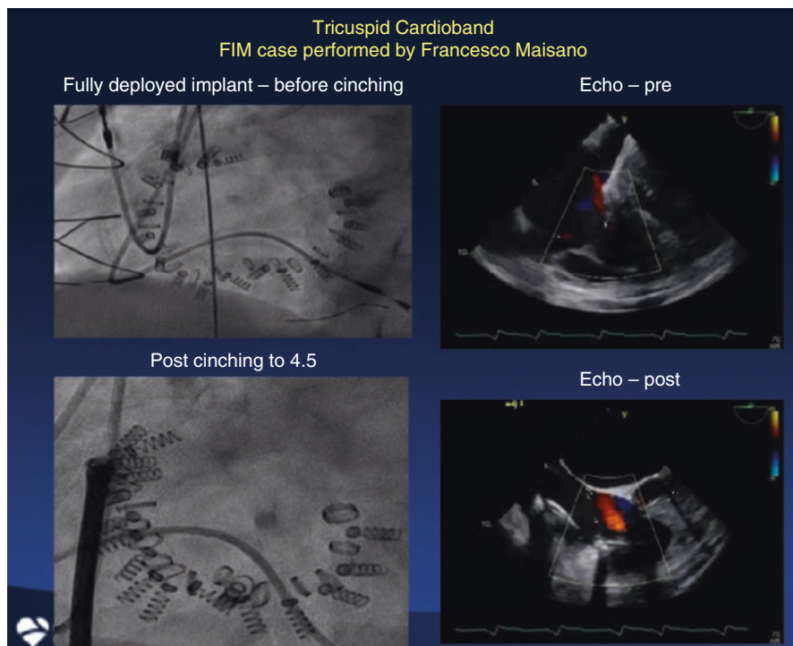
Fig. 15.12 Cardioband
