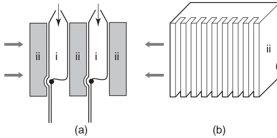
Fig. 6.22 Working diagram of a high-pressure mash filter (Waesburghe, van, 1979, 1989).
