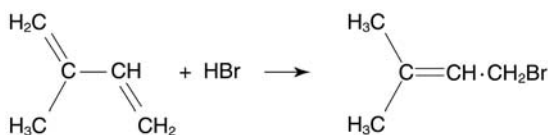
(8.23) isoprene
