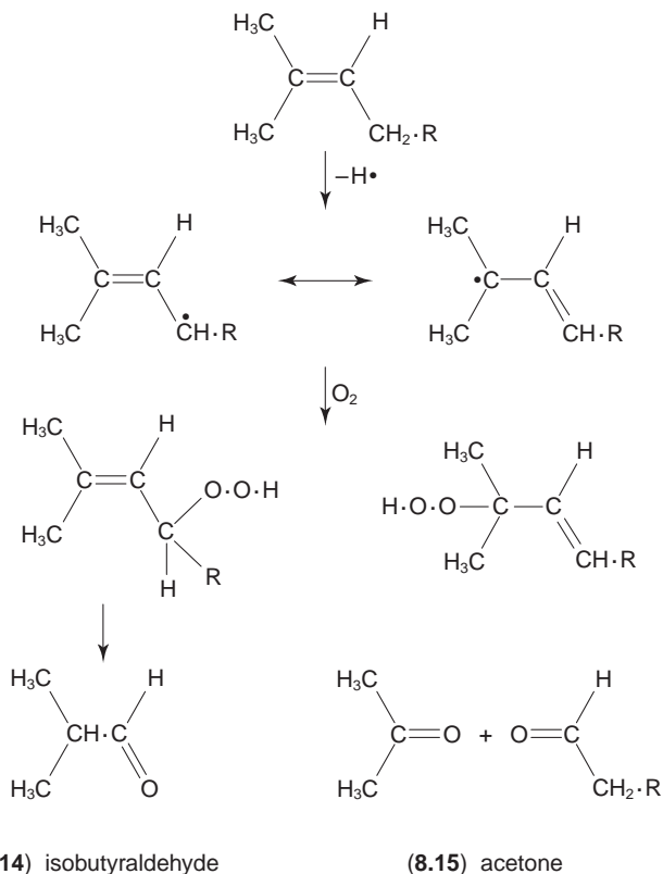
Fig. 8.9 Proposed autoxidation of 3-Methylbut-2-enyl side chains.
