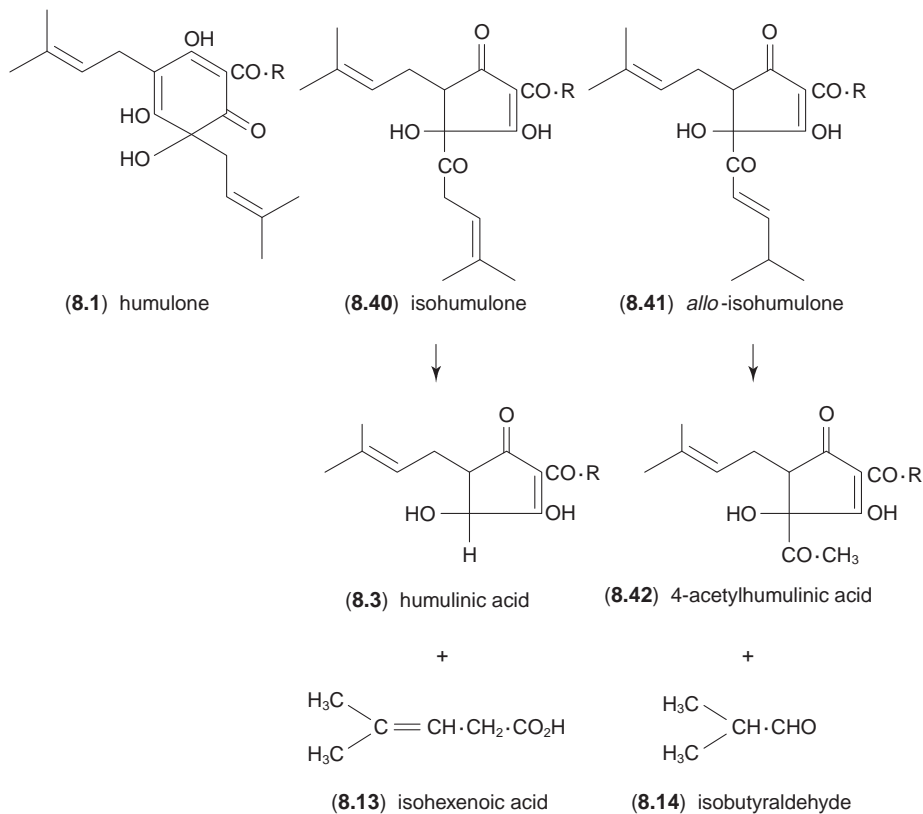
Fig. 8.7 Isomerization and hydrolysis of humulone ( R = \text{Bu}^i without stereochemistry).
