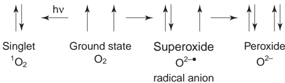
Fig. 20.9 Electronic configurations of various oxygen species (Lacan et al. , 2000).
