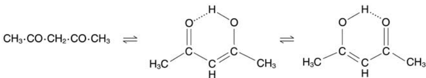
(8.16) acetylacetone
