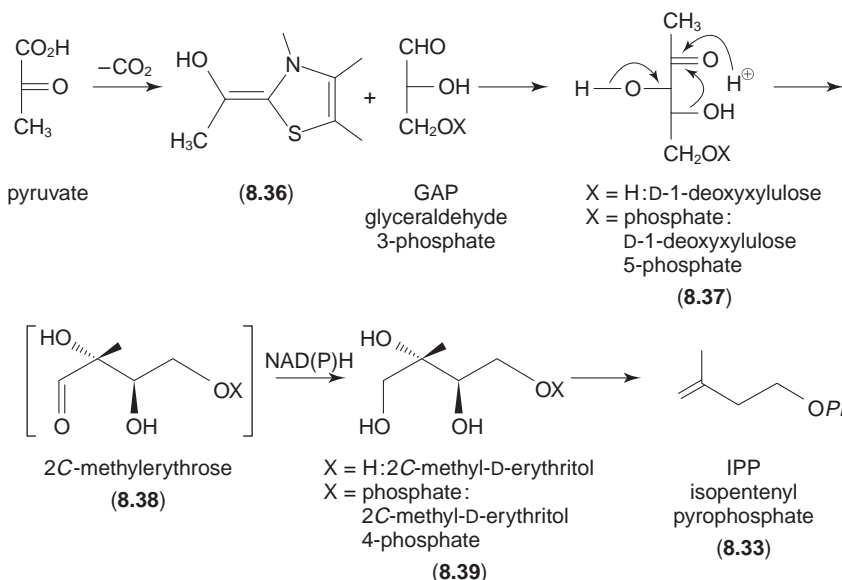
Fig. 8.4 Isoprenoid biosynthesis: (A) via the mevalonate pathway, (B) via the glyceraldehyde 3-phosphate/pyruvate pathway (Rohmer, 1998).
