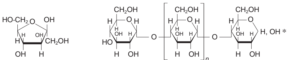
Maltotriose ( n = 1 ); maltotetraose ( n = 2 ); maltopentaose ( n = 3 )
