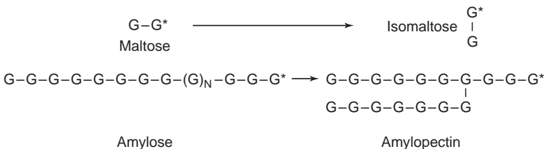
Fig. 4.19 A summary of how the enzymes, that together make up diastase, act on the polysaccharide components of starch or their breakdown products (after Briggs, 1998). G, α-D-glucopyranose residues – , (1,4)-link |; (1,6)-link; *, reducing group.
