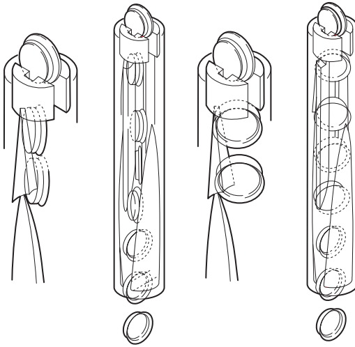
Fig. 21.7 Turning tube for orientating crown corks for bottle closure, incorrectly positioned corks are turned up to 180° to gain the correct orientation for bottle closure (Kunze, 1999).
