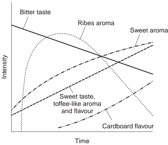
Fig. 20.8 Diagrammatic representation of sensory changes in beer flavour during ageing (Dalglish, 1977).
