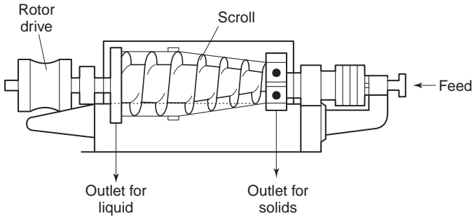
Fig 15.10 Decanter centrifuge (based on drawing received from Alfa-Laval Ltd.).
