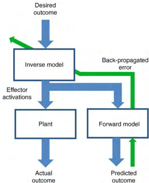
Neural Networks for Control. Figure 6 Distal learning. A network which unites the plant, referred as a forward model, is learned. At the same time, the errors in the plant output are backpropagated through the forward model network to obtain the errors of the inverse model (green arrow). These errors are used to train the network of the inverse model.
