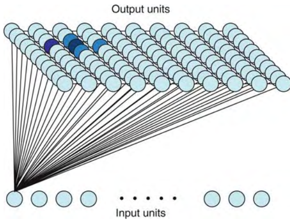
Connectionism. Figure 3 Unsupervised learning: in self-organizing maps, an active unit partly distributes its activation to its neighbors. Eventually clusters of units emerge, representing a topological map of the input.
