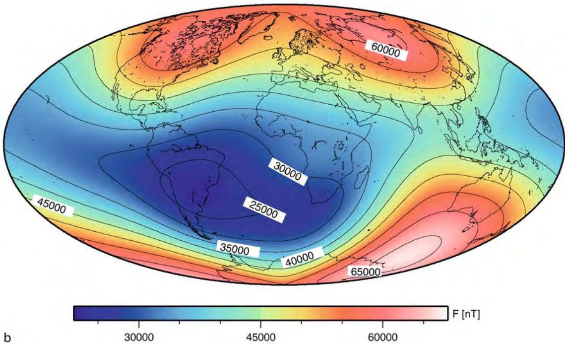
Geomagnetic Field. Figure 4 Total field intensity, F for the years 1900 (a) and 2004 (b) according to IGRF 9, in isodynamic format and equal area projection.
