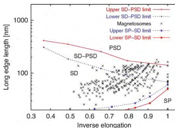
Magnetite. Figure 2 Phase diagram for magnetic domain state in submicron-sized rectangular crystals of magnetite as a function of axial ratio (width/length) and long edge length calculated for room temperature (according to [3,4]). The upper two lines demarcate the stability of single domain (SD) magnetization states against pseudo-single-domain (PSD) states [3], the lower two lines against superparamagnetic behavior [4]. The crosses represent data from edge-length measurements on magnetite particles (magnetosomes) in magnetic bacteria [5]. With a few exceptions, magnetosomes fall into the stable SD field or in the field where SD states coexist with vortex states (SD–PSD field).
