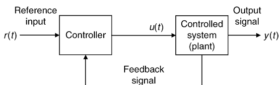
Nonlinear Control Systems. Figure 1 Basic feedback control system.
