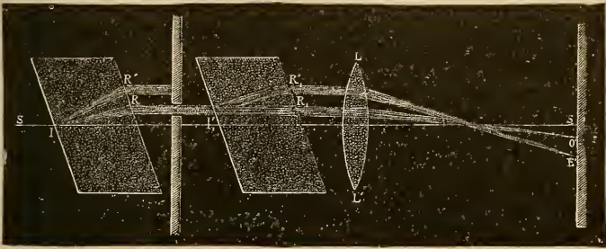
Fig. 179. The Polarizer and Analyzer.
