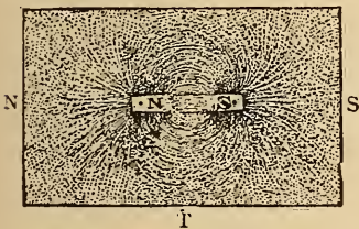
Fig. 143. Magnetic lines as shown by iron filings.
