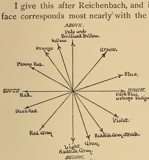
Fig. 185. Odic Colors from the North Pole of a Magnet made to revolve vertically in the Magnetic Meridian.
