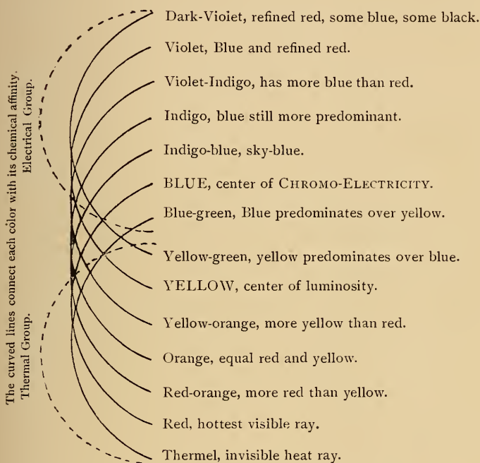
Fig. 131. The Solar Spectrum Systematized.
