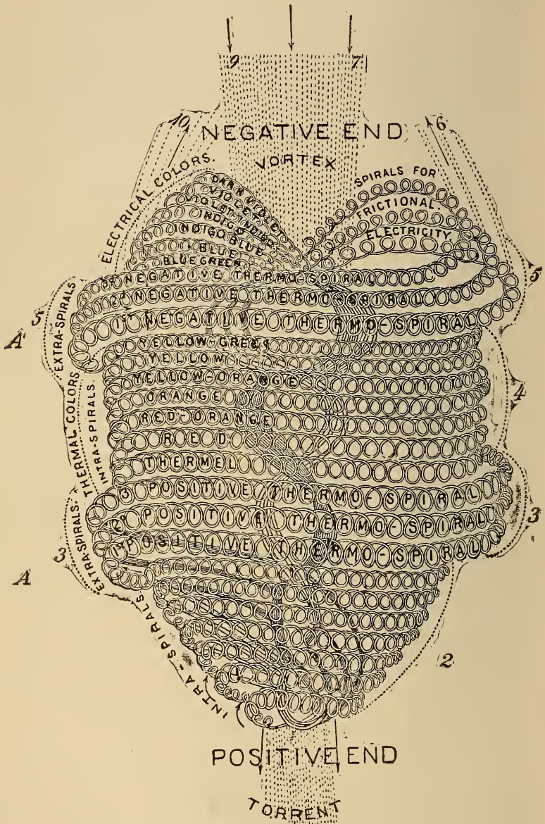
Fig. 135. The general Form of an Atom, including the spirals together with influx and efflux ethers, represented by dots, which pass through these spirals. The spirillæ with their still finer ethers are not shown. The spirals must pass around atoms in the opposite direction in different Substances, which fact will account for what chemists call dextro-rotary, rotating to the right, or levo-rotary, rotating to the left.
