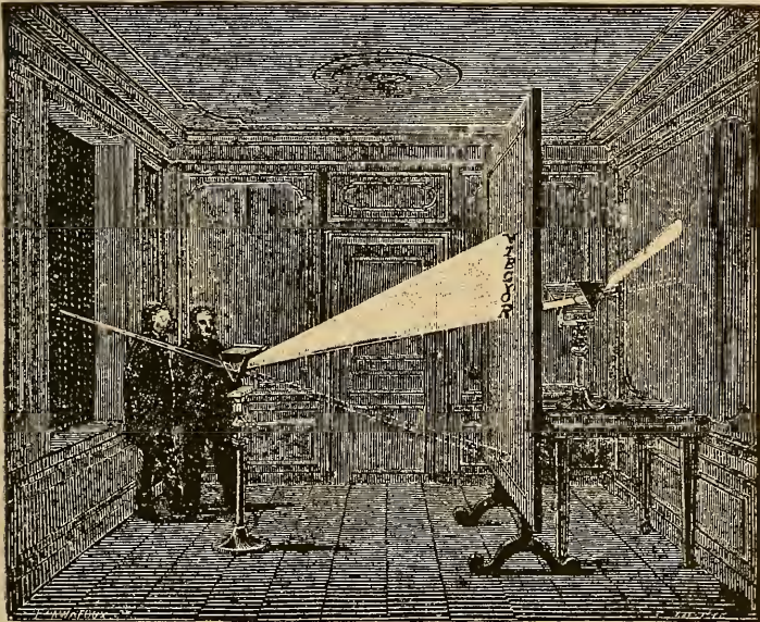
Fig. 120. Decomposition of Light by the Prism.
