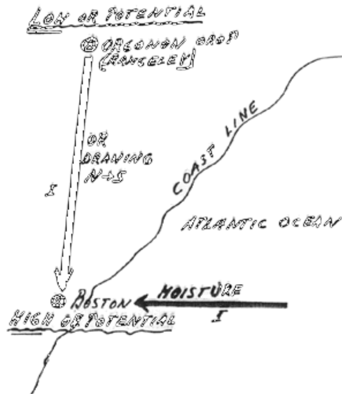
FIGURE 17a. DRAWING MOISTURE FROM OCEAN INTO CONTINENT USING DISTANT HIGH OR POTENTIAL.
