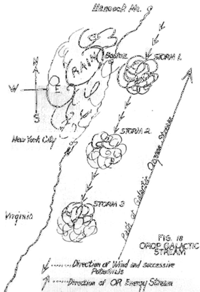
Figure 18: OROP Galactic Stream ~
