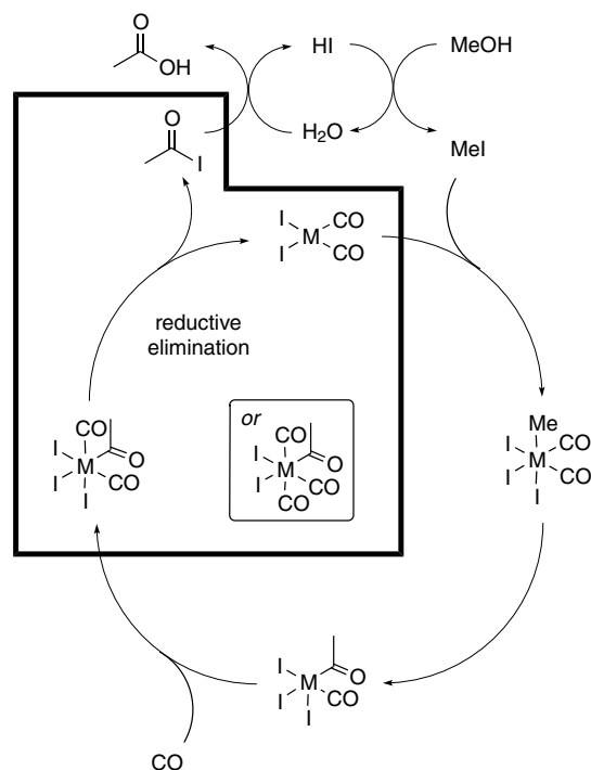
Figure 8.5 Catalytic cycle for the metal-catalyzed carbonylation of methanol, with the reductive elimination step highlighted. In the case of iridium, the diiodotriiodoacetyl species has also been suggested as a possible precursor to reductive elimination. What are the issues of stereochemistry associated with the intermediates? What special basis-set requirements will be involved in modeling this system?
