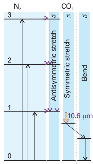
Fig. 14.45 The transitions involved in a carbon dioxide laser. The pumping also depends on the coincidental matching of energy separations; in this case the vibrationally excited \text{N}_2 molecules have excess energies that correspond to a vibrational excitation of the antisymmetric stretch of \text{CO}_2 . The laser transition is from \nu_3 = 1 to \nu_1 = 1 .
