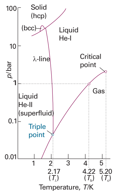
Fig. 4.7 The phase diagram for helium ( ^4\text{He} ). The \lambda -line marks the conditions under which the two liquid phases are in equilibrium. Helium-II is the superfluid phase. Note that a pressure of over 20 bar must be exerted before solid helium can be obtained. The labels hcp and bcc denote different solid phases in which the atoms pack together differently: hcp denotes hexagonal closed packing and bcc denotes body-centred cubic (see Section 20.1 for a description of these structures).
