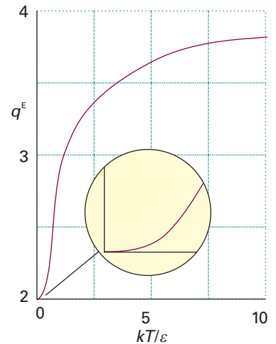
Fig. 17.7 The variation with temperature of the electronic partition function of an NO molecule. Note that the curve resembles that for a two-level system (Fig. 16.5), but rises from 2 (the degeneracy of the lower level) and approaches 4 (the total number of states) at high temperatures.
