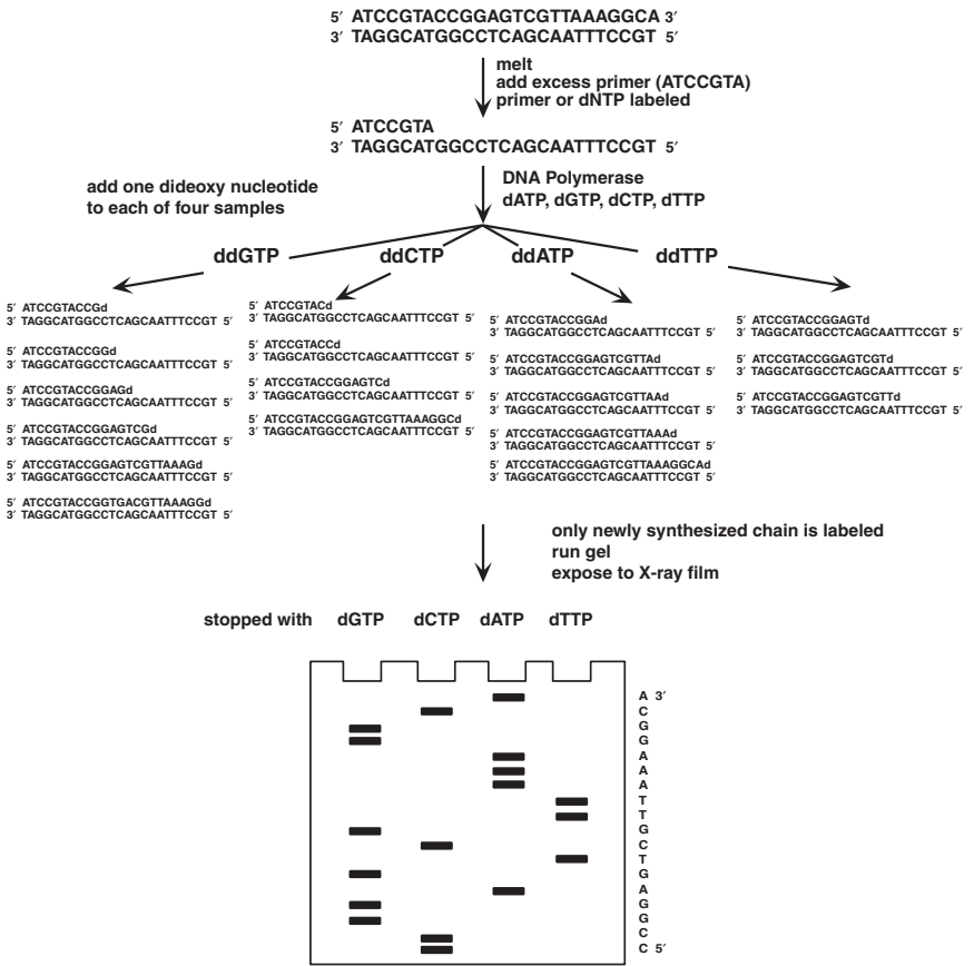
Figure 6-5 DNA Sequencing
