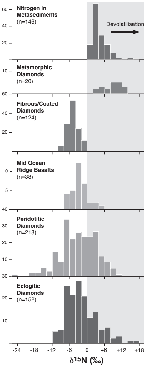
Figure 9. The rationale in using the ^{15}\text{N}/^{14}\text{N} -values in diamonds lies in the distinct distributions displayed by surface and mantle reservoirs. Nitrogen in metasedimentary and metamorphic diamonds, metagabbros and metaophiolites (not shown) being enriched in ^{15}\text{N} compared to the mantle shown here by fibrous/coated diamond, mid-ocean ridge basalts (not shown) and peridotitic diamonds. The similarities of the ^{15}\text{N}/^{14}\text{N} -distributions of eclogitic and peridotitic diamonds must be explained if the source of carbon and nitrogen in eclogitic diamond is to be largely related to subduction (see text for discussion). From Cartigny (2005).
