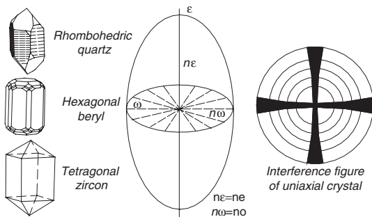
An ellipsoidal sketch of a uniaxial crystal with two different refractive indices, n_o and n_e
