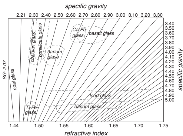
Density and refractive index of imitation glasses used for gemstone. After Bannister 1929
