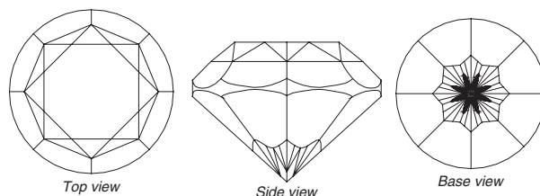
Tolkowsky Zinnia Flower Cut. Courtesy of De Beers
