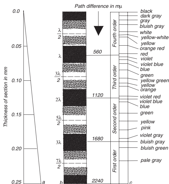
a: cross section of quartz wedge, b: monochromatic light, \lambda = 560 nm and c: colors in four orders of white light
