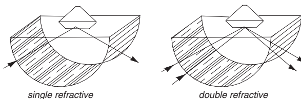
Refractive index reading in a hemisphere by single and double uniaxial crystal
