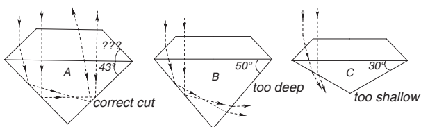
Refraction of light in cut gemstones and its effects. A: showing how correct the angles of cut stone are. B and C showing incorrect angles will result in serious losses of light through the base of the gemstones
