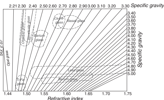
Density and refractive index of imitation glasses used for gemstone. After Bannister, 1929
