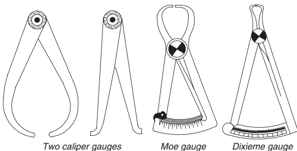
Four different gauges
