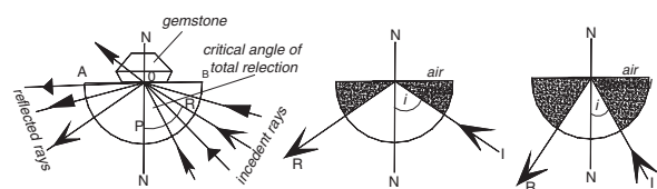
depending on critical angle or total-reflection from refraction of light between gem and hemisphere depending on critical angle from refraction of light, left in glass and right in diamond
