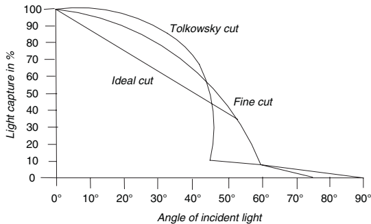
Light captured by brilliant-cut diamond as ideal-cut, fine-cut, and Talkowsky-cut due to incidence light. After Eppler 1973
