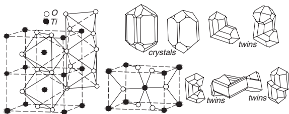
Rutile structure, crystals, and twins
