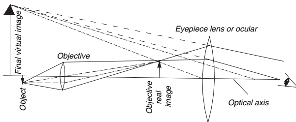
Microscope compound
