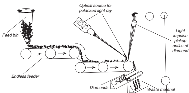
Optical separating and recovery device for diamond
