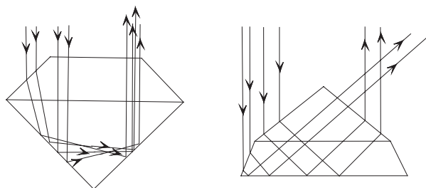
The path of light passing and reflecting back through a correct brilliant-cut and right through a Dutch-cut diamond
