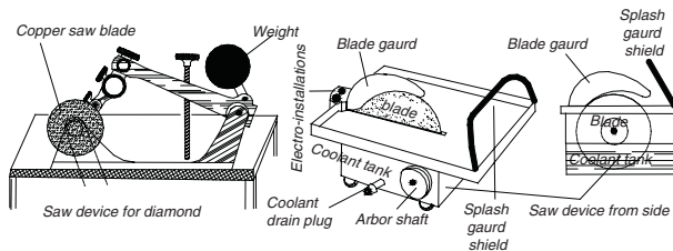
Saw apparatus for diamond and other stones
