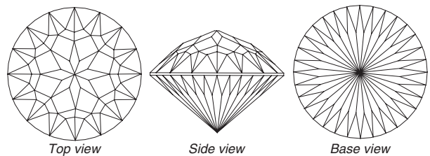
Needle brilliant-cut with 128 facets
