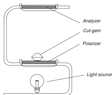
Sketch of polariscope
