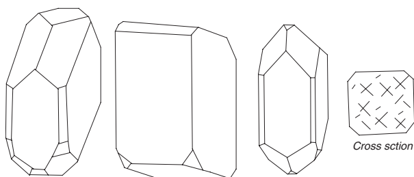
Diopside crystals and right cross section
