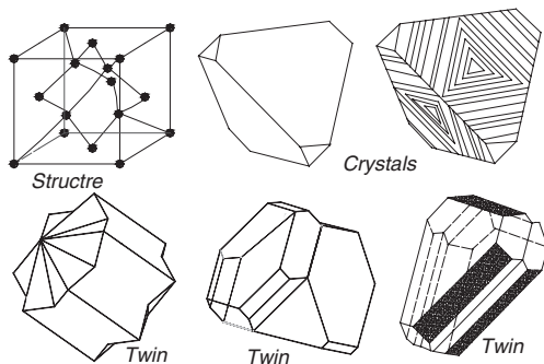
Sphalerite structure, crystals, and twins
