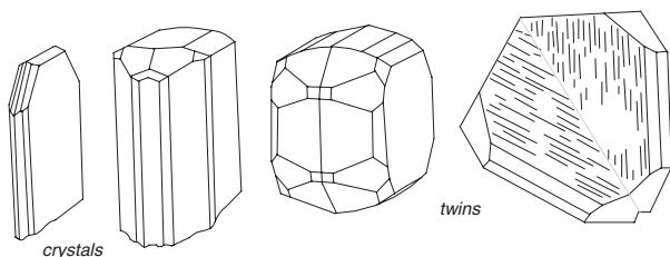
Columbite crystals and twins
