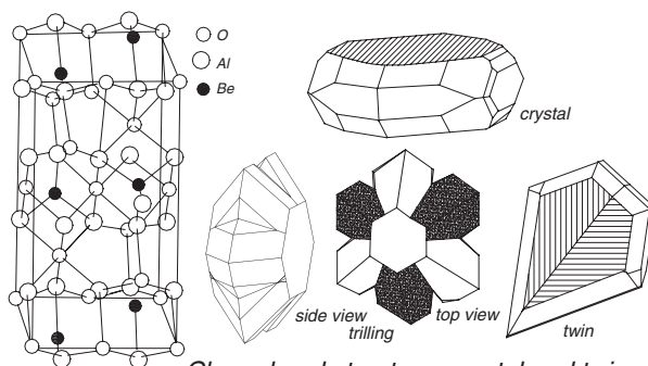
Chrysoberyl structure, crystal and twins
