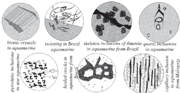
Inclusions in aquamarine from different sources
