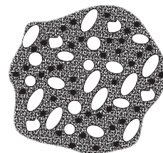
Vesiculars or porous in a rock
