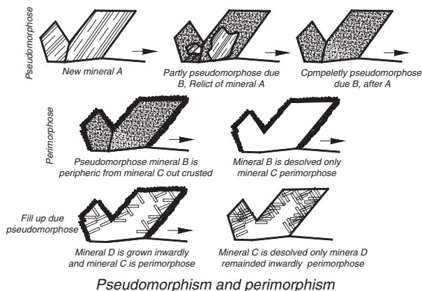
Pseudomorphism and perimorphism
