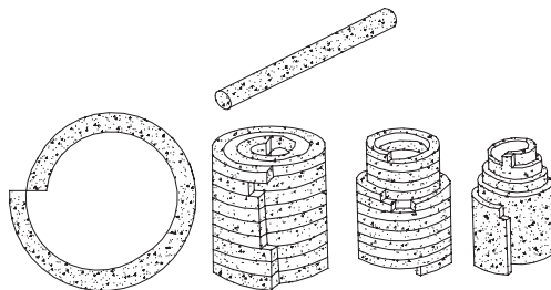
Spiral-cylindrical structure of antigorite.
