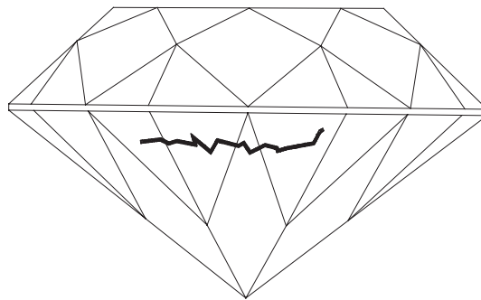
Growth lines seen on a brilliant-cut diamond
