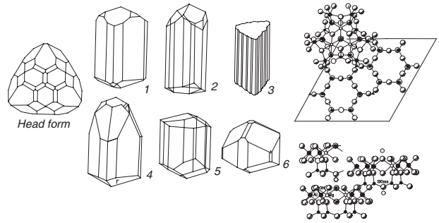
Crystals and structure of tourmaline. 3: striation on tourmaline
