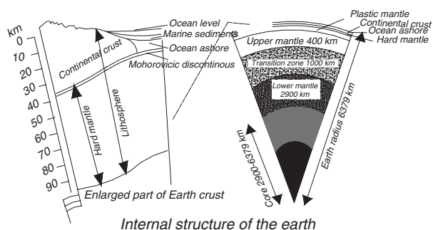
Internal structure of the earth
