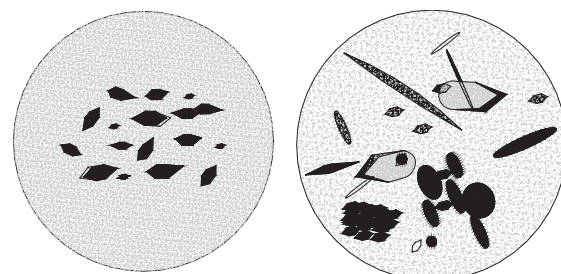
biotite scales in peridot
