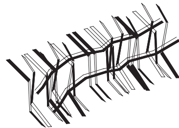
Centipede inclusions due to fissures in Sri Lanka moonstone
