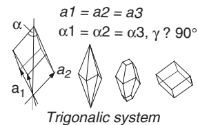
Trigonal system
