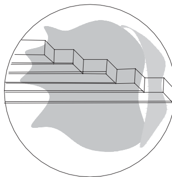
Step form twinning in chrysoberyl
