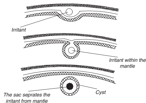
Formation of a cyst pearl
