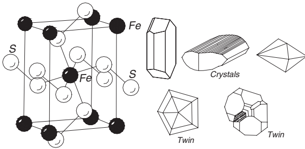
Marcasite structure, crystals, and twins
