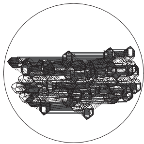
Disordered hornblende in almandine-garnet
