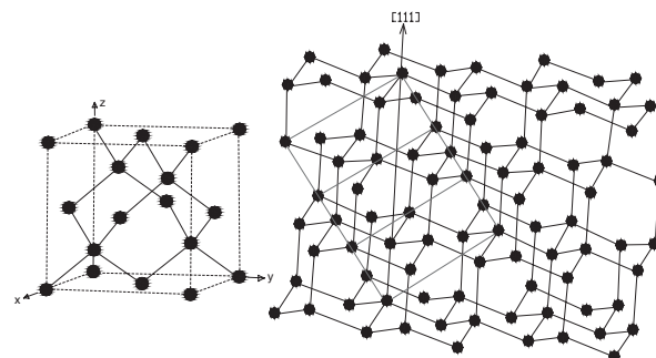
Diamond atomic structure and unit cell
