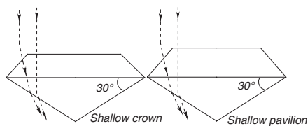
Shallow crown and pavilion
