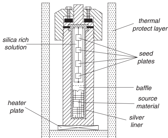
Sketch of a silver-lined autoclave for production of hydrothermal grown quartz. After Webster 1994
