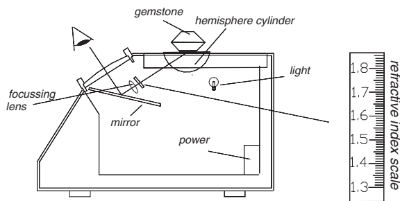
Sketch of a refractometer
