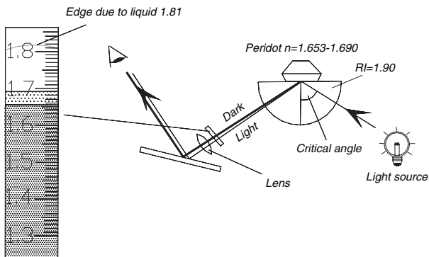
Entering light refractometer and striking a peridot gem
