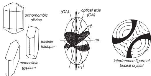
A three axial ellipsoid of a biaxial crystal with three different refractive indices, n_\alpha , n_\beta , and n_\gamma and three different biaxial crystal systems
