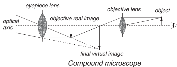
Compound microscope
