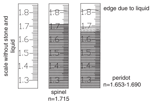
Scale of a refractometer in three condition
