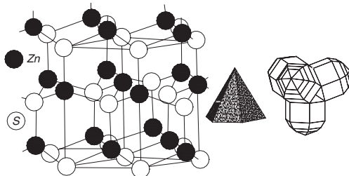
Wurtzite structure, crystal, and twin
