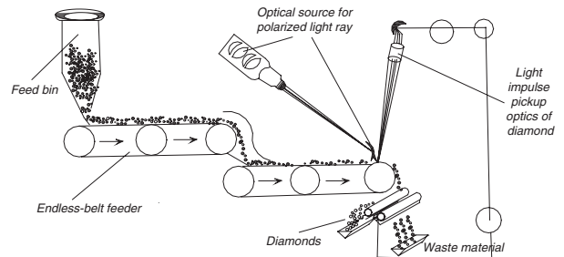
Optical separating and recovery device for diamond
