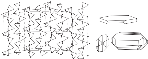
Wollastonite structure and crystals
