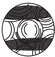
Perlite of obsidian
