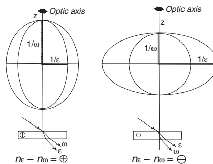
Left: section of the ray-surface of a positive and right a negative uniaxial crystal
