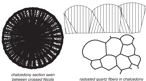
Radyated quartz fibres in chalcedony
