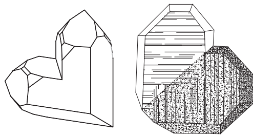
Japanese law twins of quartz
