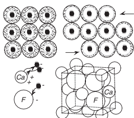
Crystal structure formation
