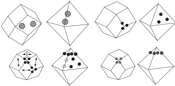
Situation of two, three and four point on octahedron and dodecahedron diamond crystals
