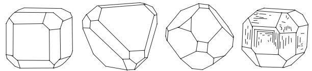
Boracite crystals
