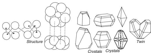
Sulfur structure, crystals, and twin
