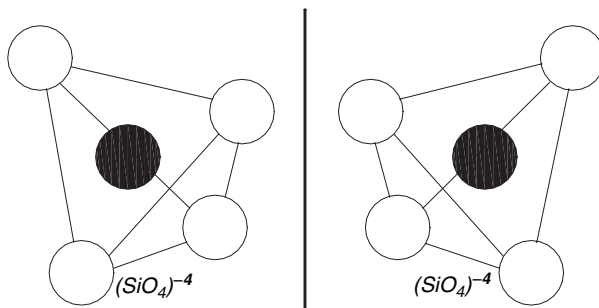
Enantiomorphism in left and right quartz structure
