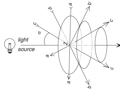
Forming of asterism on surface of a gemstone due to conical reflection of light
