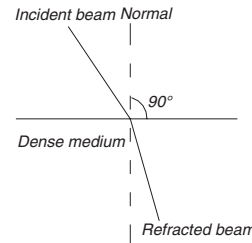
Entering of incident light in a dense medium is refracted toward the normal
