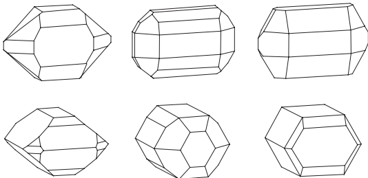
Olivine or peridot crystals
