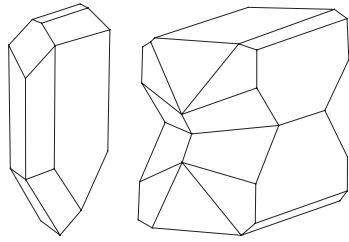
Hemimorphite or calamine crystal and twin
