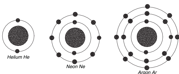
Electronic configuration of inert atoms
