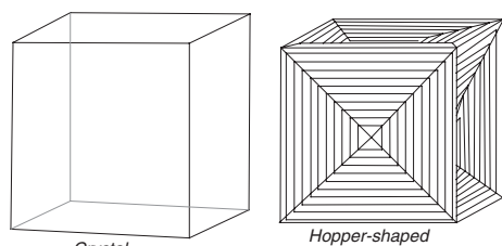
Halite crystal and hopper shaped
