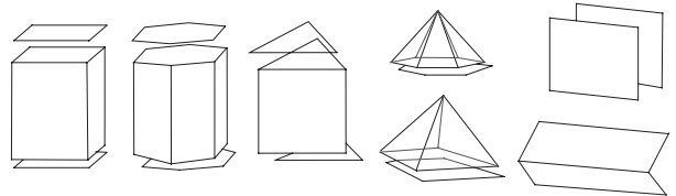
Open form of crystals
