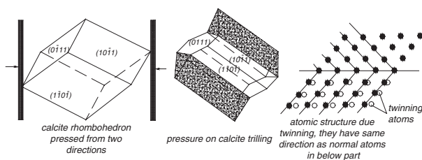
Deformation due to sliding twinning
