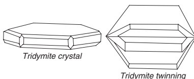
Tridymite crystal and twinning
