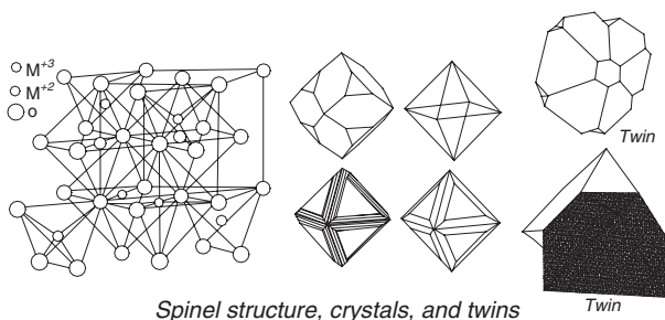
Spinel structure, crystals, and twins
