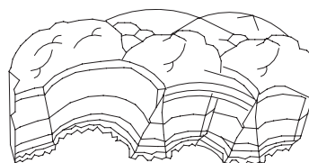
Nephroid aggregate After Sinkankas 1964
