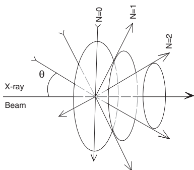
Diffraction cones of X-rays
