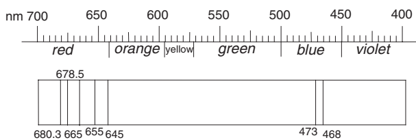
Alexandrite absorption spectrum
