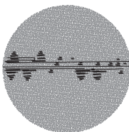
Zircon inclusions parallel to c-axis
