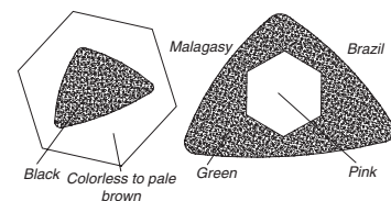
Color zoning of tourmaline. After Dietrich
