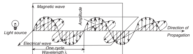
Electromagnetic vibration of light
