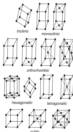
14 Bravais crystal lattices or unit cell.
