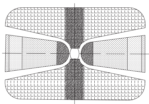
Pressure belt of synthetic diamond
