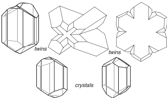
Augite or pyroxene crystals and twins
