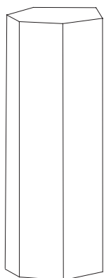
Doubly terminated beryl crystal
