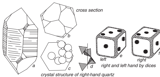
a: right quartz and b: cross section. c and d: structure of right-hand quartz in two types compare with two left and right dices (e and f)
