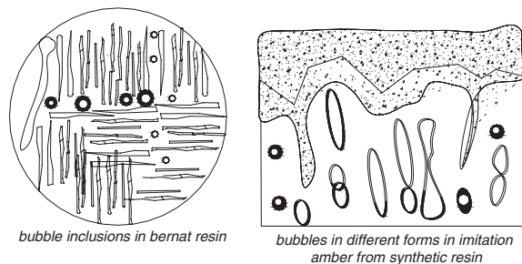
Inclusions in two different imitation ambers
