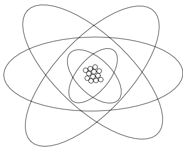
Carbon-12 structure and surrounding negative electrons orbitals the nucleus
