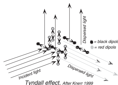
Tyndall effect. After Knerr 1999
