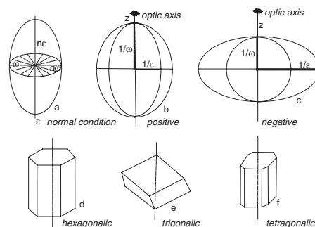
a: an ellipsoidal sketch of an uniaxial crystal with two different refractive indices, n_o and n_e , b: positive condition and c: negative condition with three uniaxial crystal systems d-f
