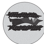
Unmixing double-refractive crystals in scapolite cat's-eye from Malagasy
