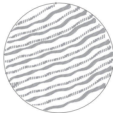
Zebra or tiger stripes in amethyst
