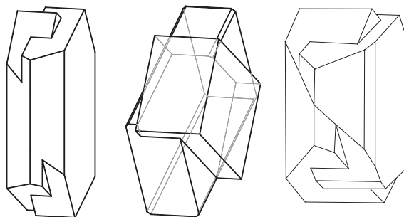
Feldspar Carlsbad twins
