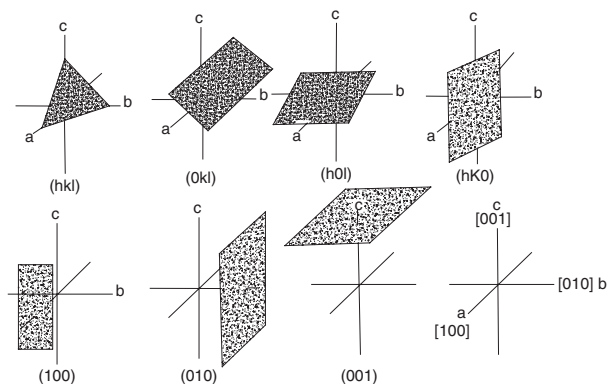
Indices of crystal faces or Miller indices. After Niggli 1941
