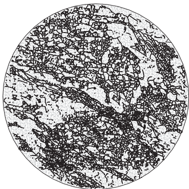
Thin section of nephrite
