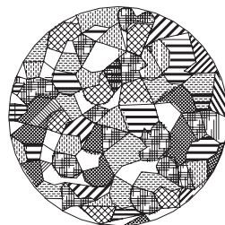
Crystalline marble aggregate under microscope
