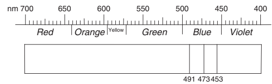
Peridot absorption spectrum
