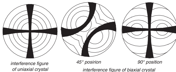
Interference figures
