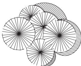
Radiated ball of wavellite
