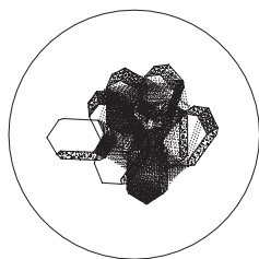
Zircon crystals in kornerupine from Malagasy
