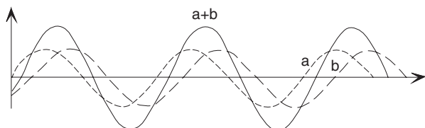
Partially interferes of two different amplitude and phases waves, b with a result wave a+b.
