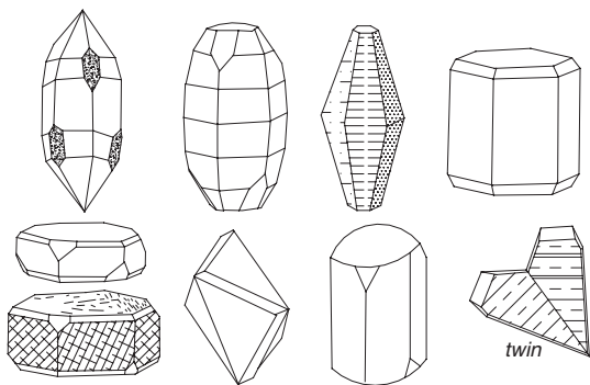
Corundum crystals and twin
