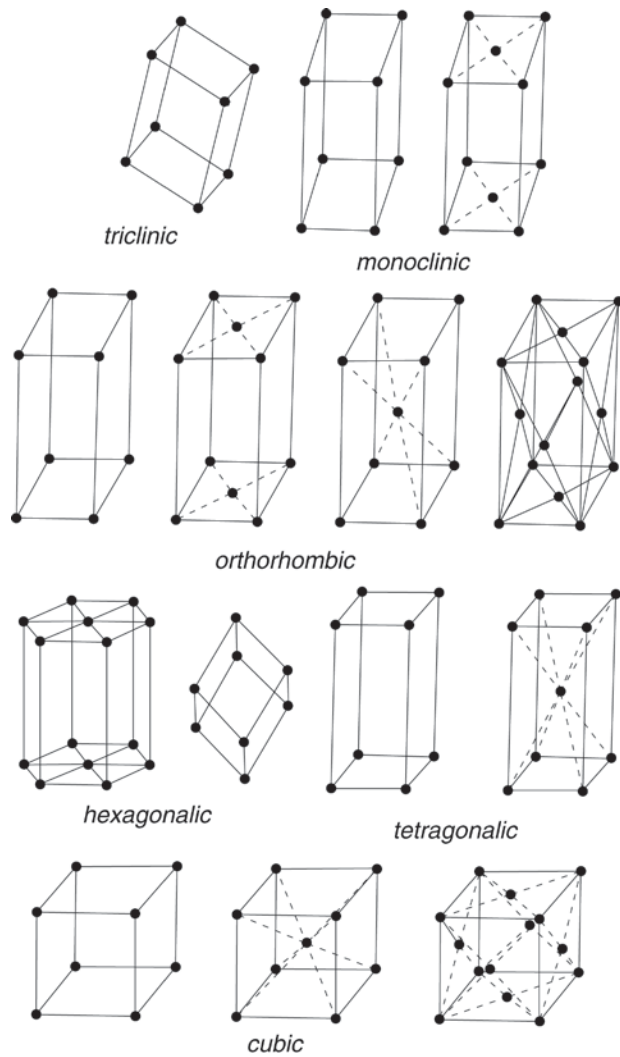
14 Bravais crystal lattices or unit cell
