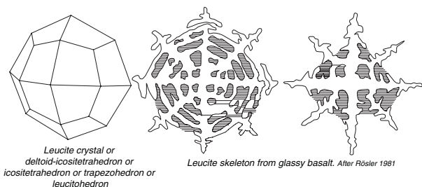
Leucite crystal and two skeleton froms of glassy basalt
