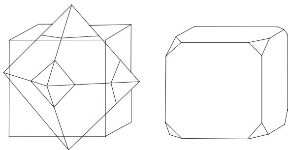
Combination of octahedron and hexahedron
