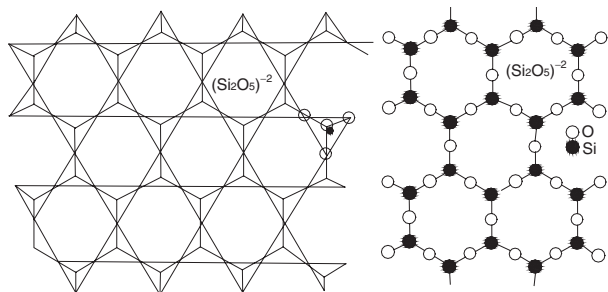
Phyllosilicate structure, hexagonals are tetrahedron of (\text{Si}_2\text{O}_5)^{-2}
