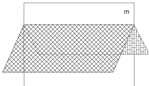
Dome or dihedron
