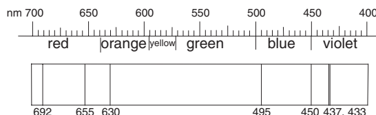
Jade absorption spectrum
