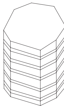
Parting in enstatite on the basal pinacoid
