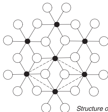
Structure of brucite
