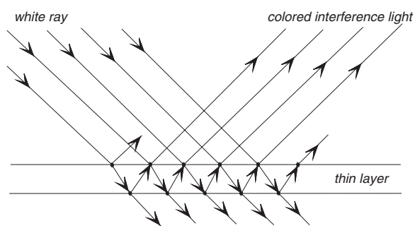
Incidence light, reflection, refraction, and interference
