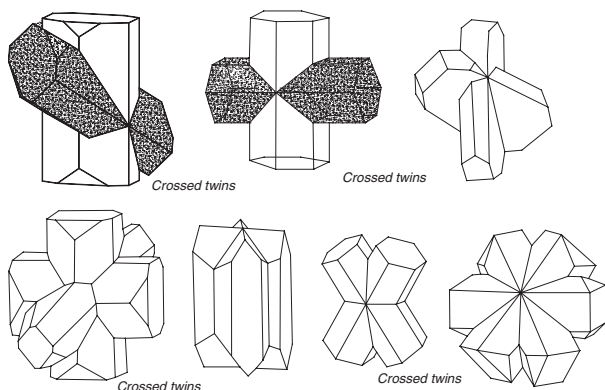
Twins of staurolite
