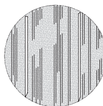
Parallel crystal needles in scapolite cat's-eye
