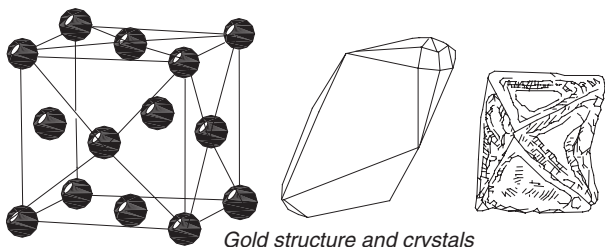
Gold structure and crystals
