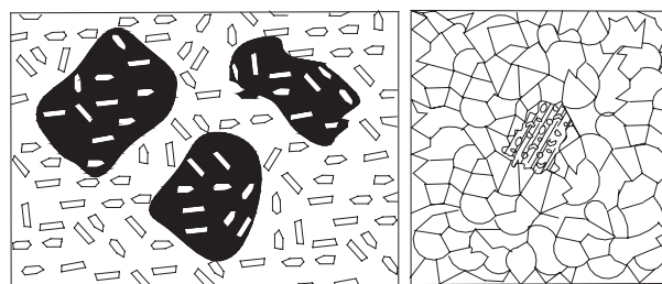
Poikiloblast structure of a xenolithic inclusion
