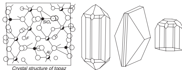
Crystal structure and topaz crystals
