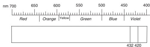
Turquoise absorption spectrum
