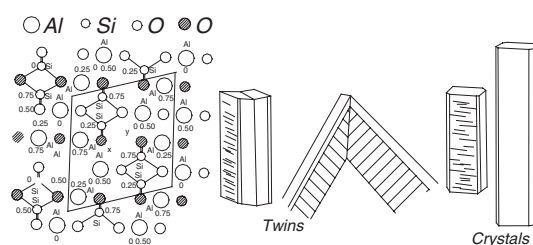
Kyanite structure, crystals, and twins
