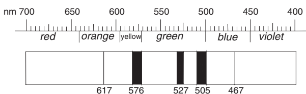
Almandine absorption spectrum
