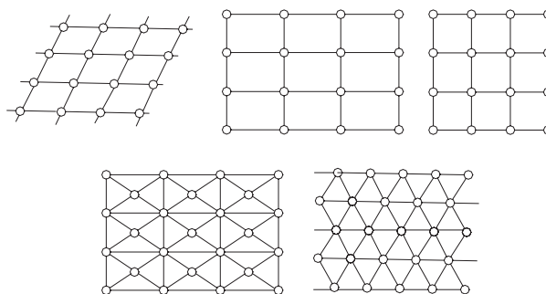
Two-dimensional lattices
