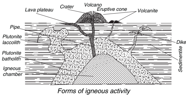
Forms of igneous activity
