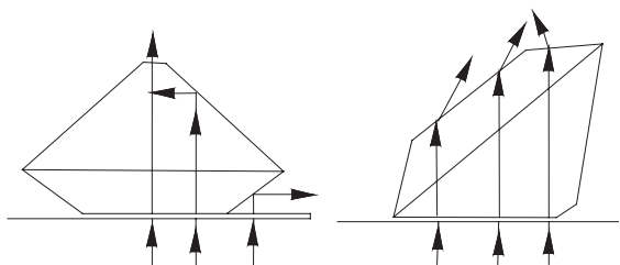
Refraction and defraction of light in cut gems
