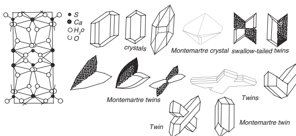
Gypsum structure, crystals, and twins
