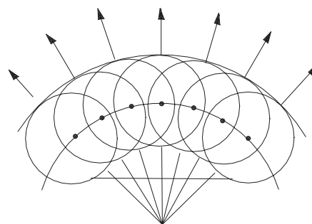
Huygens' principle of light propagation. After Nassau 1983
