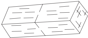
Mesolite crystal
