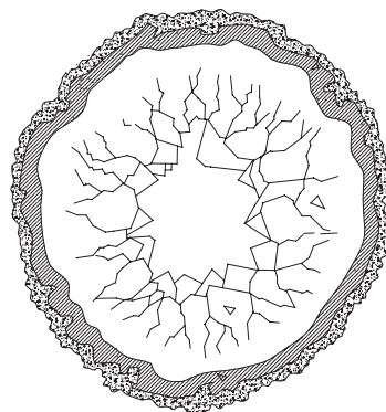
Amethyst geod surrounded by chalcedony rings.
