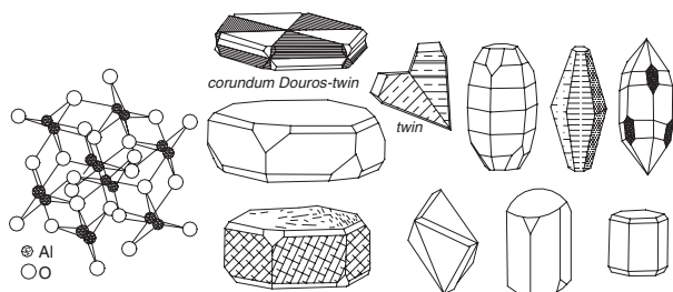
Corundum structure, crystals and twins
