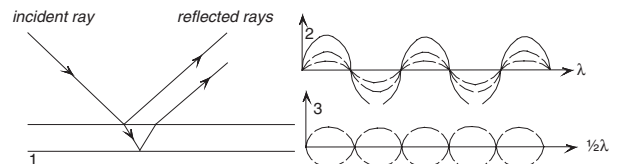
Color caused in a thin layer (1), due to mutual interference between reflected rays by one wavelength ( \lambda ) phase (2), and by 1/2 wavelength ( 1/2\lambda ) phase of rays occurs color cancellation (3)
