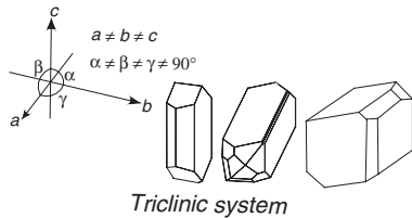
Triglinic system
