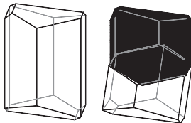
Pericline crystal and twin
