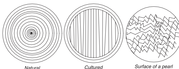
Cross section of a natural, cultured pearl and their surface
