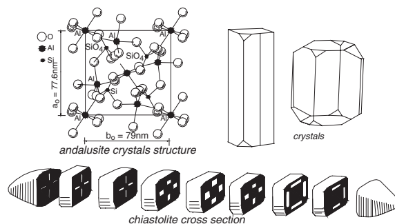
Structure, crystals and chiasolite cross section of analusite
