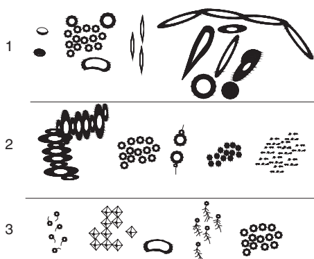
Different typical bubbles in glass (1), synthetic corundum (2), and synthetic spinel (3). After Anderson 1974
