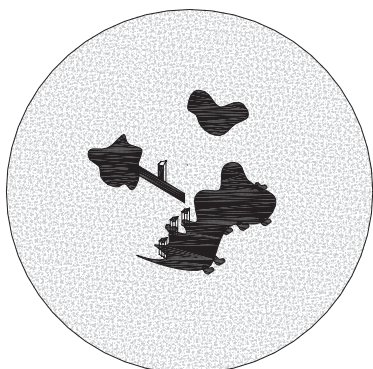
Ilmenite crystals in euclase from Minas Gerais, Brazil
