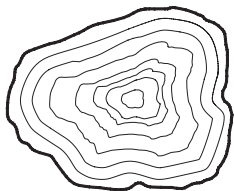
Topographic agate
