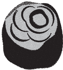
Onion shell boulder
