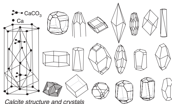
Calcite structure and crystals
