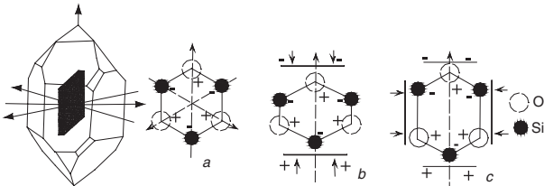
Diagrammatic piezoelectric effect of quartz with heteropolar Si-O. a: normal position. b: pressure parallel to the polar axis. c: pressure in polar axis direction.
