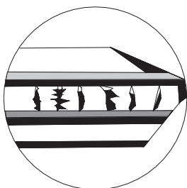
Sandwiched synthetic emerald under microscope
