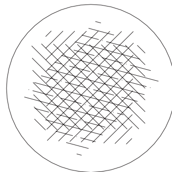
Net formation of rutile needles at 60^\circ in ruby or sapphire
