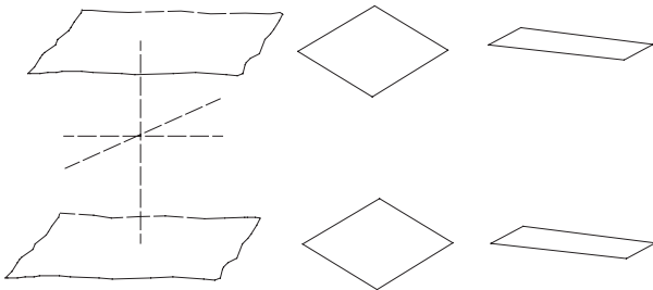
Different pattern of pinacoid or parallelepiped
