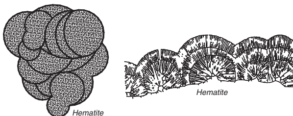
Mammillary aggregate of hematite or malachite
