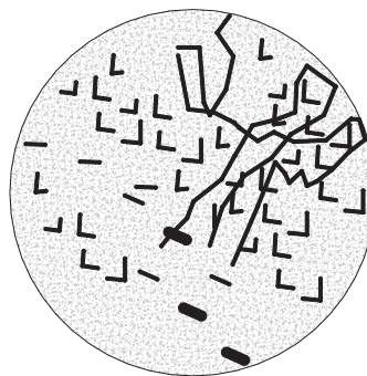
Healed cracks in blue zoisite
