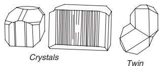
Wolframite crystals and twin
