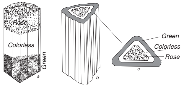
a : zoning tourmaline crystal. b: striation and zoning tourmaline. c: cross section of sample b
