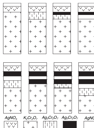
Rhythmic sedimentation. After Cuchrov
