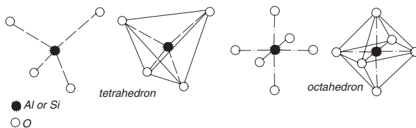
Comorphism of aluminium
