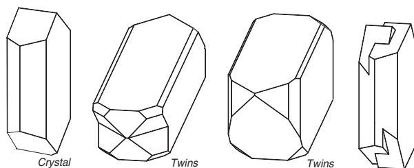
Orthoclase crystal and twins
