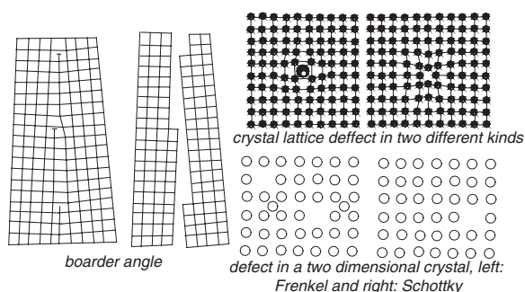
Different kinds of crystal defect
