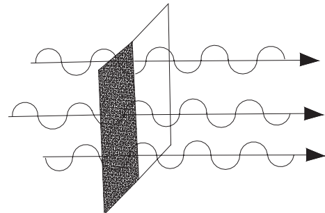
Light wave and absorption
