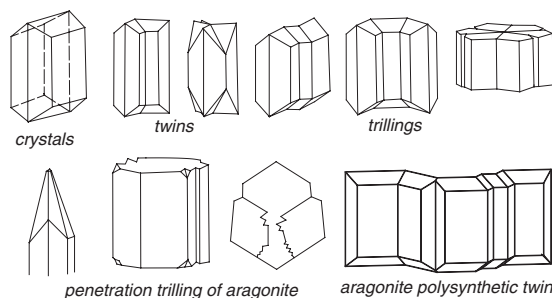
Aragonite crystals, twins, trillings, and polysynthetic twinning
