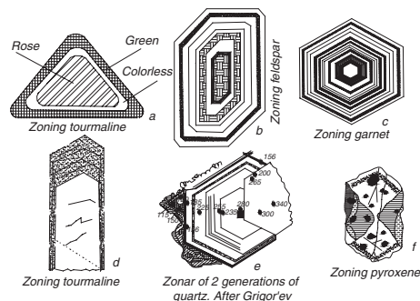
Cross section of zoning crystals. a: tourmaline b: feldspar c: garnet. d: tourmaline. e: quartz and f: pyroxene
