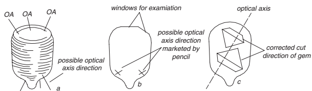
Corrected cut direction of ruby gem. a: a synthetic boule of ruby, b: polishing windows for examination of correct optical axis direction and c: correct direction for cutting gems
