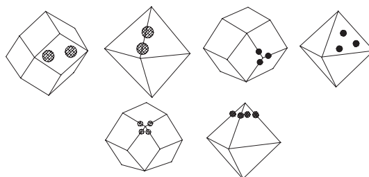
Situation of two, three, and four points, on octahedron and dodecahedron diamond crystals
