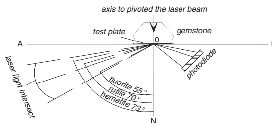
RI measurement of gemstones by using of Brewster angle of polarization. Laser light is vertically polarized therefore Brewster angle the reflected beam incident on the photodiode drops to a minimum
