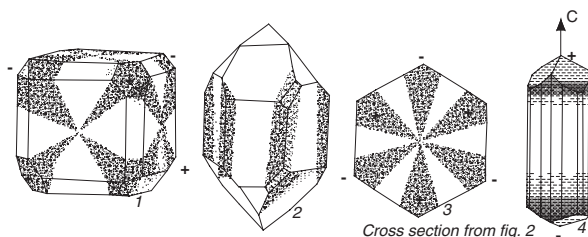
Pyroelectricity of different crystals, 1:boracite, 2-3:quartz, and 4:tourmaline
