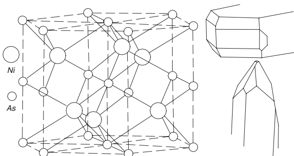
Niccolite structure and crystals
