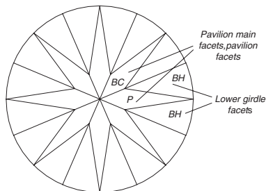
Base view of a round brilliant-cut diamond
