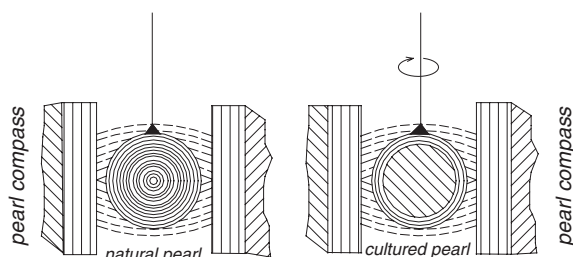
Natural and cultured pearl in a magnetic pearl compass. Cultured pearl in a magnetic field moves
