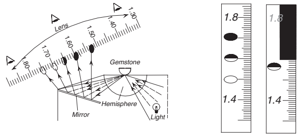
Distant or spot-method RI measuring of a cabochon, half filled bubble is the critical angle
