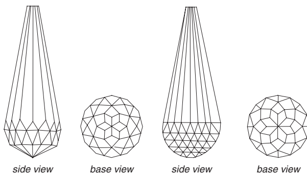
Briolette cuts with two different bases
