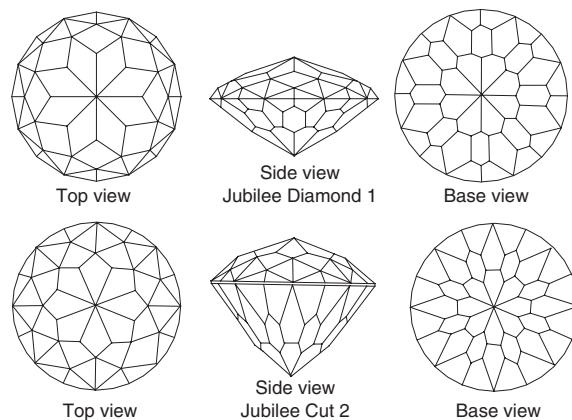
Jubilee Diamond Cuts
