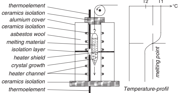
Bridgman-stockbarger method. After Strübel 1977
