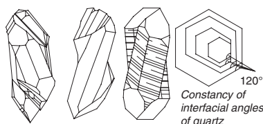
Twisted or distorted quartz
