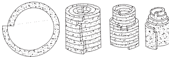
Spiral-cylindrical concentric layers structure of chrysotile and cross section. After Grimm 1962, 1968
