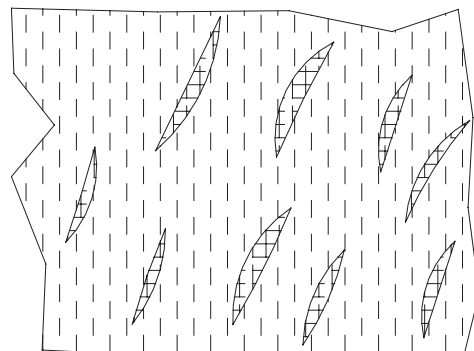
Antiperthite of orthoclase in albite
