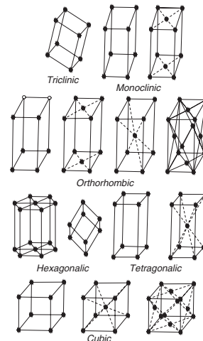
Unit cell or 14 Bravais crystal lattices
