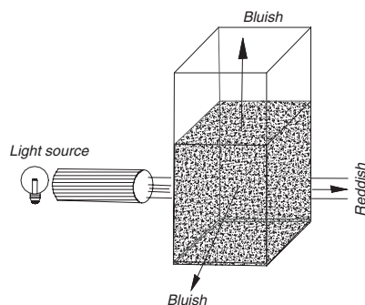
Scattering of light passing through diluted milk
