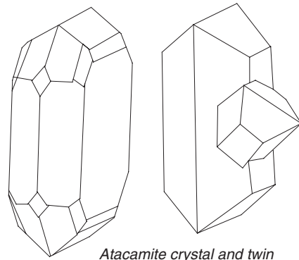
Atacamite crystal and twin
