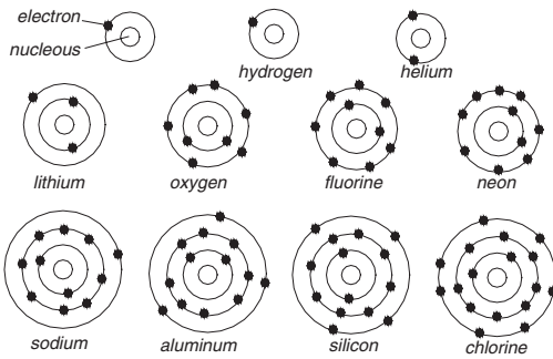
Configuration of atoms. Nucleus: positively charged protons surrounded by negatively charged orbital electrons
