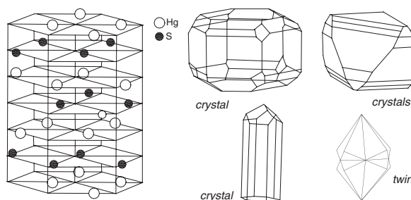
Cinnaber structure, crystals and twin
