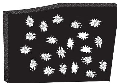
Snowflakes on obsidian
