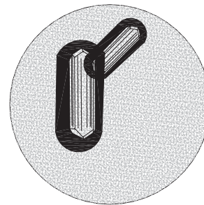
Olivine crystals in blue diamond. ca. 2000x
