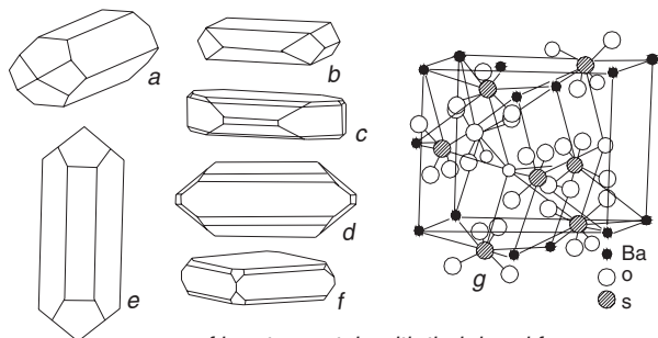
a–f baryte crystals with their head form (e) and (g): crystal structure
