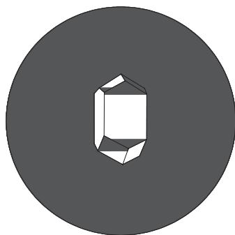
A typical negative crystal in Sri Lanka sapphire
