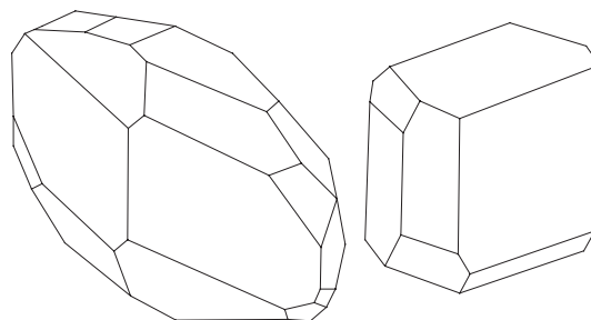
Allanite or orthite crystals
