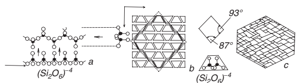
a: pyroxene chain, b: formation of cleavage, and c: section through crystal with its cleavage
