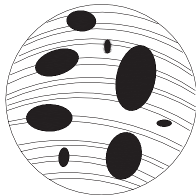
A typical gas-bubbles in a synthetic ruby
