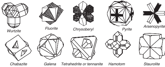
Different kind of interpenetration twinning crystals
