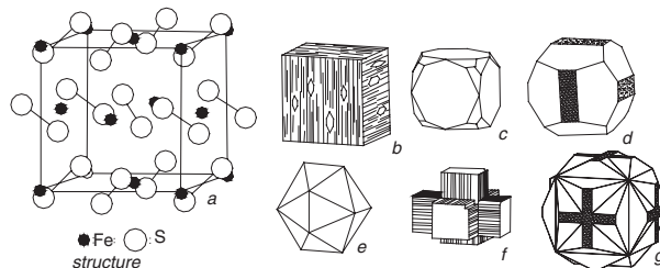
a: pyrite crystal structure, b-e: crystals, f and g: pyrite twins, and g so-called iron cross
