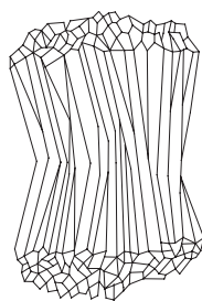
Sheaflike aggregate of stilbite
