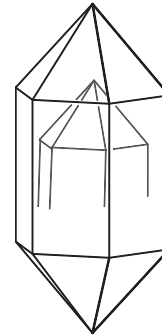
Quartz phantom crystal
