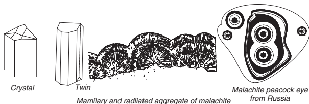
Malachite crystal, twin, mammillary aggregate, and peacock eye
