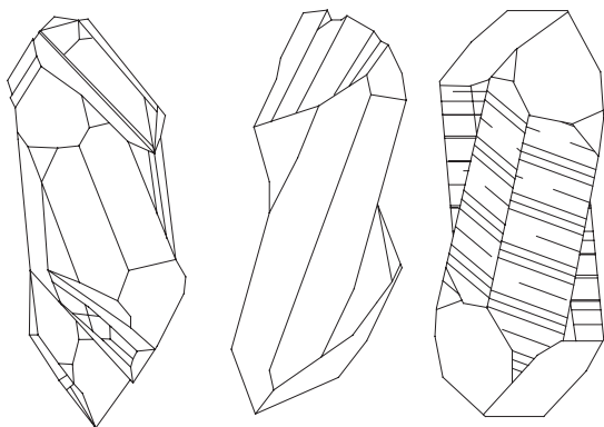
Deformed or twisted quartz
