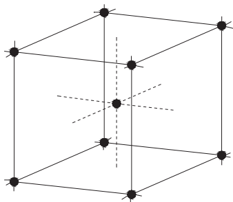
Body-centred cubic crystal
