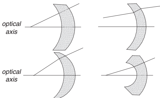
Four different aplanatic lenses
