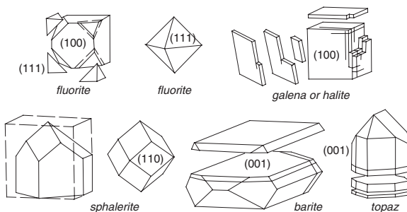
Cleavage direction of different crystals
