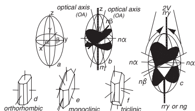
A three axial ellipsoid of a biaxial crystal with three different refractive indices, n\alpha, n\beta and n\gamma . Two circular section are perpendicular to each other, b shows positive condition and c negative condition and d-f three different biaxial crystal systems
