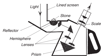
Tully refractometer
