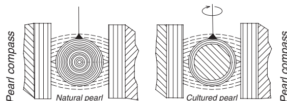
Susceptibility action of natural and cultured pearl in a magnetic pearl compass. Natural pearl has no turning. Cultured pearl layers tend to orient themselves in line with the magnetic field therefore pearl moves
