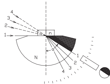
Hemisphere with different incident light and total reflection
