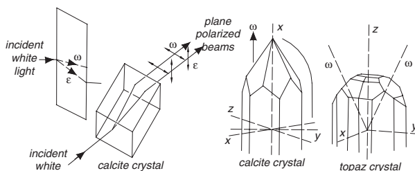
Birefringence in minerals
