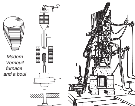
Verneuil furnace draw from Verneuil himself. Redraw from author
