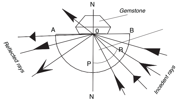
Depending of critical angle or total reflection from refraction of light between gem and glass sphere
