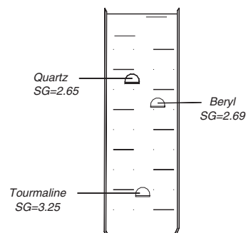
Diffusion column of heavy liquid, methylene iodide, and benzol
