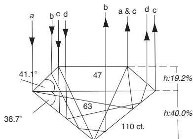
Brilliance and paths of light passing and reflecting back through ideal brilliant-cut diamond
