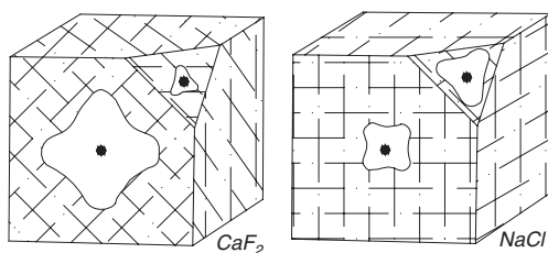
Scratch hardness curves on the cubic and octahedron crystal surfaces
