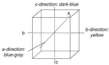
Trichroism of cordierite an optic biaxial crystal
