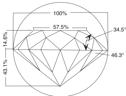
Proportion of facets and their angles on a standard Scan DN brilliant cut. The angles are related to girdle diameter
