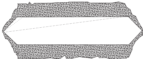
Cross-section of Linde-Lechleitner synthetic emerald overgrowth on a thin seed of colorless beryl. After Sinkankas 1981
