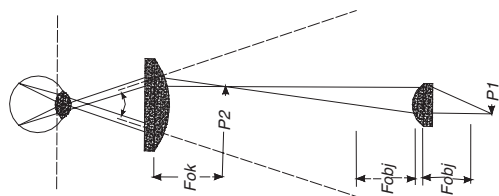
Orthoscope passing light
