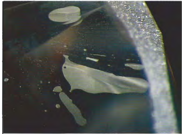
Figure 14. Large trapped gas bubbles such as those shown here probably result from the incomplete filling of the fracture in this diamond. Magnified 35 \times .
