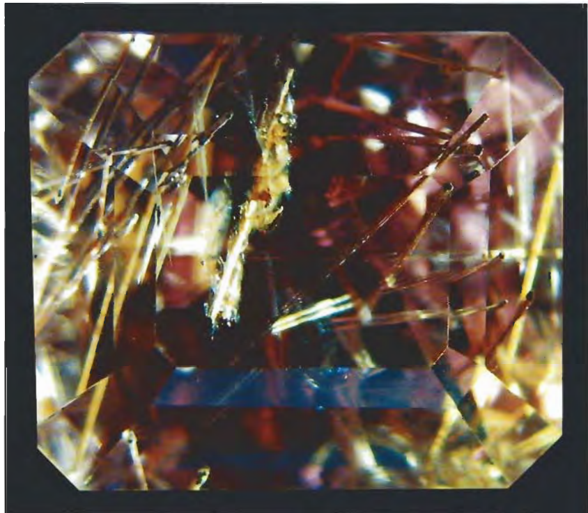
Figure 15. These inclusions in a zircon from Orissa, India, appear to be intermixed rutile-hematite. Darkfield and oblique illumination; magnified 3.5 \times .
