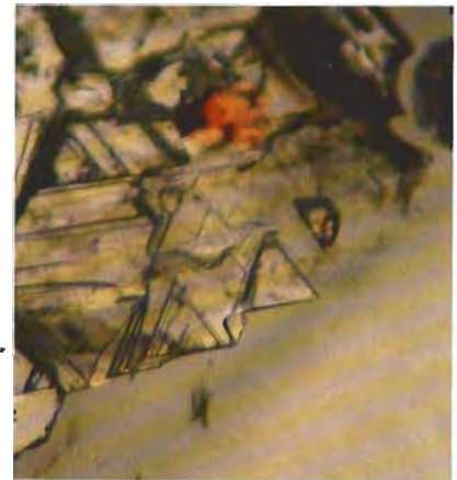
Figure 7. Brown irradiation stains, as seen here in the larger diamond in figure 6, were present in both stones. Note also the irregular green color zoning. Magnified 60×.
