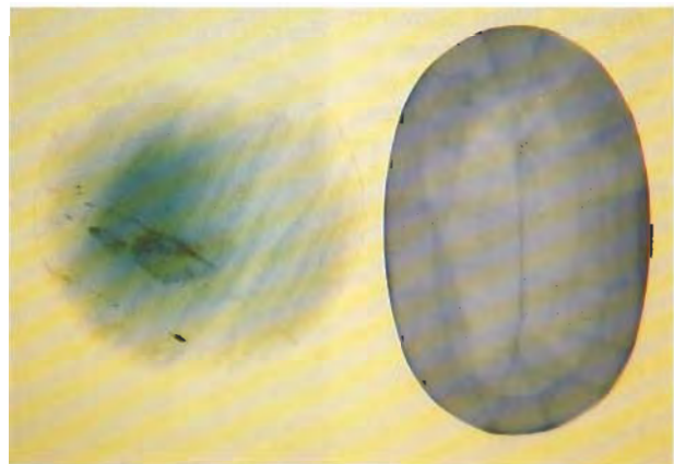
Figure 7. Immersion in methylene iodide reveals the high relief characteristic of a diffusion-treated sapphire (right), as exemplified by a blue outlining of facet junctions and the girdle edge. The heat-treated blue sapphire (left) does not show any outline facet junctions except near the girdle where some areas are slightly abraded. Photomicrograph by Robert E. Kane; magnified 10 \times .
