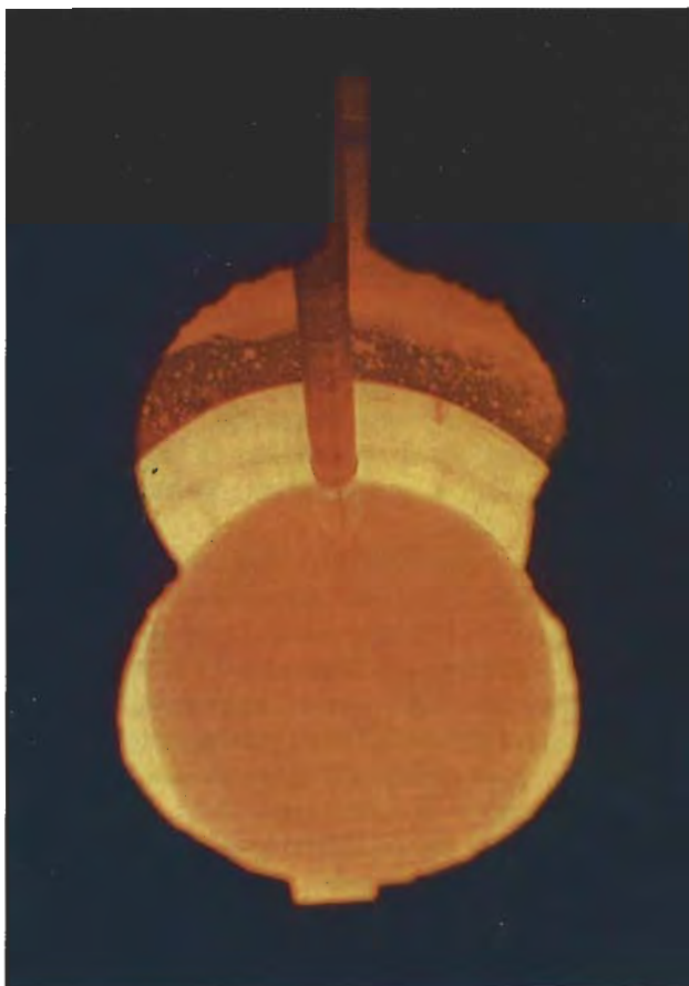
Figure 1. Significant advances in the technology of Czochralski pulling led to the increased production of Czochralski-pulled gem-quality synthetic alexandrite during the 1980s. In the Czochralski-pulling melt growth process, a furnace such as the one illustrated at left is used to grow synthetic alexandrite similar to that produced by Kyocera Corp., shown here to the right of its natural counterpart from Tanzania. Natural alexandrite (top spectrum) can be separated from its synthetic counterpart (bottom spectrum) using infrared spectroscopy, which was applied much more broadly in gemology during the 1980s. Furnace photo courtesy of Union Carbide; stone photo by Robert Weldon.
