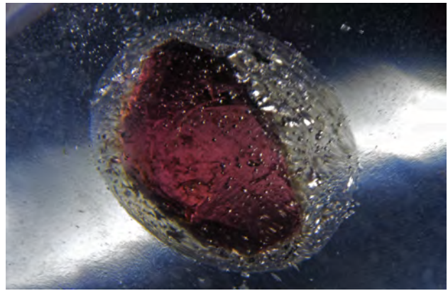
Figure 10. Gas bubbles can be seen in an otherwise nearly invisible glue layer between the quartz cabochons; these bubbles are abundant in the vicinity of the red garnet fragment. The fragment resides in a hollowed-out pocket and is surrounded with glue. Photomicrograph by Nathan Renfro; field of view 10.28 mm.
