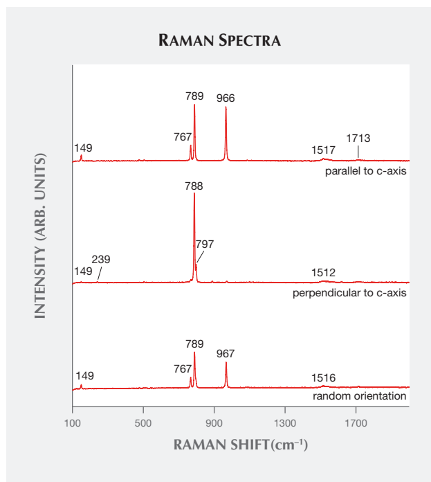
Figure 17. Raman analysis of the emerald step cut from three different optical orientations, using a near-infrared wavelength of 785 nm, confirmed its identity as synthetic moissanite.
