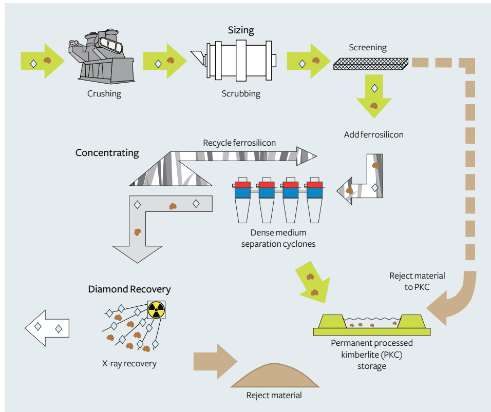
Figure 20. This diagram illustrates the steps in processing the bulk kimberlite ore to recover the diamonds. Courtesy of Diavik Diamond Mine.
