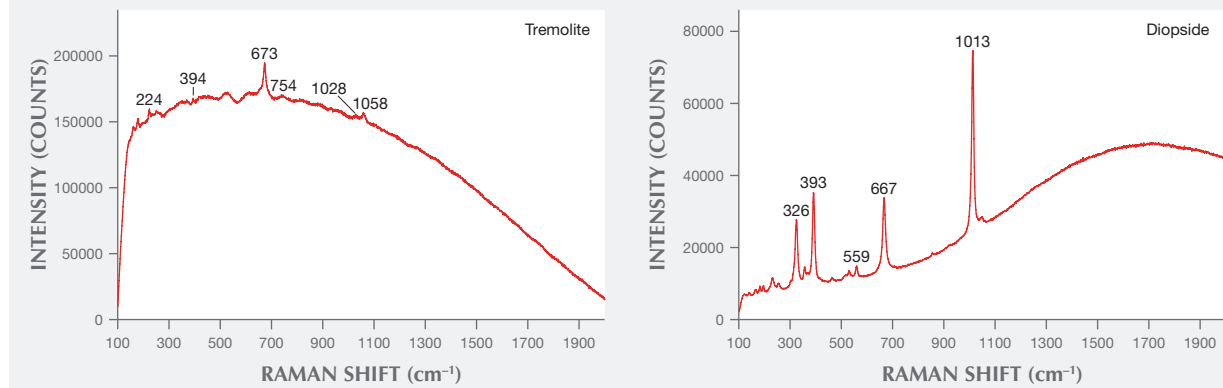
Figure 14. Raman spectra of the barrel-shaped bead. Left: Peaks at 224, 394, 673, 754, 1028, and 1058 \text{cm}^{-1} were indicative of tremolite. Right: Peaks at 326, 393, 559, 667, and 1013 \text{cm}^{-1} were consistent with diopside.
