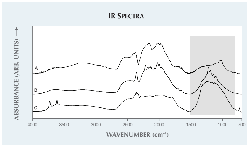
Figure 8. IR spectra of the three black samples (offset for clarity) show unusual broad peaks in the 760–1500 \text{cm}^{-1} region (highlighted in gray): 0.70 ct natural black diamond (A), 1.51 ct NPD (B), and 0.90 ct NPD (C).
