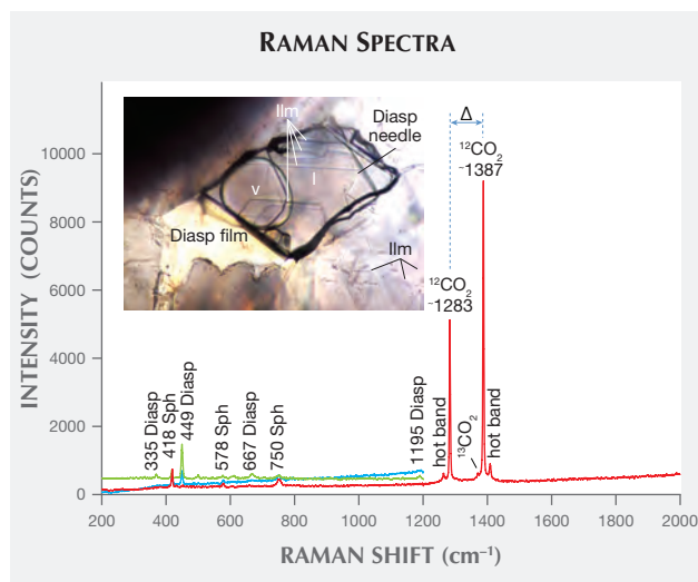
Figure 10. Raman spectra at room temperature of a fluid inclusion trapped in a sapphire from the Ilmen Mountains: ^{12}\text{CO}_2 Fermi doublet along with hot bands and ^{13}\text{CO}_2 peak (red trace), diaspore needle (blue), and a diaspore thin film (green). For ^{12}\text{CO}_2 , the average distance between Fermi doublet peaks ( \Delta ) was calculated as 104.25\text{ cm}^{-1} . Diasp = diaspore, Sph = sapphire, Ilm = ilmenite, l = liquid \text{CO}_2 , v = vapor \text{CO}_2 . Photomicrograph by Elena S. Sorokina; polarized transmitted light, field of view 0.288\text{ mm} .
