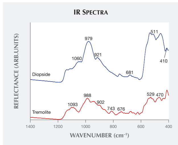
Figure 13. IR spectroscopy identified the whitish mineral in the bead as tremolite (red trace, peaks at 1093, 988, 902, 743, 676, 529, and 470 cm -1 ) and the greenish one as diopside (blue trace, peaks at 1060, 979, 921, 681, 511, and 410 cm -1 ). The spectra are offset for clarity.
