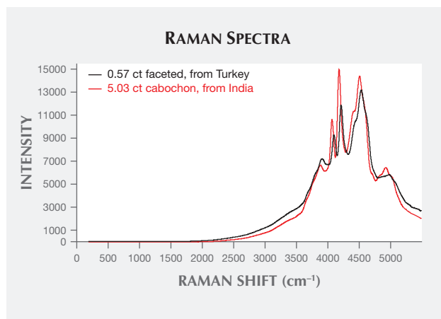
Figure 3. Raman spectra showing characteristic peaks of k ammererite at 3877, 4063, 4175, 4500, and 4920 \text{cm}^{-1} .
