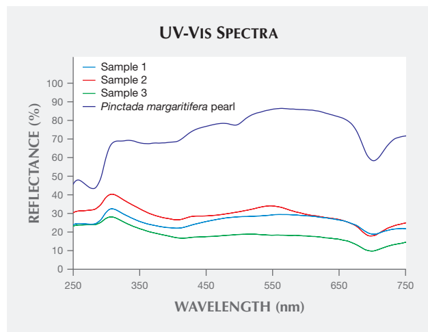
Figure 6. UV-visible reflectance spectra of the darker gray nacre areas of all three P. mazatlanica shell samples shown in figure 5 are similar to the spectrum from a P. margaritifera pearl. All show a uroporphyrin feature at 405 nm and a feature at 700 nm, which is diagnostic of P. margaritifera . These spectra prove the similar spectral characteristics between P. mazatlanica and P. margaritifera .
