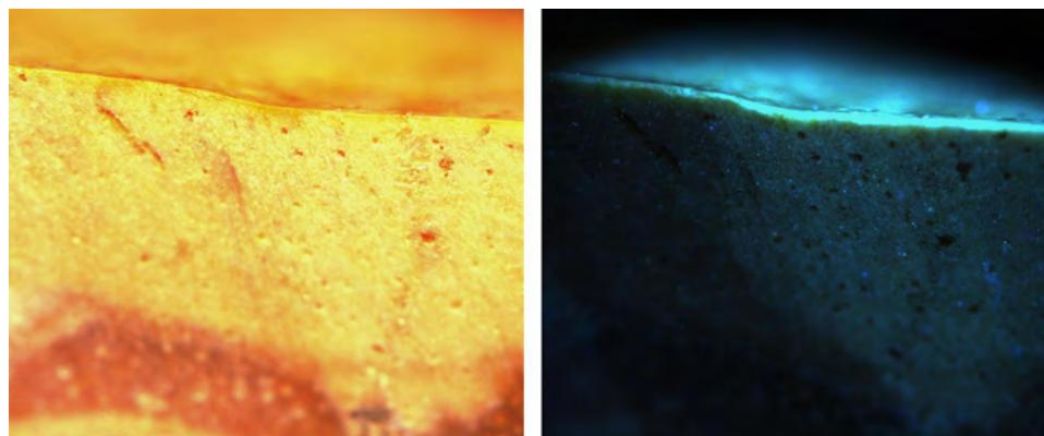
Figure 23. Diamond-View imaging showed that the inner portion of the serpentine was inert, while the surface exhibited a strong bluish fluorescence. These images show the reflection from the polymer-coated surface in visible (left) and UV light (right). Images by Lai Tai-An Gem Lab.
