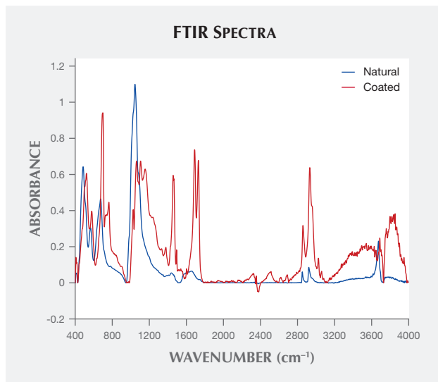
Figure 24. FTIR spectroscopy revealed peaks indicative of coating at 2858, 2932, 3025, and 3060 \text{cm}^{-1} (red) and serpentine peaks at 485, 564, 673, and 1045 \text{cm}^{-1} (blue).
