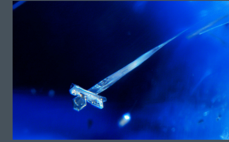
This platinum crystal inclusion in a synthetic sapphire shows a characteristic tapered morphology. This feature is diagnostic of flux growth, as in this Chatham synthetic sapphire. Field of view 1.72 mm.
