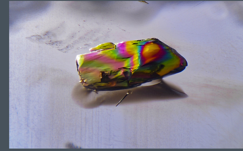
A mica crystal shows colorful interference colors in this sapphire from Sri Lanka, observed under plane-polarized light. Field of view 1.99 mm.
