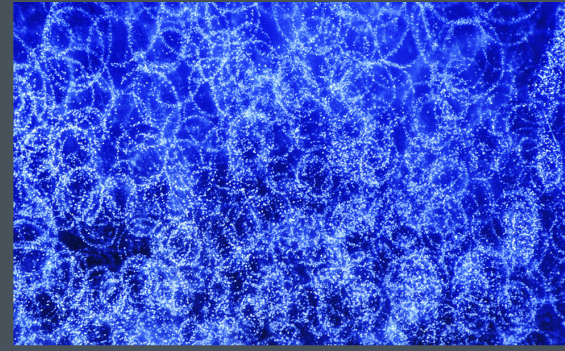
This treated blue sapphire shows "smoke ring" decorated dislocations, a result of beryllium diffusion. Field of view 1.26 mm.
