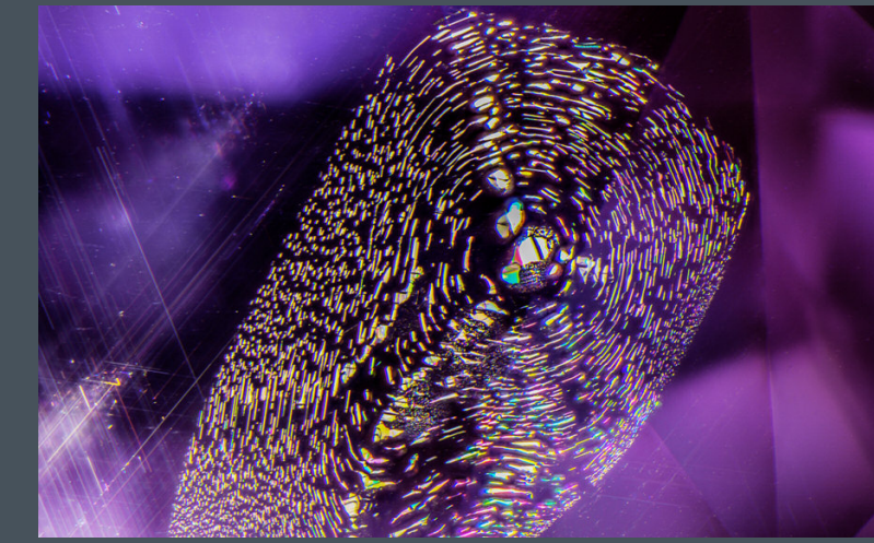
"Fingerprints" are arrays of tiny fluid or multiphase inclusions that result from the thermal healing of cracks in the growth environment, as in this Sri Lankan purple sapphire. Field of view 3.74 mm.
