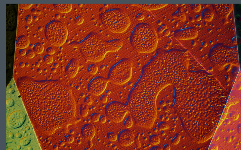
In this false-color image obtained using differential interference contrast microscopy, the surface of the sapphire shows obvious melt damage on the facet surfaces, proving heat treatment. Field of view 1.23 mm.
