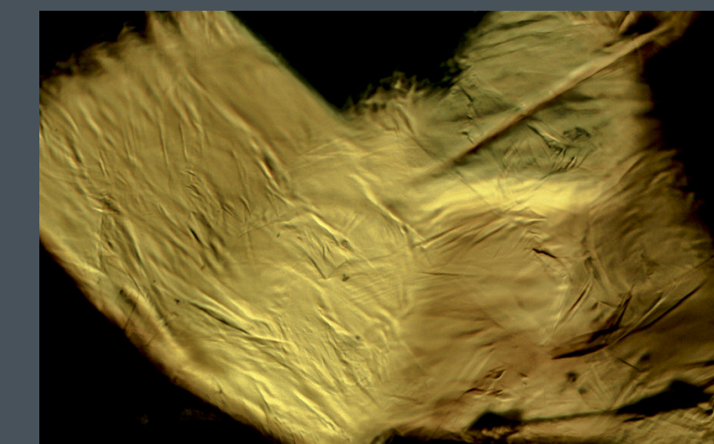
Hydrothermally grown sapphire is a rare synthetic gem material. Observed microscopically, it displays a diagnostic chevron or rolled growth structure, as seen in this yellow example. Field of view 3.00 mm.
