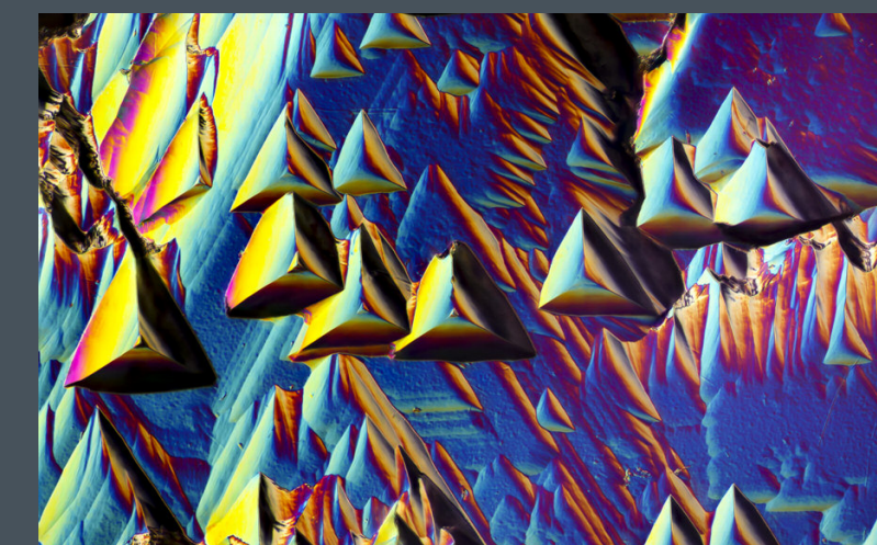
The lamprophyre dike that brought Yogo sapphires to the earth's surface partially dissolved the crystals' surface. Differential interference contrast microscopy shows crystallographic patterns and trigons. Field of view 1.44 mm.
