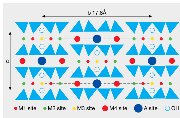
Figure 2. The crystal structure of tremolite. Adapted from Li (2008).
