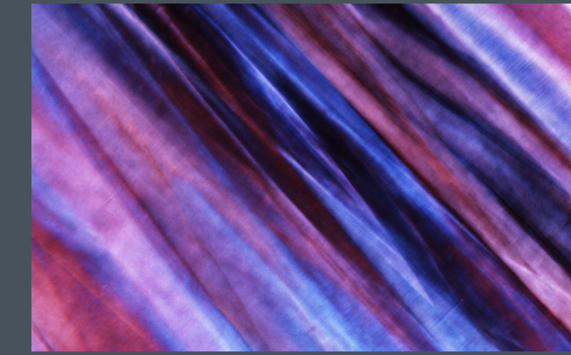
Plato-Sandmeier lines are resolved using cross-polarized light when viewed along the optic axis. They appear as shadowy subparallel striations in flame-fusion pink synthetic sapphire. Field of view 8.68 mm.
