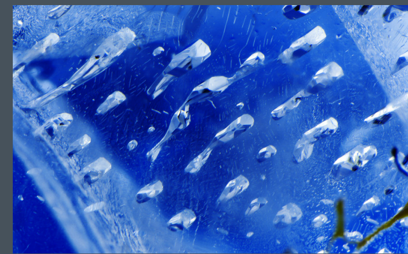
Negative crystals are a common inclusion in sapphires from metamorphic source rocks, such as this Sri Lankan specimen. They often contain a carbon dioxide fluid, graphite, and diaspore crystals. Field of view 2.62 mm.
