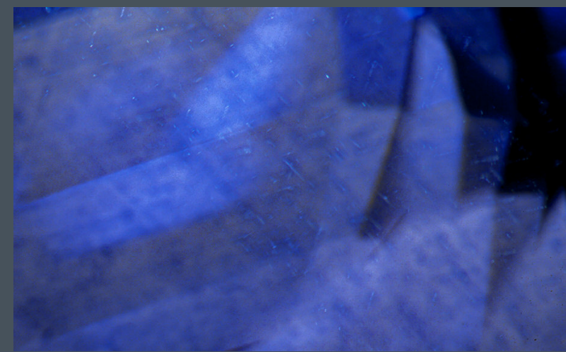
"Internal diffusion" occurs when rutile needles dissolve into the crystal lattice during heat treatment. Titanium from the rutile pairs with iron in the sapphire, increasing the blue color. Field of view 3.00 mm.
