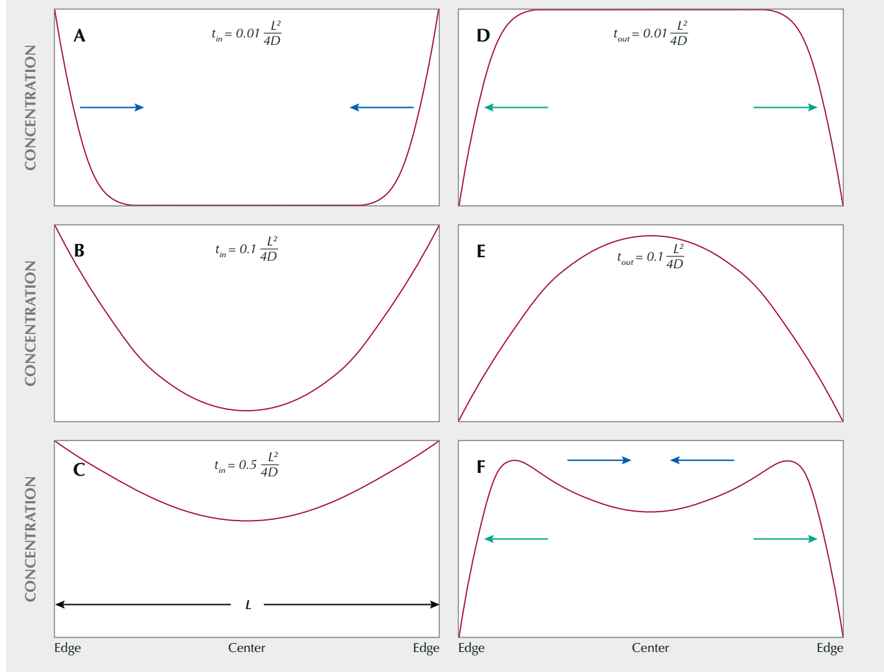
Figure 16. Schematic concentration profiles of a diffuser element (with a diffusion coefficient of D ) in a crystal (with a thickness of L ) after various diffusion processes with different directions and times. A, B, and C show typical inward diffusion profiles (initial concentration in the crystal is zero) with increasing times (at t = 0.01L^2/4D , t = 0.1L^2/4D and t = 0.5L^2/4D , respectively). D and E show outward diffusion profiles starting from a homogeneous concentration (at t = 0.01L^2/4D and t = 0.1L^2/4D , respectively). Note that inward diffusion and outward diffusion are exactly inverse processes. The profile in F can result from an incomplete inward diffusion followed by a short period of outward diffusion ( C + D ).
