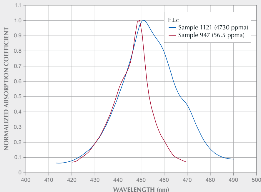
Figure 8. The E.Lc 450 nm Fe 3+ absorption coefficient plots show the band shapes for the sample with the lowest Fe 3+ concentration and the sample with the highest Fe 3+ concentration studied. Peak values are normalized to 1.0.
