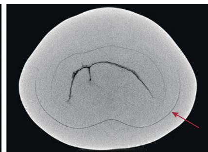
Figure 22. Left: RTX image of the pearl's internal structure with a large linear feature. Right: \mu -CT image showing a freshwater-type linear feature in the center and a faint boundary (arrow).
