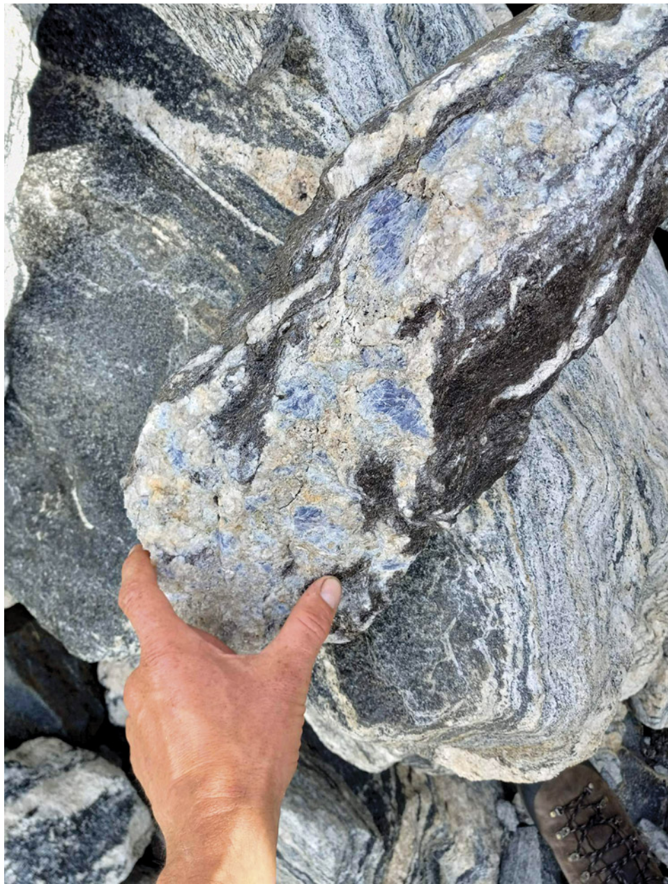
Figure 10. Cordierite-bearing biotite-quartzofeldspathic gneiss near the Blue Bear occurrence. This lithology is not known to contain gem-quality cordierite. Photo by Herb Hyder.
