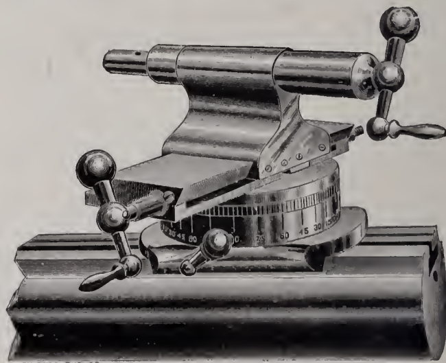
UNIVERSAL TAIL STOCK.
