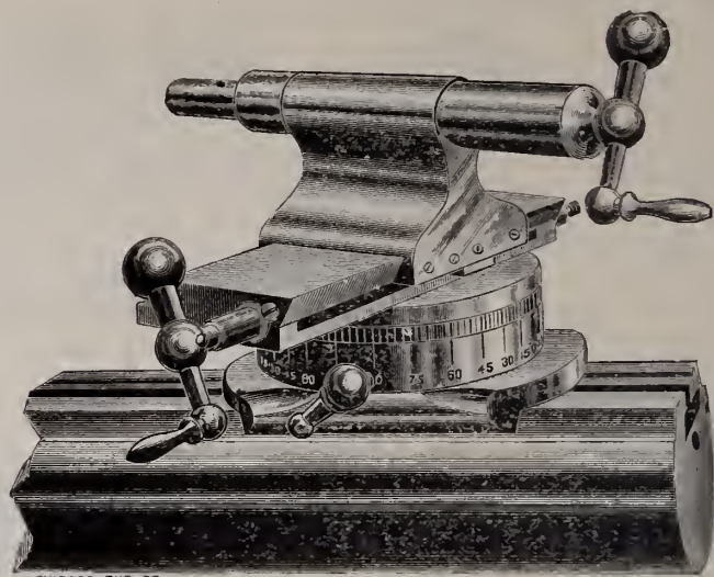
UNIVERSAL TAIL STOCK. (PATENT APPLIED FOR.)
