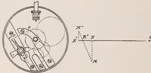
PLAN FOR ADJUSTING WATCHES.
