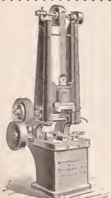
No. 5 Automatic Drop.
