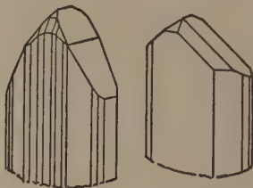
2. Zoisite p. 297 (Wardsborough, Vermont)
