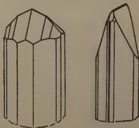
6. Danburite (Russel, St. Lawrence County, New York)
