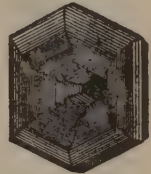
Fig. 26 Rutile "sixling"
