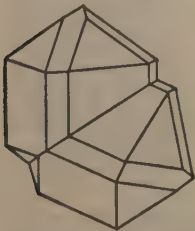
Fig. 27 Cassiterite twin
