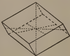
Fig. 20 Rhombohedron axes
