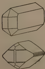
5. Antlerite (Chuquicamata, Chile)
