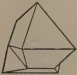
Fig. 24 Spinel twin
