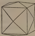
Fig. 15 Tetrahex- ahedron
