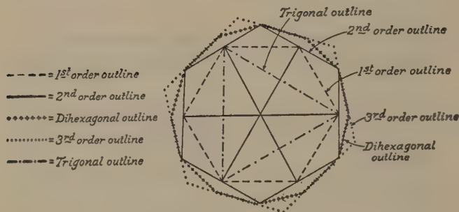
Fig. 19 Hexagon outlines
