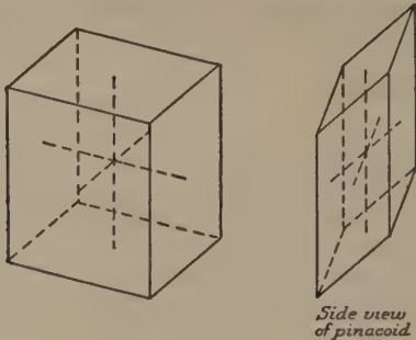
Fig 23 Triclinic system axes and pinacoids
