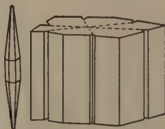
4. Aragonite: twinned crystals (Agrigento, Sicily)
