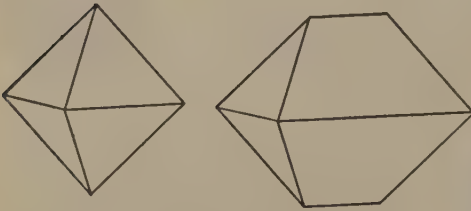
Fig. 29b Normal and elongated octahedron
