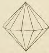
Fig. 39. Dihexagonale Pyramide.
