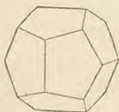
Fig. 32. Pentagondodekaeder. Schwefelkies.
