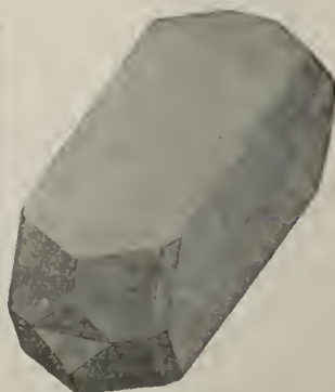
Fig. 296. Manebach Twin.
