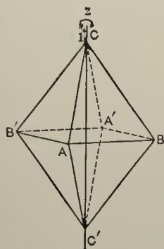
Fig. 6. Symmetry Axis.
