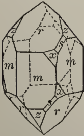
Fig. 251. Right-handed Crystal.
