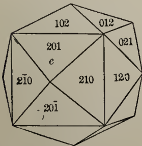
Fig. 40. Tetrahexahedron.
