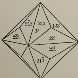
Fig. 46. Trisoctahedron.
