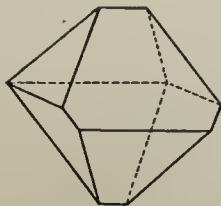
Fig. 20. Distorted Octahedron.
