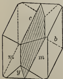
Fig. 5. Symmetry Plane.
