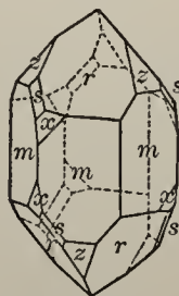
Fig. 145. Left-handed Quartz.
