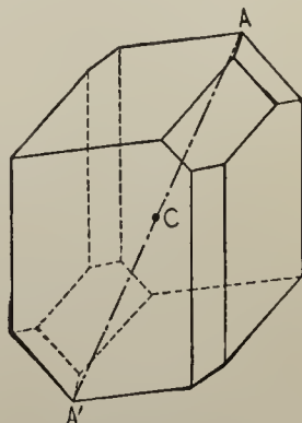
Fig. 7. Symmetry Center.
