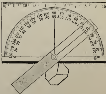
Fig. 4. Contact Goniometer.
