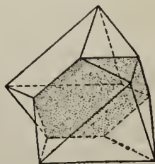
Fig. 24. Twinned Octahedron.
