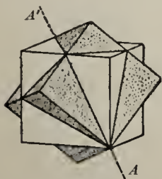
Fig. 23. Twinned Cubes.
