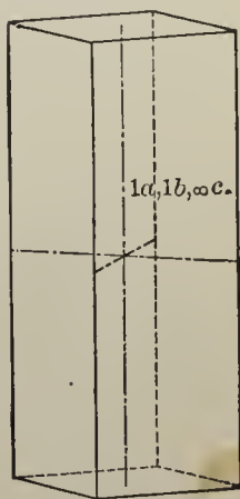
Fig. 10. Orthorhombic Prism.
