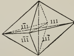
Fig. 184. Pyramids.
