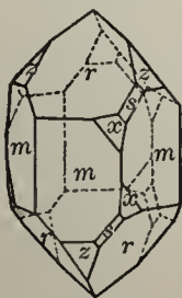
Fig. 144. Right-handed Quartz.
