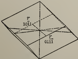
Fig. 123. Positive Rhombohedron.
