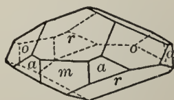
Fig. 141. Tourmaline.
