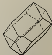
Fig. 22. Distorted Dodecahedron.
