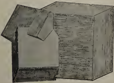
Fig. 229. Striated Cubes.
