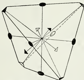
Fig. 99. Symmetry Axes.
