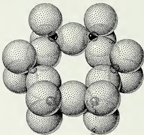
Fig. 561. \text{Si}_6\text{O}_{18} Ring.
