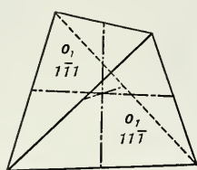
Fig. 105. Negative Tetrahedron.
