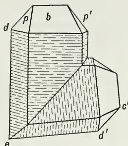
Fig. 318. Japanese Twin.
