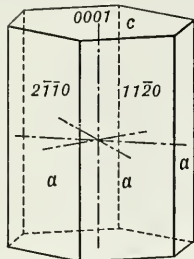
Fig. 138. Second-Order Prism.
