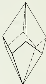
Fig. 36. Tetragonal Trapezohedron.
