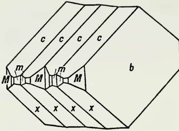
Fig. 303. Albite Twins.
