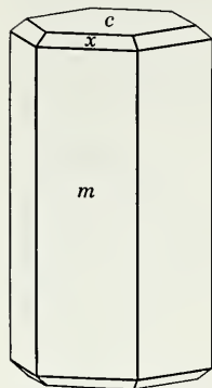
Fig. 526. Pyromorphite.
