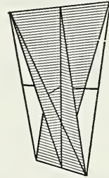
Fig. 224. Symmetry Planes.
