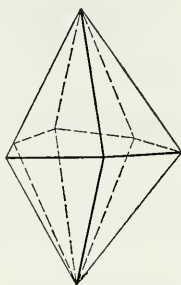
Fig. 151. Ditrigonal Dipyramid.
