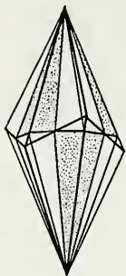
Fig. 176. Relation between Dihexagonal Dipyramid and Scalenohedron.
