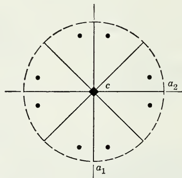
Fig. 222. Stereogram of Ditetragonal Pyramid.
