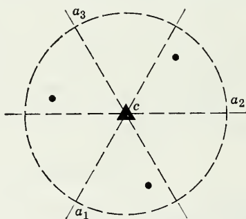
Fig. 196. Stereogram of Trigonal Pyramid.
