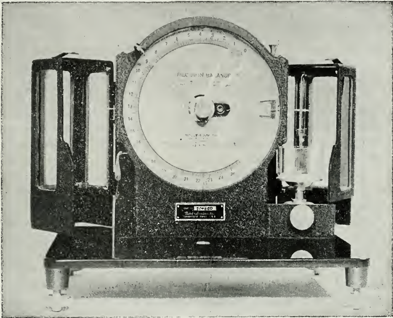
Fig. 364. Berman Balance.
