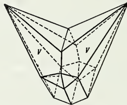
Fig. 494. Calcite Twinned on the Unit Rhombohedron.
