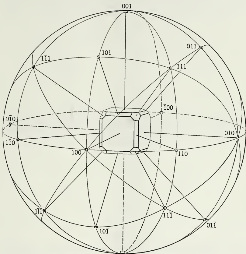
Fig. 53. Spherical Projection of Isometric Forms.
