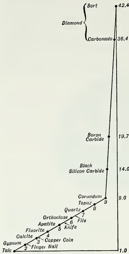
Fig. 361. Relative Hardness of Minerals in the Scale of Hardness (after Wooddell).
