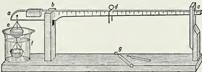
Fig. 365. Beam Balance.
