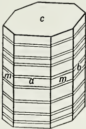
Fig. 358. Basal Parting of Pyroxene.
