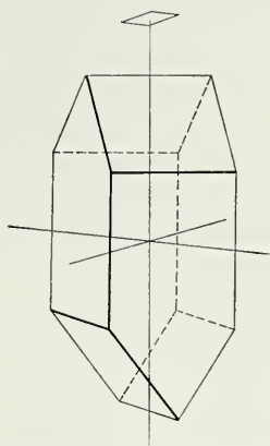
Fig. 9. Four-fold Axis of Rotary Inversion.
