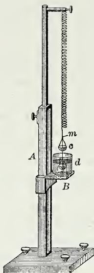
Fig. 362. Jolly Balance.
