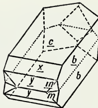
Fig. 329. Carlsbad Twin. Fig. 330. Manebach Twin. Fig. 331. Baveno Twin. Fig. 332. Albite Twinning.
