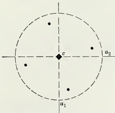
Fig. 234. Stereogram of Tetragonal Pyramid.
