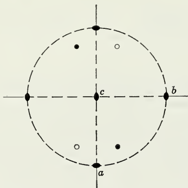
Fig. 260. Stereogram of Rhombic Disphenoid.
