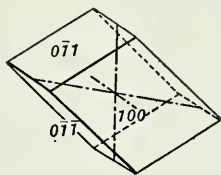
Fig. 295. First-Order Pinacoids and Front Pinacoid.
