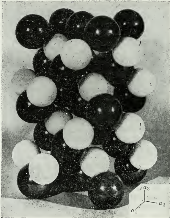
Fig. 412. Sphalerite, ZnS, Packing Model. Zn (black) and S (white) are both in 4-fold coordination. Note sheets of atoms parallel to (111). If they are rotated 180^\circ alternately, the wurtzite structure results.
