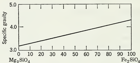
Fig. 533. Specific Gravity of Olivine.
