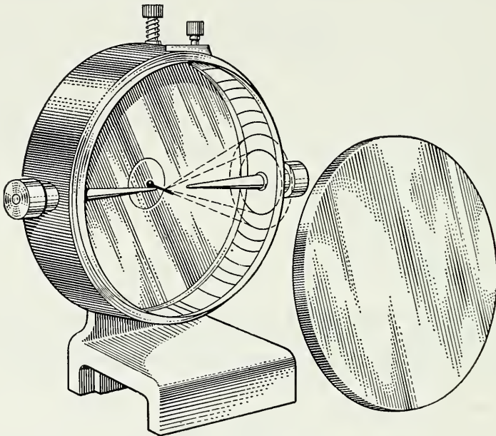
Fig. 351. Powder Camera.
