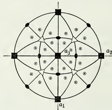
Fig. 74. Stereogram of Hexoctahedron.
