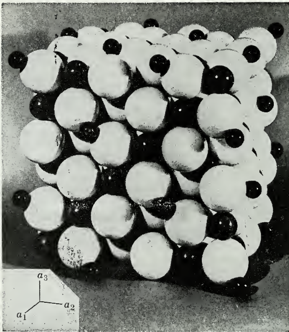
Fig. 438. Spinel, MgAl_2O_4 , Packing Model. A number of related minerals, including magnetite FeFe_2O_4 , gahnite ZnAl_2O_4 , and chromite FeCr_2O_4 , also have this structure, in which Mg, Fe^{II} or Zn (small dark) is in 4-fold coordination and Al, Fe^{III} or Cr (large dark) is in 6-fold coordination with O (white).
