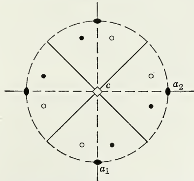
Fig. 226. Stereogram of Tetragonal Scalenohedron.
