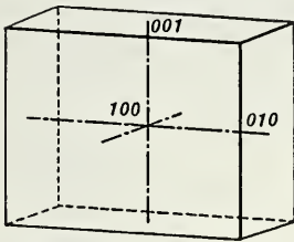
Fig. 243. Orthorhombic Pinacoids.
