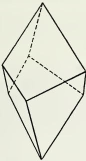
Fig. 183. Trigonal Trapezohedron.
