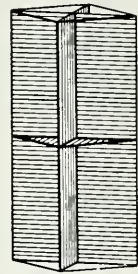
Fig. 240. Symmetry Planes.
