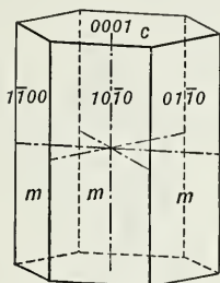
Fig. 137. First-Order Prism.
