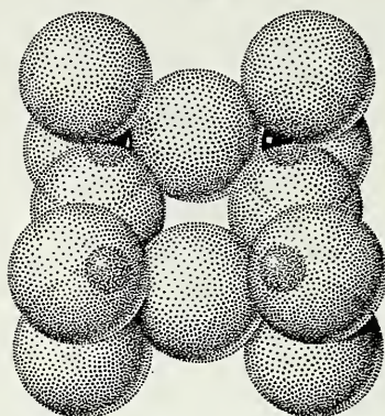
Fig. 560. \text{Si}_4\text{O}_{12} Ring.
