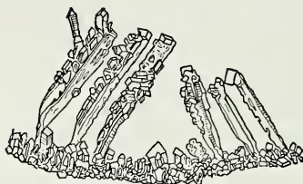
Fig. 393. Dendritic Copper.
