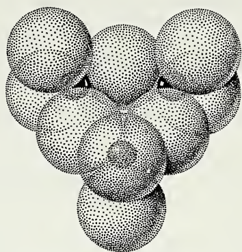
Fig. 559. \text{Si}_3\text{O}_9 Ring.
