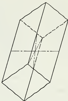
Fig. 267. Monoclinic Prism.
