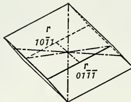
Fig. 165. Positive Rhombohedron.
