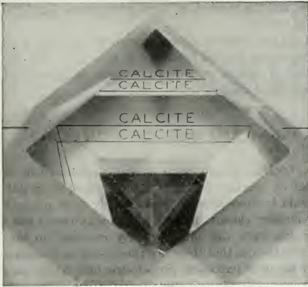
Fig. 369. Calcite, Viewed Normal to the Rhombohedron Face Showing Double Refraction. The double repetition of "calcite" at the top of the photograph is seen through a face cut on the specimen parallel to the base.
