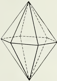
Fig. 40. Hexagonal Dipyramid.
