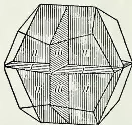
Fig. 116. Symmetry Planes.
