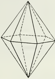
Fig. 153. Hexagonal Dipyramid.
