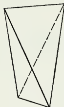
Fig. 236. Tetragonal Disphenoid.
