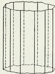
Fig. 26. Dihexagonal Prism.
