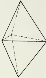
Fig. 38. Trigonal Dipyramid.
