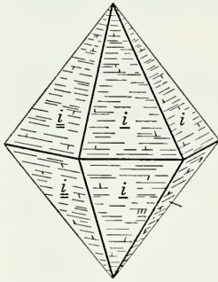
Fig. 502. Witherite.
