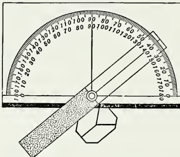
Fig. 62. Contact Goniometer.
