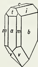
Fig. 554. Hemimorphite.
