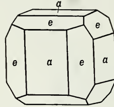
Fig. 123. Cube and Pyritohedron.
