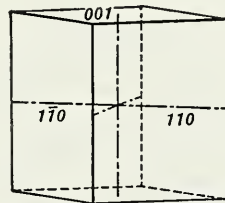
Fig. 246. Unit Third-Order Prism and Basal Pinacoid.
