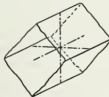
Fig. 28. Horizontal Orthorhombic Prism.
