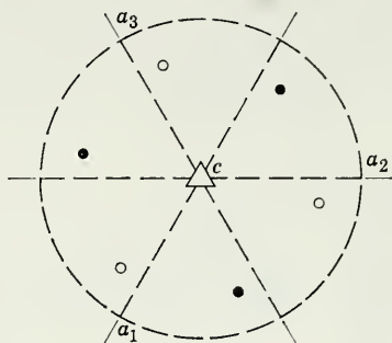
Fig. 194. Stereogram of Rhombohedron.
