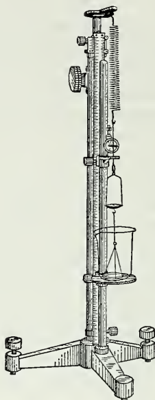
Fig. 363. Improved Jolly Balance.
