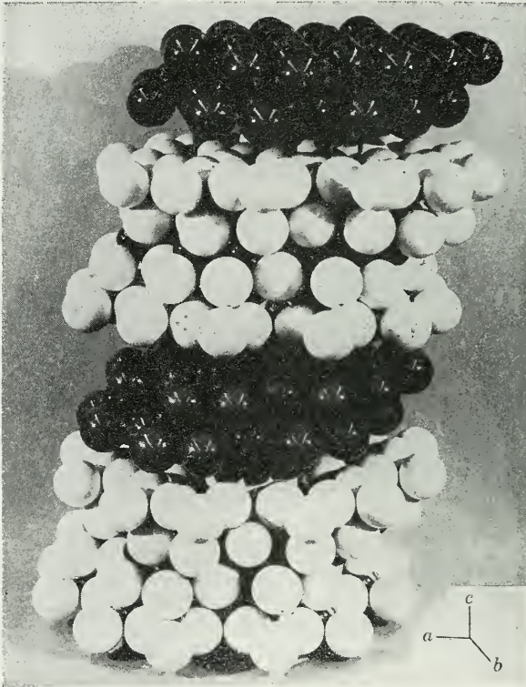
Fig. 594. Chlorite, Mg_3Si_4O_{10}(OH)_2 \cdot Mg_3(OH)_6 . Packing Model. O white, (OH) large black, Mg small black; c axis vertical. The model shows "t-o-t" sheets alternating with "o" sheets. Fe II , Fe III and Al may substitute for Mg and Al for Si.
