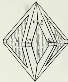
Fig. 323. Aragonite. Fig. 324. Cross Section of Cyclic Aragonite Twin. Fig. 325. Cerussite.
