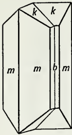
Fig. 323. Aragonite. Fig. 324. Cross Section of Cyclic Aragonite Twin. Fig. 325. Cerussite.
