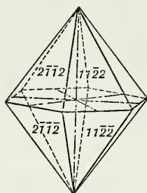
Fig. 141. Second-Order Dipyramid.
