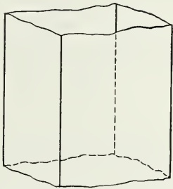
Fig. 24. Tetragonal Prism.
