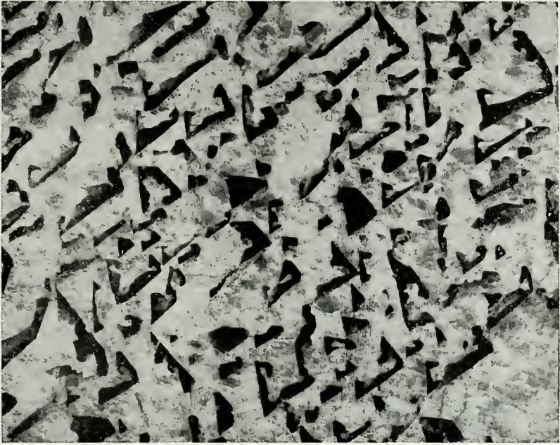
Fig. 612. Graphic Granite, Hybla, Ontario. Quartz dark, feldspar light.
