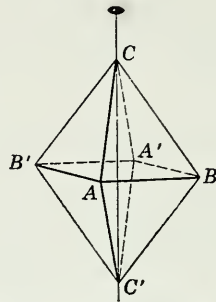
Fig. 7. Symmetry Axis.
