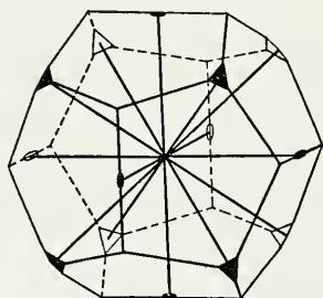
Fig. 115. Symmetry Axes.
