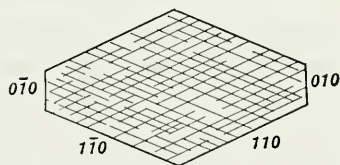
Fig. 579. Amphibole Cleavage.
