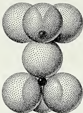
Fig. 553. \text{Si}_2\text{O}_7 Group.
