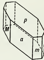
Fig. 302. Chalcanthite.
