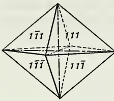
Fig. 247. Orthorhombic Dipyramid.
