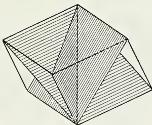
Fig. 161. Symmetry Planes.
