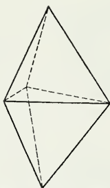
Fig. 158. Trigonal Dipyramid.
