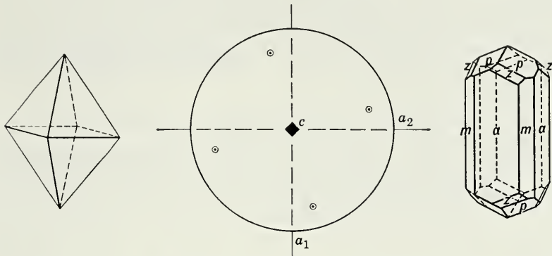
Fig. 230. Tetragonal Dipyramid.
