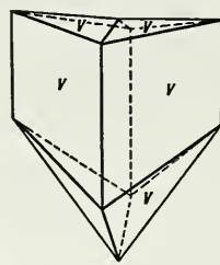
Fig. 313. Calcite Twinned on \{01\bar{1}2\} .
