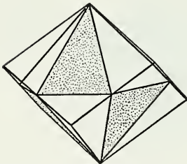
Fig. 164. Relation between First-Order Hexagonal Dipyrmaid and Rhombohedron.
