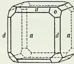
Fig. 83. Cube, Octahedron, and Dodecahedron.
