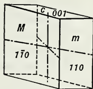
Fig. 297. Third-Order Pinacoids and Basal Pinacoid.
