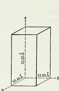
Fig. 11. Unit Cell of Sulfur.
