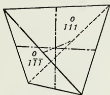
Fig. 104. Positive Tetrahedron.
