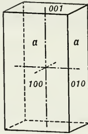
Fig. 204. Second-Order Prism.
