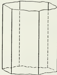
Fig. 25. Hexagonal Prism.
