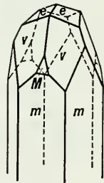
Fig. 182. Prism, Positive Scalenohedron, Positive Rhombohedron, Negative Rhombohedron.
