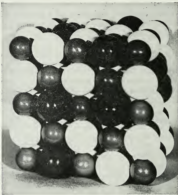
Fig. 333. Random Substitution of Anions in Sodium Chloride Structure. Cations — small dark; anions — large white and black.
