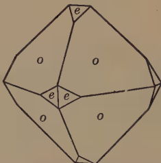
Fig. 60. Octahedron and Pyritohedron.
