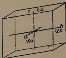
Fig. 188. Macropinacoid, Brachypinacoid, and Basal Pinacoid.
