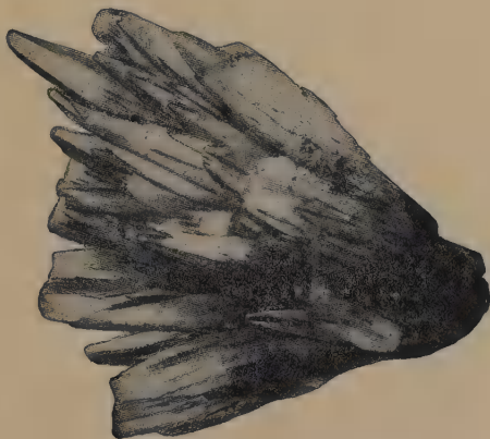
B. Aragonite, Cleator Moor, England.
