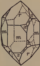
Fig. 144. Right-handed Quartz.
