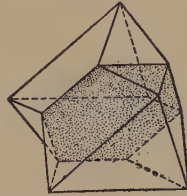
Fig. 24. Twinned Octahedron.
