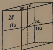
Fig. 185. Prisms and Basal Pinacoid.
