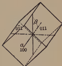
Fig. 174. Clinodome and Orthopinacoid.
