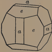
Fig. 231. Cube and Pyritohedron.
