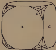
Fig. 49. Cube and Hexoctahedron.
