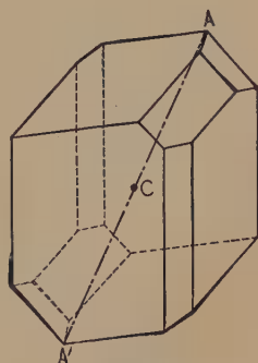
Fig. 7. Symmetry Center.
