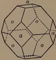
Fig. 34. Octahedron and Cube.
