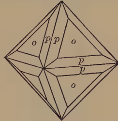
Fig. 47. Octahedron and Trisoctahedron.
