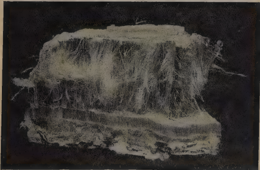
A. Crystallized—Quartz. B. Stalactitic—Limonite.
