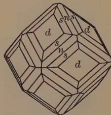
Fig. 51. Dodecahedron, Trapezohedron and Hexoctahedron.
