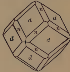
Fig. 43. Dodecahedron and Trapezohedron.
