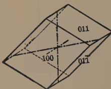
Fig. 187. Brachydomes and Macropinacoid.
