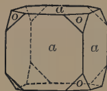
Fig. 215. Cube and Octahedron.
