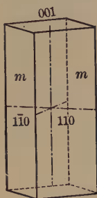
Fig. 82. First Order Prism.
