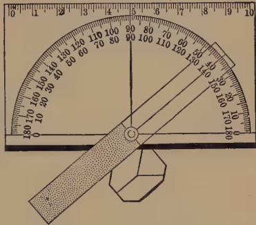
Fig. 4. Contact Goniometer.
