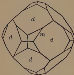
Fig. 44. Dodecahedron and Trapezohedron.
