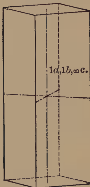
Fig. 10. Orthorhombic Prism.
