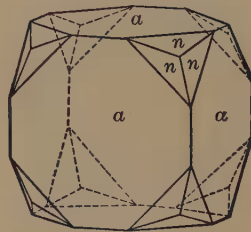
Fig. 45. Cube and Trapezohedron.
