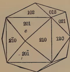
Fig. 40. Tetrahexahedron.
