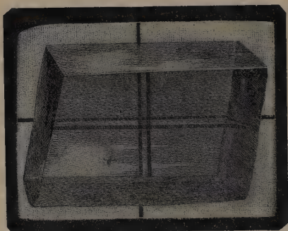
Fig. 199. Double Refraction in Calcite.
