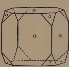
Fig. 33. Cube and Octahedron.
