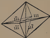
Fig. 184. Pyramids.
