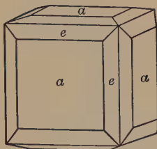
Fig. 41. Cube and Tetrahexahedron.
