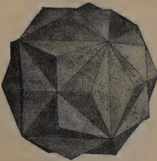
Fig. 234. Twinned Pyritohedrons.
