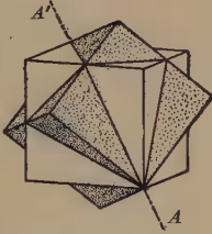
Fig. 23. Twinned Cubes.
