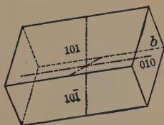
Fig. 186. Macrodomes and Brachypinacoid.
