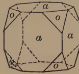
Fig. 15. Cube Truncated by Octahedron.
