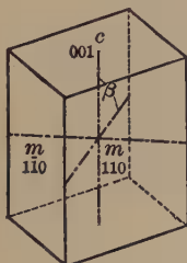
Fig. 172. Prism and Base.
