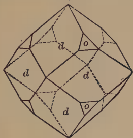
Fig. 38. Dodecahedron and Octahedron.
