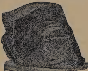
Fig. 193. Conchoidal Fracture — Volcanic Glass.
