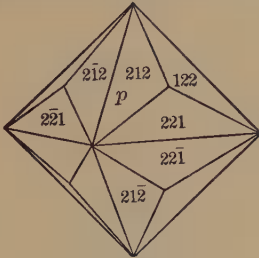
Fig. 46. Trisoctahedron.
