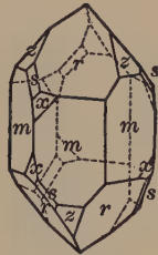
Fig. 145. Left-handed Quartz.
