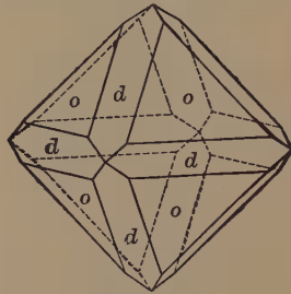
Fig. 37. Octahedron and Dodecahedron.
