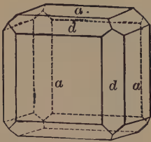
Fig. 36. Cube and Dodecahedron.
