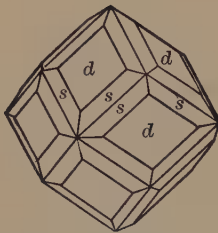
Fig. 50. Dodecahedron and Hexoctahedron.
