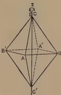
Fig. 6. Symmetry Axis.
