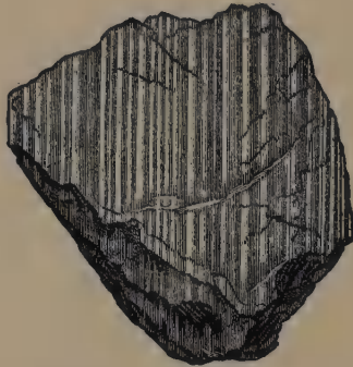
Fig. 301. Albite Twinning.
