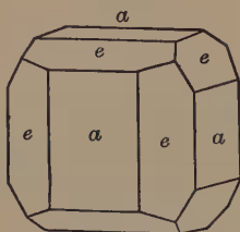
Fig. 59. Cube and Pyritohedron.
