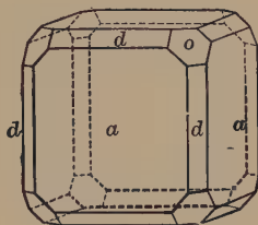
Fig. 39. Cube, Octahedron and Dodecahedron.
