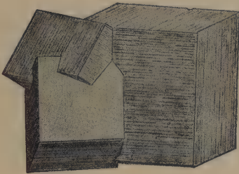
Fig. 229. Striated Cubes.
