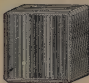
Fig. 58. Striated Cube.
