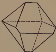
Fig. 20. Distorted Octahedron.
