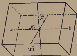
Fig. 173. Orthodomes and Clinopinacoid.
