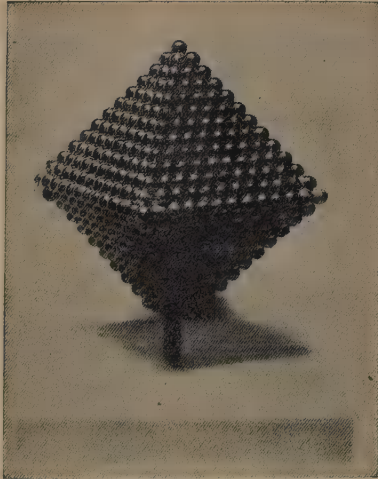
B. Octahedron. Models made of Steel Balls.
