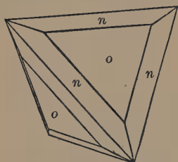
Fig. 78. Tetrahedron and Tristetrahedron.
