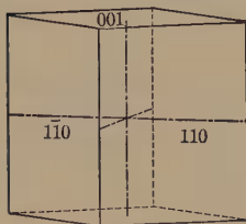
Fig. 150. Prism and Base.
