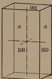
Fig. 83. Second Order Prism.
