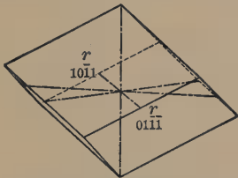
Fig. 123. Positive Rhombohedron.
