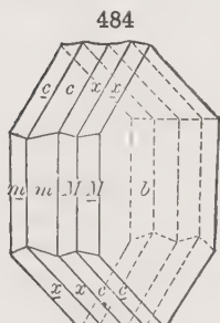
Albite
