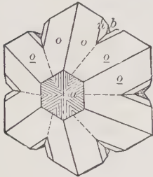
Chrysoberyl
