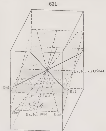
Horizontal Dispersion
