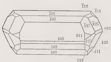
Projection on (001)
