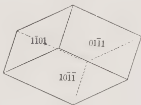
Negative Rhombohedron
