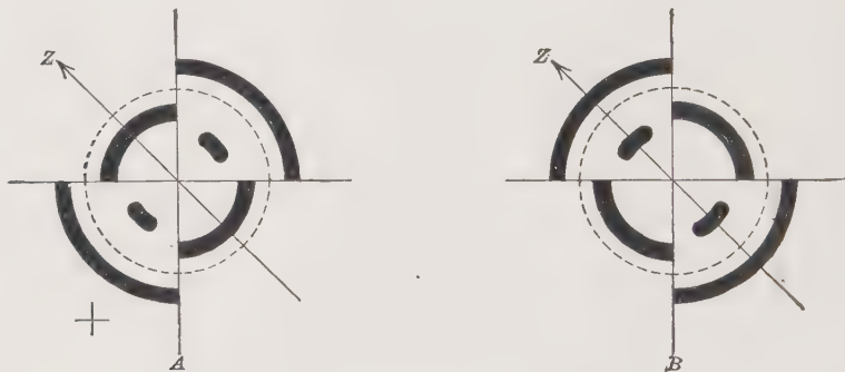
Determination of Optical Character with Mica Plate
