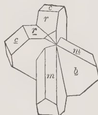
Arsenopyrite
