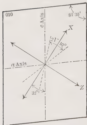
Optical Orientation of Wollastonite.
