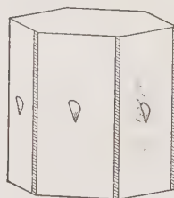
Nephelite
