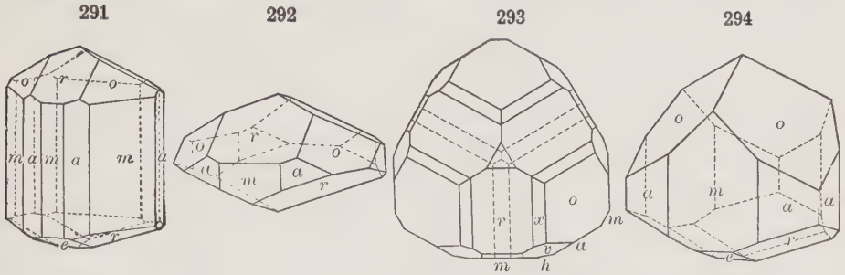
Figs. 291-294, Tourmaline
