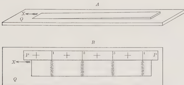
Quartz Wedge
