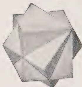
Fluorite
