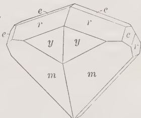
Figs. 445–452, Calcite
