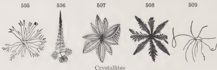
Crystallites
