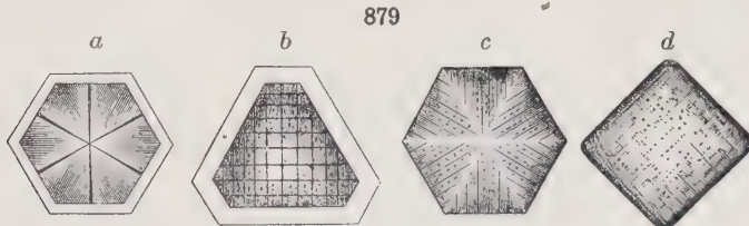
Sections of crystals of h aüynite (after M ohl)
