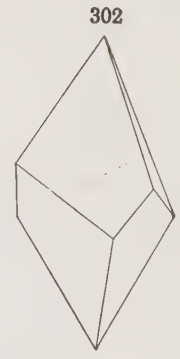
Trigonal Trapezohedrons
