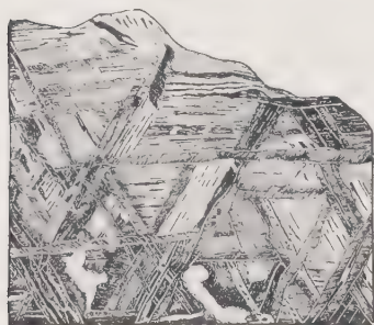
Glorieta Mt., New Mexico
