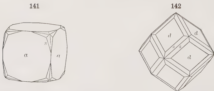
Fluorite. Cube and Hexoctahedron
