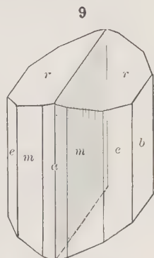
Amphibole
