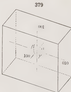
Triclinic Pinacoids
