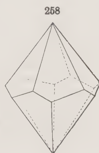
Hexagonal Trapezohedron
