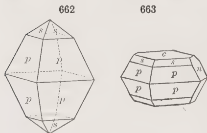
Sulphur Crystals
