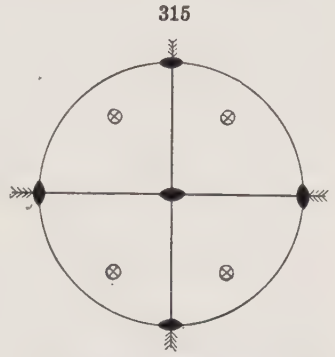
Symmetry of Normal Class Orthorhombic System
