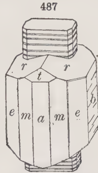
Amphibole enclosing pyroxene in parallel position
