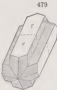
Phillipsite
