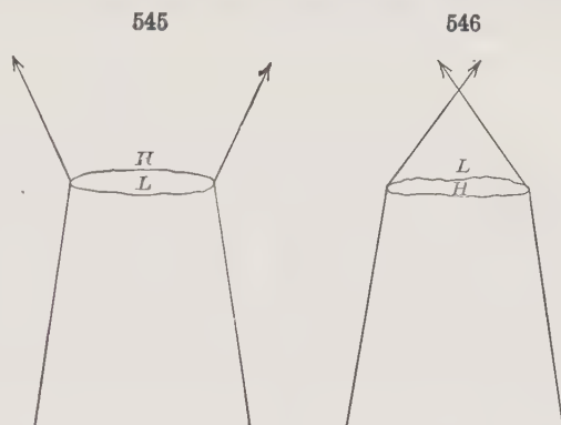
545 Grain with Low Refractive Index immersed in Liquid of High Refractive Index 546 Grain with High Refractive Index immersed in Liquid of Low Refractive Index
