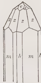
Cassiterite
