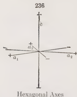
Hexagonal Axes
