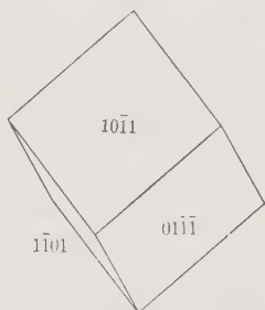
Positive Rhombohedron Hematite
