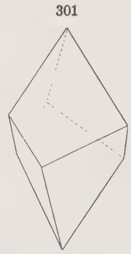
Trigonal Trapezohedrons
