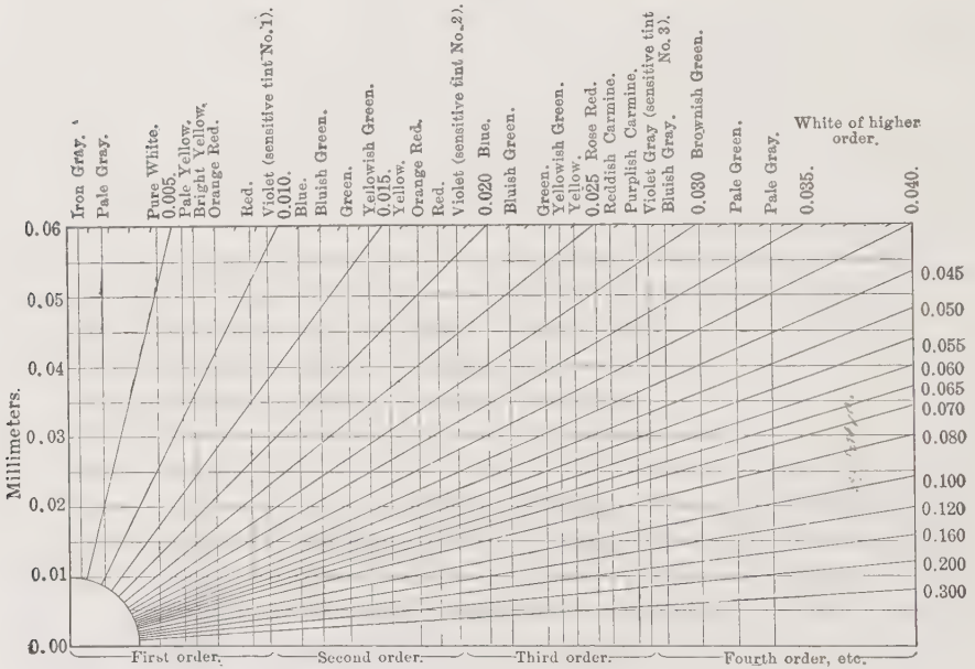
Determination of the Strength of Birefringence (after Pirsson and Robinson)
