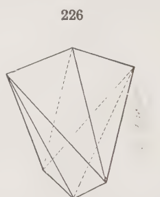
Tetragonal Scalenohedron
