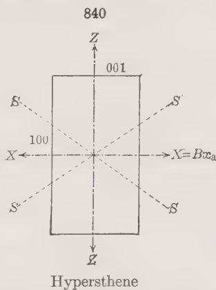
Hypersthene
