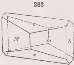
Albite
