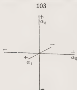
Isometric Axes
