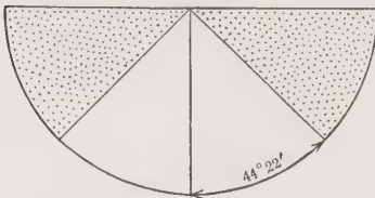
Total Reflection in Fluorite n = 1.43
