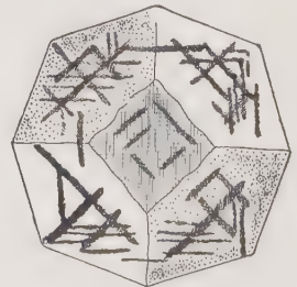
Leucite, || 100
