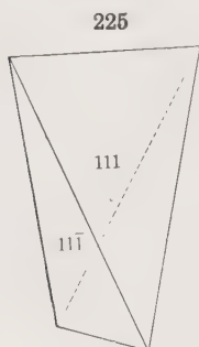
Sphenoid
