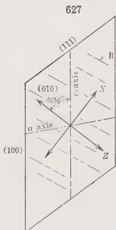
Optical Orientation of Gypsum
