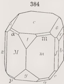
Anorthite
