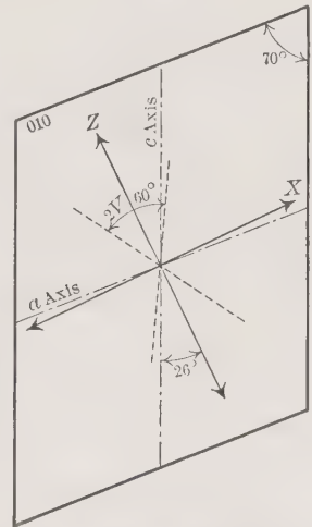
Optical Orientation of Spodumene.
