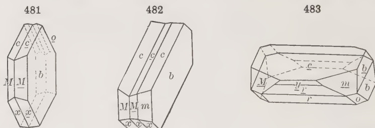
Albite
