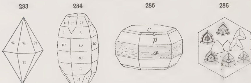
Figs. 283, 284, Corundum
