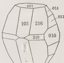
Humite , Sweden
