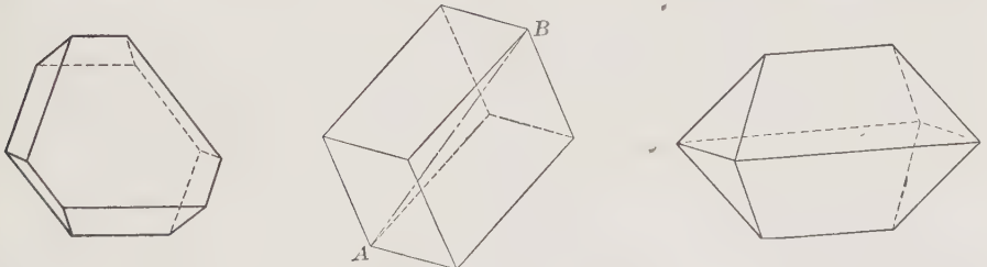
Distorted Octahedrons
