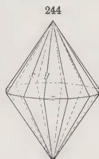
Dihexagonal Pyramid
