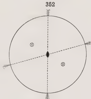
352 Symmetry of Normal Class
