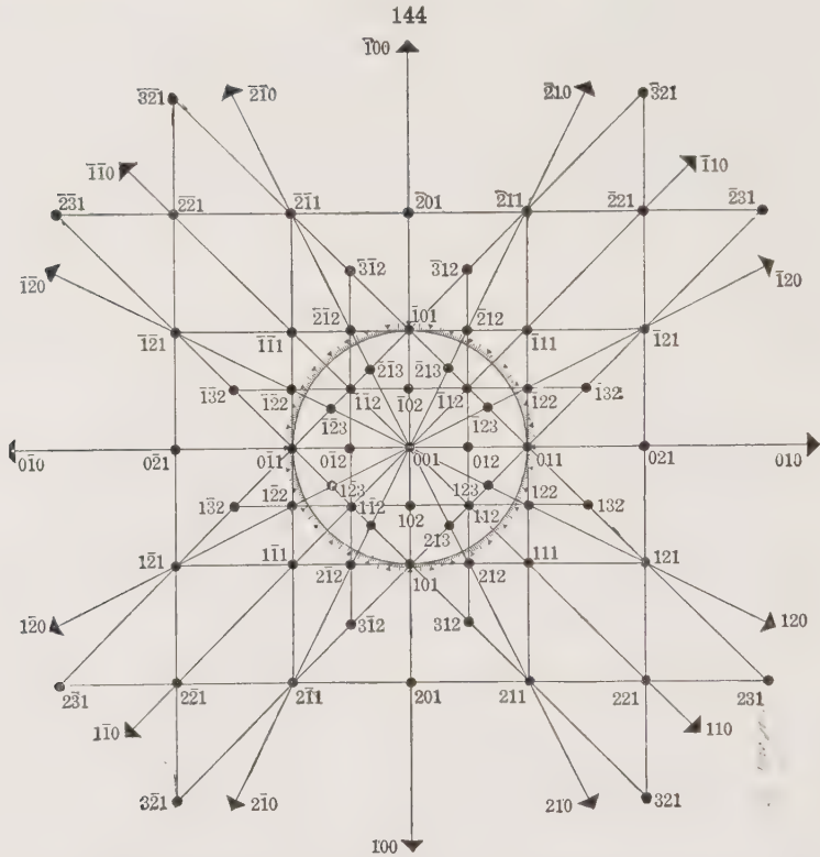
Gnomonic Projection of Isometric Forms (Cube (100), Octahedron (111), Dodecahedron (110), Tetrahedron (210), Trisoctahedron (211), Trapezohedron (211), Hexoctahedron (321))
