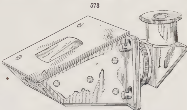
Smith Total Refractometer (Actual Size)
