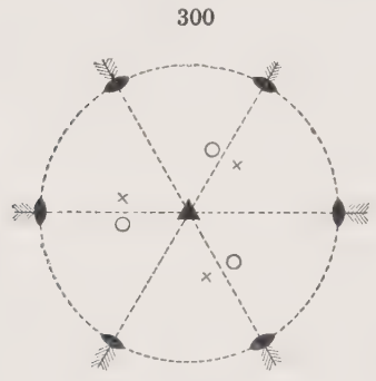
Symmetry of Trapezohedral Class
