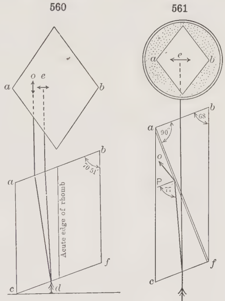
Nicol Prism
