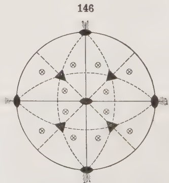
Symmetry of Pyritohedral class
