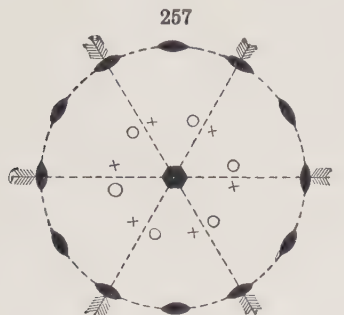
Symmetry of Trapezohedral Class
