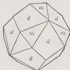
m = (311)
