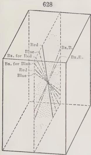
Inclined Dispersion
