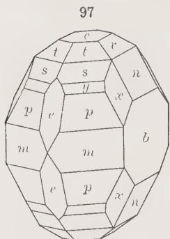
Sulphur
