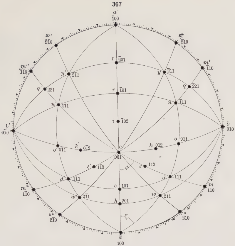
Stereographic Projection of Epidote Crystal
