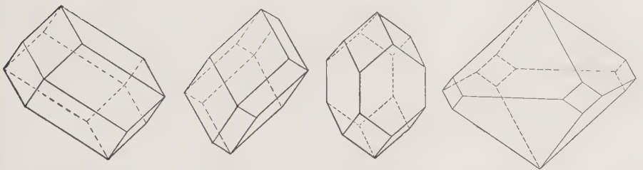
Distorted Dodecahedrons
