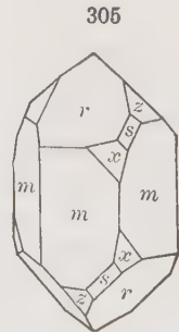
Figs. 303-307, Quartz
