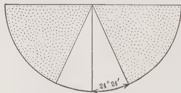
Total Reflection in Diamond n = 2.42
