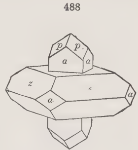
Xenotime enclosing zircon in parallel position
