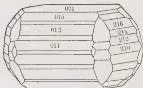
Humite , Vesuvius
