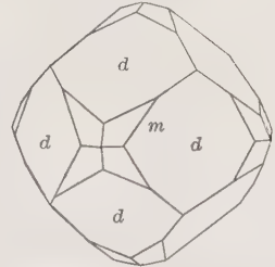
Magnetite. Dodecahedron and Trapezohedron
