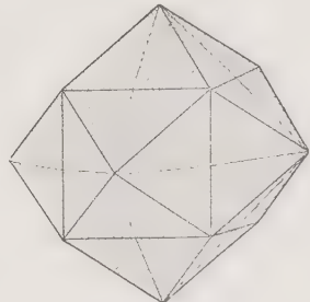
Phillipsite
