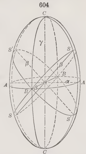
Biaxial Indicatrix
