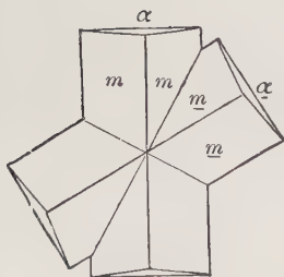
Arsenopyrite
