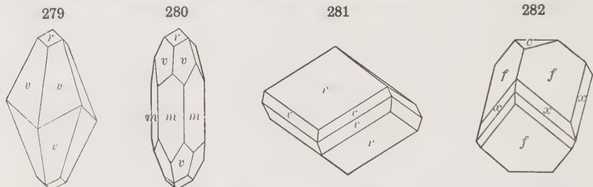
Figs. 279-282, Calcite
