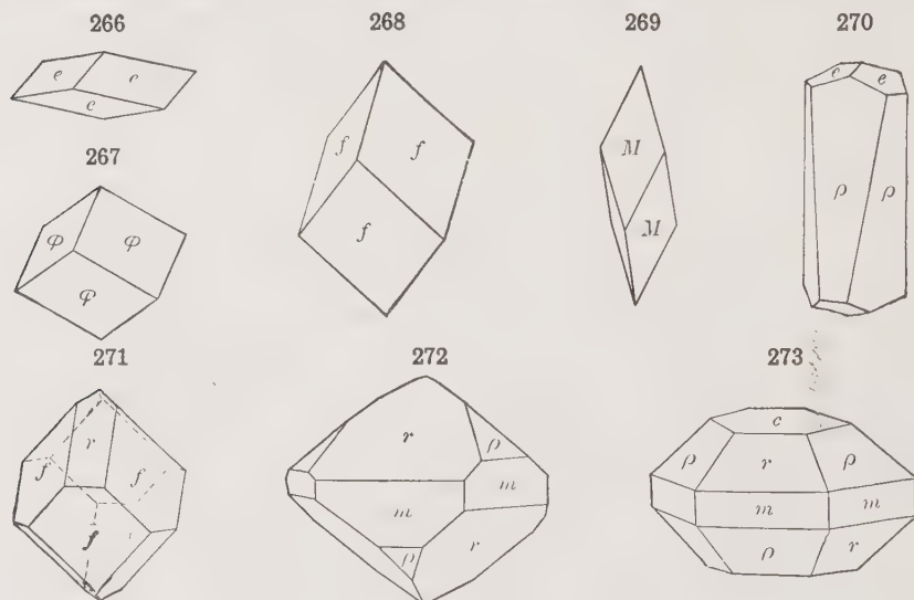
Figs. 266-271, Calcite Figs. 272-273, Gmelinite
