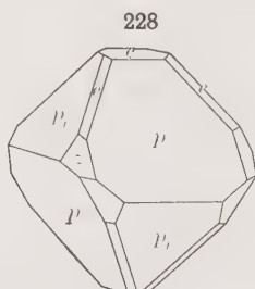
Chalcopyrite
