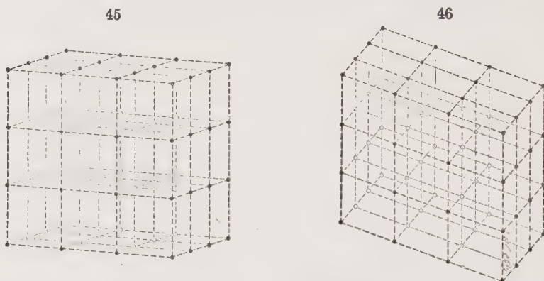
Crystal Networks
