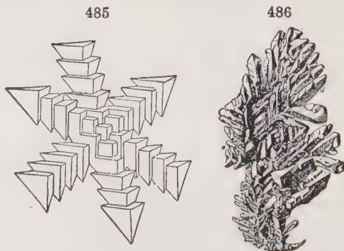
Copper
