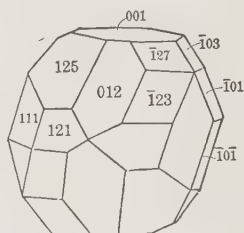
Chondrodite , Sweden
