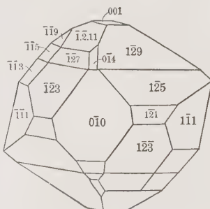
Clinohumite , Brewster
