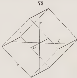
Dome (011), (0kl)
