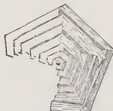
Arsenopyrite
