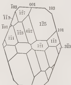
Projection on (010)
