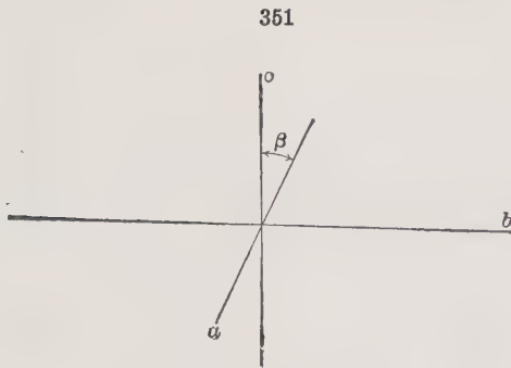
351 Crystal Axes of Orthoclase a:b:c = 0.66:1:0.55 . \beta = 64^\circ
