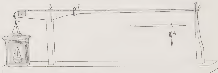
Beam Balance for Specific Gravity, \frac{1}{2} th Natural Size (after Penfield)
