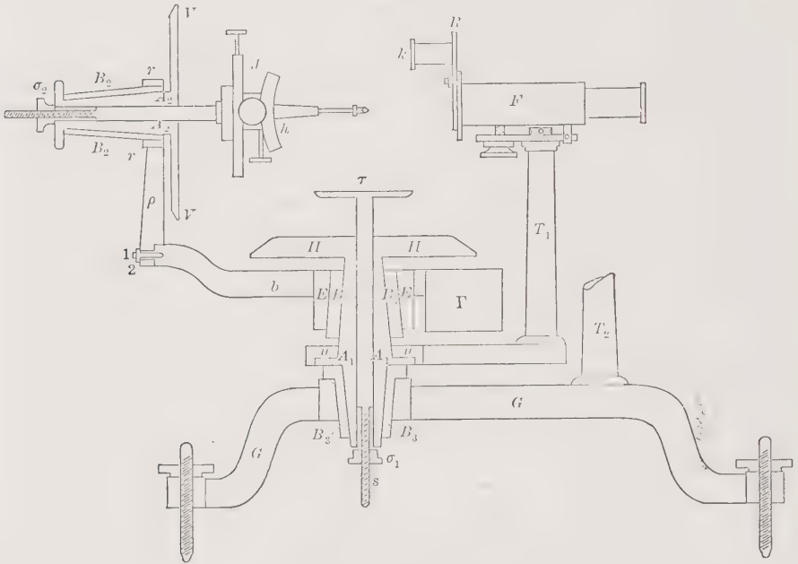
Two-circle Reflection Goniometer
