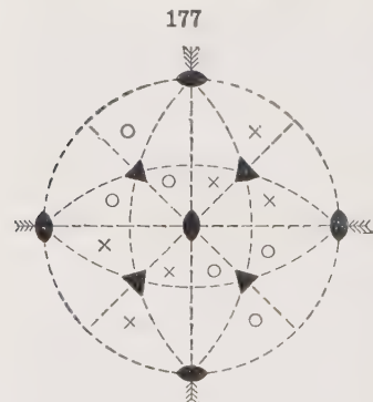
Symmetry of Tetartohedral Class
