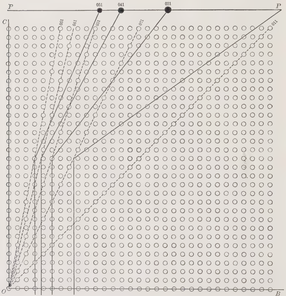
X-ray Reflection in KCl
