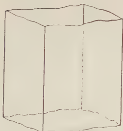
Fig. 24. Tetragonal Prism.
