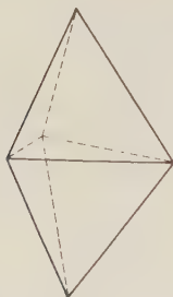
Fig. 158. Trigonal Dipyramid.
