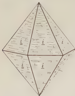
Fig. 502. Witherite.
