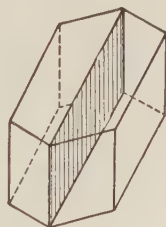
Fig. 266. Symmetry Plane.
