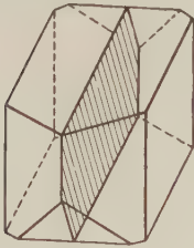
Fig. 6. Symmetry Plane.
