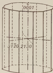
Fig. 139. Dihexagonal Prism.
