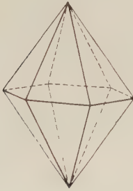
Fig. 153. Hexagonal Dipyramid.
