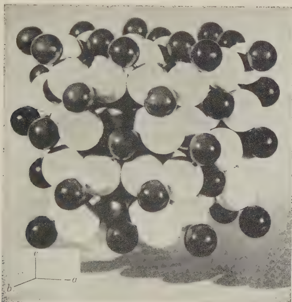
Fig. 479. Aragonite, \text{CaCO}_3 , Packing Model. Ca dark; O white; C at the center of the \text{CO}_3 triangle is not seen. Each \text{CO}_3 group lies between six calcium ions.
