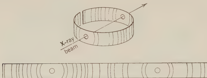
Fig. 353. X-Ray Diffraction from Powder Mount Recorded on Cylindrical Film.
