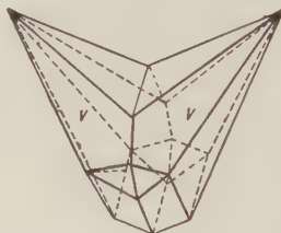
Fig. 315. Calcite Twinned on \{10\bar{1}1\} .
