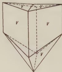
Fig. 313. Calcite Twinned on \{01\bar{1}2\} .
