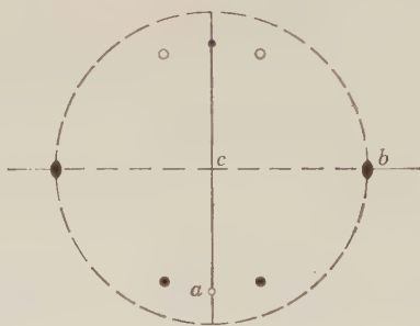
Fig. 268. Stereogram of Monoclinic Prism.
