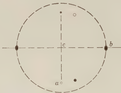
Fig. 287. Stereogram of Sphenoid.
