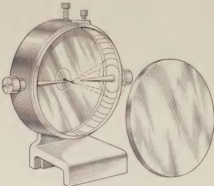
Fig. 351. Powder Camera.
