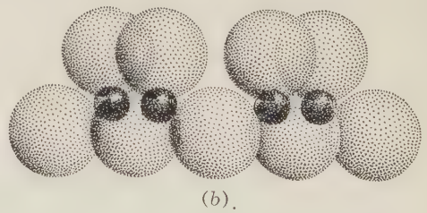
Fig. 571. \text{Si}_4\text{O}_{11} . (a) Chain; (b) Cross section.
