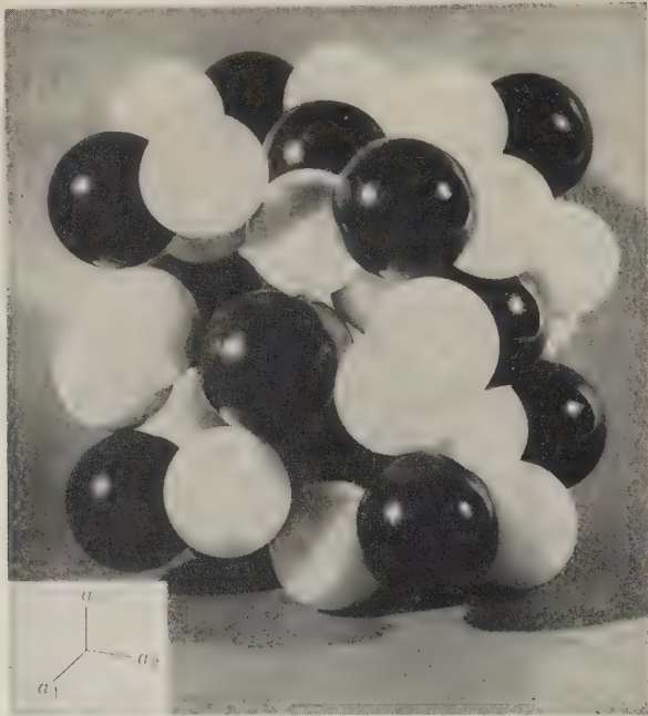
Fig. 428. Pyrite, FeS, Packing Model. Fe black; S white. Note that the sulfur pairs are aligned along the 3-fold symmetry axes.
