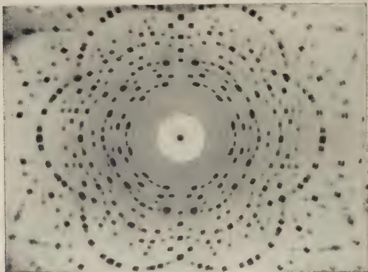
Fig. 343. Laue Photograph of Beryl.
