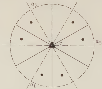
Fig. 188. Stereogram of Ditrigonal Pyramid.
