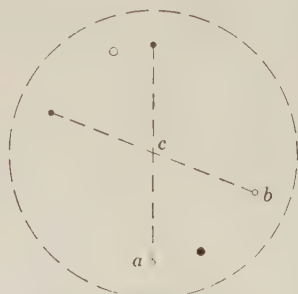
Fig. 293. Stereogram of Pinacoid.
