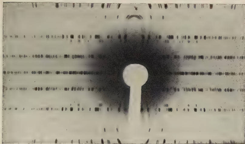
Fig. 344. Rotation Photograph of Scolecite.
