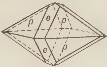
Fig. 216. Cassiterite with First- and Second-Order Dipyramids.
