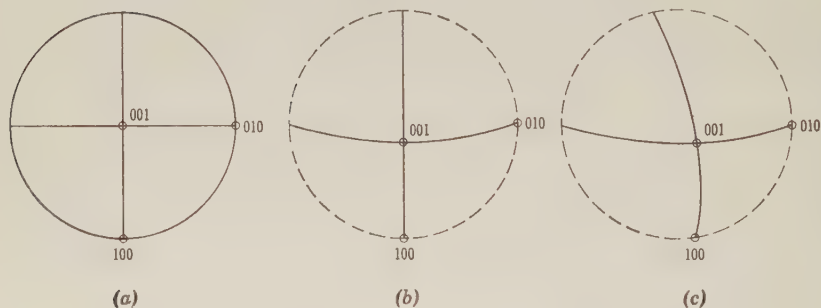
Fig. 334. (a) Orthorhombic, (b) Monoclinic, (c) Triclinic stereograms showing the relationships between the three principal zones.
