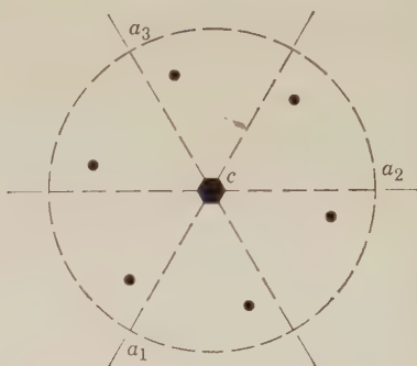
Fig. 157. Stereogram of Hexagonal Pyramid.
