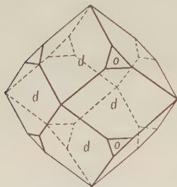
Fig. 82. Dodecahedron and Octahedron.
