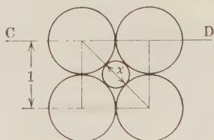
Fig. 376. Limiting Condition for Octahedral Coordination.
