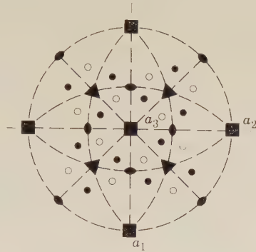
Fig. 98. Stereogram of Gyroid.
