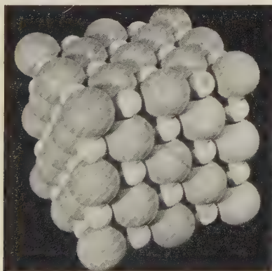
Fig. 466. Halite, \text{NaCl} , Packing Model. Na white, Cl gray.
