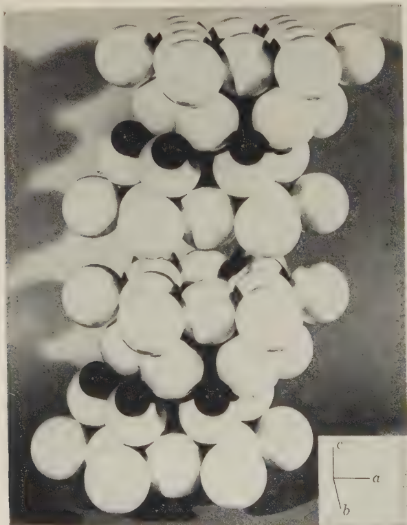
Fig. 590. Talc, \text{Mg}_3\text{Si}_4\text{O}_{10}(\text{OH})_2 , Packing Model. O white, Mg black. (OH) not visible. c axis vertical. The model shows the wide spacing between two closely packed “ t-o-t ” sheets.
