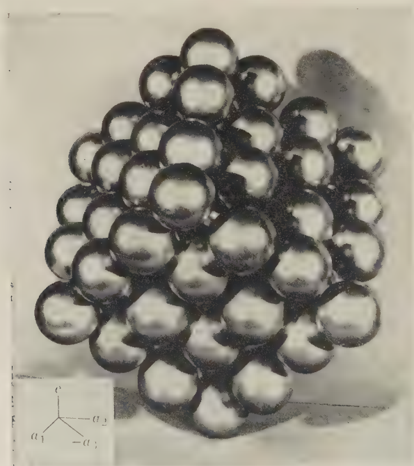
Fig. 395. Bismuth, Bi, Packing Model. The model shows the layered nature of the structure resulting from the fact that each atom is somewhat closer to three of its neighbors than to the other three.
