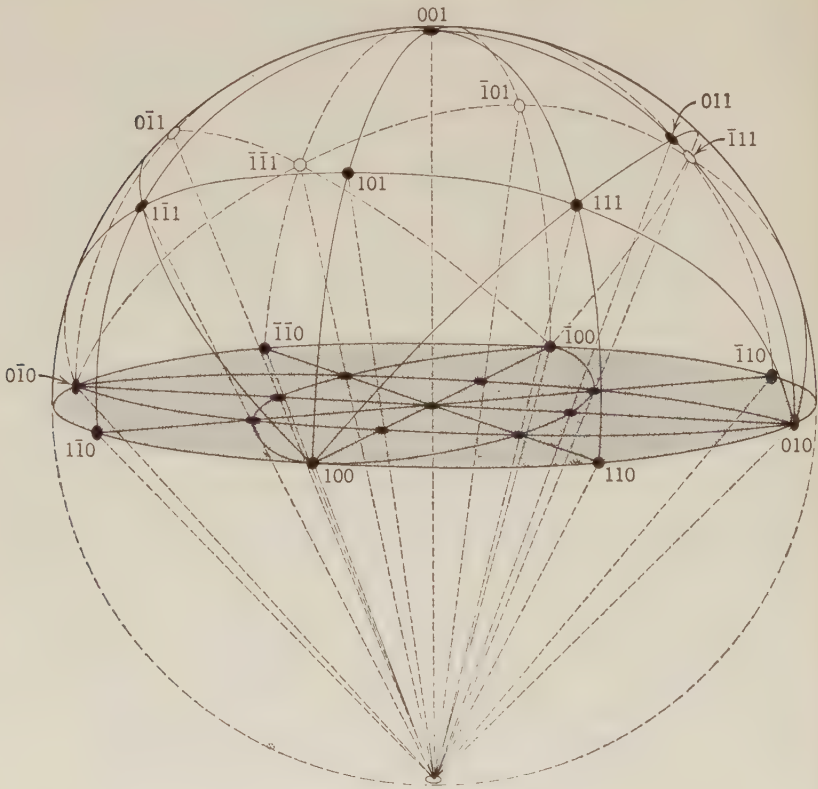
Fig. 54. Relation of Spherical and Stereographic Projections. After E. E. Wahlstrom, Optical Crystallography , John Wiley and Sons, New York, 1951.
