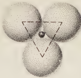
Fig. 379. Triangular Coordination of X Ions about an A Ion.
