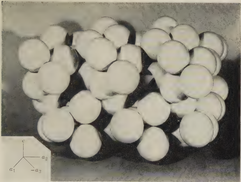
Fig. 603. High-Temperature Quartz, \text{SiO}_2 , Packing Model. c -axis vertical. As in low-temperature quartz, the \text{SiO}_4 tetrahedra are arranged in three layers but are shifted in such a way as to convert the 3-fold axis to a 6-fold axis.
