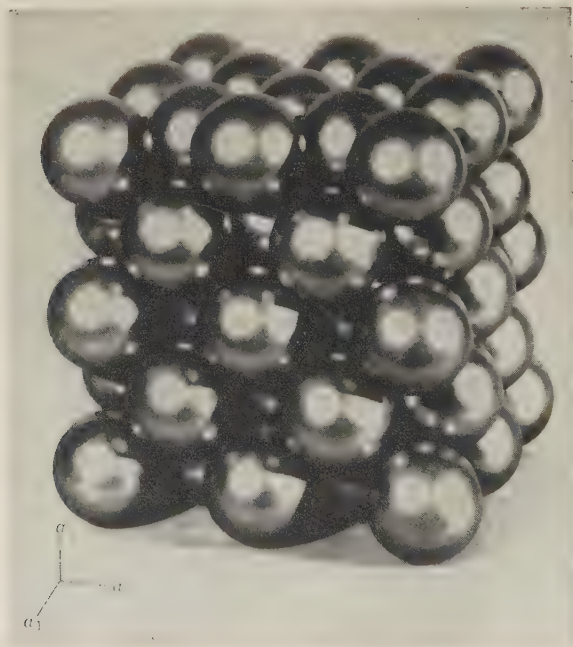
Fig. 339. Copper, Cu, Packing Model. The photograph shows copper atoms in 12-fold coordination (cubic closest packing) arranged in a face-centered cubic lattice. This structure is shared by silver, gold, and many other metals.
