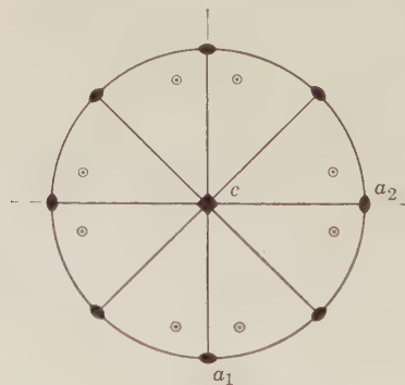
Fig. 202. Stereogram of Ditetragonal Dipyramid.
