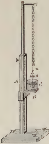
Fig. 362. Jolly Balance.
