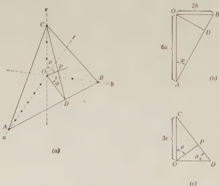
Fig. 336. Intercepts of Face (132).
