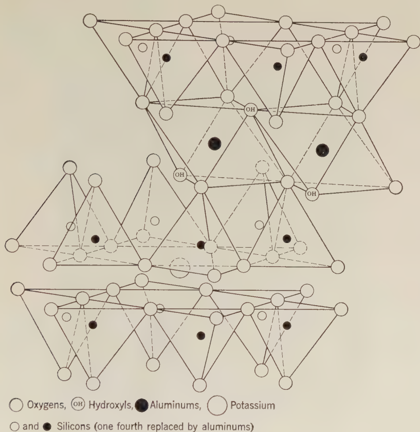
Fig. 591. Diagrammatic Sketch of the Muscovite Structure (after Grim).
