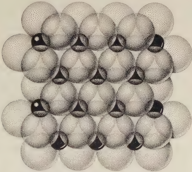
Fig. 584. Brucite Sheet. Large spheres hydroxyl, small spheres magnesium.
