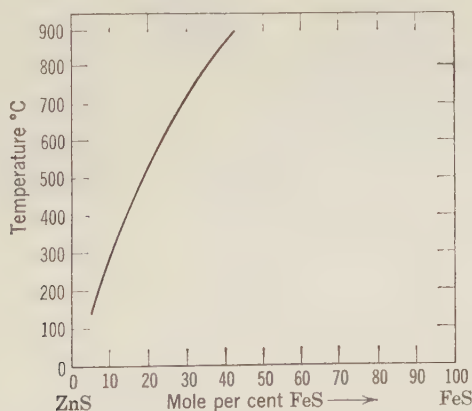
Fig. 382. Substitution of \text{Fe}^{++} for Zn in Sphalerite (after Kullerud).
