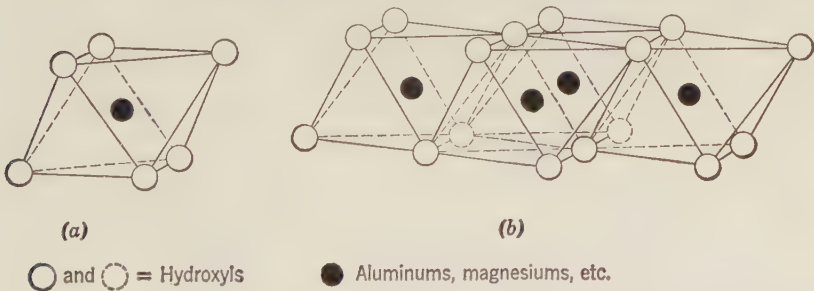
Fig. 585. Diagrammatic Sketch Showing (a) Single Octahedral Unit and (b) Sheet of Octahedral Units (after Grim).
