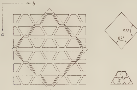
Fig. 572. Section of pyroxene structure at right angles to c axis showing how it controls cleavage (modified from Bragg).
