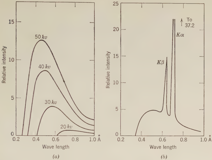
Fig. 340. X-ray Spectrum. (a) Distribution of intensity with wave length in the continuous x-ray spectrum of tungsten at various voltages. (b) Intensity curve showing characteristic wave length superimposed on the continuous x-ray spectrum of molybdenum. (After Ulrey, Phys. Rev. , 11 , 401.)
