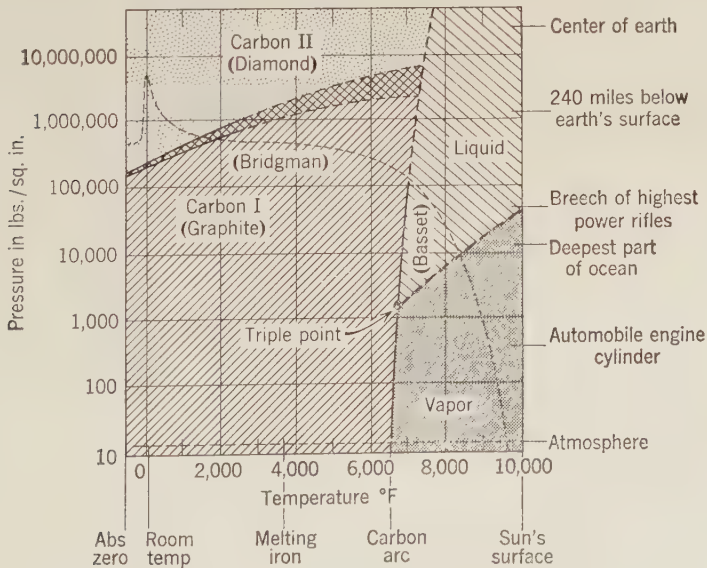
Fig. 400. Carbon Phase Diagram. ( Man-Made Diamonds , General Electric Research Laboratory, Research Information Service, 1955.)
