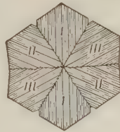
Fig. 324. Cross Section of Cyclic Aragonite Twin.
