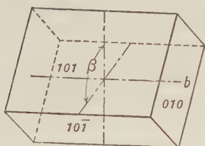
Fig. 272. Positive and Negative Second-Order Pinacoids and Side Pinacoid.
