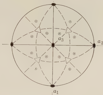
Fig. 118. Stereogram of Diploid.
