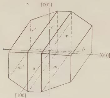
Fig. 45. Crystal Zones and Zone Axes.
