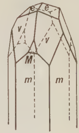
Fig. 182. Prism, Positive Scalenohedron, Positive Rhombohedron, Negative Rhombohedron.
