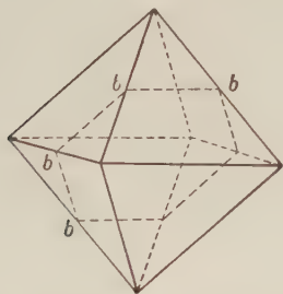
Fig. 307. Octahedron Showing Orientation of Twin Plane.
