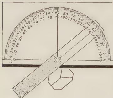
Fig. 62. Contact Goniometer.
