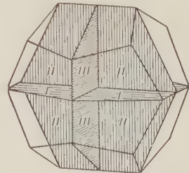
Fig. 116. Symmetry Planes.
