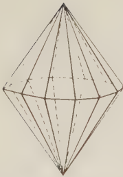
Fig. 135. Dihexagonal Dipyramid.
