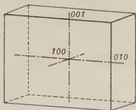
Fig. 243. Orthorhombic Pinacoids.
