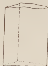
Fig. 23. Trigonal Prism.
