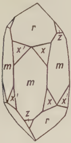
Fig. 316. Brazil Twin.
