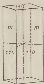
Fig. 203. First-Order Prism.
