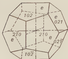
Fig. 119. Positive Pyritohedron.
