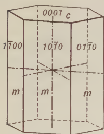
Fig. 137. First-Order Prism.
