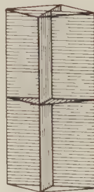
Fig. 240. Symmetry Planes.
