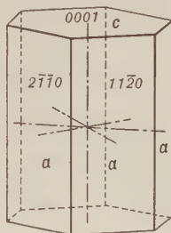
Fig. 138. Second-Order Prism.
