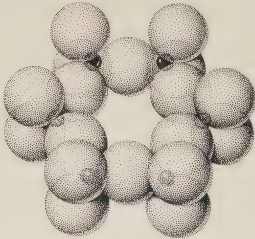
Fig. 561. \text{Si}_6\text{O}_{18} Ring.
