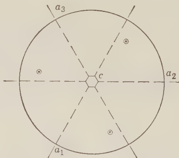
Fig. 159. Stereogram of Trigonal Dipyramid.
