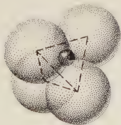
Fig. 378. Tetrahedral or 4-Fold Coordination of X Ions about an A Ion.
