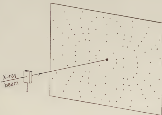
Fig. 342. Laue Photograph.
