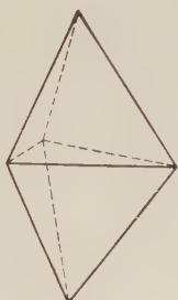
Fig. 38. Trigonal Dipyramid.
