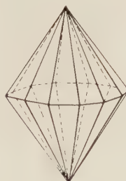
Fig. 42. Dihexagonal Dipyramid.
