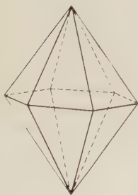
Fig. 40. Hexagonal Dipyramid.
