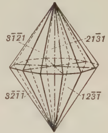
Fig. 142. Dihexagonal-Dipyramid.
