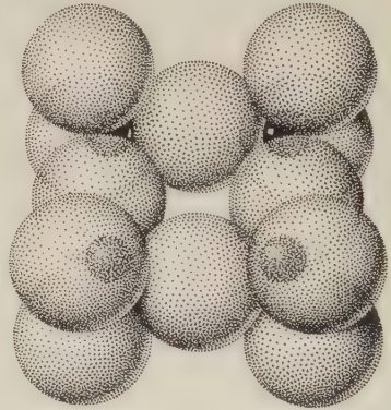
Fig. 560. \text{Si}_4\text{O}_{12} Ring.
