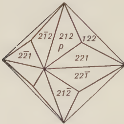
Fig. 90. Trisoctahedron.
