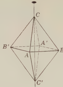
Fig. 7. Symmetry Axis.
