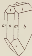
Fig. 554. Hemimorphite.
