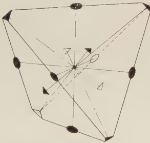
Fig. 99. Symmetry Axes.
