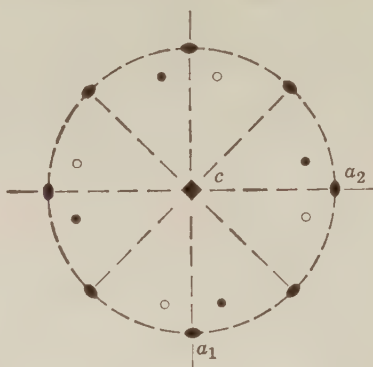
Fig. 220. Stereogram of Tetragonal Trapezohedron.
