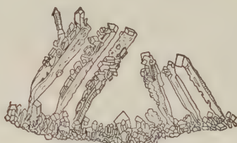
Fig. 393. Dendritic Copper.
