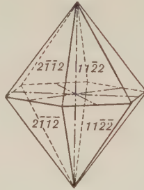
Fig. 141. Second-Order Dipyramid.
