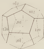
Fig. 120. Negative Pyritohedron.
