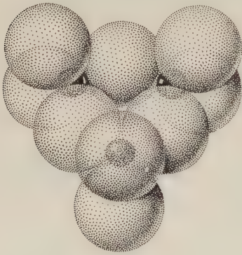
Fig. 559. \text{Si}_3\text{O}_9 Ring.
