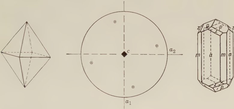
Fig. 230. Tetragonal Dipyramid.
