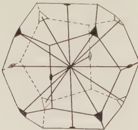
Fig. 115. Symmetry Axes.
