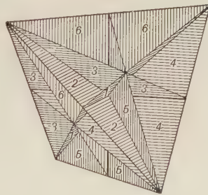
Fig. 100. Symmetry Planes.
