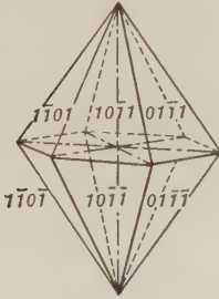
Fig. 140. First-Order Dipyramid.
