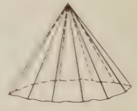
Fig. 32. Dihexagonal Pyramid.
