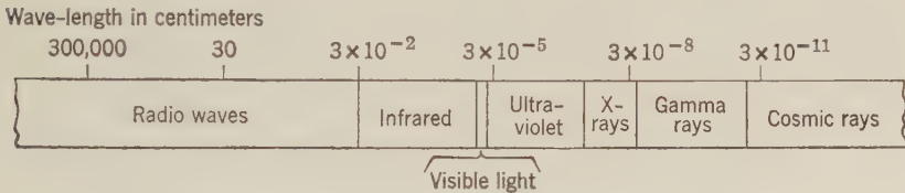
Fig. 339. The Electromagnetic Spectrum.
