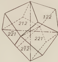
Fig. 108. Deltoid Dodecahedron.
