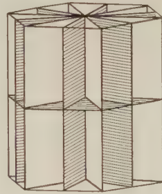
Fig. 134. Symmetry Planes.
