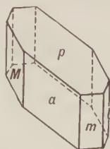
Fig. 302. Chalcanthite.
