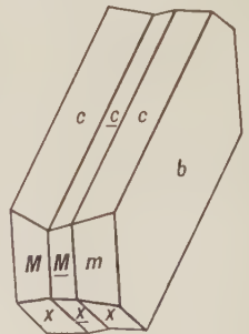
Fig. 332. Albite Twinning.
