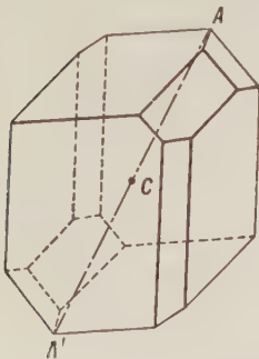
Fig. 8. Symmetry Center.
