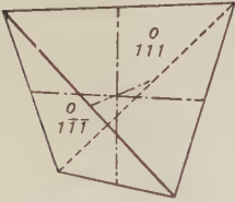
Fig. 104. Positive Tetrahedron.
