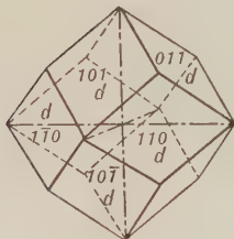
Fig. 79. Dodecahedron.
