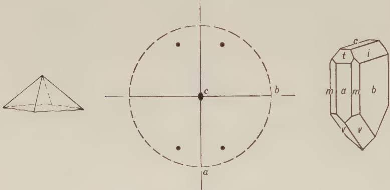
Fig. 261. Rhombic Pyramid.
