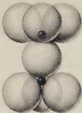
Fig. 553. \text{Si}_2\text{O}_7 Group.
