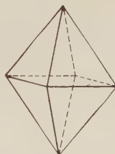
Fig. 39. Tetragonal Dipyramid.
