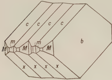
Fig. 303. Albite Twins.
