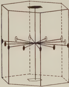
Fig. 133. Symmetry Axes.
