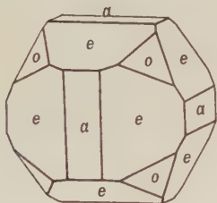
Fig. 127. Pyritohedron, Cube,
