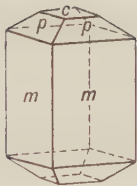
Fig. 213. Idocrase with First-Order Prism, First-Order Dipyramid, Basal Pinacoid.
