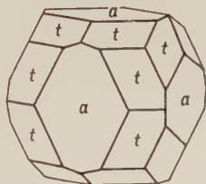
Fig. 128. Diploid and Cube and Octahedron.
