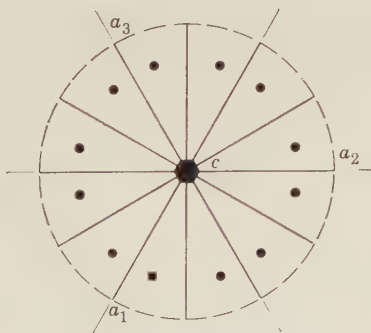
Fig. 149. Stereogram of Dihexagonal Pyramid.
