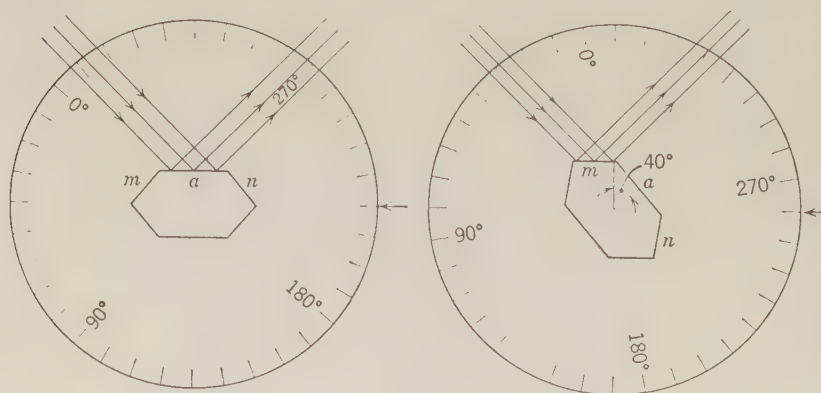
Fig. 61. Angular Measurement by Reflecting Goniometer.
