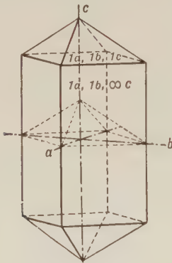
Fig. 14. Prism and Dipyramid.
