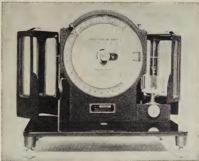
Fig. 364. Berman Balance.
