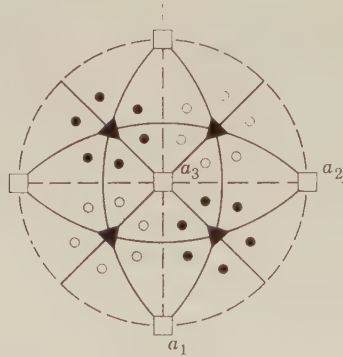
Fig. 102. Stereogram of Hextetrahedron.
