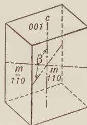
Fig. 274. Third-Order Prism and Basal Pinacoid.
