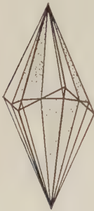
Fig. 176. Relation between Dihexagonal Dipyramid and Scalenohedron.
