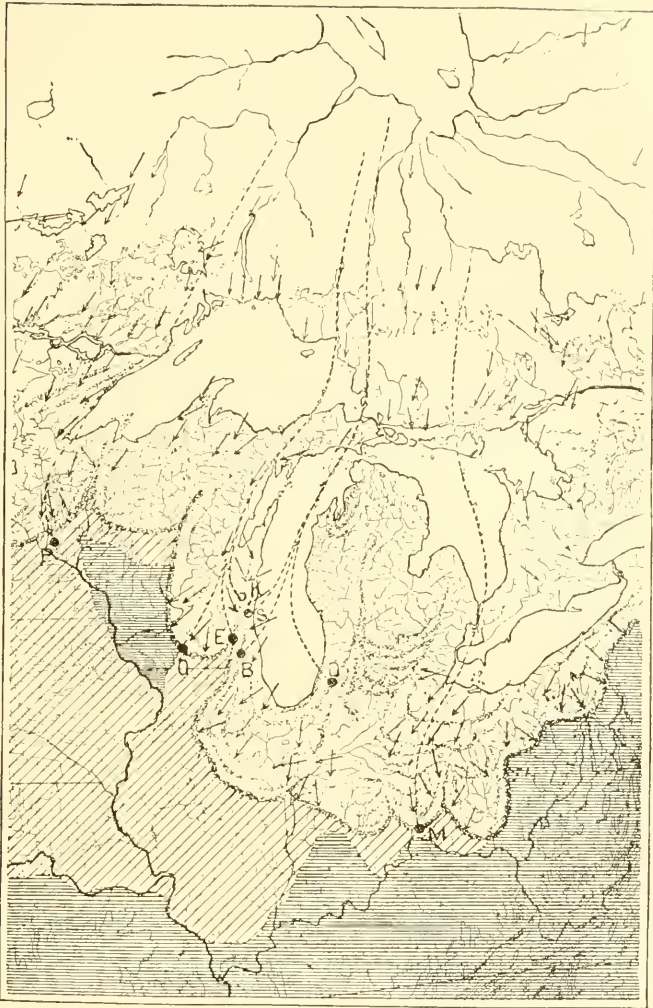
GLACIAL MAP OF THE GREAT LAKES REGION.
