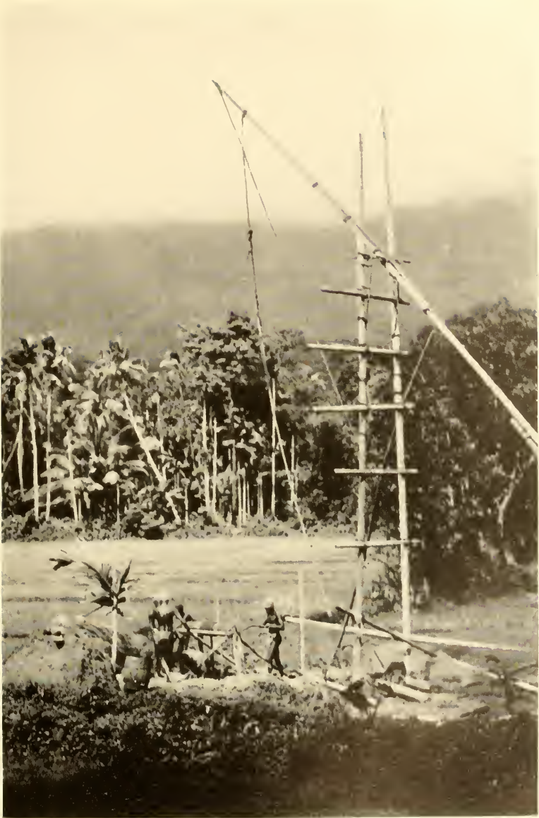
Singhalese sinking a shaft for sapphires, Palmadulla, Ceylon. (Photo by F. D. Adams)
