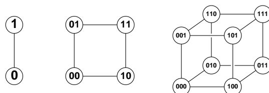
The 1-dimensional, 2-dimensional, and 3-dimensional hypercubes.
