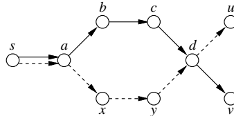
If s \rightarrow a \rightarrow b \rightarrow c \rightarrow d \rightarrow v and s \rightarrow a \rightarrow x \rightarrow y \rightarrow d \rightarrow u are shortest paths, then s \rightarrow a \rightarrow b \rightarrow c \rightarrow d \rightarrow u is also a shortest path.
