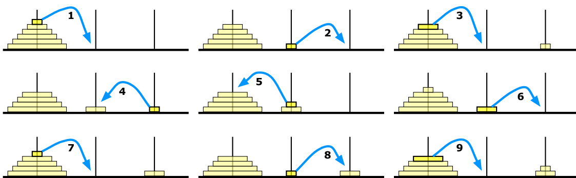
The first nine moves in a restricted Towers of Hanoi solution.
