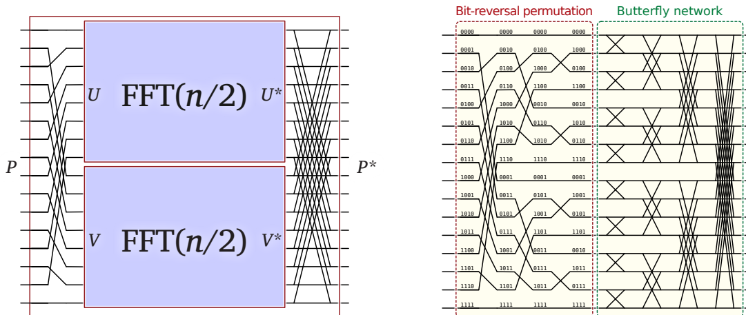
The recursive structure of the FFT algorithm.
