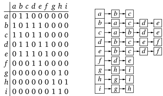
Adjacency matrix and adjacency list representations for the example graph.
