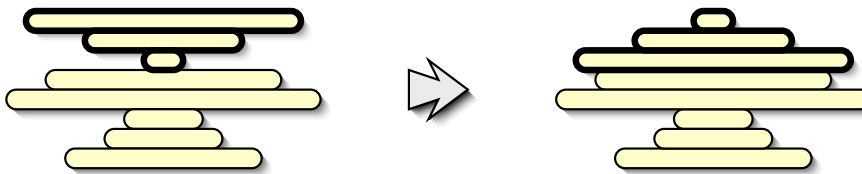
Flipping the top three pancakes.
