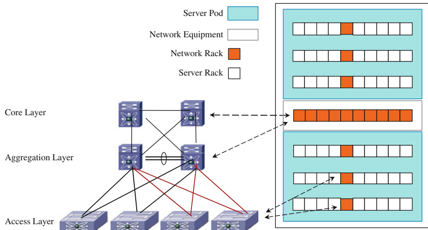
Fig. 4.2 Data center network architecture
