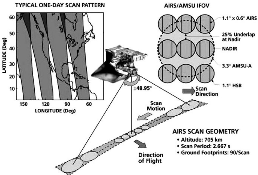
Fig. 16.3 Geo-Reprojection
