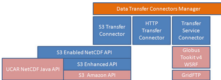
Fig. 26.6 The NetCDF service transfer connector architecture
